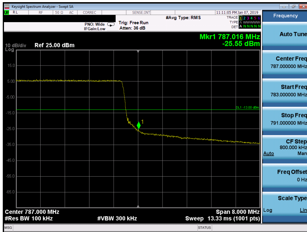
Plot 7-184. Upper Band Edge Plot (Band 13 -10.0MHz QPSK - Full RB Configuration)
