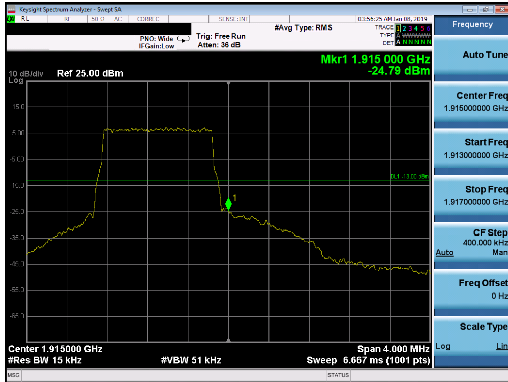
Plot 7-251. Upper Band Edge Plot (Band 25 - 1.4MHz QPSK - Full RB Configuration)
