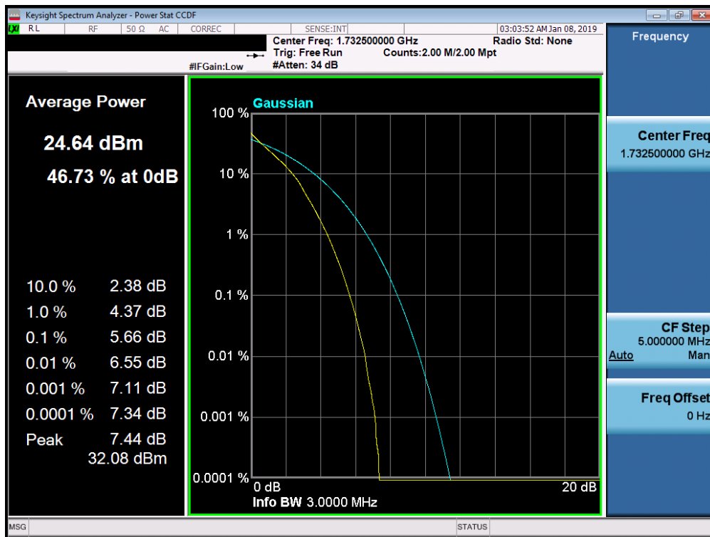
Plot 7-316. PAR Plot (Band 4 - 3.0MHz QPSK - Full RB Configuration)
