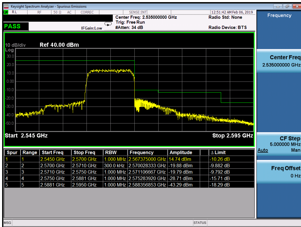
Plot 7-308. Upper ACP Plot (Band 7 - 10.0MHz QPSK - Full RB Configuration)
