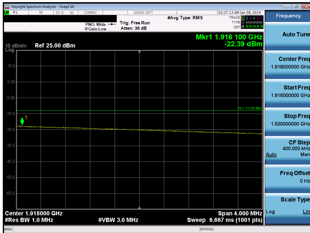
Plot 7-272. Upper Extended Band Edge Plot (Band 25 - 20.0MHz QPSK - Full RB Configuration)
