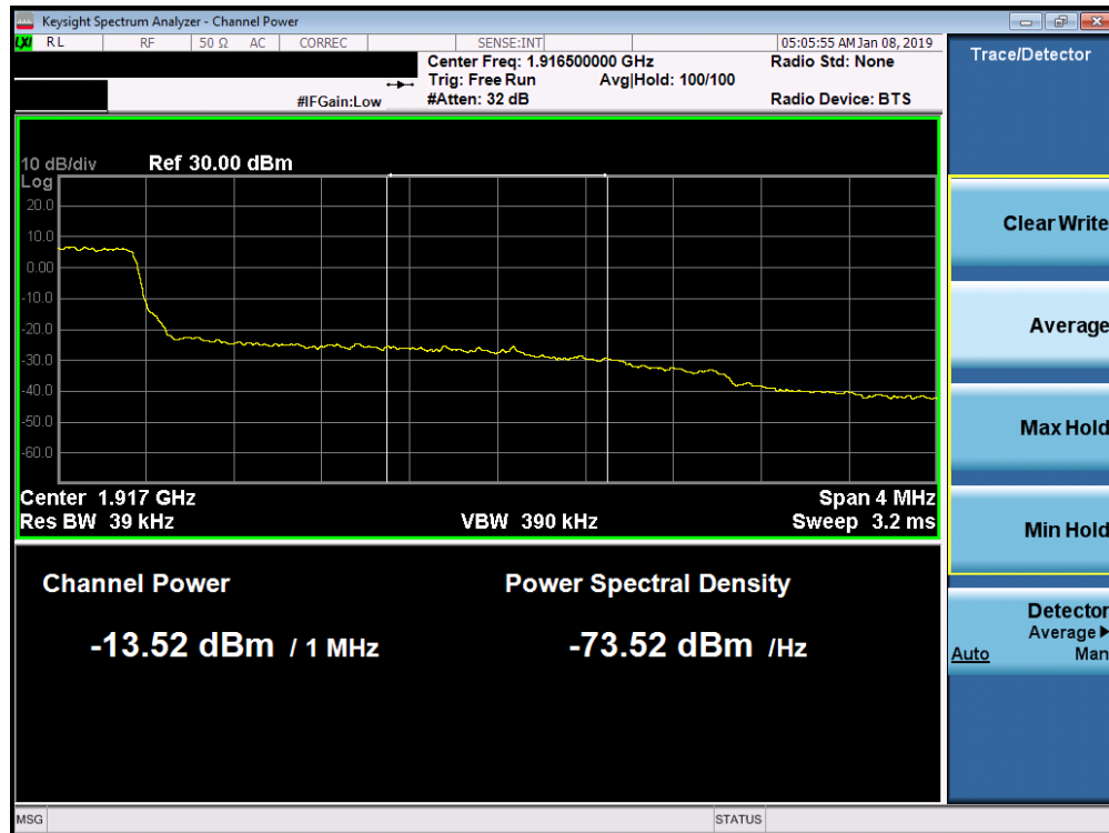
Plot 7-256. Upper Extended Band Edge Plot (Band 25 - 3.0MHz QPSK - Full RB Configuration)
