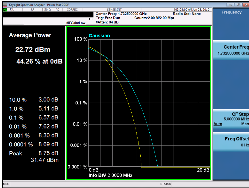
Plot 7-315. PAR Plot (Band 4 - 1.4MHz 64-QAM - Full RB Configuration)
