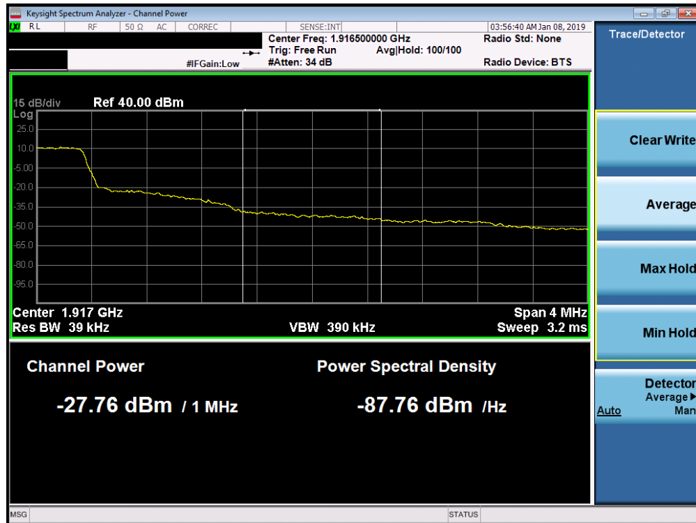
Plot 7-252. Upper Extended Band Edge Plot (Band 25 - 1.4MHz QPSK - Full RB Configuration)
