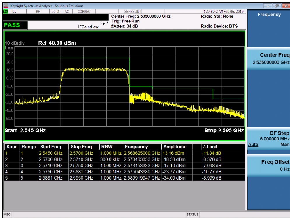
Plot 7-310. Upper ACP Plot (Band 7 - 15.0MHz QPSK - Full RB Configuration)
