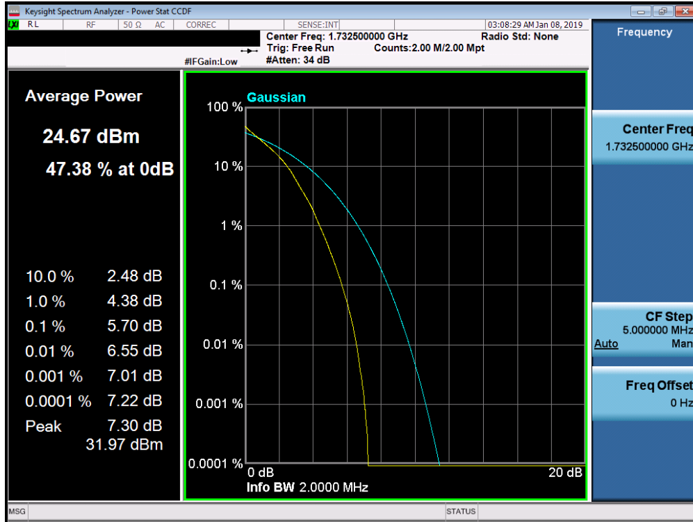
Plot 7-313. PAR Plot (Band 4 - 1.4MHz QPSK - Full RB Configuration)
