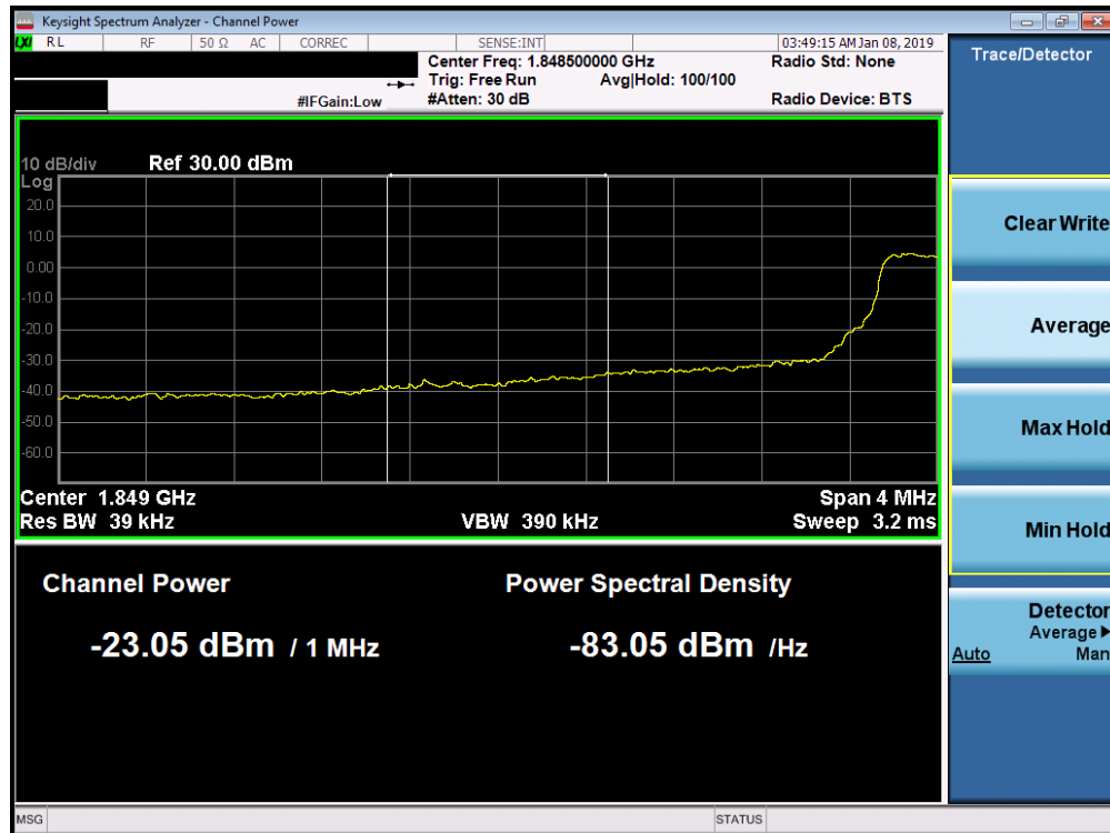
Plot 7-258. Lower Extended Band Edge Plot (Band 25 - 5.0MHz QPSK - Full RB Configuration)
