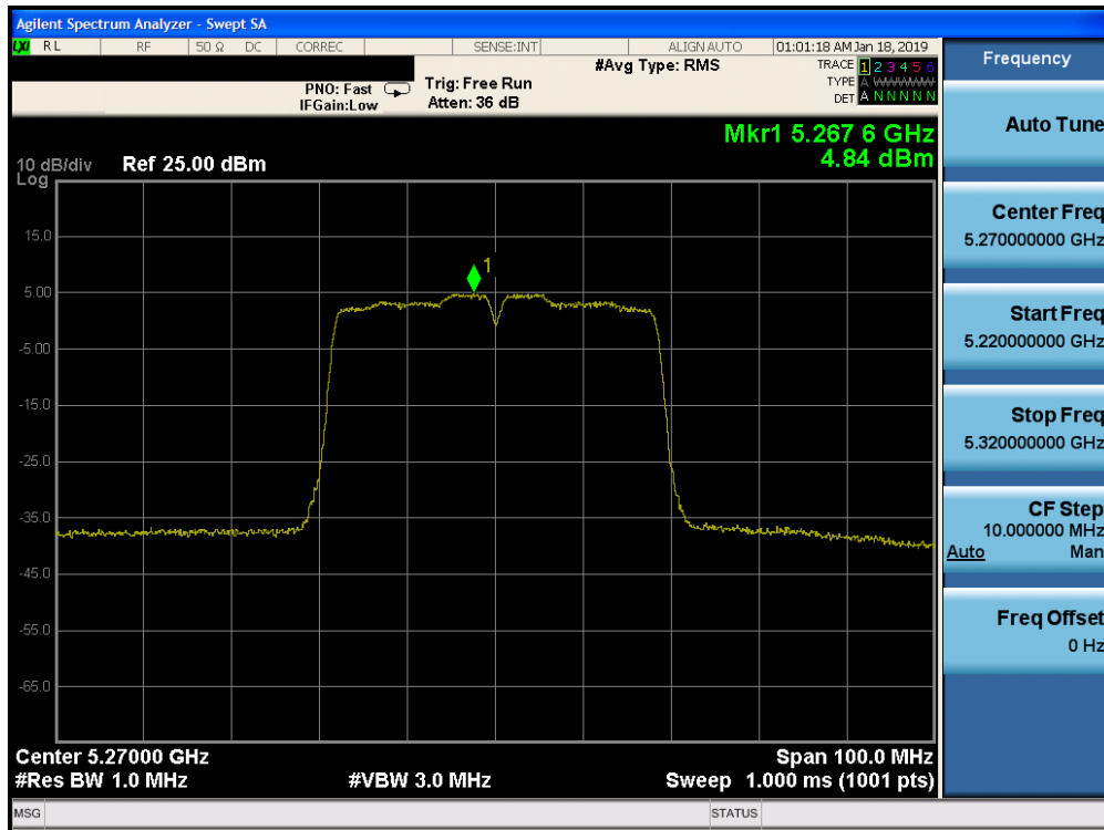
Plot 7-136. Power Spectral Density Plot MIMO/CDD CORE0 (40MHz BW 802.11n (UNII Band 2A) – Ch. 54)
