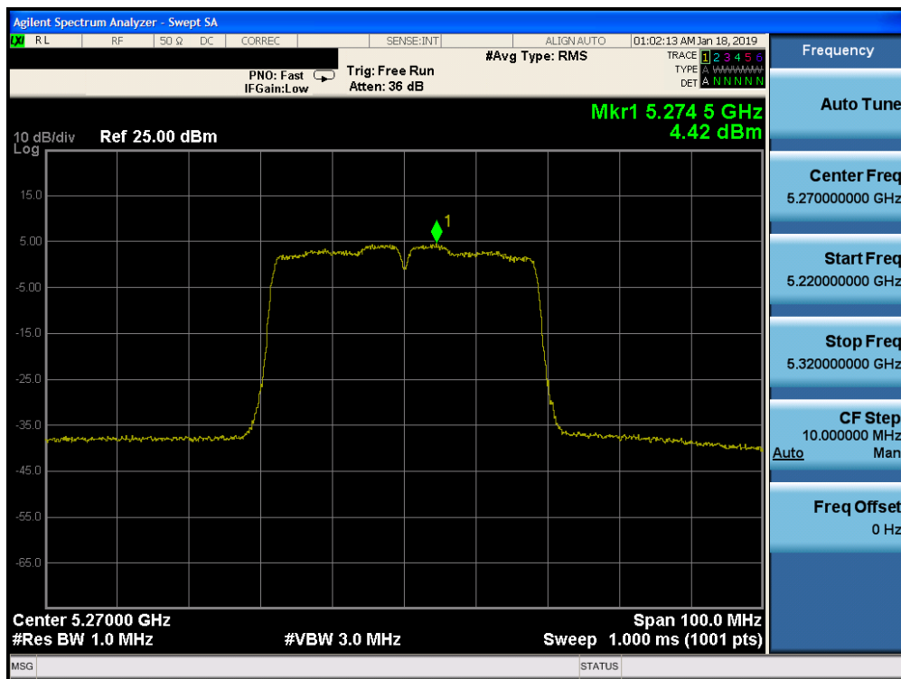
Plot 7-137. Power Spectral Density Plot MIMO/CDD CORE1 (40MHz BW 802.11n (UNII Band 2A) – Ch. 54)
