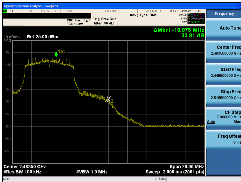
Plot 7-70. Band Edge Plot SISO CORE 1 (802.11n – Ch. 11)
