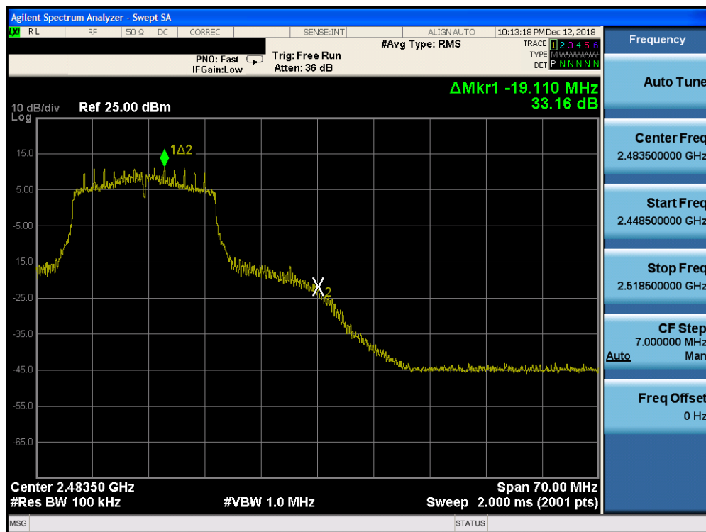
Plot 7-58. Band Edge Plot SISO CORE 0 (802.11n – Ch. 11)
