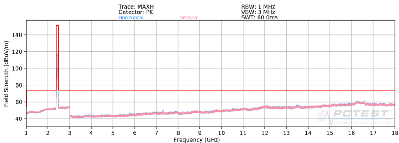
Plot 7-92. Radiated Spurious Plot above 1GHz CDD (802.11n – Ch. 6)
