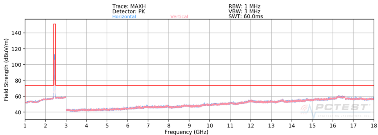
Plot 7-86. Radiated Spurious Plot above 1GHz SISO CORE 0 (802.11b – Ch. 6)
