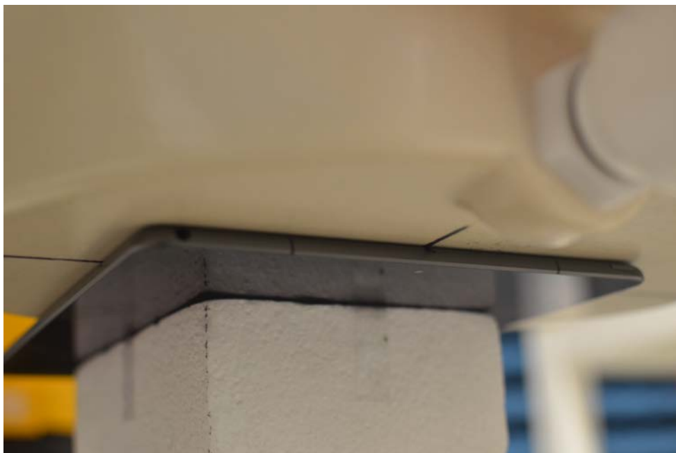
SAR Test Setup Photo 1: Back Side at 0.0 cm – ANTWF3/WF5
