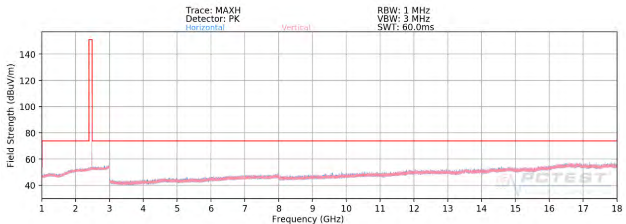
Plot 7-93. Radiated Spurious Plot Above 1GHz ANT 2 (1Mbps, ePA – Ch. 39)
