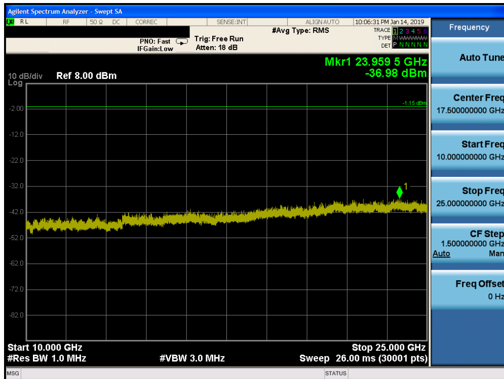
Plot 7-80. Conducted Spurious Plot ANT 1 (Bluetooth, GFSK, ePA – Ch. 0)
