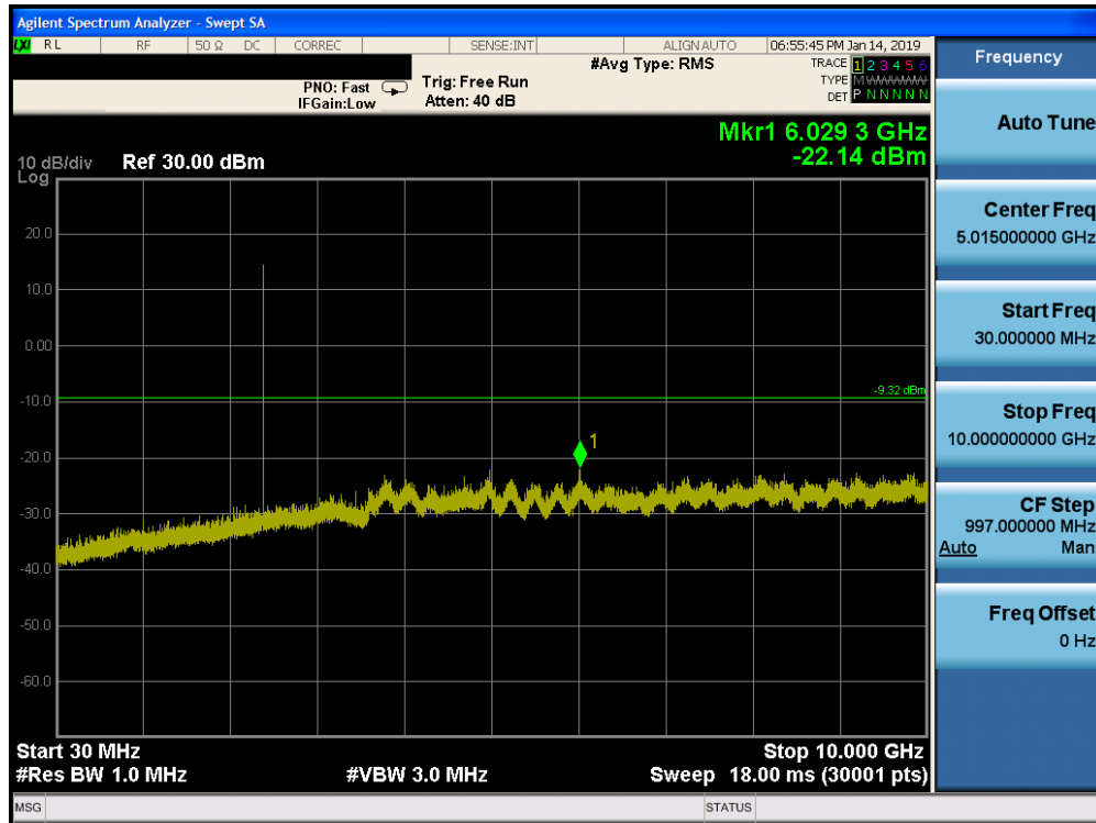
Plot 7-73. Conducted Spurious Plot ANT 0 (Bluetooth, 8DPSK, ePA – Ch. 0)
