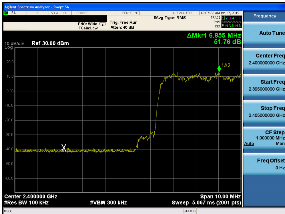
Plot 7-33. Band Edge Plot ANT 1 (Bluetooth with Hopping Enabled, 8DPSK, ePA)
