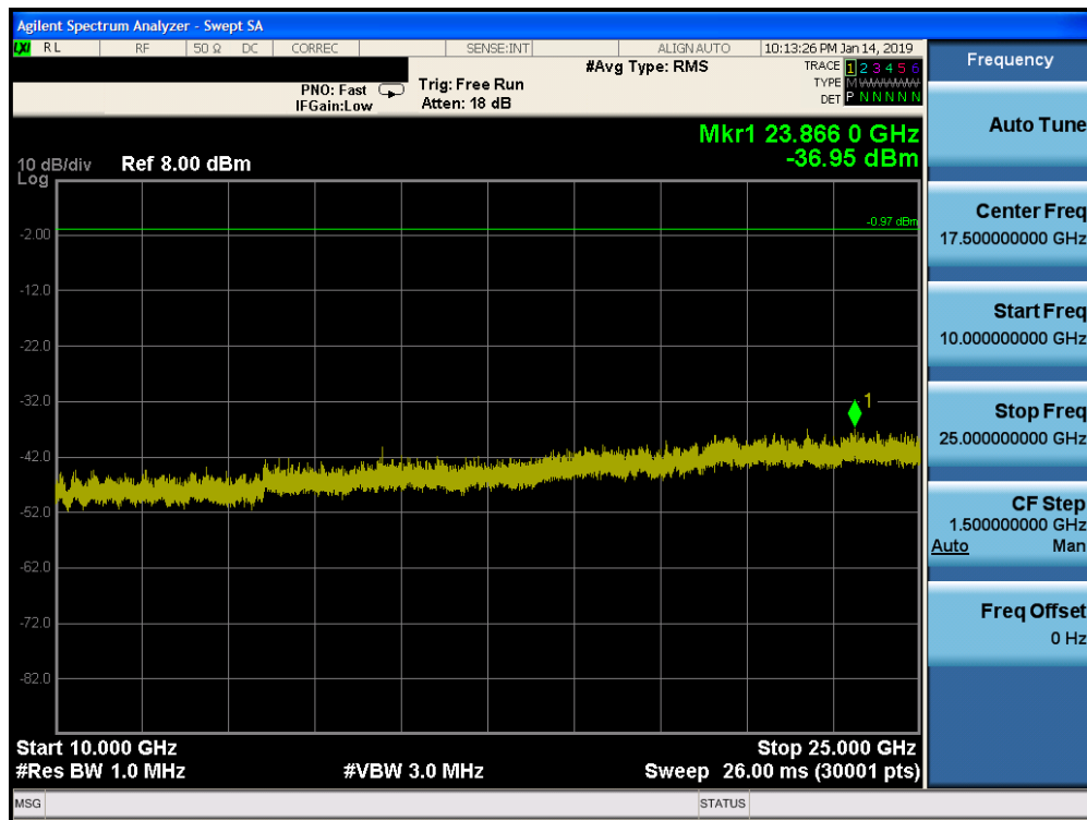
Plot 7-82. Conducted Spurious Plot ANT 1 (Bluetooth, GFSK, ePA Ch. 39)
