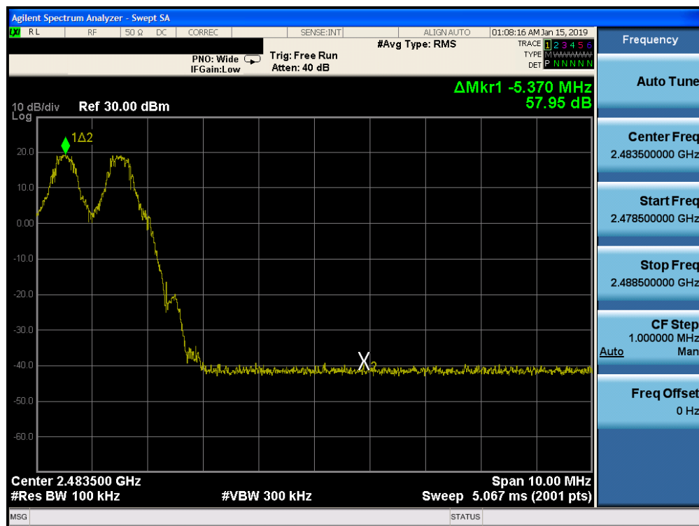
Plot 7-22. Band Edge Plot ANT 0 (Bluetooth with Hopping Enabled, GFSK, ePA)
