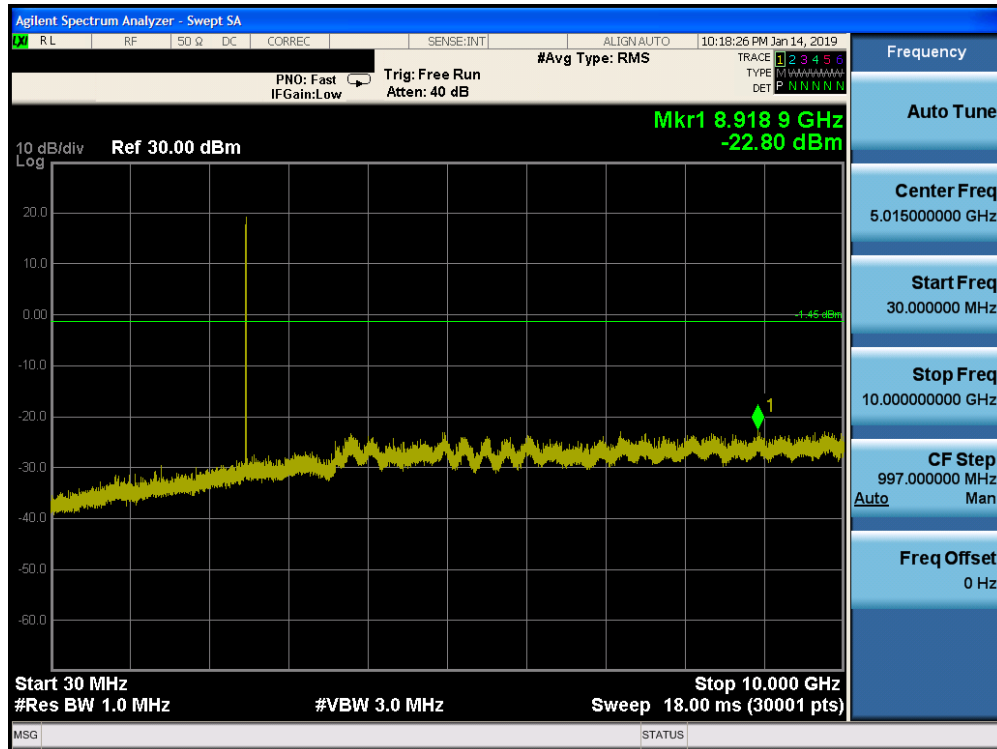
Plot 7-83. Conducted Spurious Plot ANT 1 (Bluetooth, GFSK, ePA – Ch. 78)
