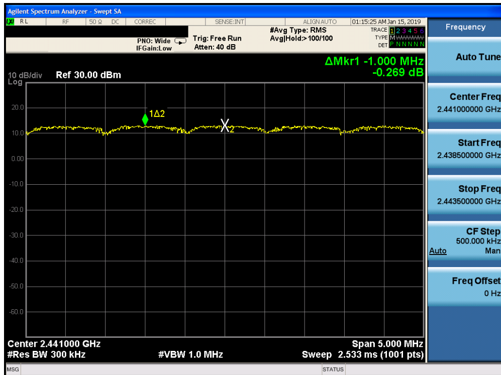
Plot 7-44. Channel Spacing Plot ANT 0 (Bluetooth, 8DPSK, ePA)
