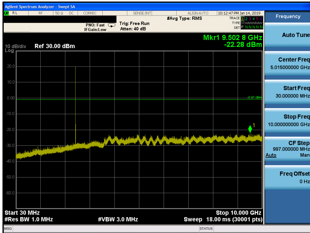
Plot 7-81. Conducted Spurious Plot ANT 1 (Bluetooth, GFSK, ePA – Ch. 39)
