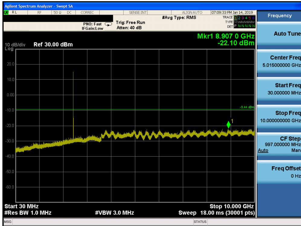
Plot 7-75. Conducted Spurious Plot ANT 0 (Bluetooth, 8DPSK, ePA – Ch. 39)
