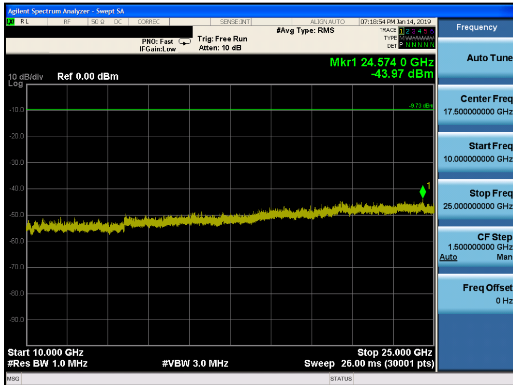
Plot 7-78. Conducted Spurious Plot ANT 0 (Bluetooth, 8DPSK, ePA – Ch. 78)
