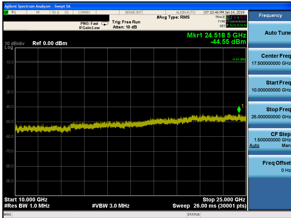
Plot 7-76. Conducted Spurious Plot ANT 0 (Bluetooth, 8DPSK, ePA Ch. 39)
