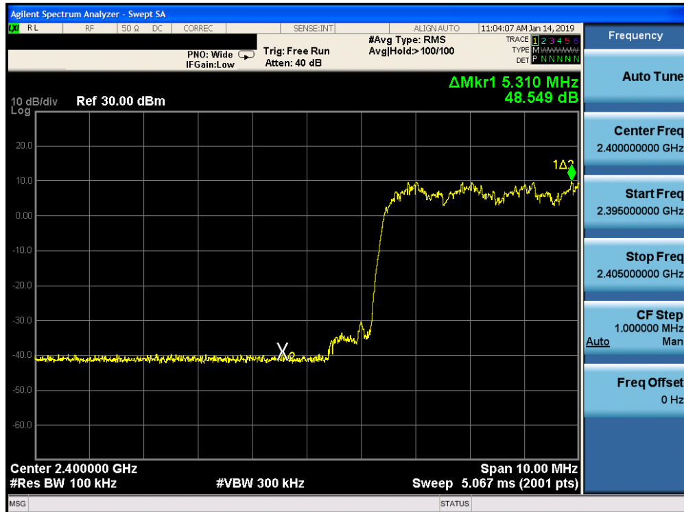
Plot 7-41. Band Edge Plot ANT 2 (Bluetooth with Hopping Enabled, 8DPSK, ePA)
