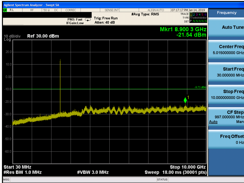
Plot 7-77. Conducted Spurious Plot ANT 0 (Bluetooth, 8DPSK, ePA – Ch. 78)
