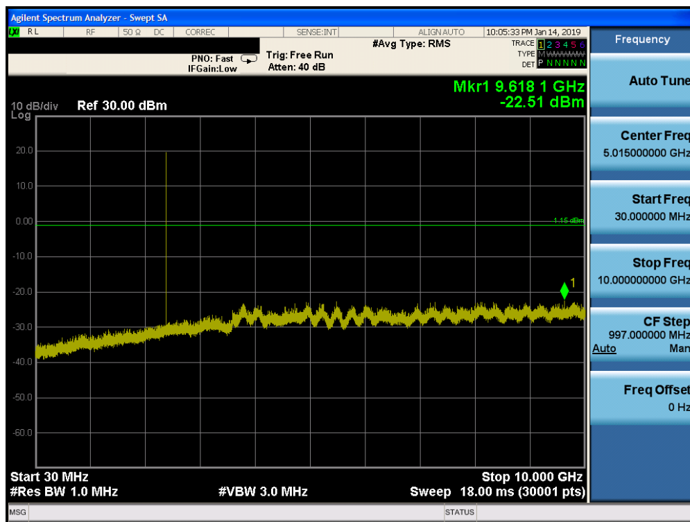
Plot 7-79. Conducted Spurious Plot ANT 1 (Bluetooth, GFSK, ePA – Ch. 0)
