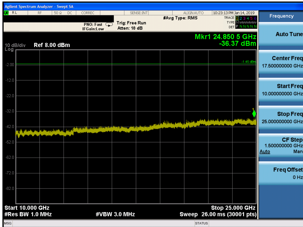
Plot 7-84. Conducted Spurious Plot ANT 1 (Bluetooth, GFSK, ePA – Ch. 78)
