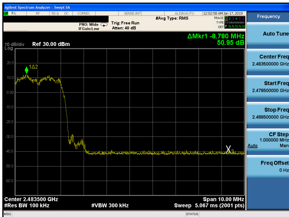
Plot 7-34. Band Edge Plot ANT 1 (Bluetooth with Hopping Enabled, 8DPSK, ePA)
