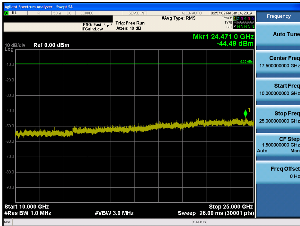
Plot 7-74. Conducted Spurious Plot ANT 0 (Bluetooth, 8DPSK, ePA – Ch. 0)
