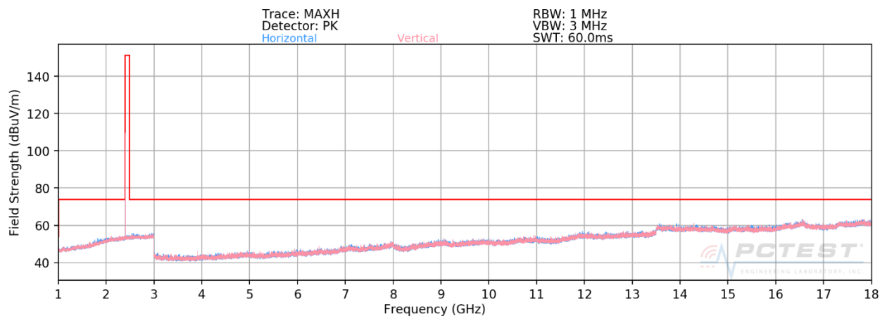
Plot 7-103. Radiated Spurious Plot above 1GHz ANT 0 (BT GFSK ePA – Ch. 0)
