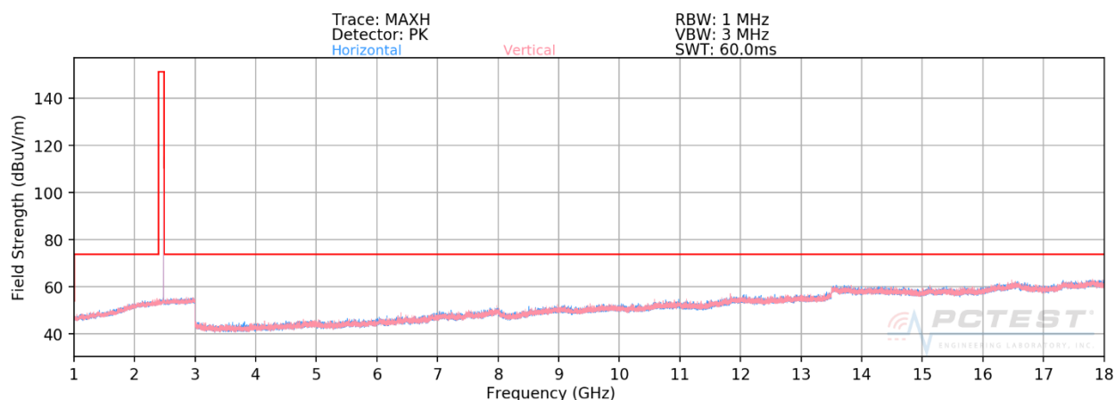
Plot 7-105. Radiated Spurious Plot above 1GHz ANT 0 (BT GFSK ePA – Ch. 78)
