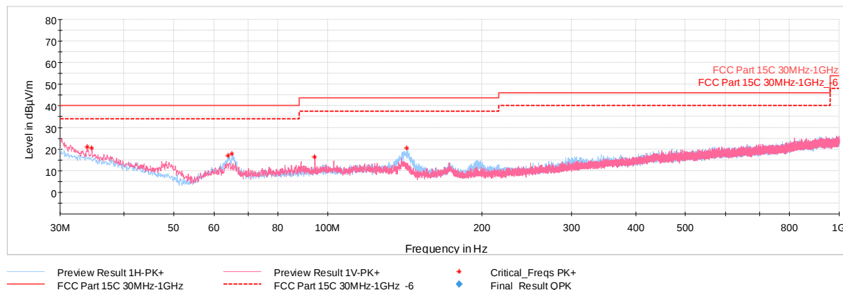
Plot 7-130. Radiated Spurious Plot below 1GHz (2.4GHz – 5GHz), with AC/DC Adapter
