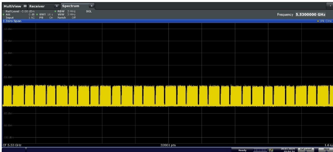
Figure 9-17. 5530MHz - Channel Loading - Mode 3 (80MHz)
