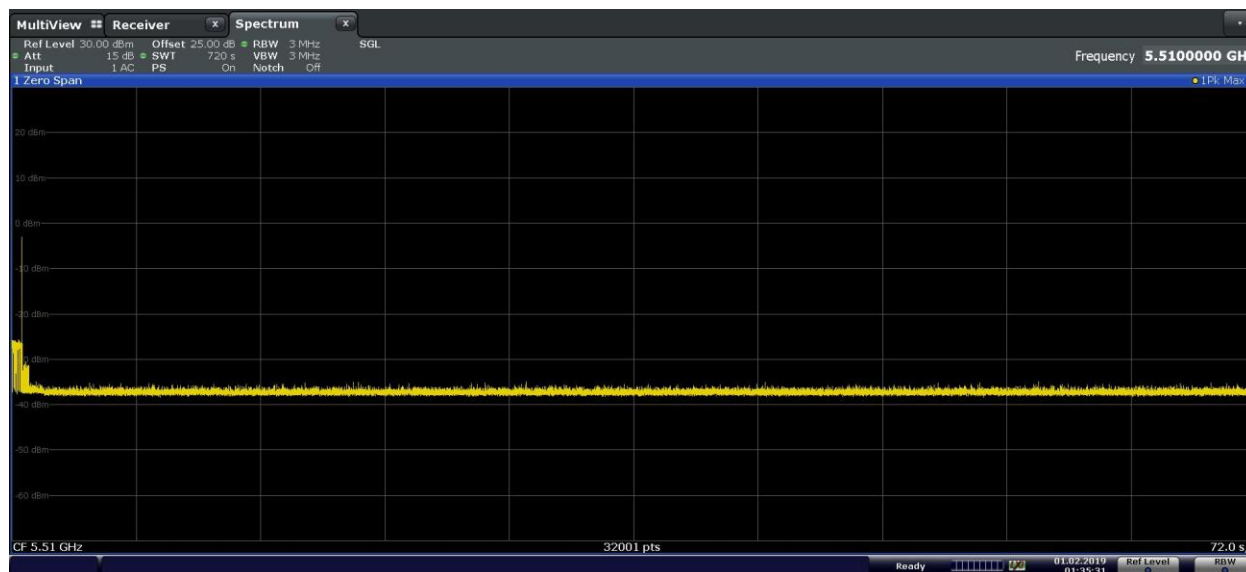
Figure 9-41. 5510MHz - Non-Occupancy Period (10 Minutes) - Mode 2 (40MHz)
