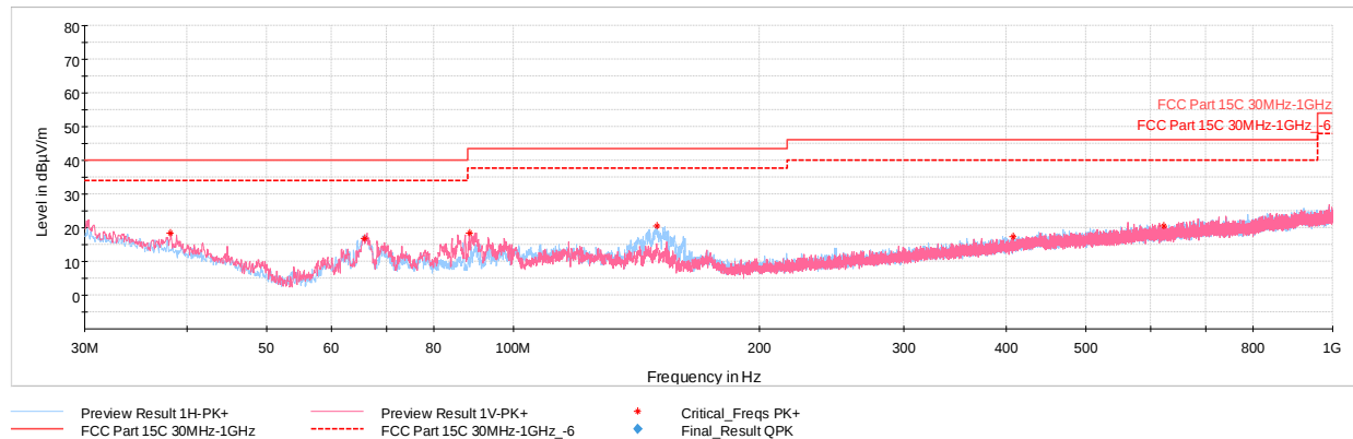
Plot 7-270. Radiated Spurious Plot below 1GHz MIMO/CDD – Ch.36, with AC/DC Adapter
