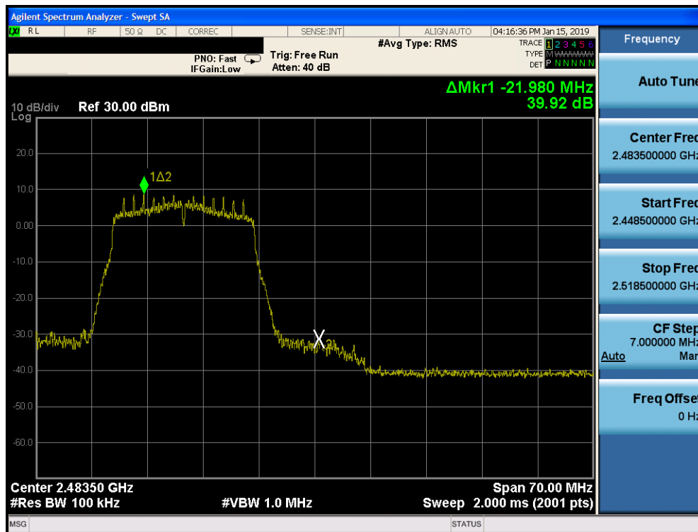
Plot 7-113. Band Edge Plot SISO CORE 1 (802.11n – Ch. 12)
