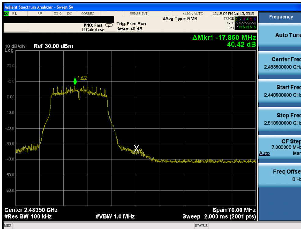
Plot 7-97. Band Edge Plot SISO CORE 0 DIVERSITY (802.11g – Ch. 12)
