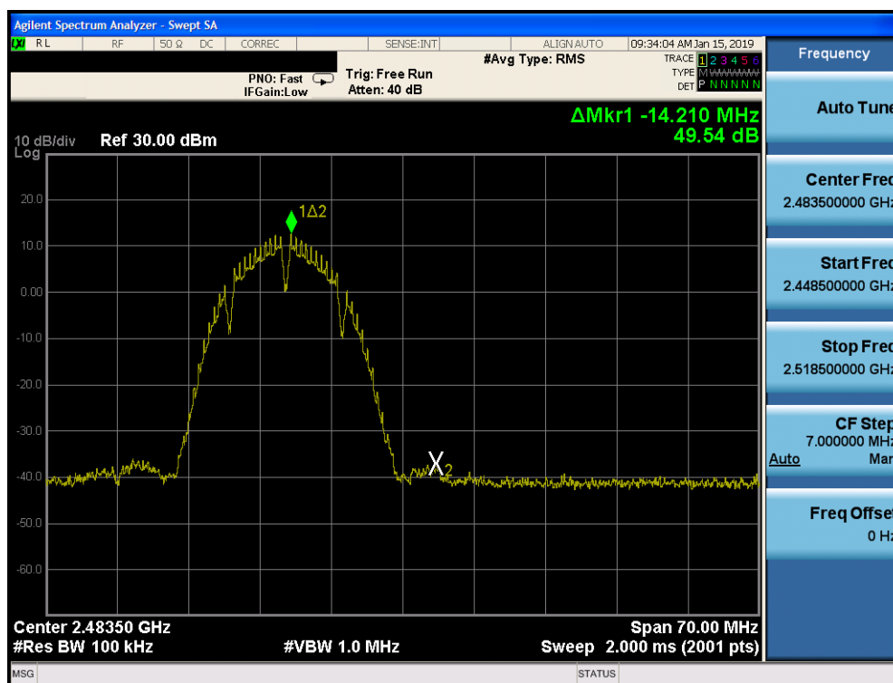
Plot 7-82. Band Edge Plot SISO CORE 0 PRIMARY (802.11b – Ch. 13)
