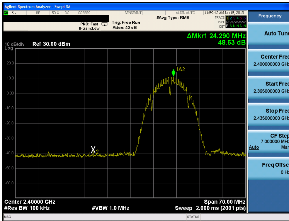
Plot 7-91. Band Edge Plot SISO CORE 0 DIVERSITY (802.11b – Ch. 1)
