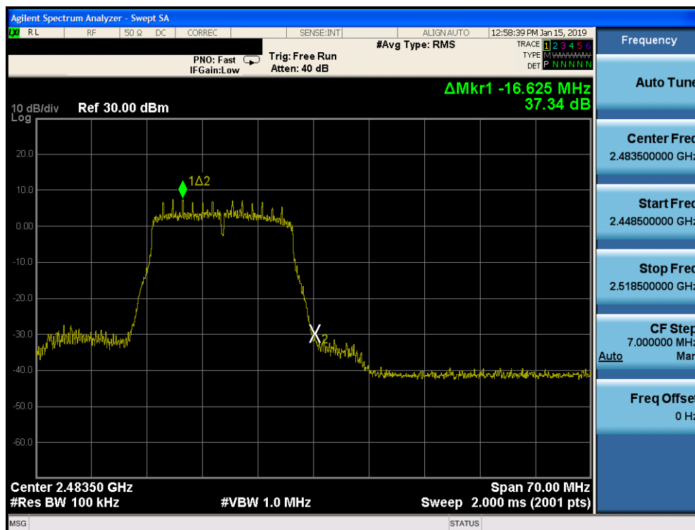
Plot 7-102. Band Edge Plot SISO CORE 0 DIVERSITY (802.11n – Ch. 13)
