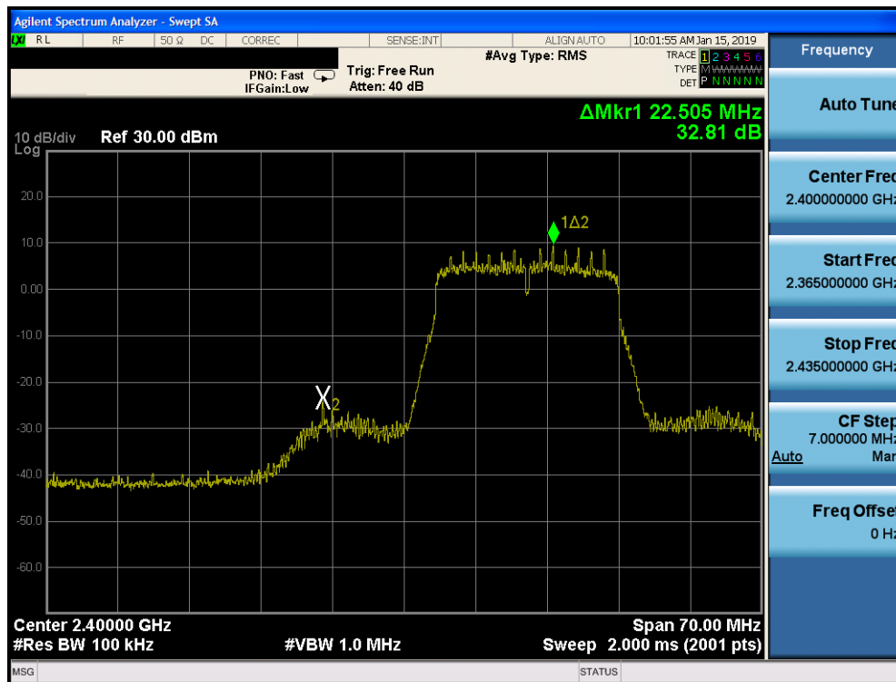
Plot 7-87. Band Edge Plot SISO CORE 0 PRIMARY (802.11n (2.4GHz) – Ch. 1)
