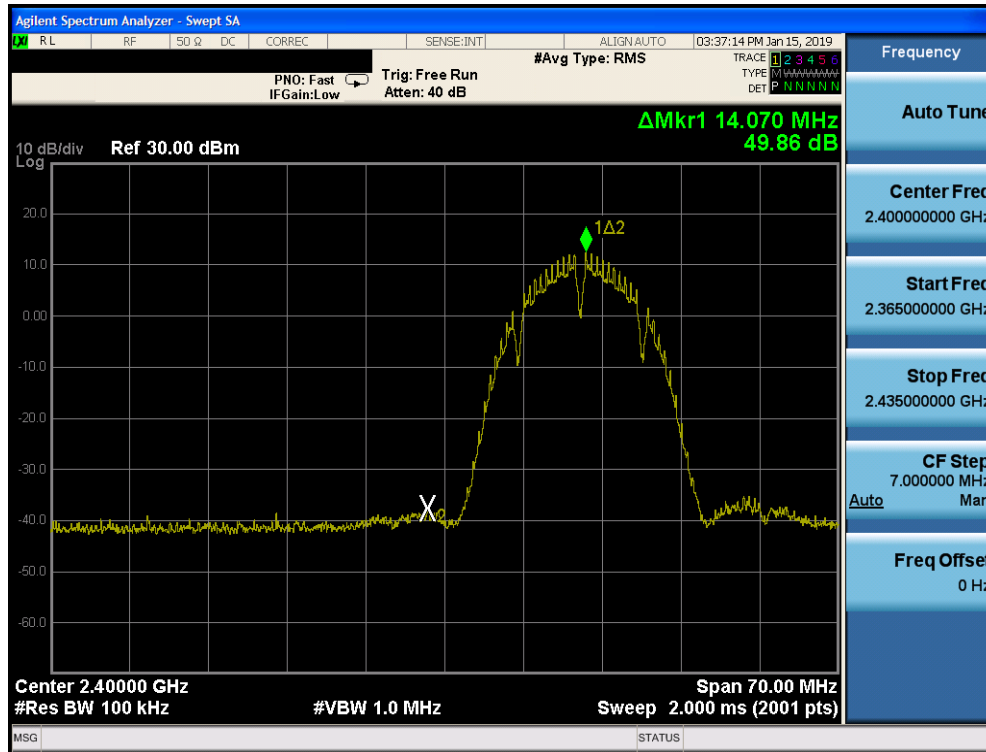
Plot 7-103. Band Edge Plot SISO CORE 1 (802.11b – Ch. 1)
