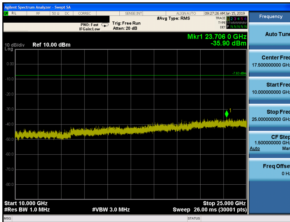
Plot 7-118. Conducted Spurious Plot SISO CORE 0 PRIMARY (802.11b – Ch. 6)
