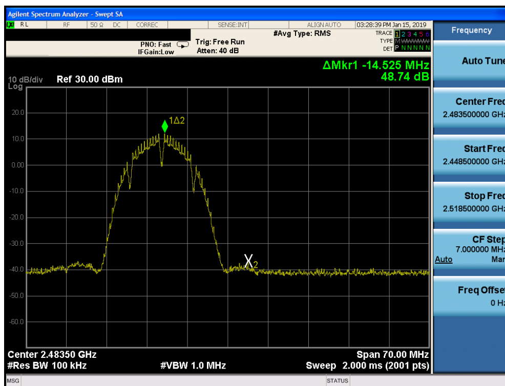
Plot 7-106. Band Edge Plot SISO CORE 1 (802.11b - Ch. 13)
