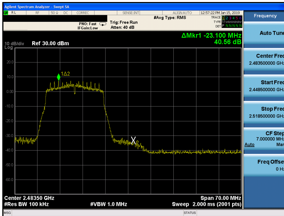
Plot 7-101. Band Edge Plot SISO CORE 0 DIVERSITY (802.11n – Ch. 12)
