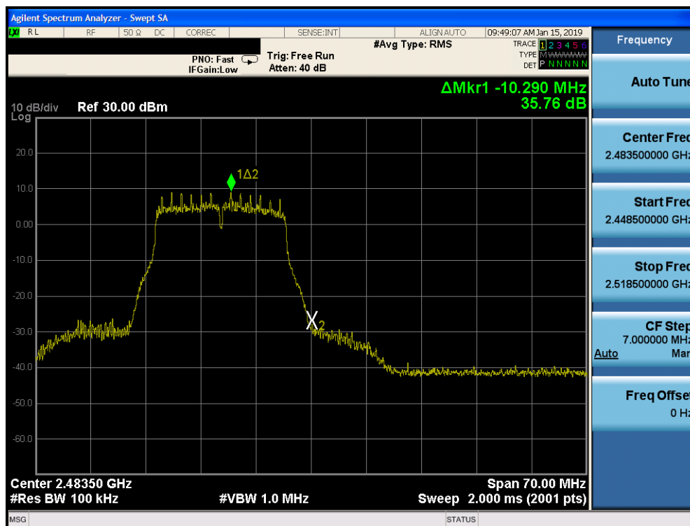
Plot 7-86. Band Edge Plot SISO CORE 0 PRIMARY (802.11g – Ch. 13)
