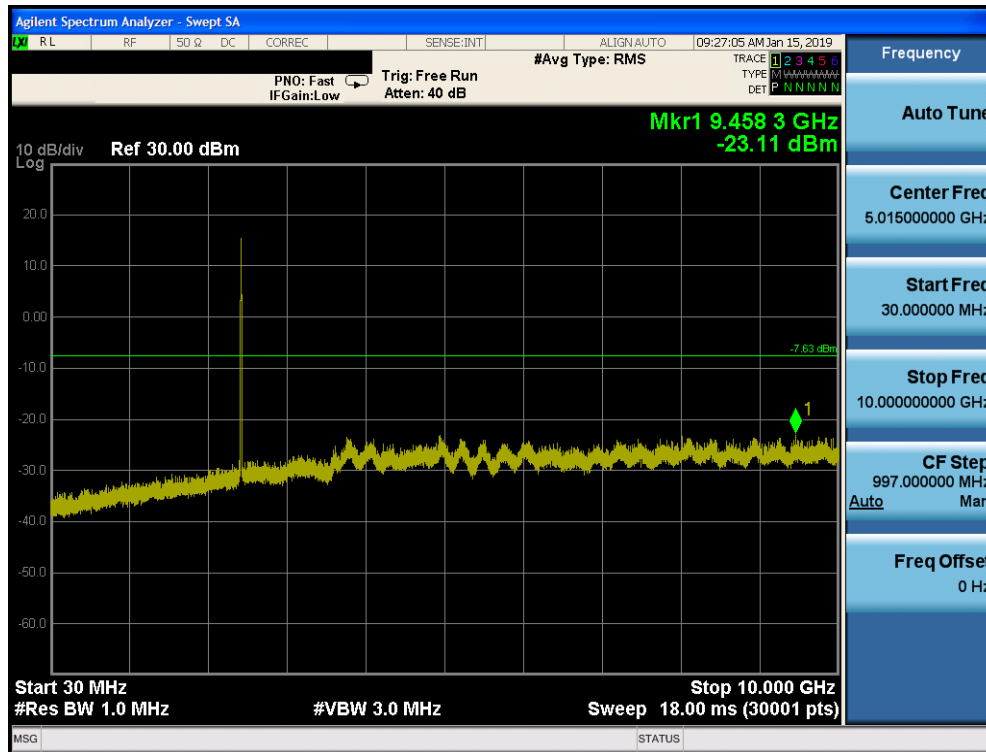
Plot 7-117. Conducted Spurious Plot SISO CORE 0 PRIMARY (802.11b – Ch. 6)
