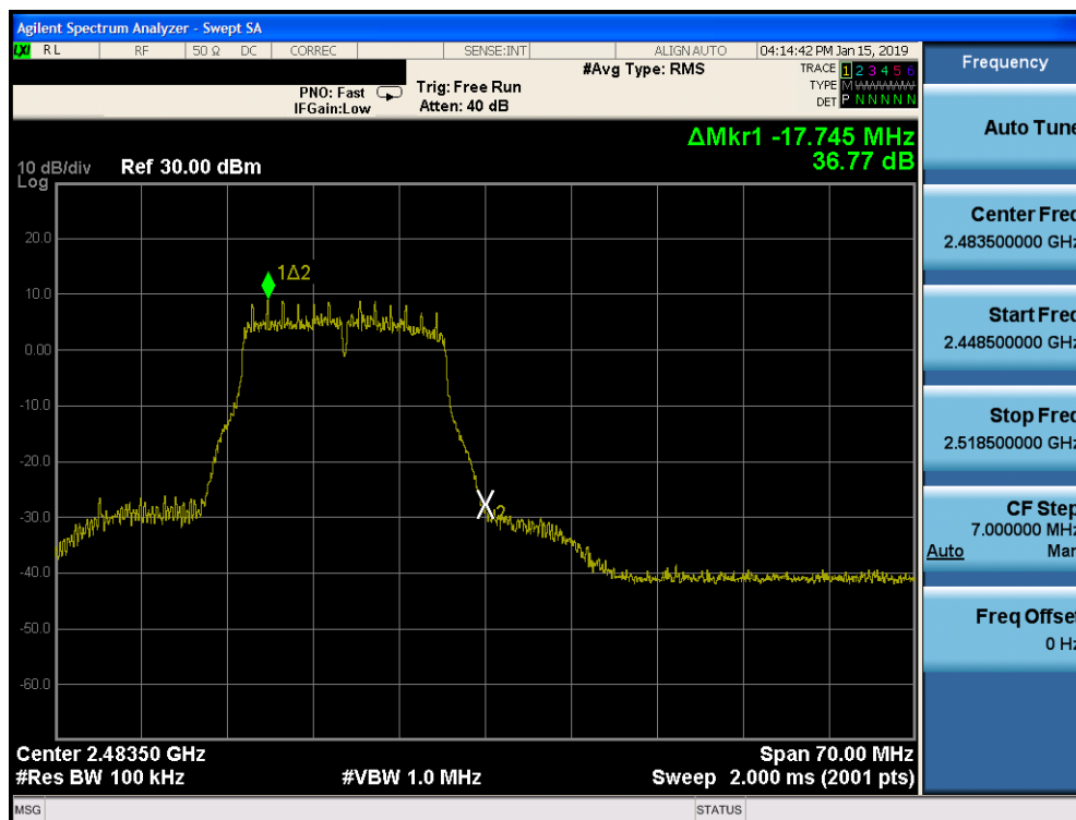
Plot 7-114. Band Edge Plot SISO CORE 1 (802.11n – Ch. 13)
