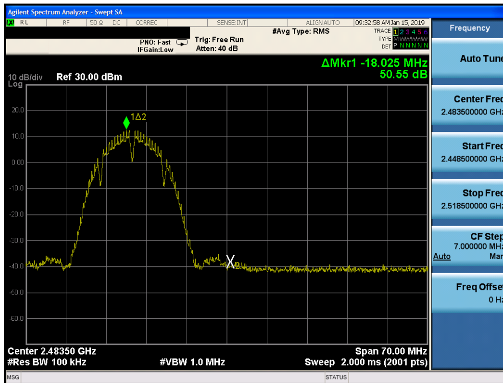
Plot 7-81. Band Edge Plot SISO CORE 0 PRIMARY (802.11b – Ch. 12)
