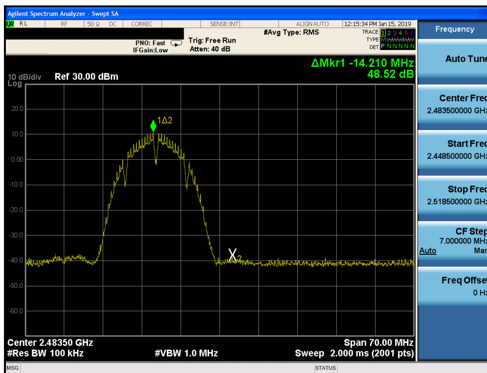
Plot 7-94. Band Edge Plot SISO CORE 0 DIVERSITY (802.11b – Ch. 13)
