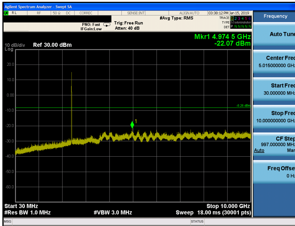
Plot 7-127. Conducted Spurious Plot SISO CORE 1 (802.11b – Ch. 1)
