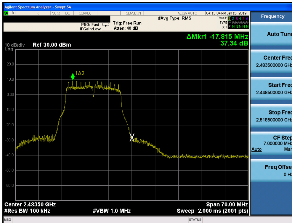
Plot 7-110. Band Edge Plot SISO CORE 1 (802.11g – Ch. 13)
