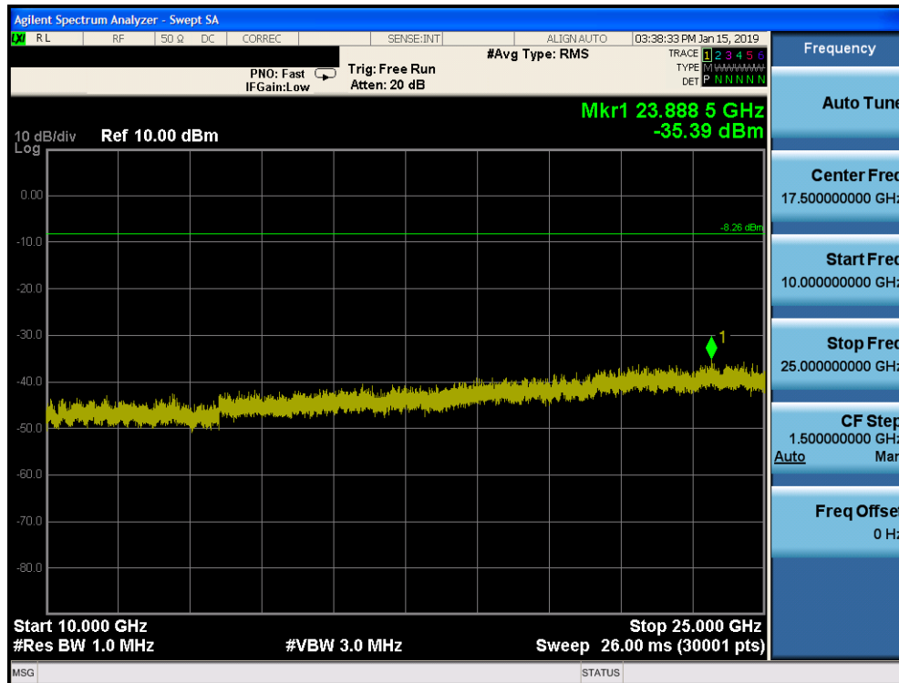
Plot 7-128. Conducted Spurious Plot SISO CORE 1 (802.11b – Ch. 1)
