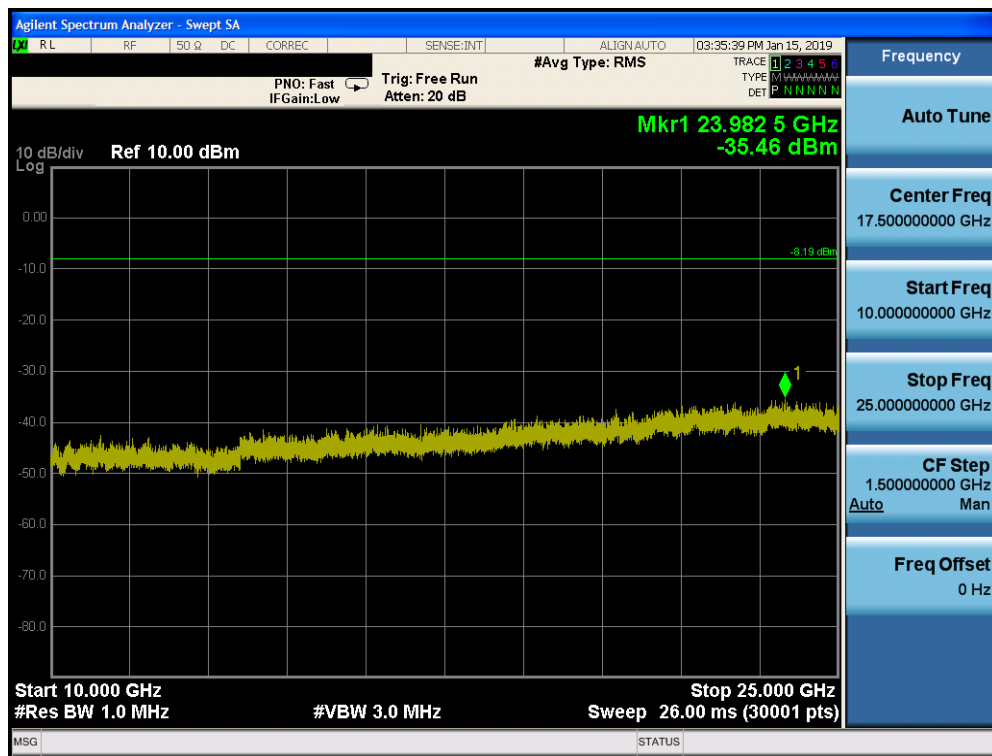
Plot 7-130. Conducted Spurious Plot SISO CORE 1 (802.11b – Ch. 6)
