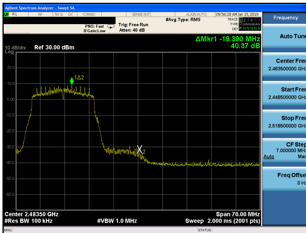
Plot 7-88. Band Edge Plot SISO CORE 0 PRIMARY (802.11n – Ch. 11)
