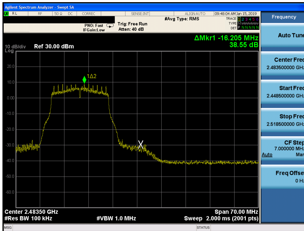
Plot 7-85. Band Edge Plot SISO CORE 0 PRIMARY (802.11g – Ch. 12)
