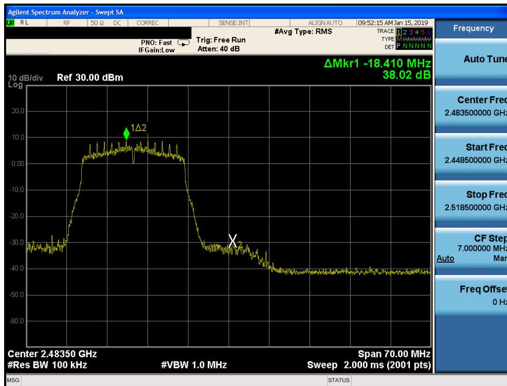
Plot 7-89. Band Edge Plot SISO CORE 0 PRIMARY (802.11n – Ch. 12)
