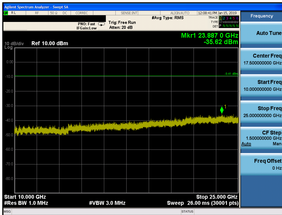
Plot 7-124. Conducted Spurious Plot SISO CORE 0 DIVERSITY (802.11b – Ch. 6)
