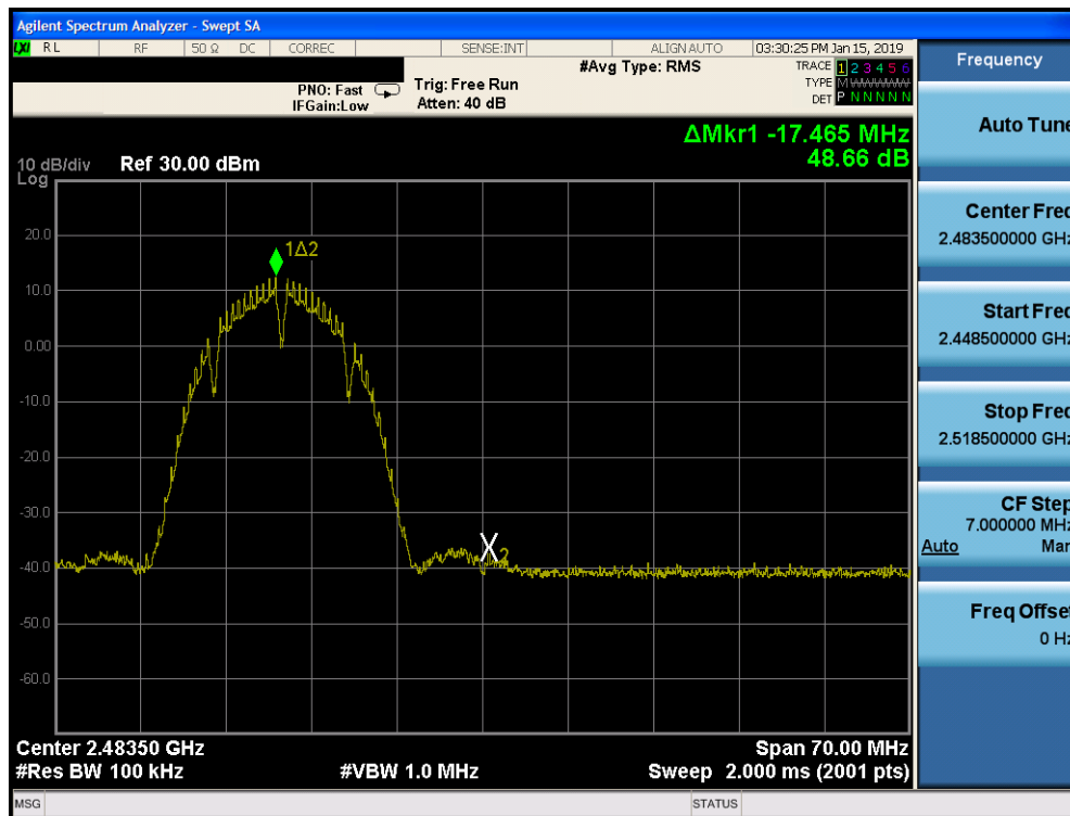
Plot 7-105. Band Edge Plot SISO CORE 1 (802.11b - Ch. 12)
