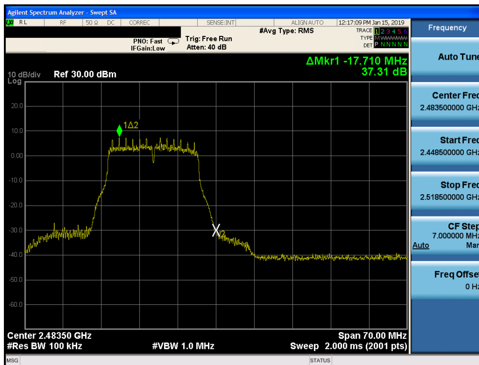
Plot 7-98. Band Edge Plot SISO CORE 0 DIVERSITY (802.11g – Ch. 13)
