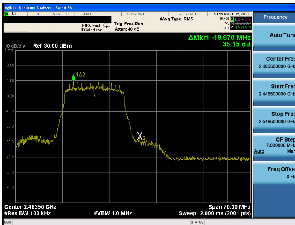
Plot 7-90. Band Edge Plot SISO CORE 0 PRIMARY (802.11n – Ch. 13)
