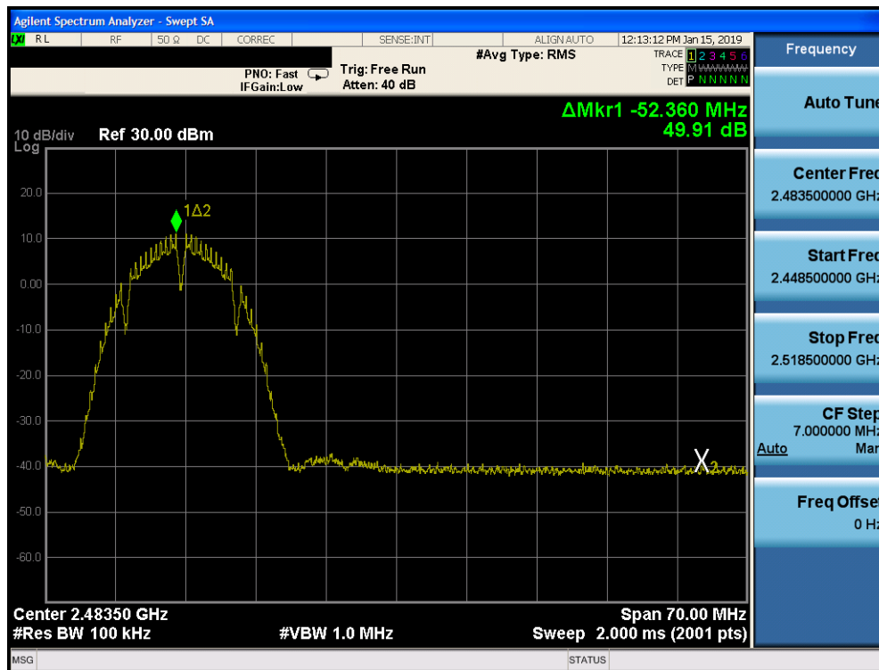
Plot 7-92. Band Edge Plot SISO CORE 0 DIVERSITY (802.11b – Ch. 11)
