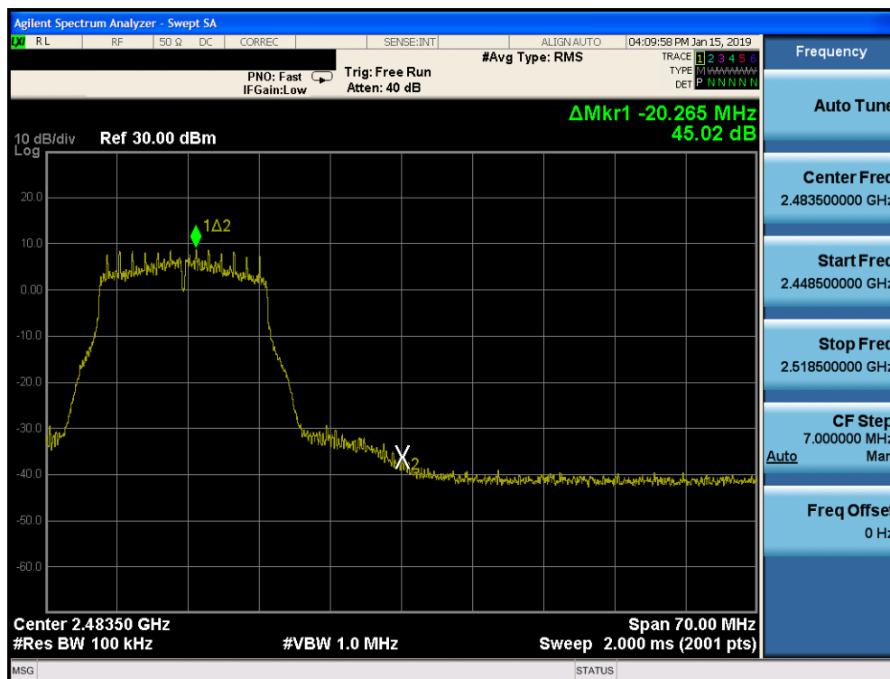
Plot 7-108. Band Edge Plot SISO CORE 1 (802.11g – Ch. 11)
