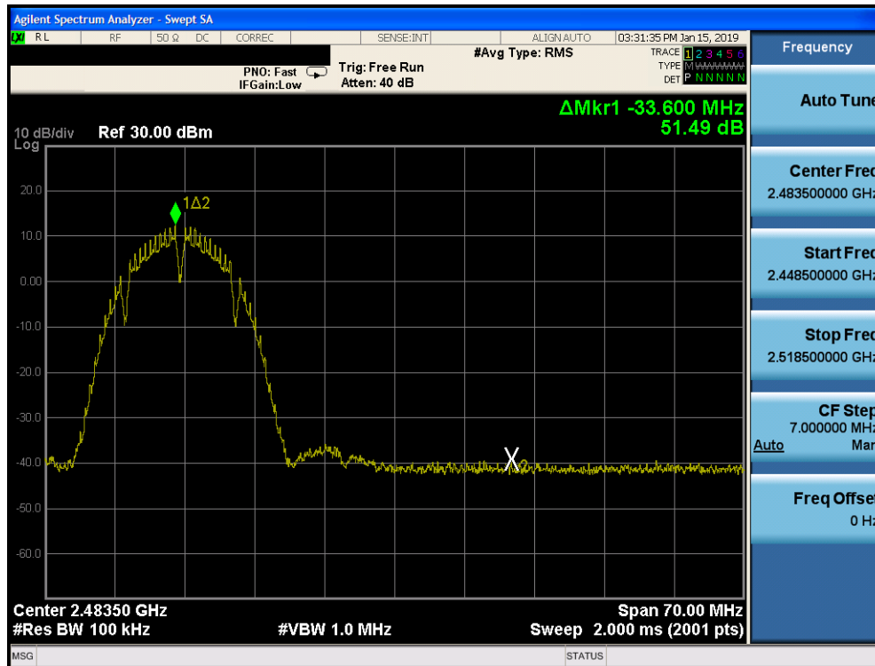
Plot 7-104. Band Edge Plot SISO CORE 1 (802.11b – Ch. 11)
