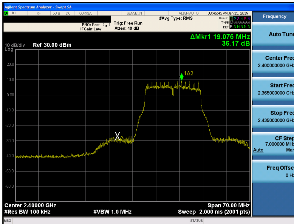
Plot 7-107. Band Edge Plot SISO CORE 1 (802.11g– Ch. 1)
