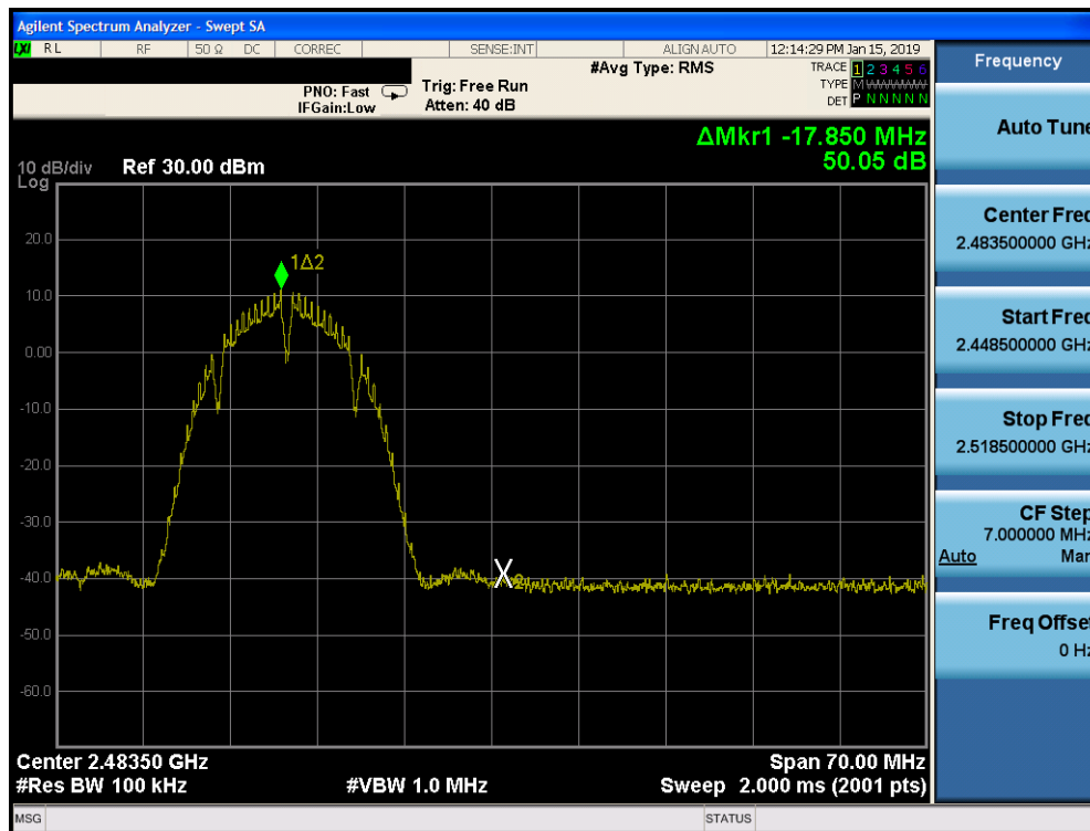
Plot 7-93. Band Edge Plot SISO CORE 0 DIVERSITY (802.11b – Ch. 12)
