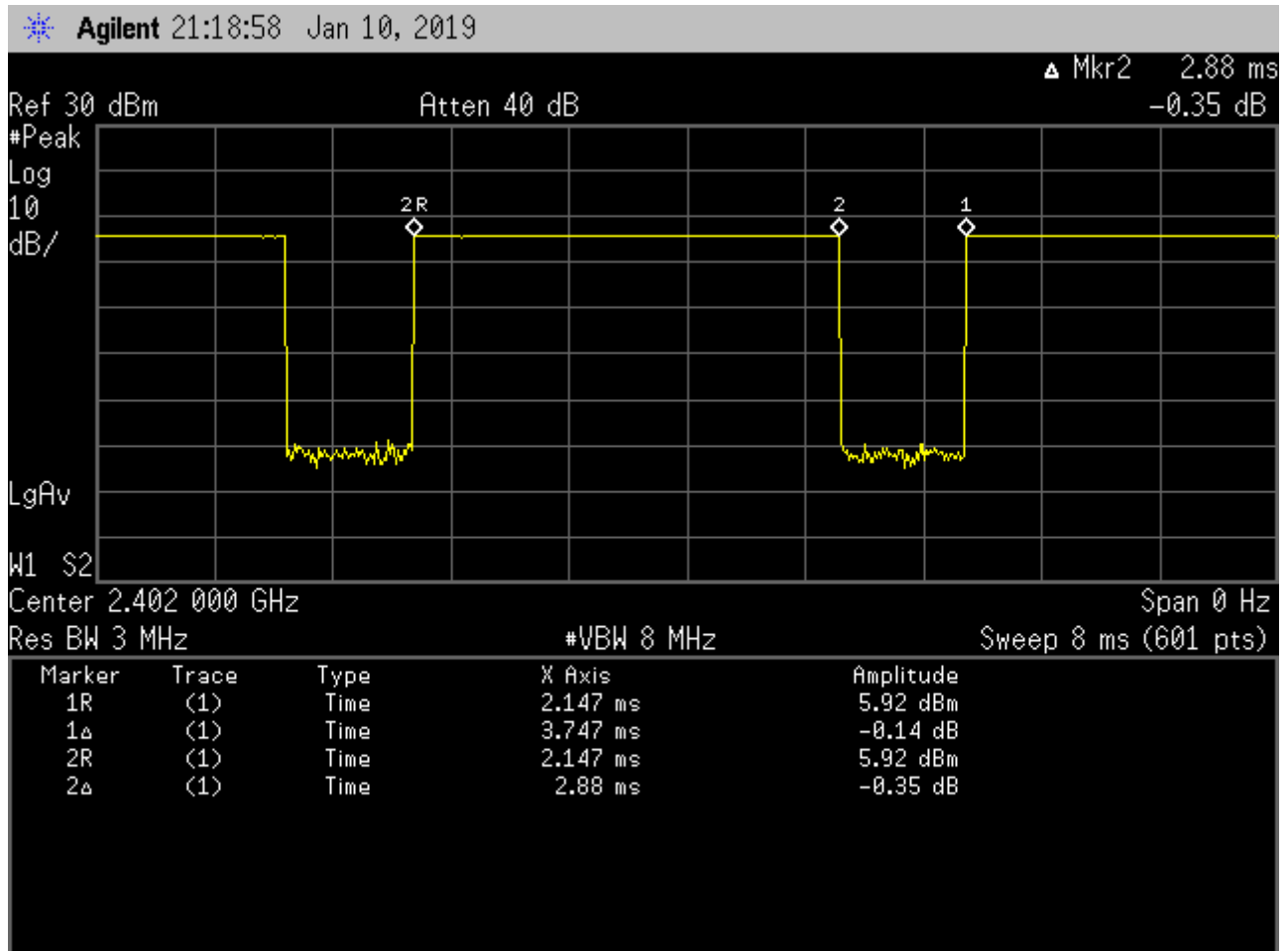
Figure 8-12 Reduced Bluetooth Transmission Plot & Duty Cycle Calculation – Ant WF2 Variant 2
