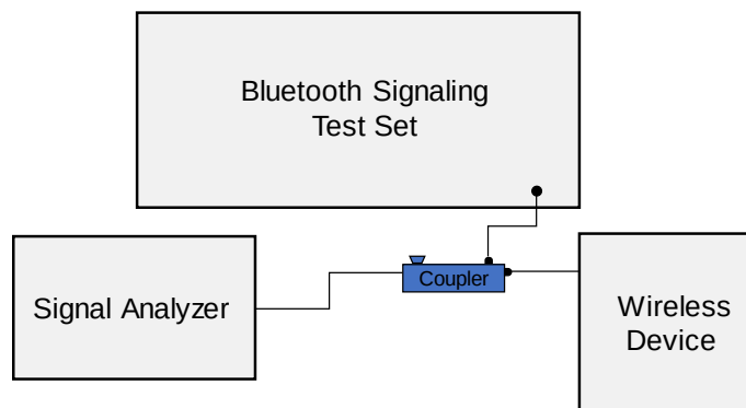
Figure 8-15 Power Measurement Setup
