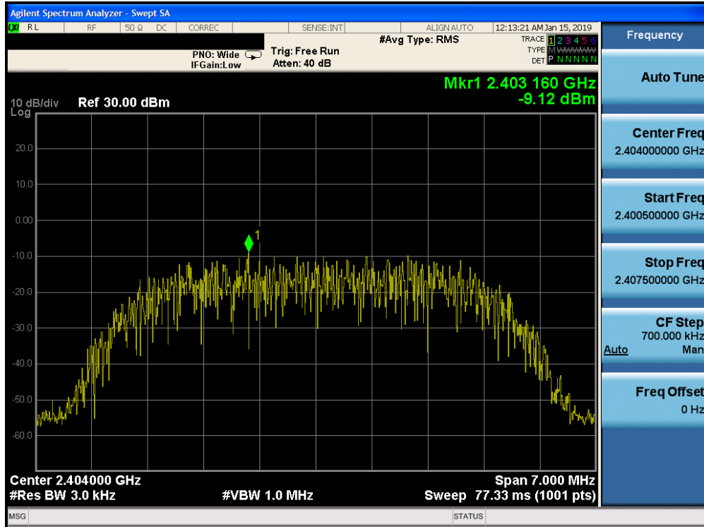
Plot 7-37. Power Spectral Density Plot Ant-1 (Bluetooth (HDR8), 8Mbps, ePA – Ch. 1)
