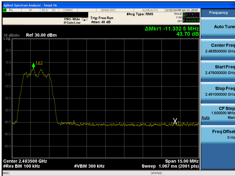
Plot 7-64. Band Edge Plot Ant-2 (Bluetooth (HDR4), ePA – Ch. 75)
