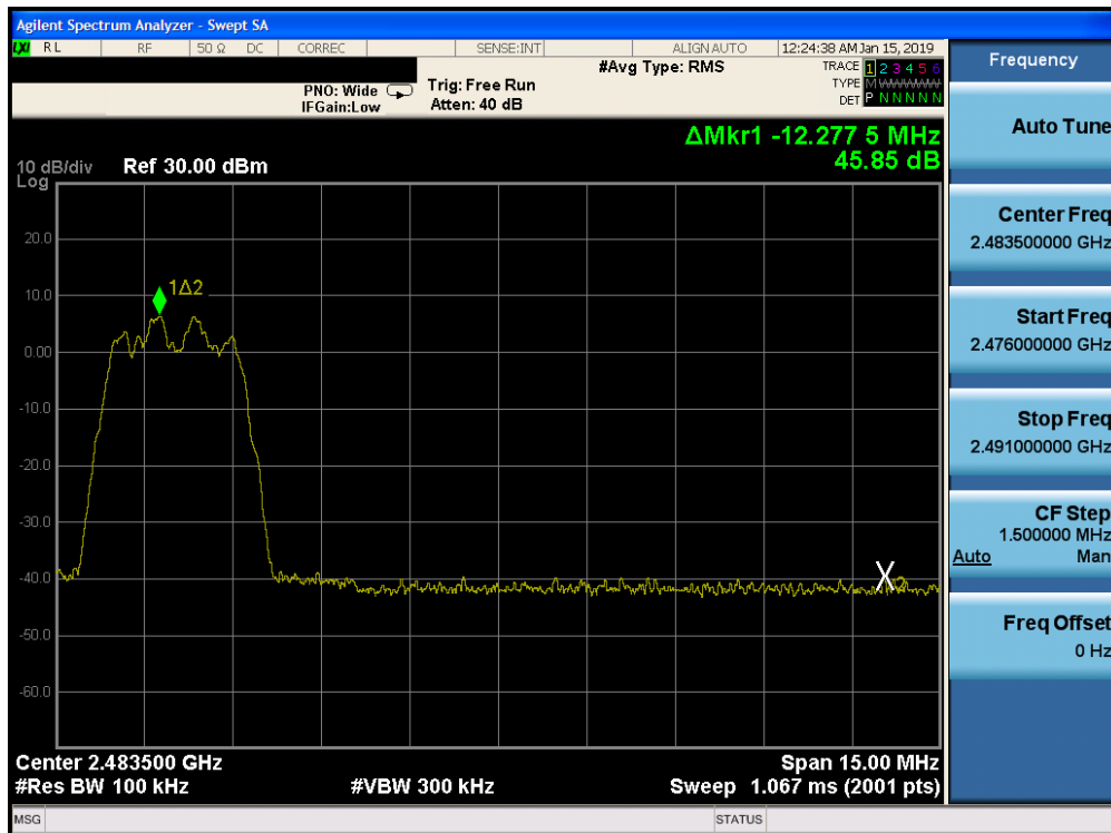
Plot 7-60. Band Edge Plot Ant-1 (Bluetooth (HDR4), ePA – Ch. 75)
