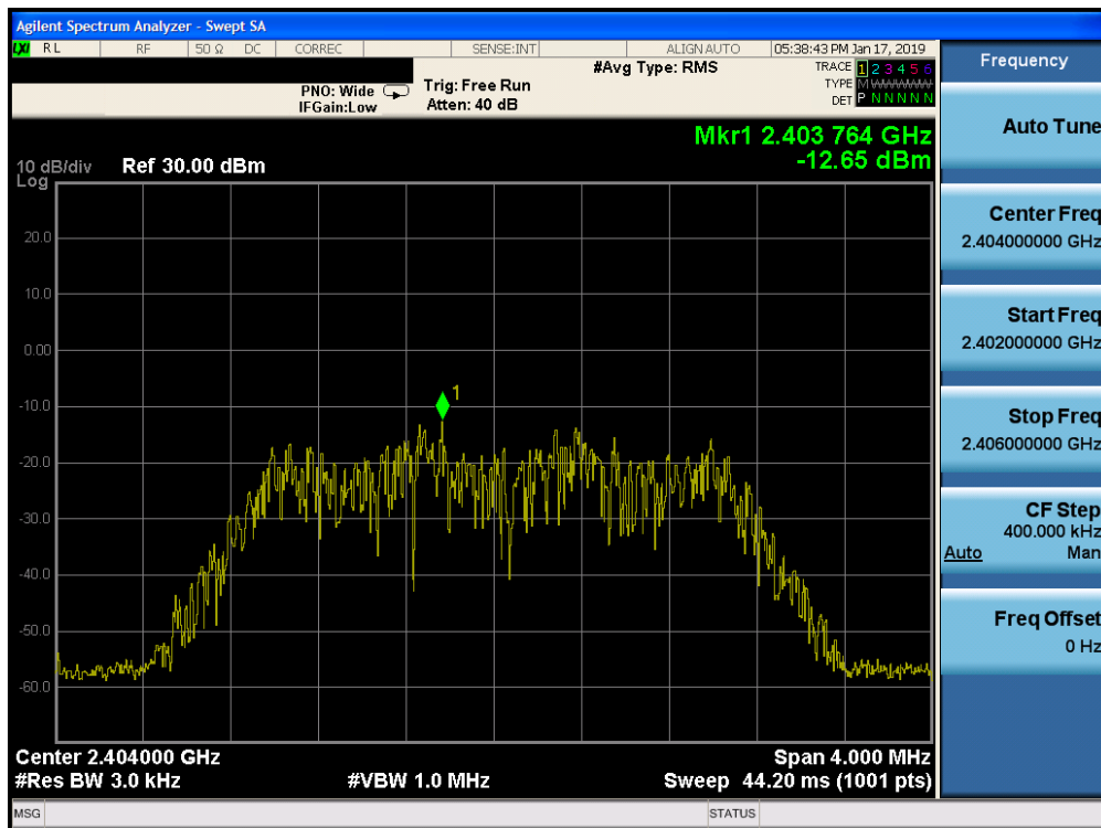
Plot 7-22. Power Spectral Density Plot Ant-0 (Bluetooth (HDR4), 4Mbps, iPA – Ch. 1)
