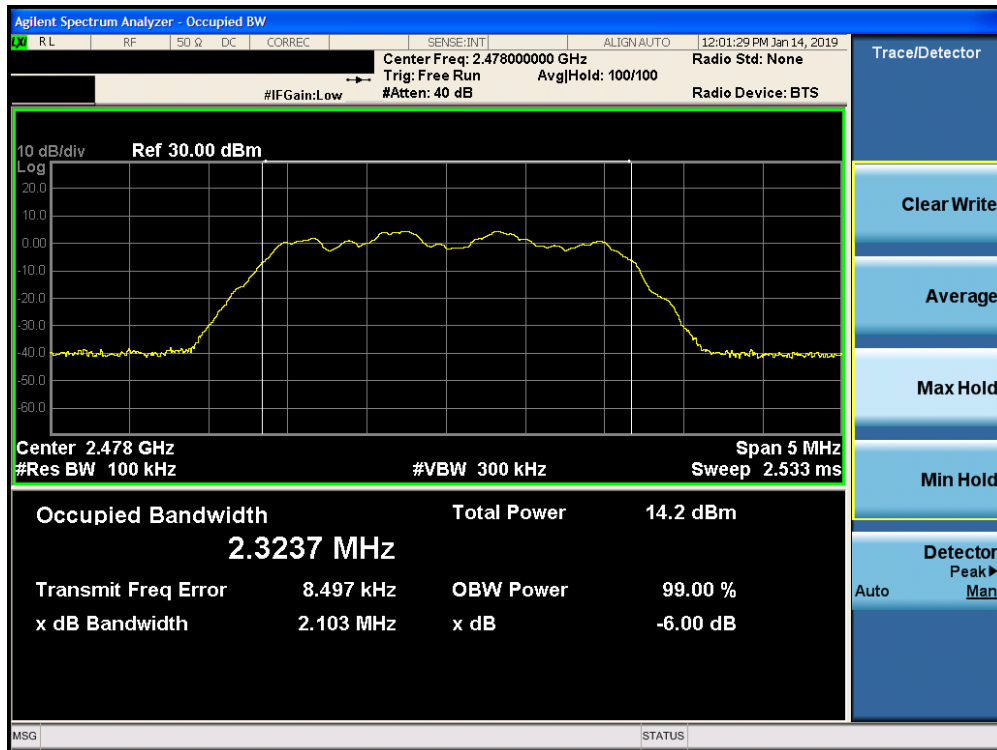
Plot 7-15. 6dB Bandwidth Plot Ant-2 (Bluetooth (HDR4), 4Mbps, ePA - Ch. 75)
