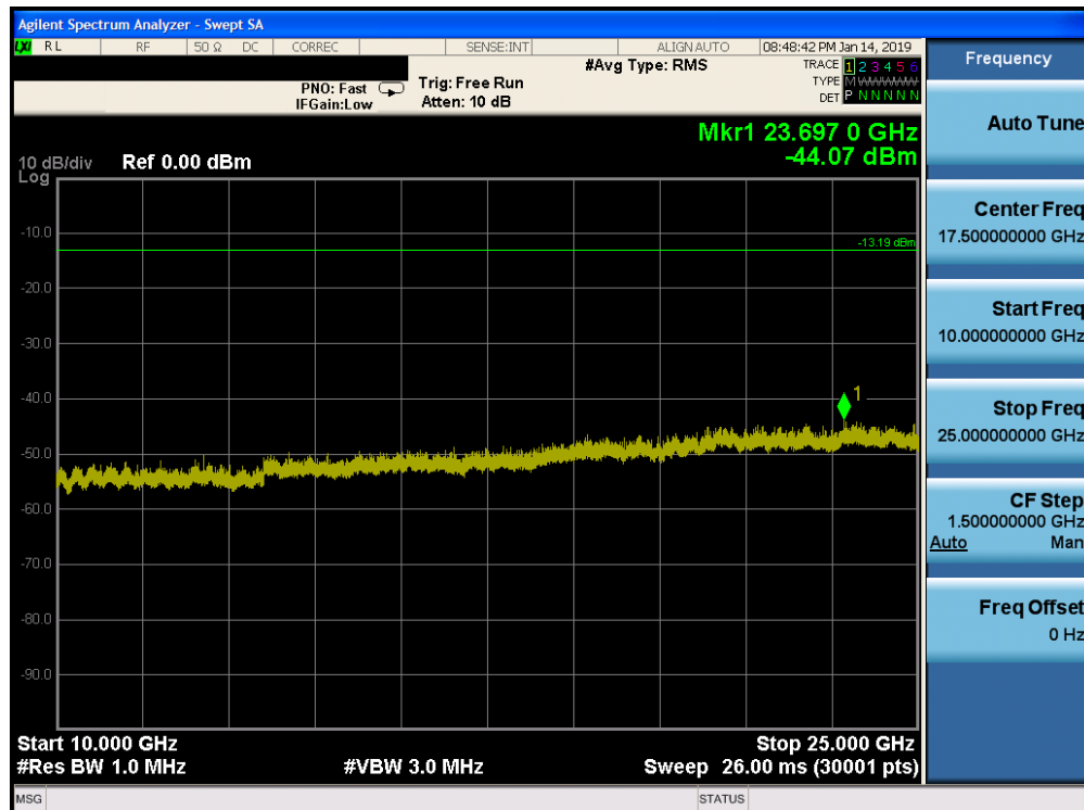
Plot 7-68. Conducted Spurious Plot Ant-0 (Bluetooth (HDR4), Mbps, ePA – Ch. 1)
