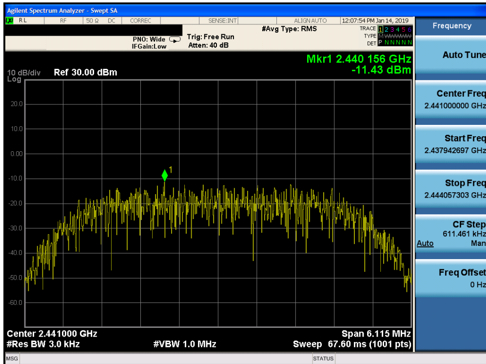
Plot 7-50. Power Spectral Density Plot Ant-2 (Bluetooth (HDR8), 8Mbps, ePA – Ch. 38)
