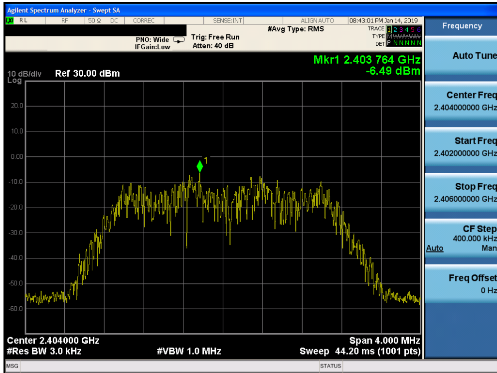
Plot 7-19. Power Spectral Density Plot Ant-0 (Bluetooth (HDR4), 4Mbps, ePA – Ch. 1)
