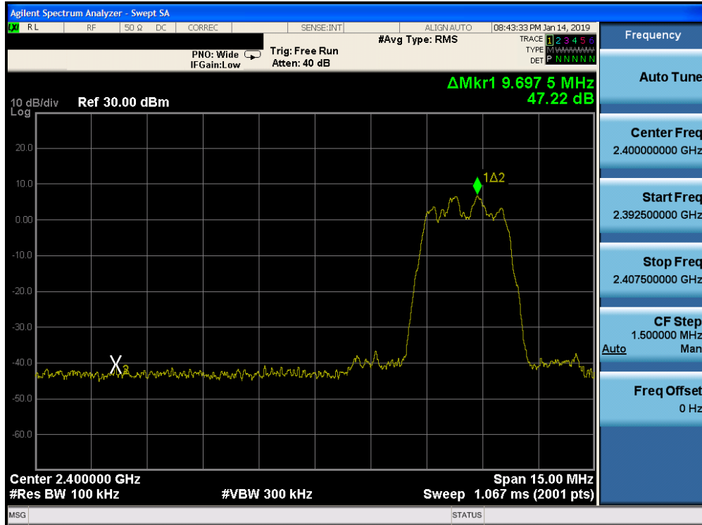
Plot 7-55. Band Edge Plot Ant-0 (Bluetooth (HDR4), ePA – Ch. 1)
