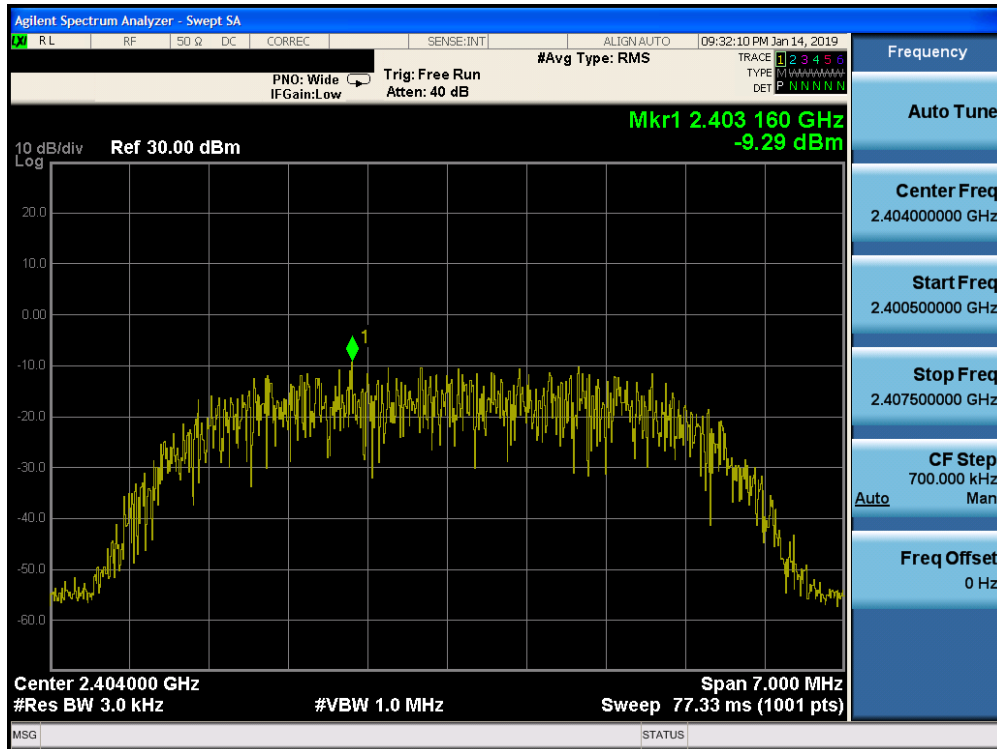
Plot 7-25. Power Spectral Density Plot Ant-0 (Bluetooth (HDR8), 8Mbps, ePA – Ch. 1)
