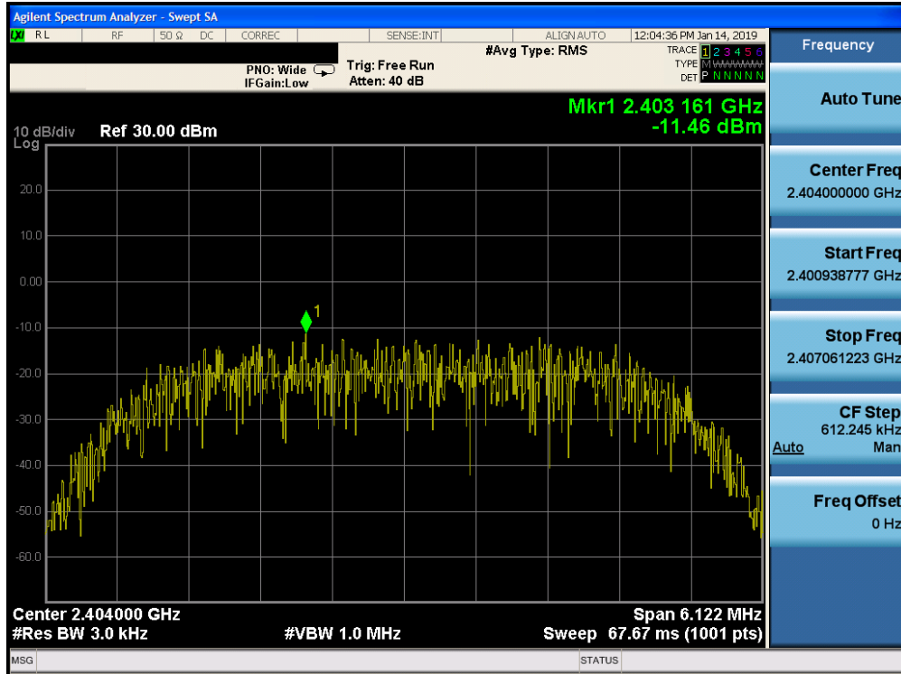
Plot 7-49. Power Spectral Density Plot Ant-2 (Bluetooth (HDR8), 8Mbps, ePA – Ch. 1)
