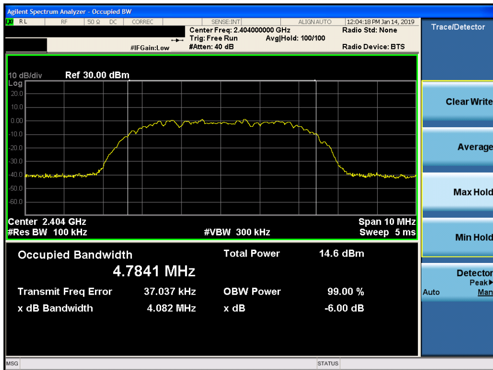
Plot 7-16. 6dB Bandwidth Plot Ant-2 (Bluetooth (HDR8), 8Mbps, ePA - Ch. 1)
