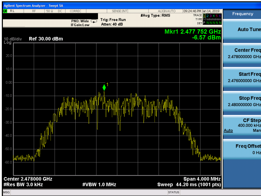
Plot 7-21. Power Spectral Density Plot Ant-0 (Bluetooth (HDR4), 4Mbps, ePA – Ch. 75)
