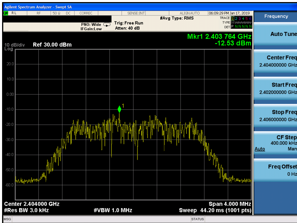
Plot 7-34. Power Spectral Density Plot Ant-1 (Bluetooth (HDR4), 4Mbps, iPA – Ch. 1)
