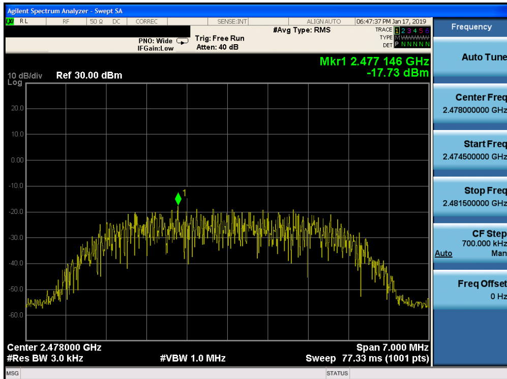
Plot 7-54. Power Spectral Density Plot Ant-2 (Bluetooth (HDR8), 8Mbps, iPA – Ch. 75)
