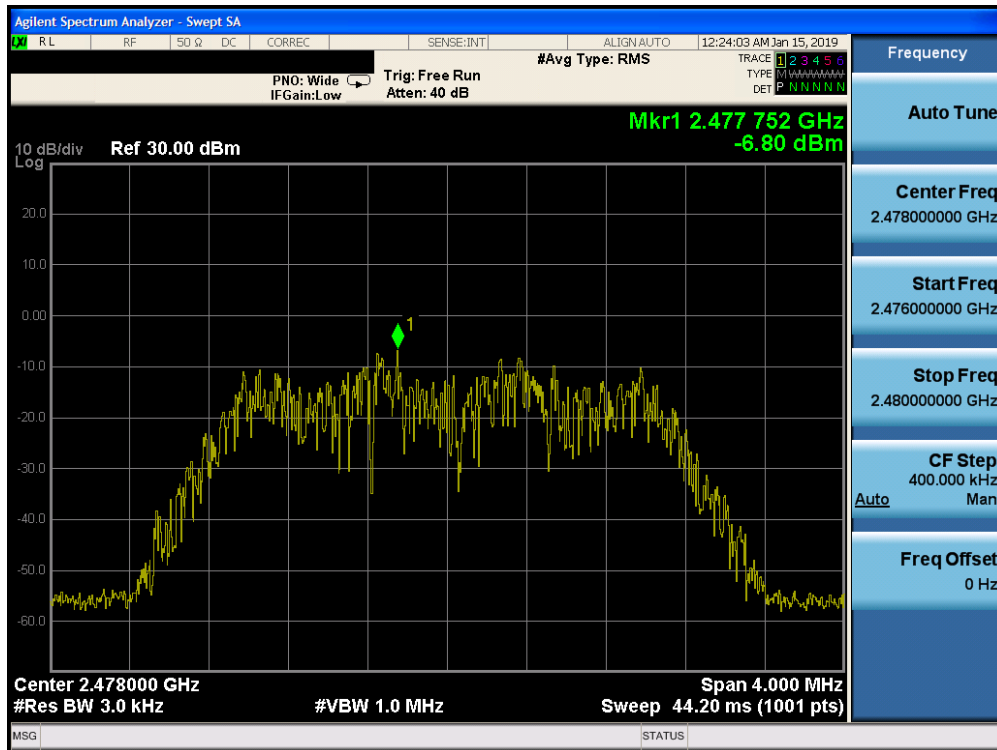
Plot 7-33. Power Spectral Density Plot Ant-1 (Bluetooth (HDR4), 4Mbps, ePA – Ch. 75)
