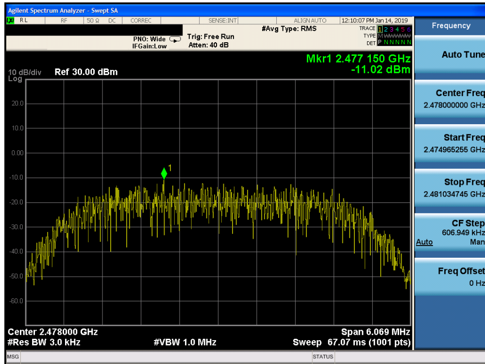
Plot 7-51. Power Spectral Density Plot Ant-2 (Bluetooth (HDR8), 8Mbps, ePA – Ch. 75)
