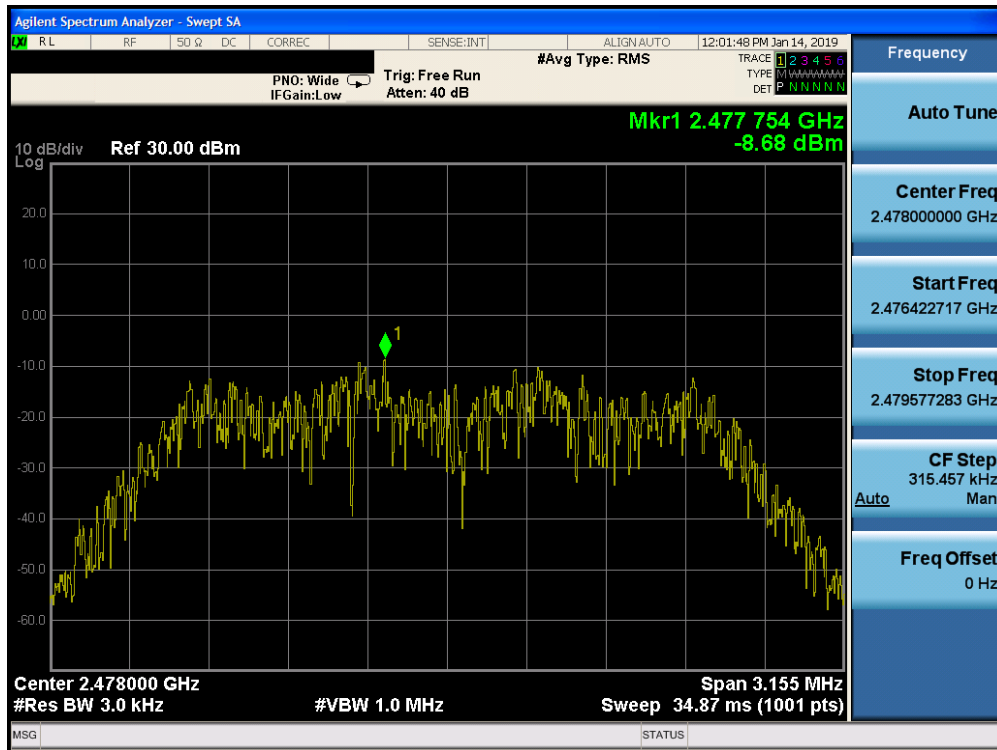
Plot 7-45. Power Spectral Density Plot Ant-2 (Bluetooth (HDR4), 4Mbps, ePA – Ch. 75)
