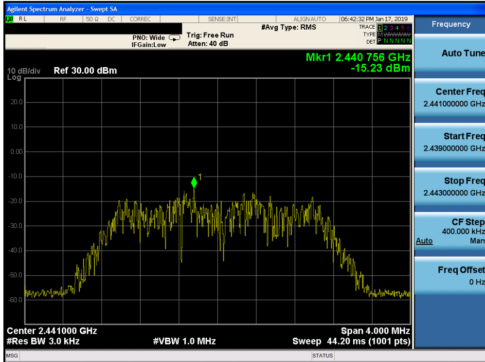
Plot 7-47. Power Spectral Density Plot Ant-2 (Bluetooth (HDR4), 4Mbps, iPA – Ch. 38)
