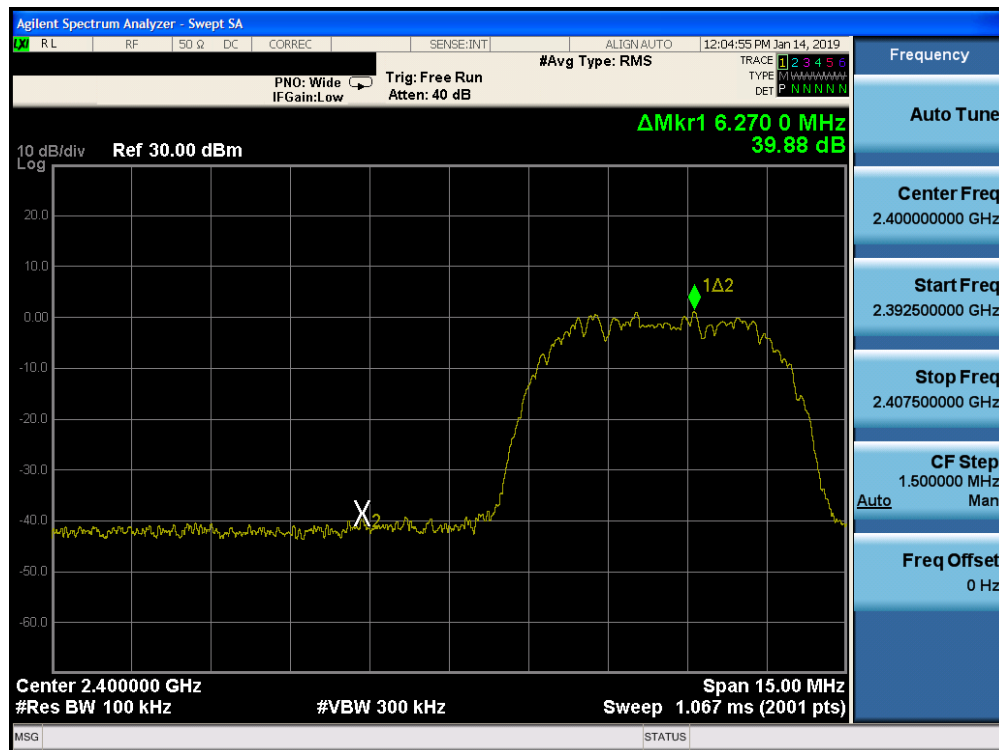
Plot 7-65. Band Edge Plot Ant-2 (Bluetooth (HDR8), ePA – Ch. 1)
