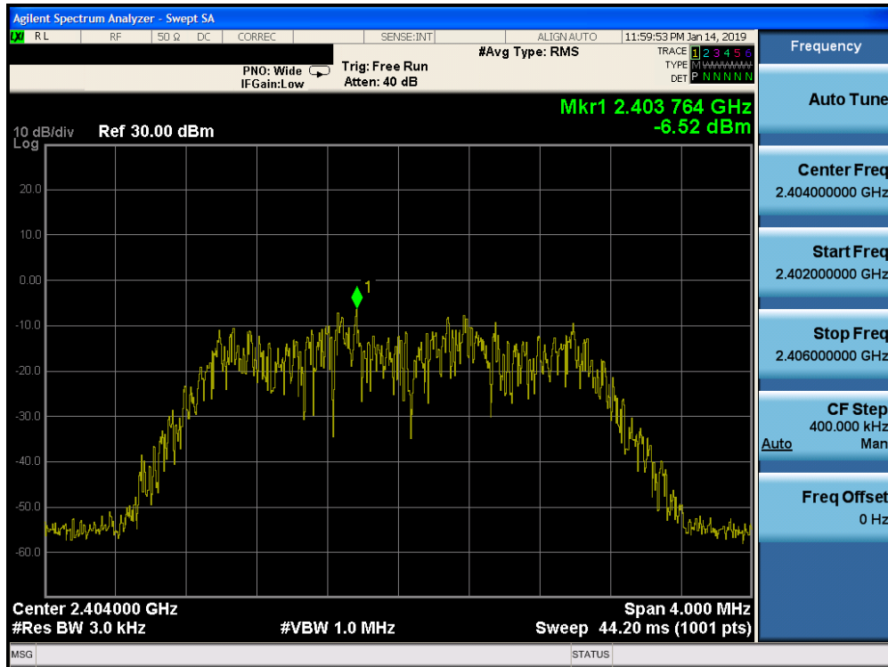
Plot 7-31. Power Spectral Density Plot Ant-1 (Bluetooth (HDR4), 4Mbps, ePA – Ch. 1)
