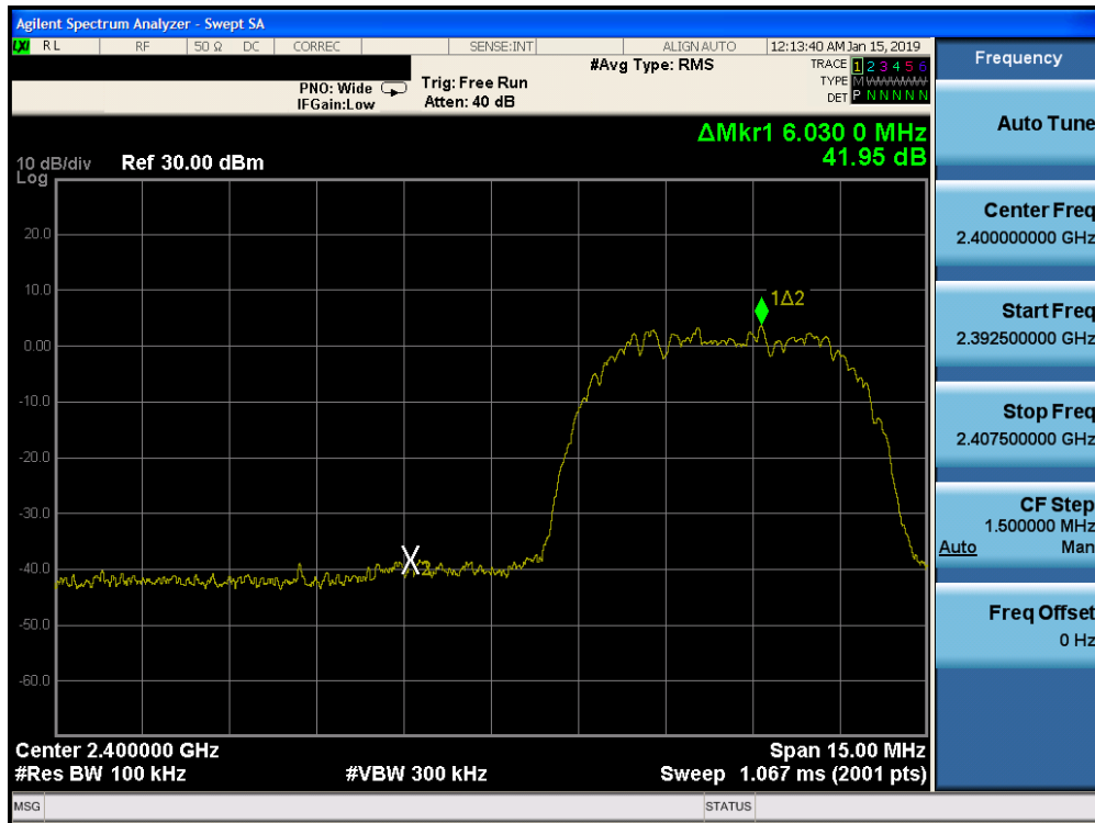
Plot 7-61. Band Edge Plot Ant-1 (Bluetooth (HDR8), ePA – Ch. 1)
