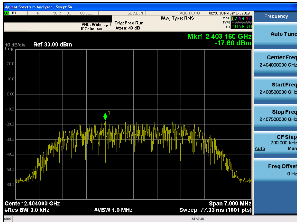
Plot 7-52. Power Spectral Density Plot Ant-2 (Bluetooth (HDR8), 8Mbps, iPA – Ch. 1)
