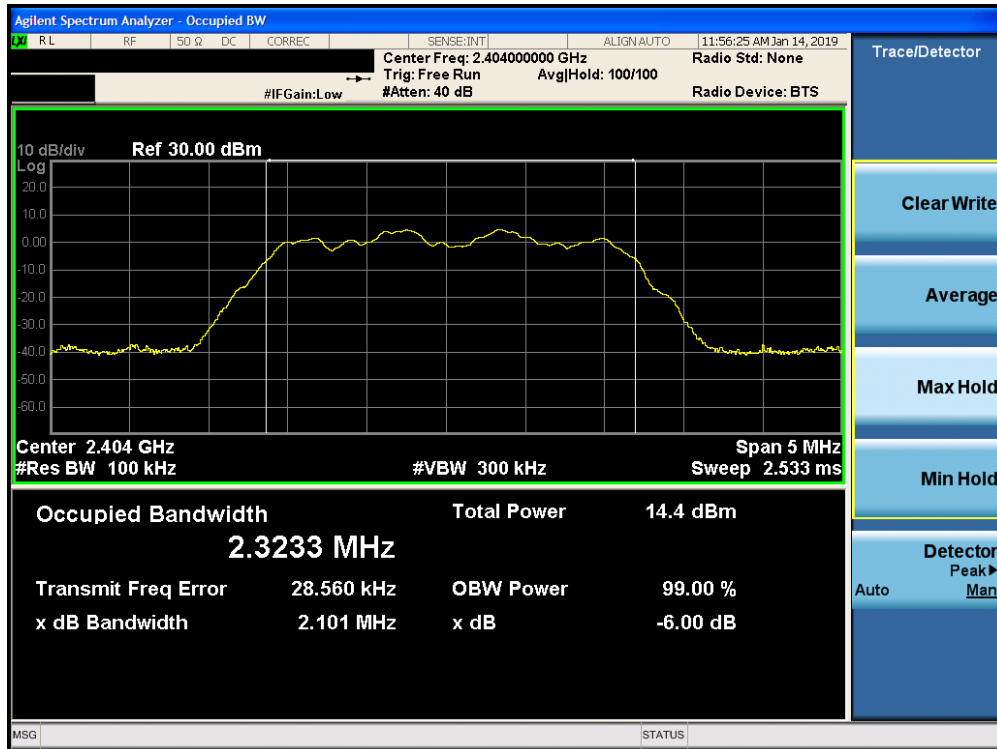
Plot 7-13. 6dB Bandwidth Plot Ant-2 (Bluetooth (HDR4), 4Mbps, ePA – Ch. 1)
