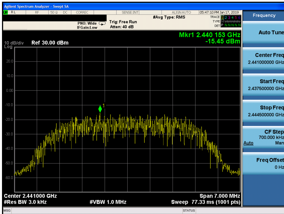
Plot 7-29. Power Spectral Density Plot Ant-0 (Bluetooth (HDR8), 8Mbps, iPA – Ch. 38)
