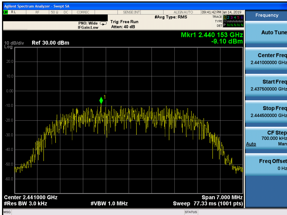
Plot 7-26. Power Spectral Density Plot Ant-0 (Bluetooth (HDR8), 8Mbps, ePA – Ch. 38)
