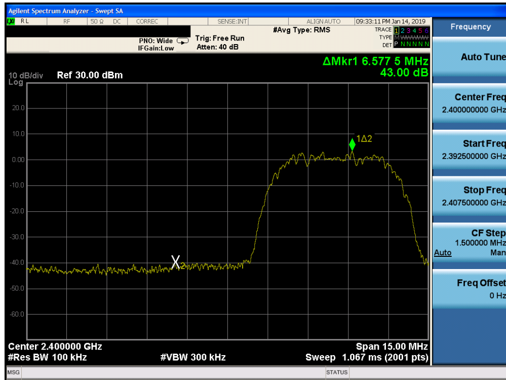
Plot 7-57. Band Edge Plot Ant-0 (Bluetooth (HDR8), ePA - Ch. 1)
