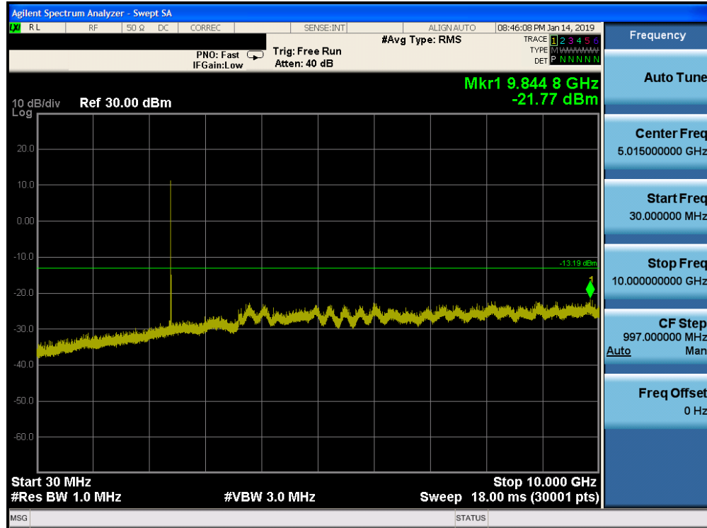
Plot 7-67. Conducted Spurious Plot Ant-0 (Bluetooth (HDR4), Mbps, ePA – Ch. 1)
