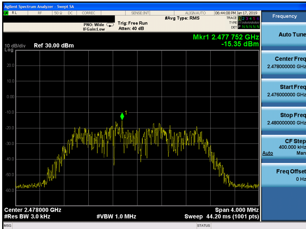
Plot 7-48. Power Spectral Density Plot Ant-2 (Bluetooth (HDR4), 4Mbps, iPA – Ch. 75)
