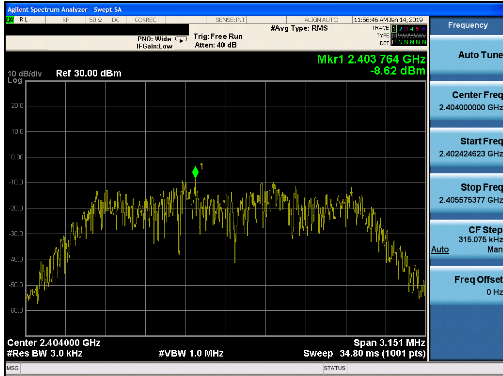
Plot 7-43. Power Spectral Density Plot Ant-2 (Bluetooth (HDR4), 4Mbps, ePA – Ch. 1)
