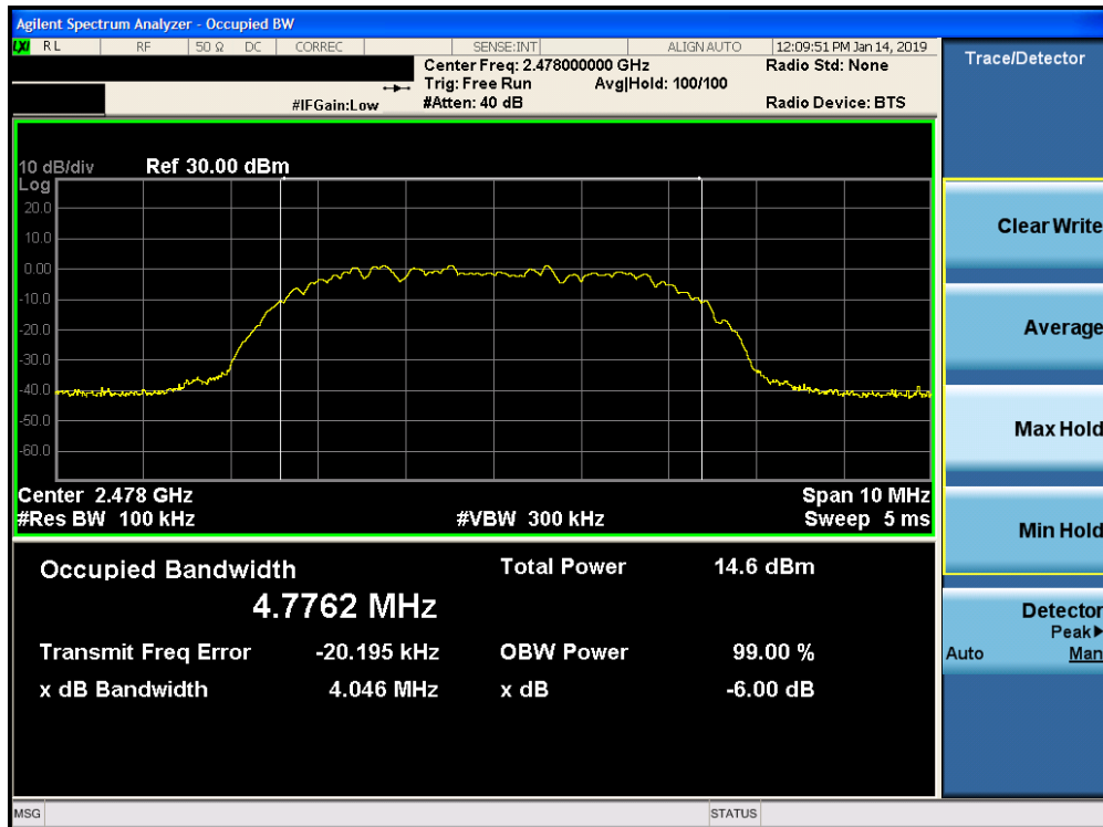
Plot 7-18. 6dB Bandwidth Plot Ant-2 (Bluetooth (HDR8), 8Mbps, ePA – Ch. 75)
