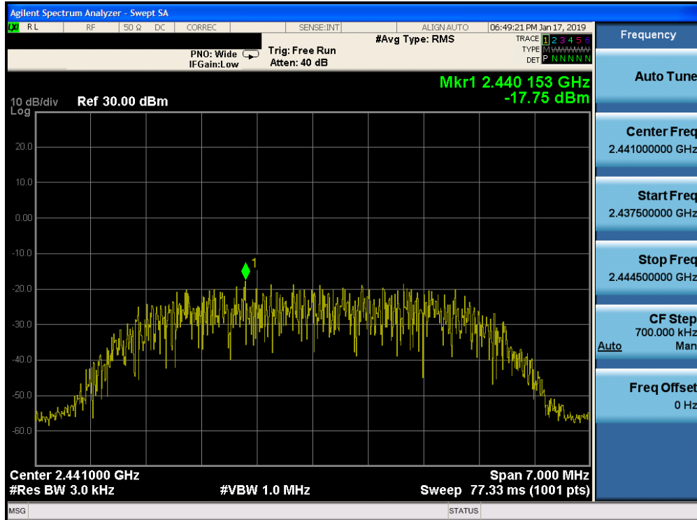
Plot 7-53. Power Spectral Density Plot Ant-2 (Bluetooth (HDR8), 8Mbps, iPA – Ch. 38)
