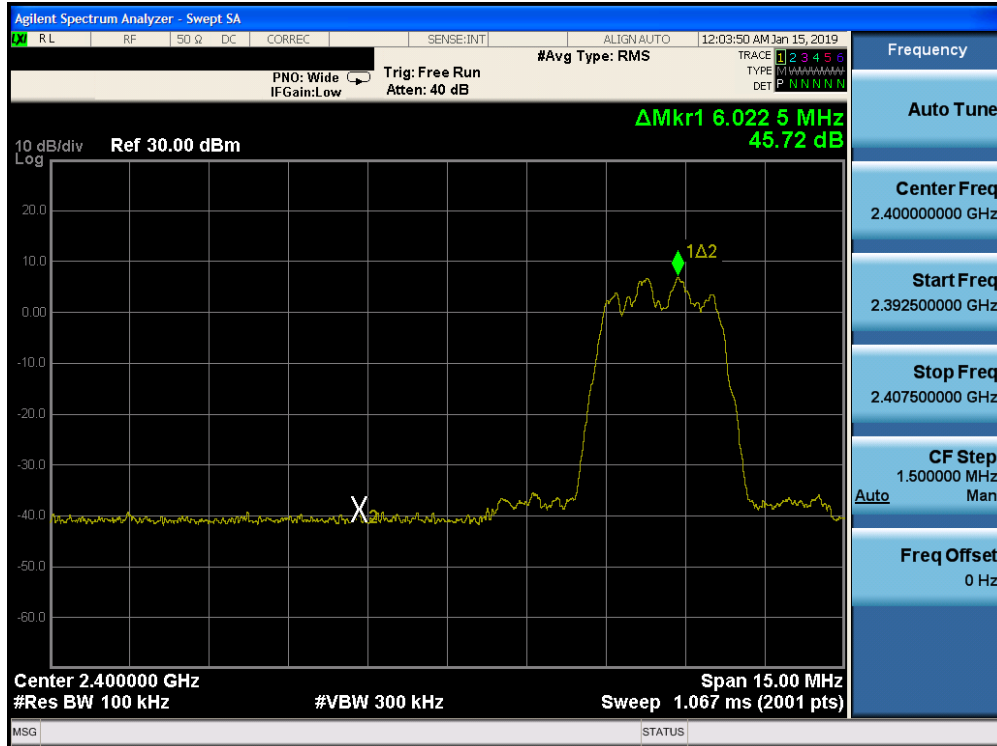
Plot 7-59. Band Edge Plot Ant-1 (Bluetooth (HDR4), ePA – Ch. 1)
