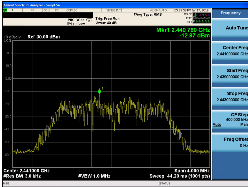
Plot 7-23. Power Spectral Density Plot Ant-0 (Bluetooth (HDR4), 4Mbps, iPA – Ch. 38)
