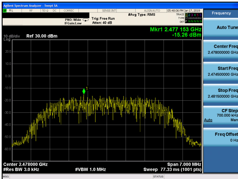
Plot 7-30. Power Spectral Density Plot Ant-0 (Bluetooth (HDR8), 8Mbps, iPA – Ch. 75)
