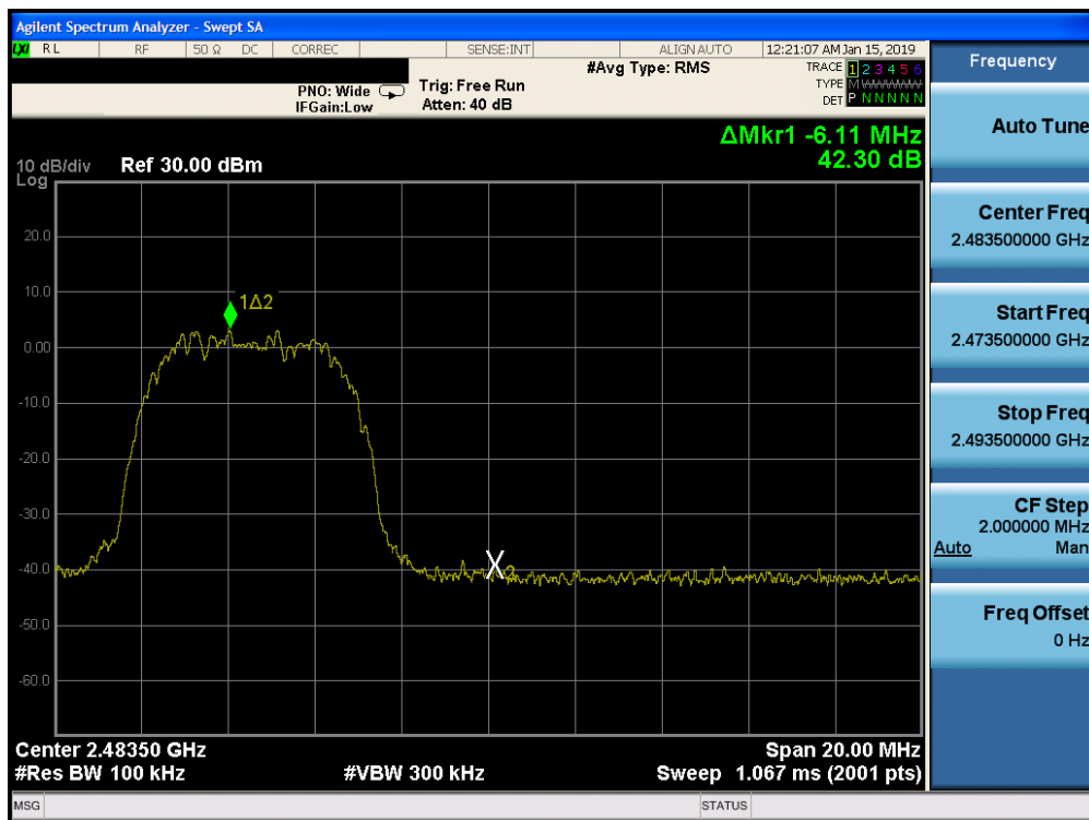
Plot 7-62. Band Edge Plot Ant-1 (Bluetooth (HDR8), ePA – Ch. 75)
