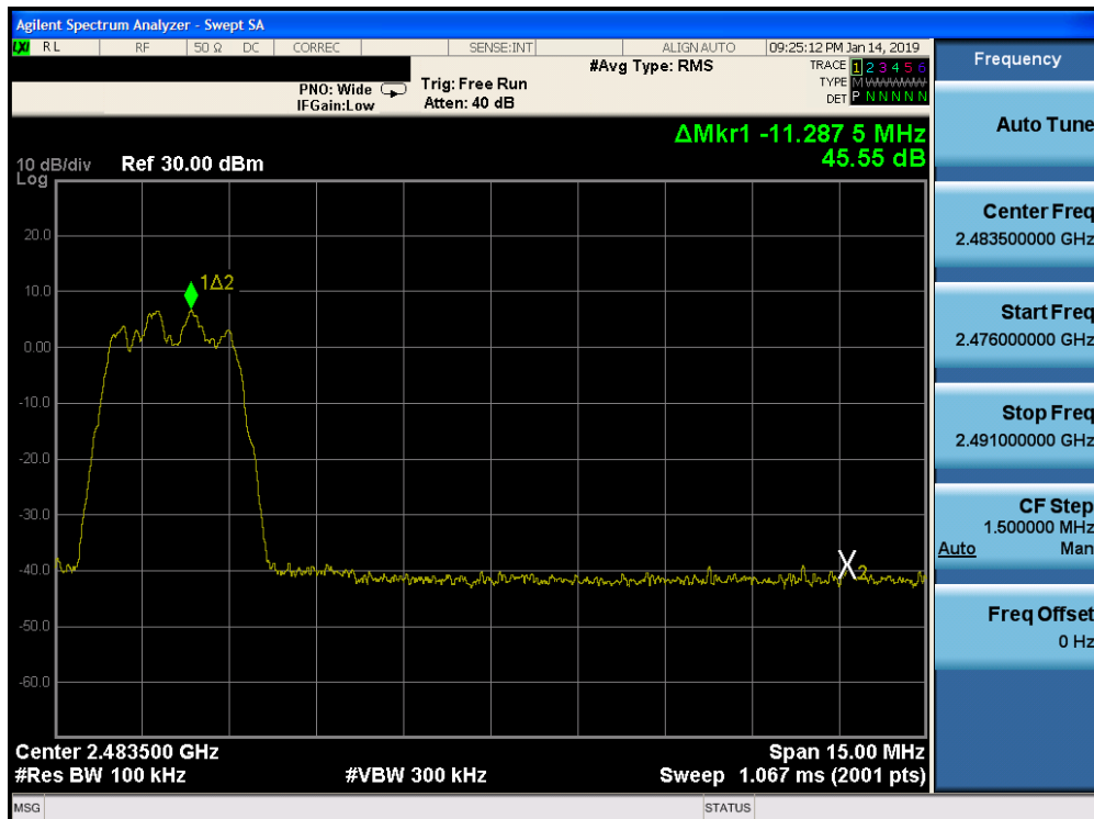
Plot 7-56. Band Edge Plot Ant-0 (Bluetooth (HDR4), ePA – Ch. 75)
