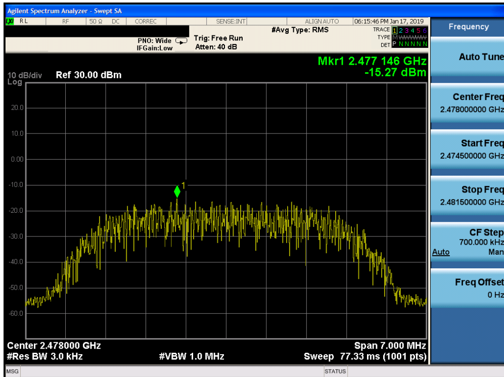
Plot 7-42. Power Spectral Density Plot Ant-1 (Bluetooth (HDR8), 8Mbps, iPA – Ch. 75)
