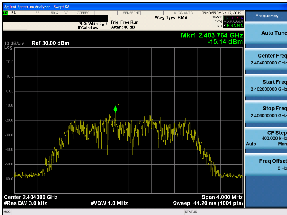
Plot 7-46. Power Spectral Density Plot Ant-2 (Bluetooth (HDR4), 4Mbps, iPA – Ch. 1)
