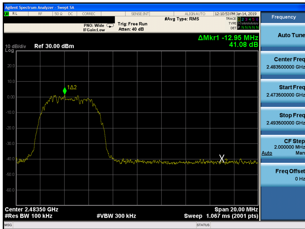
Plot 7-66. Band Edge Plot Ant-2 (Bluetooth (HDR8), ePA – Ch. 75)
