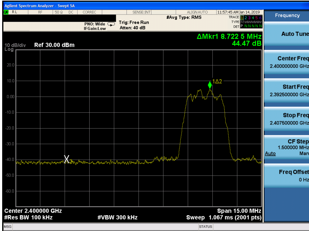
Plot 7-63. Band Edge Plot Ant-2 (Bluetooth (HDR4), ePA – Ch. 1)
