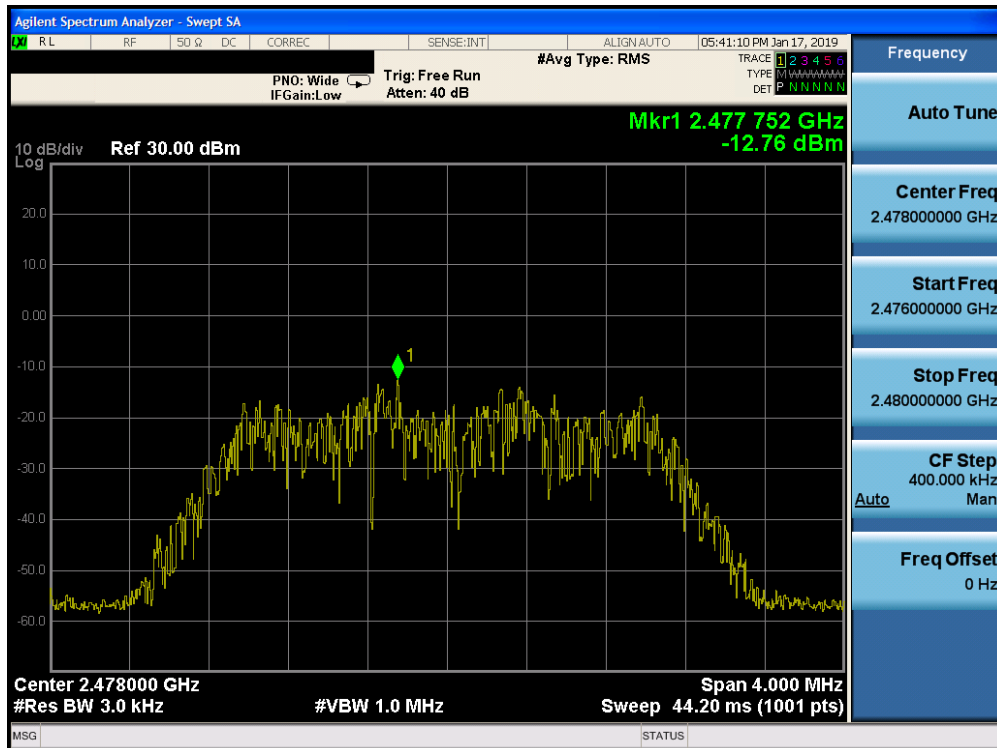
Plot 7-24. Power Spectral Density Plot Ant-0 (Bluetooth (HDR4), 4Mbps, iPA – Ch. 75)
