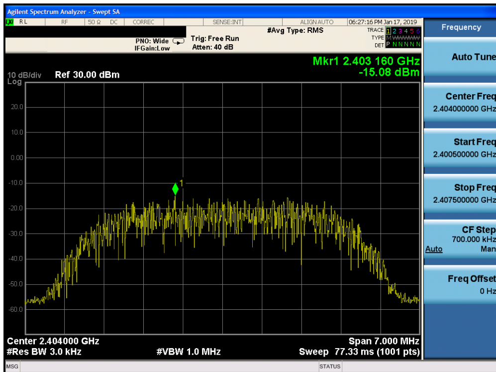
Plot 7-40. Power Spectral Density Plot Ant-1 (Bluetooth (HDR8), 8Mbps, iPA – Ch. 1)
