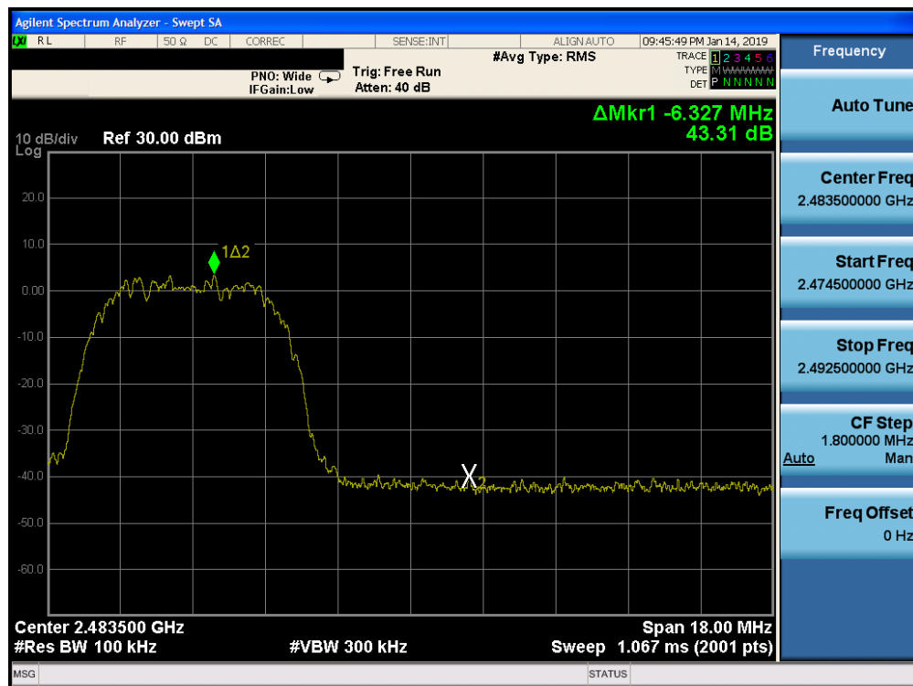
Plot 7-58. Band Edge Plot Ant-0 (Bluetooth (HDR8), ePA - Ch. 75)
