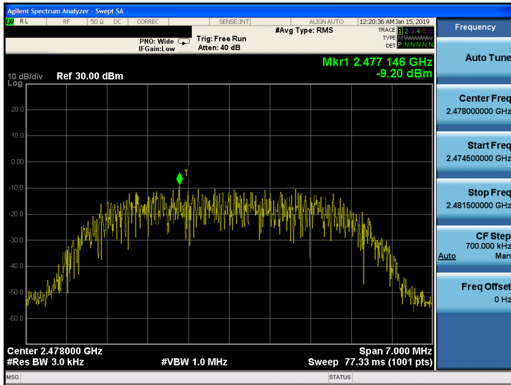
Plot 7-39. Power Spectral Density Plot Ant-1 (Bluetooth (HDR8), 8Mbps, ePA – Ch. 75)
