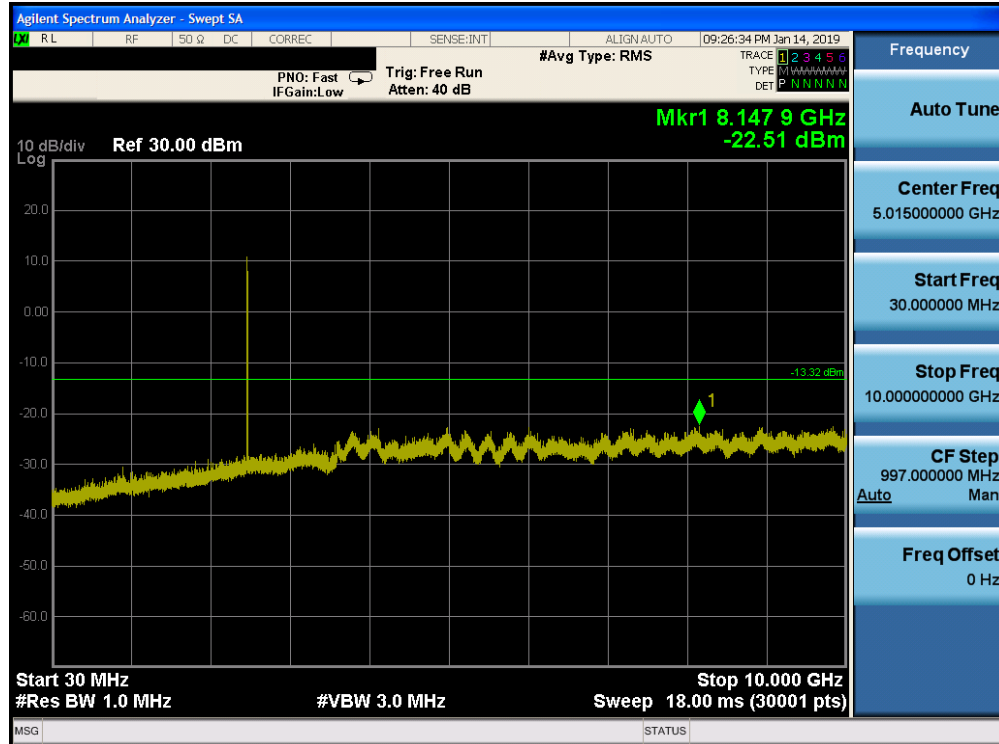
Plot 7-71. Conducted Spurious Plot Ant-0 (Bluetooth (HDR4), Mbps, ePA – Ch. 75)
