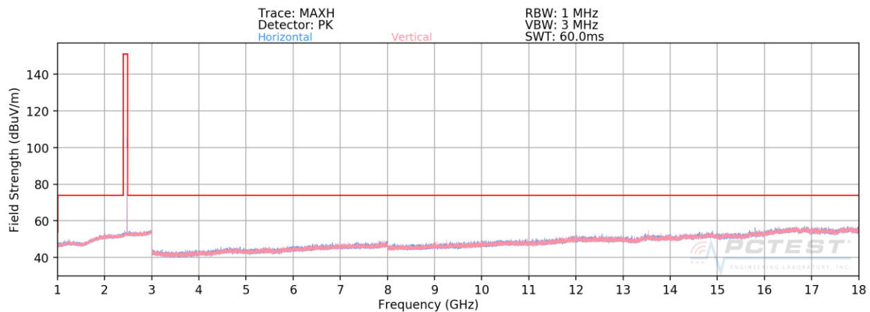
Plot 7-93. Radiated Spurious Plot 1-18GHz Ant-2 (4Mbps, HDR4, ePA – Ch. 75, Ant. Pol. H & V)
