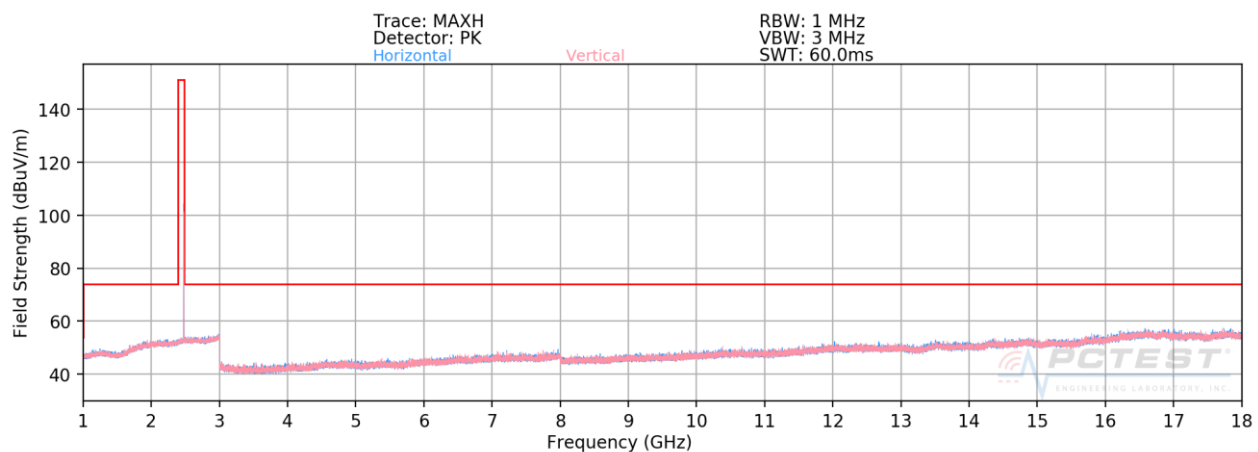
Plot 7-87. Radiated Spurious Plot 1-18GHz Ant-0 (4Mbps, HDR4, ePA – Ch. 75, Ant. Pol. H & V)
