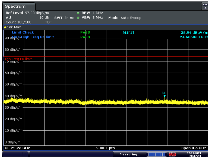
Plot 7-95. Radiated Spurious Plot Above 18GHz Ant-0 (8Mbps, HDR8, ePA – Ch.38, Ant. Pol. V)
