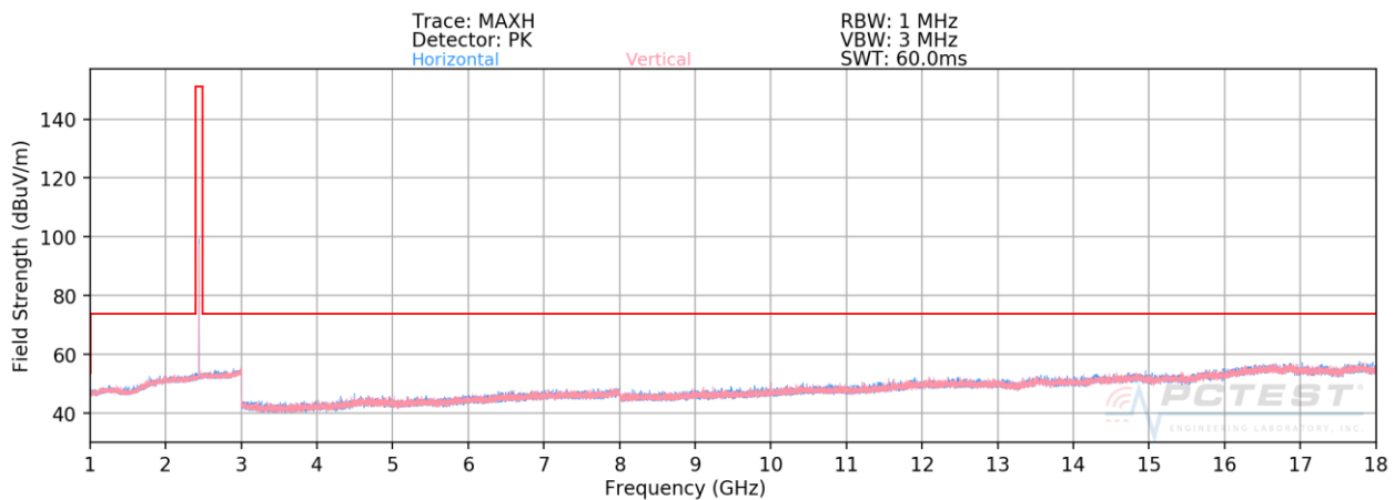
Plot 7-89. Radiated Spurious Plot 1-18GHz Ant-1 (4Mbps, HDR4, ePA – Ch. 38, Ant. Pol. H & V)
