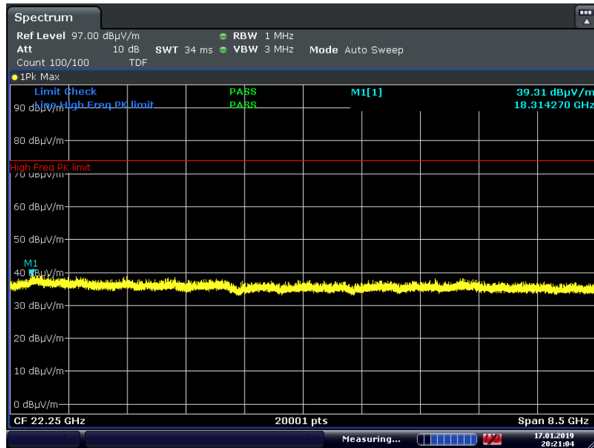
Plot 7-94. Radiated Spurious Plot Above 18GHz Ant-0 (4Mbps, HDR4, ePA – Ch.38, Ant. Pol. H)
