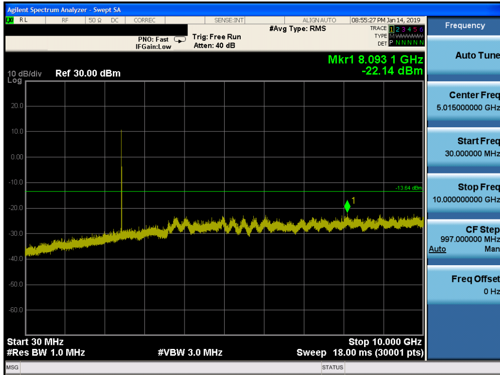
Plot 7-69. Conducted Spurious Plot Ant-0 (Bluetooth (HDR4), Mbps, ePA – Ch. 38)
