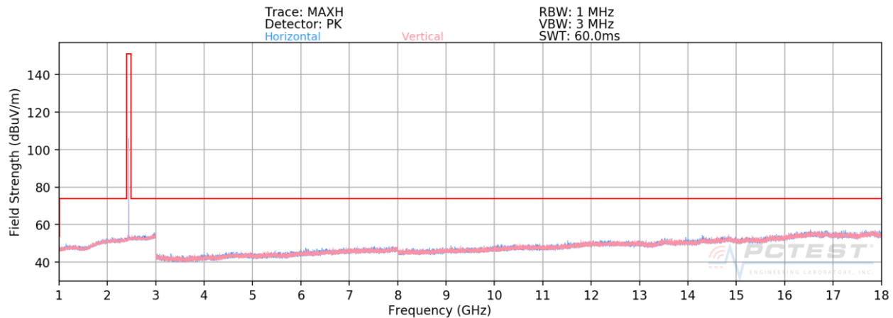
Plot 7-92. Radiated Spurious Plot 1-18GHz Ant-2 (4Mbps, HDR4, ePA – Ch. 38, Ant. Pol. H & V)
