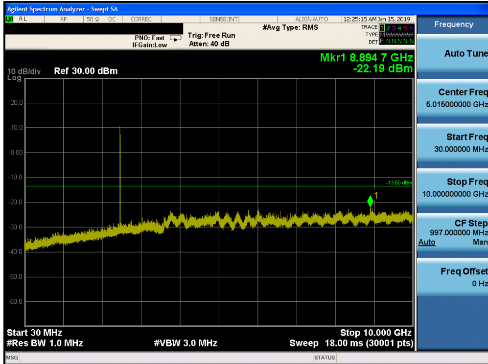
Plot 7-77. Conducted Spurious Plot Ant-1 (Bluetooth (HDR4), Mbps, ePA – Ch. 75)
