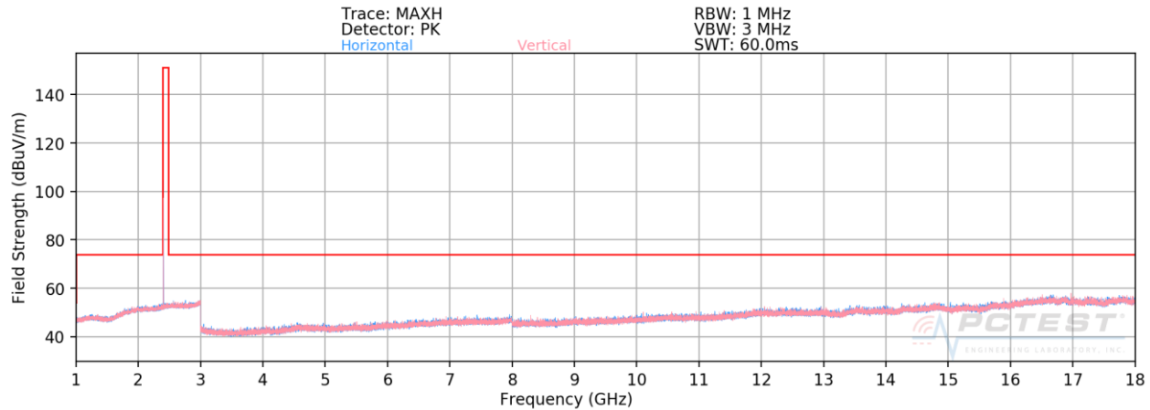
Plot 7-91. Radiated Spurious Plot 1-18GHz Ant-2 (4Mbps, HDR4, ePA – Ch. 1, Ant. Pol. H & V)
