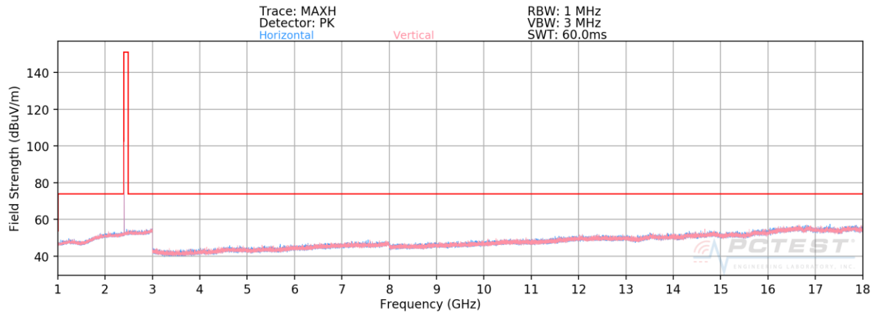
Plot 7-85. Radiated Spurious Plot 1-18GHz Ant-0 (4Mbps, HDR4, ePA – Ch. 1, Ant. Pol. H & V)
