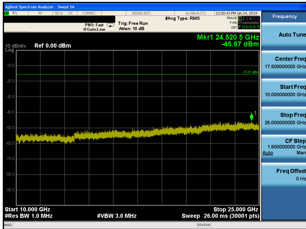
Plot 7-82. Conducted Spurious Plot Ant-2 (Bluetooth (HDR4), Mbps – Ch. 38)
