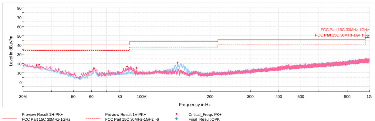
Plot 7-108. Radiated Spurious Plot below 1GHz (4Mbps, ePA – Ch.39, Pol. H & V, with AC/DC Adapter)
