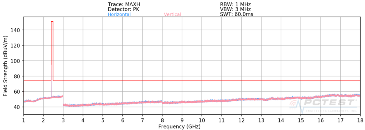
Plot 7-88. Radiated Spurious Plot 1-18GHz Ant-1 (4Mbps, HDR4, ePA – Ch. 1, Ant. Pol. H & V)
