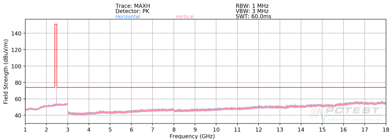
Plot 7-90. Radiated Spurious Plot 1-18GHz Ant-1 (4Mbps, HDR4, ePA – Ch. 75, Ant. Pol. H & V)
