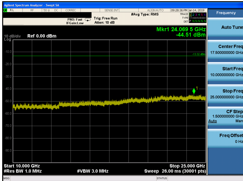
Plot 7-72. Conducted Spurious Plot Ant-0 (Bluetooth (HDR4), Mbps, ePA – Ch. 75)
