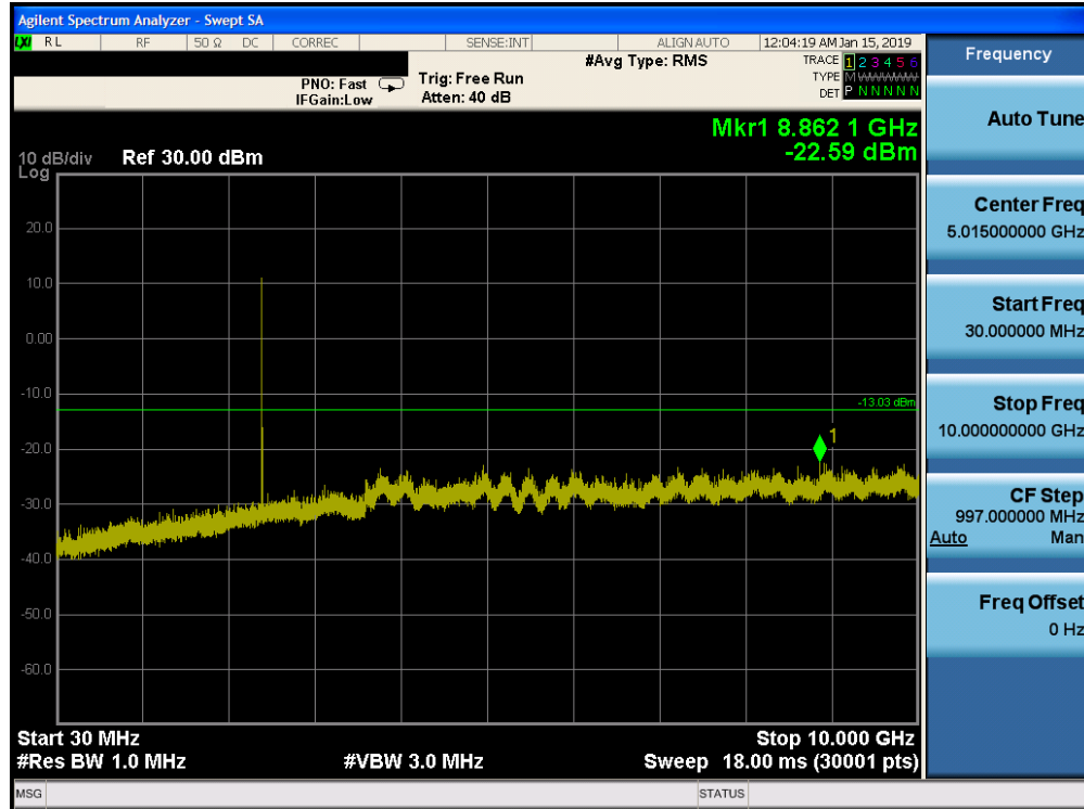
Plot 7-73. Conducted Spurious Plot Ant-1 (Bluetooth (HDR4), Mbps, ePA – Ch. 1)
