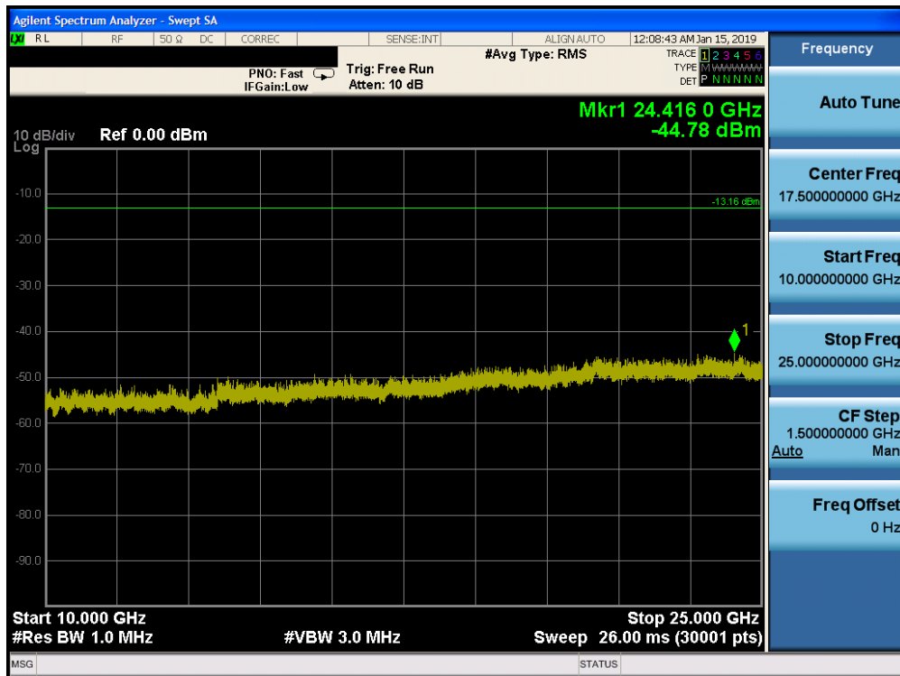
Plot 7-76. Conducted Spurious Plot Ant-1 (Bluetooth (HDR4), Mbps – Ch. 38)
