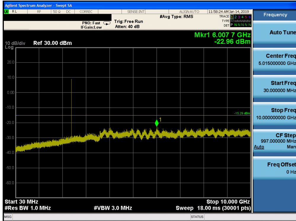
Plot 7-79. Conducted Spurious Plot Ant-2 (Bluetooth (HDR4), Mbps, ePA – Ch. 1)
