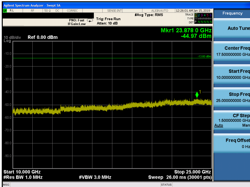
Plot 7-78. Conducted Spurious Plot Ant-1 (Bluetooth (HDR4), Mbps, ePA – Ch. 75)
