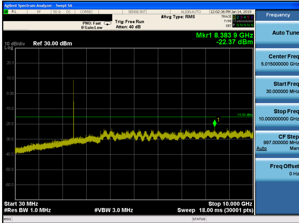
Plot 7-83. Conducted Spurious Plot Ant-2 (Bluetooth (HDR4), Mbps, ePA – Ch. 75)
