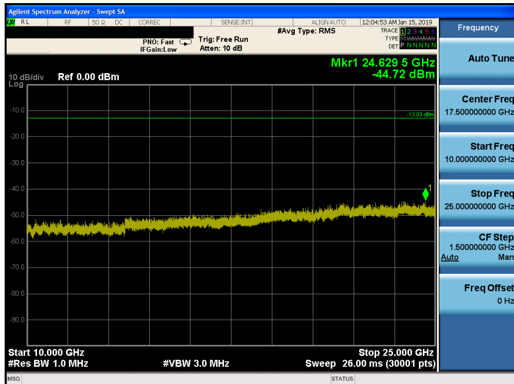
Plot 7-74. Conducted Spurious Plot Ant-1 (Bluetooth (HDR4), Mbps, ePA – Ch. 1)
