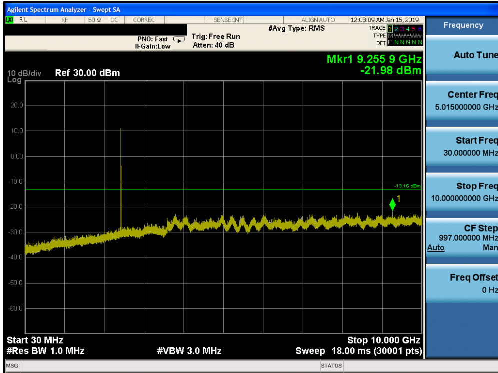
Plot 7-75. Conducted Spurious Plot Ant-1 (Bluetooth (HDR4), Mbps, ePA – Ch. 38)
