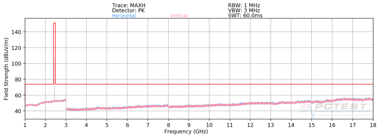
Plot 7-86. Radiated Spurious Plot 1-18GHz Ant-0 (4Mbps, HDR4, ePA – Ch. 38, Ant. Pol. H & V)
