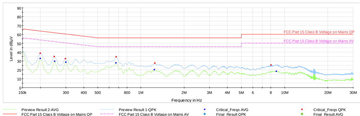
Plot 7-109. Line Conducted Plot with Bluetooth HDR4 – Ch.39 (L1, with AC/DC Adapter)
