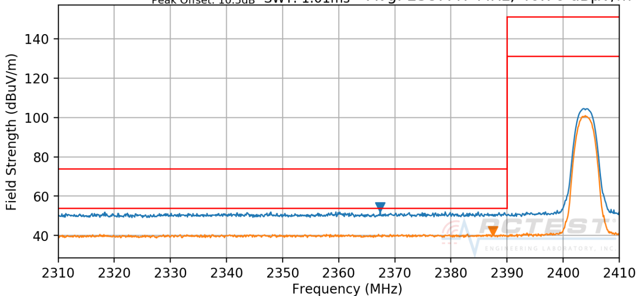
Plot 7-104. Radiated Restricted Lower Band Edge Measurement Ant-2 (Average & Peak)
