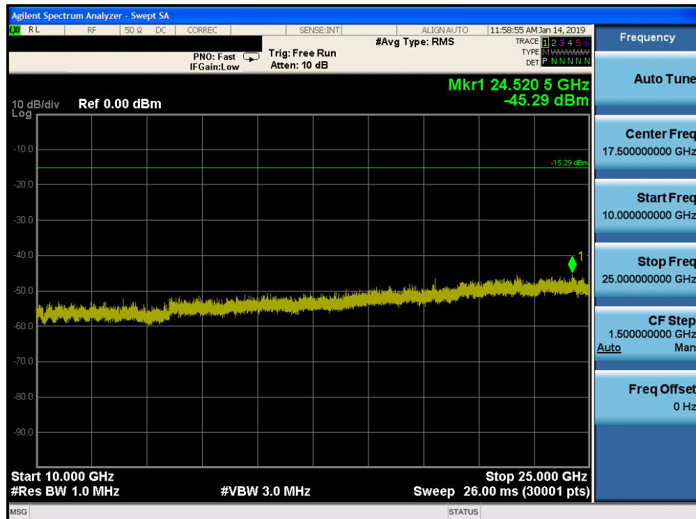
Plot 7-80. Conducted Spurious Plot Ant-2 (Bluetooth (HDR4), Mbps, ePA – Ch. 1)
