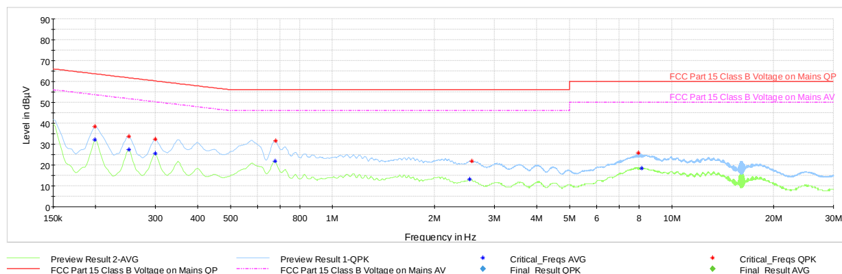
Plot 7-110. Line Conducted Plot with Bluetooth HDR4 – Ch.39 (N, with AC/DC Adapter)
