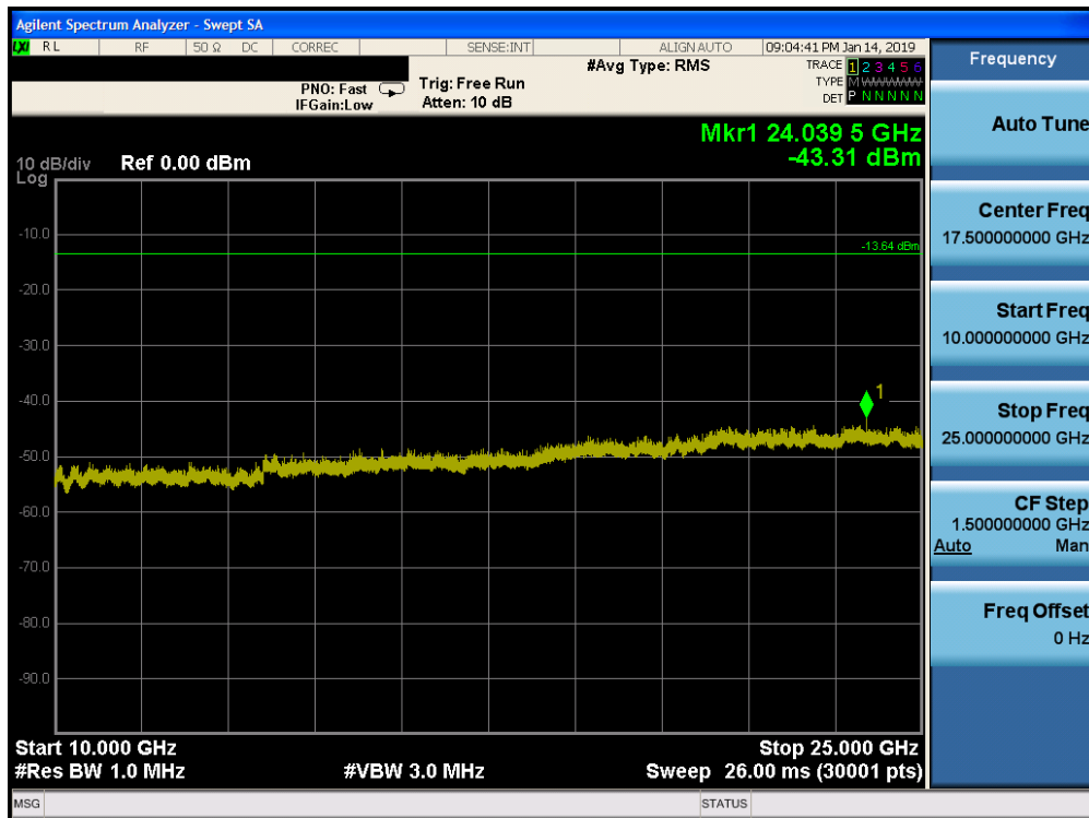
Plot 7-70. Conducted Spurious Plot Ant-0 (Bluetooth (HDR4), Mbps – Ch. 38)
