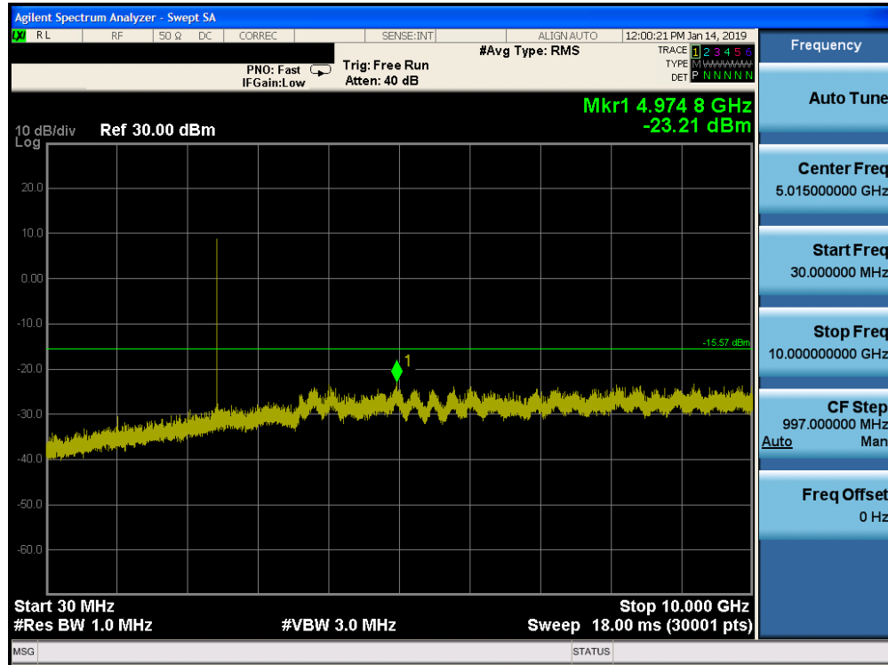
Plot 7-81. Conducted Spurious Plot Ant-2 (Bluetooth (HDR4), Mbps, ePA – Ch. 38)
