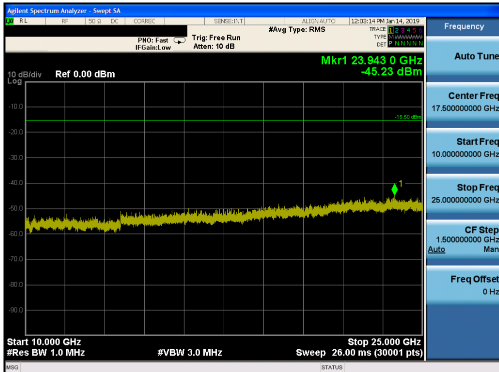
Plot 7-84. Conducted Spurious Plot Ant-2 (Bluetooth (HDR4), Mbps, ePA – Ch. 75)
