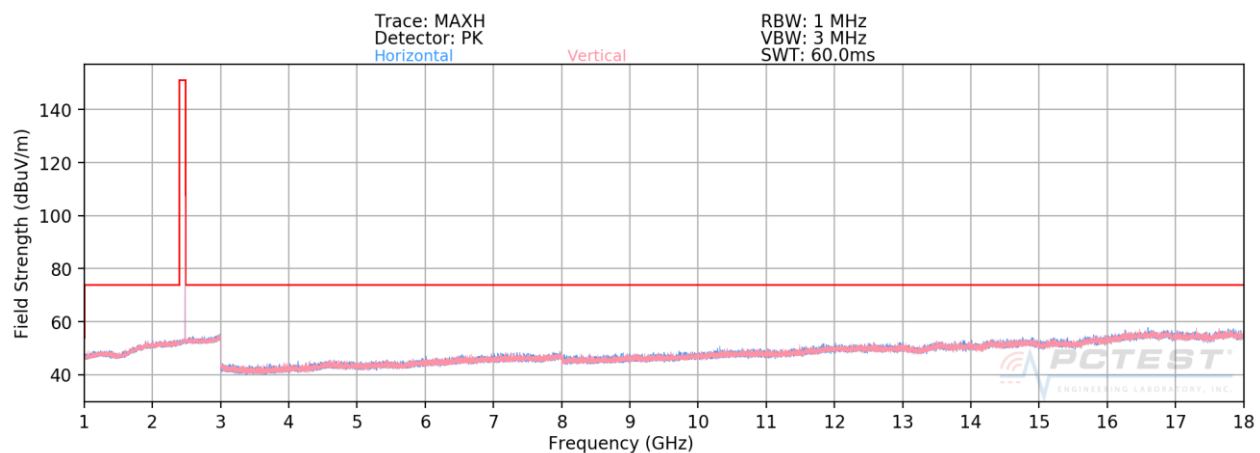
Plot 7-90. Radiated Spurious Plot Above 1GHz ANT 1 (1Mbps, ePA – Ch. 39)
