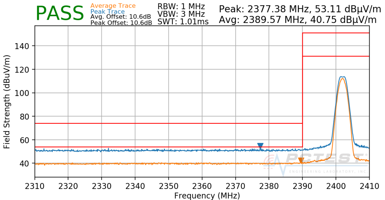
Plot 7-97. Radiated Restricted Lower Band Edge Measurement ANT 0 (Average & Peak)
