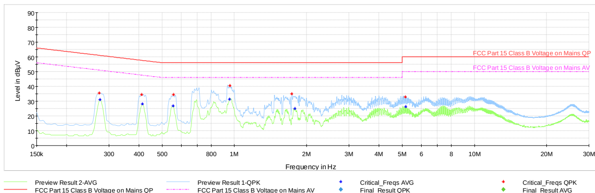
Plot 7-110. Line Conducted Plot with Bluetooth LE (N, with AC/DC Adapter)
