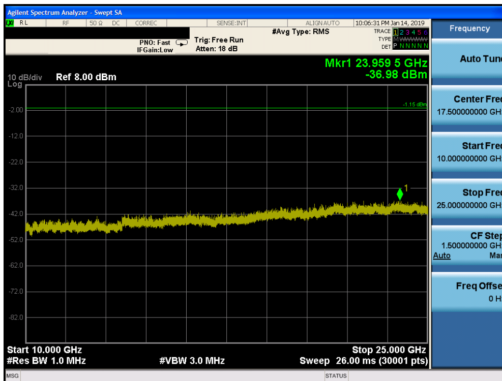
Plot 7-80. Conducted Spurious Plot ANT 1 (Bluetooth, GFSK, ePA – Ch. 0)
