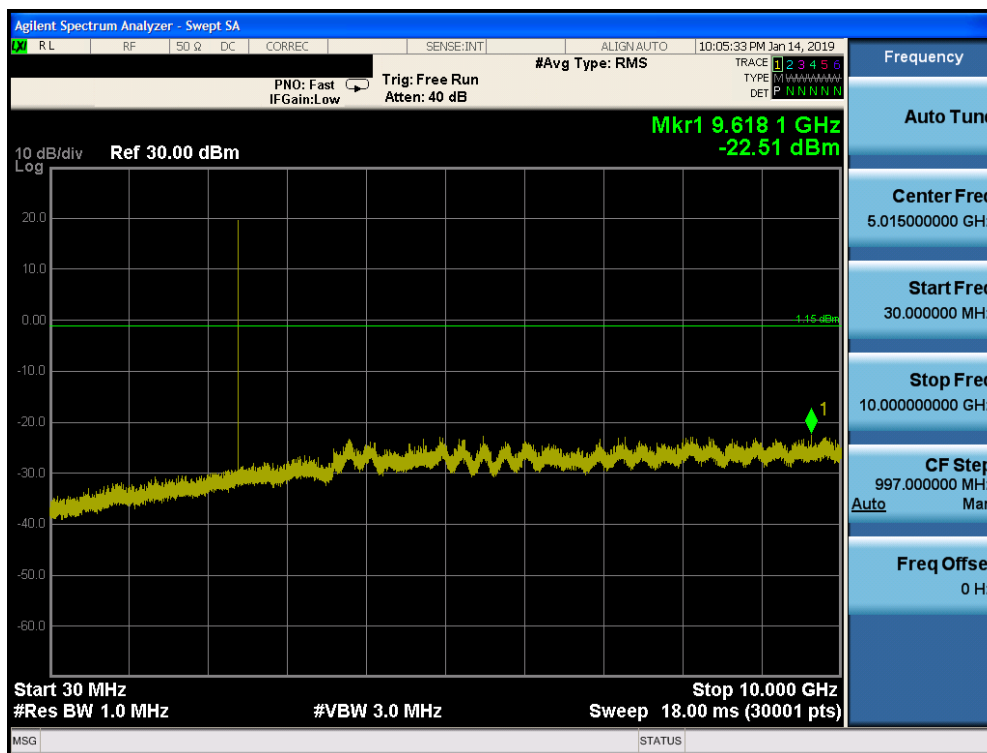
Plot 7-79. Conducted Spurious Plot ANT 1 (Bluetooth, GFSK, ePA – Ch. 0)
