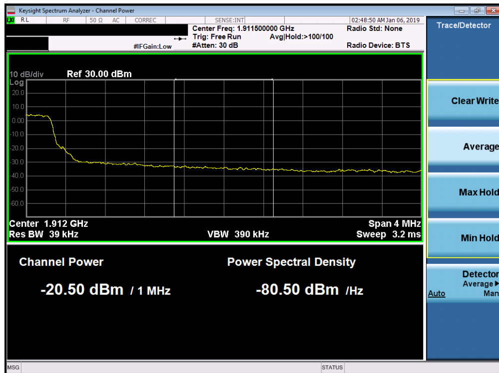
Plot 7-293. Upper Extended Band Edge Plot (Band 2 - 5.0MHz QPSK - Full RB Configuration)
