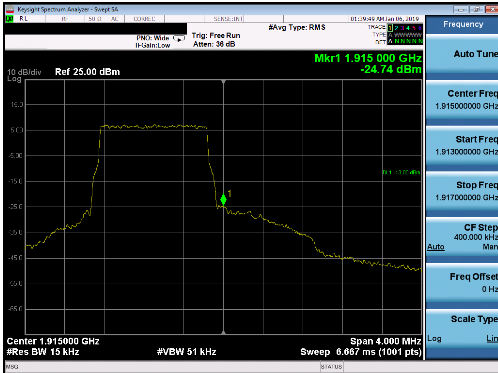
Plot 7-308. Upper Band Edge Plot (Band 25 - 1.4MHz QPSK - Full RB Configuration)
