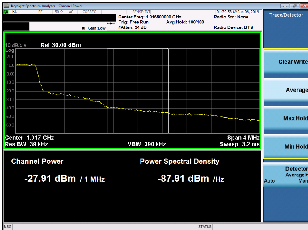
Plot 7-309. Upper Extended Band Edge Plot (Band 25 - 1.4MHz QPSK - Full RB Configuration)
