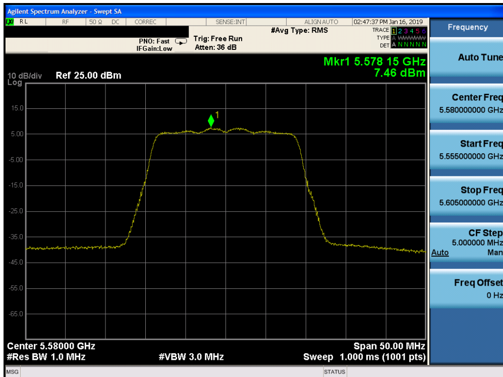
Plot 7-92. Power Spectral Density Plot SISO CORE 1 (20MHz BW 802.11n (UNII Band 2C) – Ch. 116)
