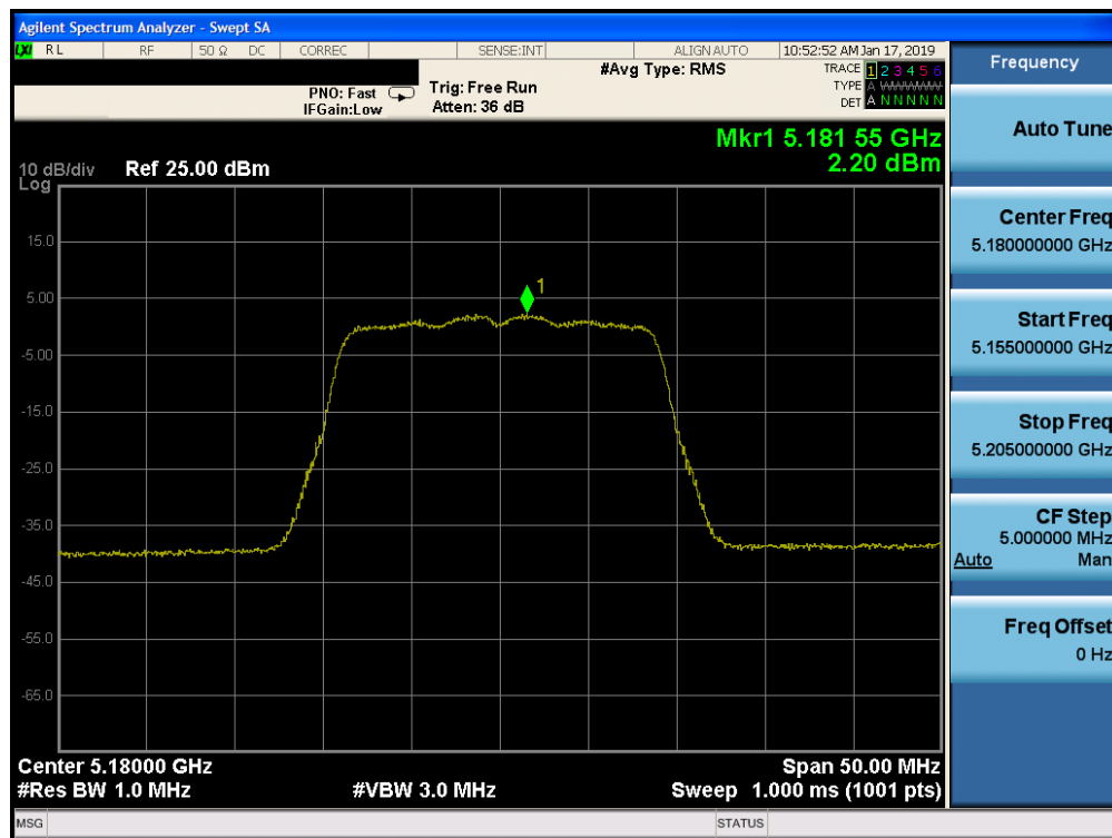
Plot 7-105. Power Spectral Density Plot MIMO/CDD CORE 0 (20MHz BW 802.11n (UNII Band 1) – Ch. 36)
