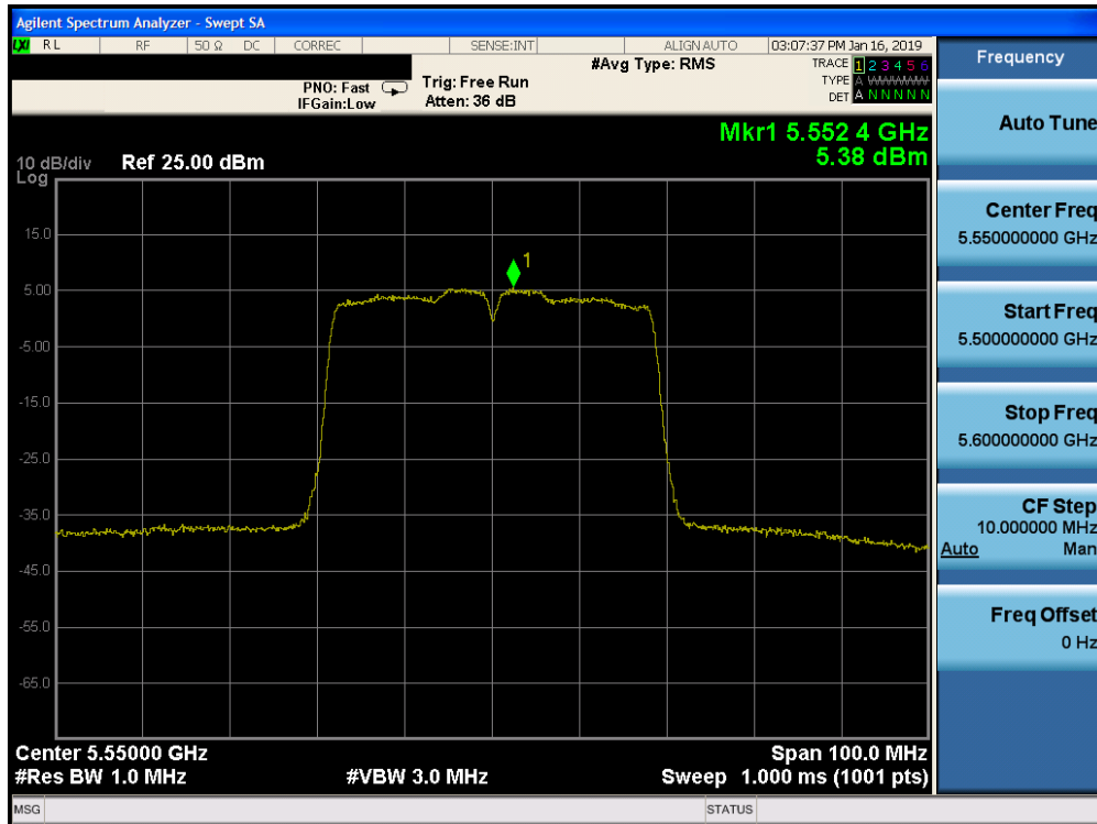
Plot 7-95. Power Spectral Density Plot SISO CORE 1 (40MHz BW 802.11n (UNII Band 2C) – Ch. 110)
