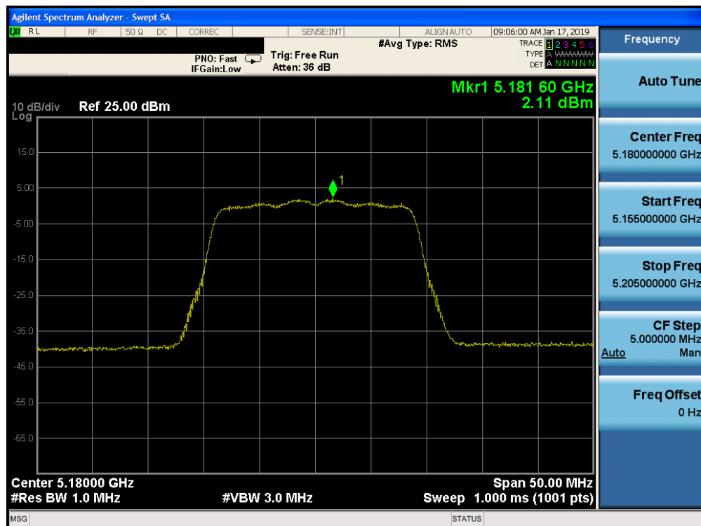
Plot 7-106. Power Spectral Density Plot MIMO/CDD CORE 1 (20MHz BW 802.11n (UNII Band 1) – Ch. 36)
