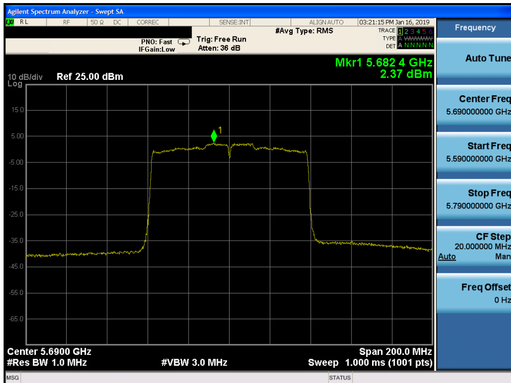
Plot 7-98. Power Spectral Density Plot SISO CORE 1 (80MHz BW 802.11ac (UNII Band 2C) – Ch. 138)
