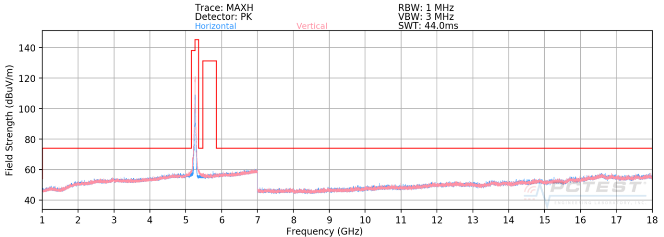
Plot 7-184. Radiated Spurious Plot above 1GHz MIMO/CDD (802.11n – U2A Ch. 52)
