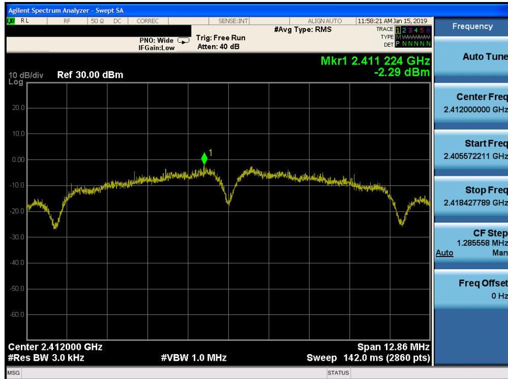
Plot 7-37. Power Spectral Density Plot SISO CORE 0 DIVERSITY (802.11b – Ch. 1)
