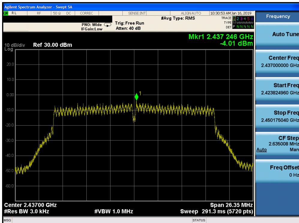
Plot 7-64. Power Spectral Density Plot CDD PRIMARY CORE 1 (802.11n (2.4GHz) – Ch. 6)
