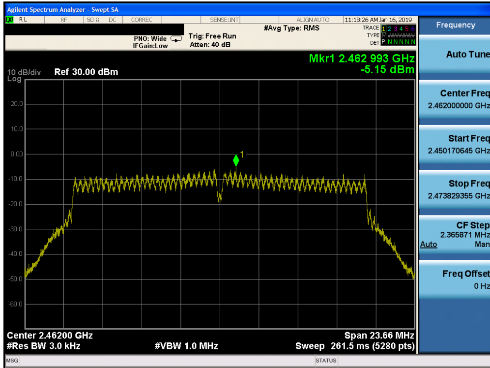
Plot 7-77. Power Spectral Density Plot CDD DIVERSITY CORE 0 (802.11n (2.4GHz) – Ch. 11)
