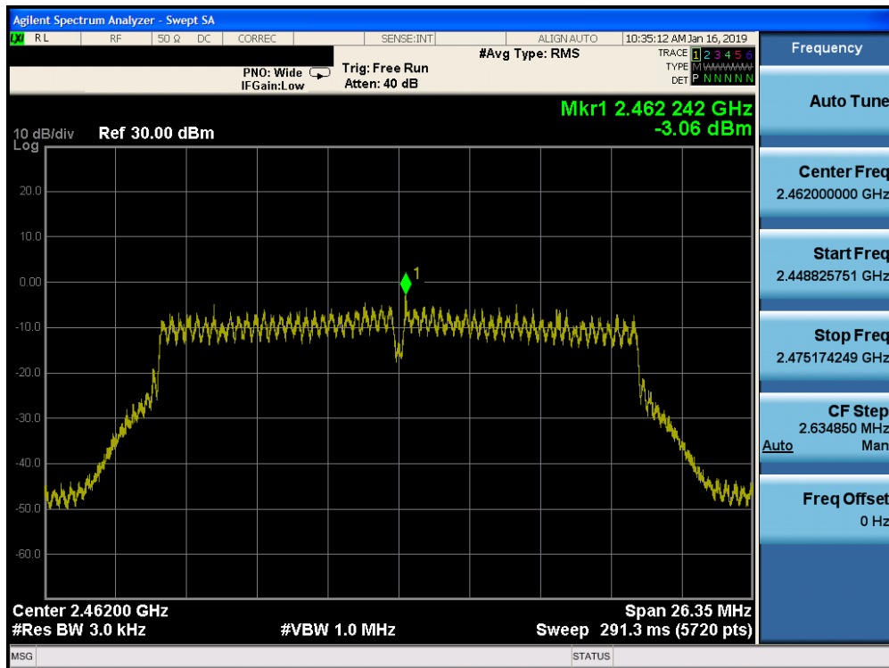
Plot 7-66. Power Spectral Density Plot CDD PRIMARY CORE 1 (802.11n (2.4GHz) – Ch. 11)
