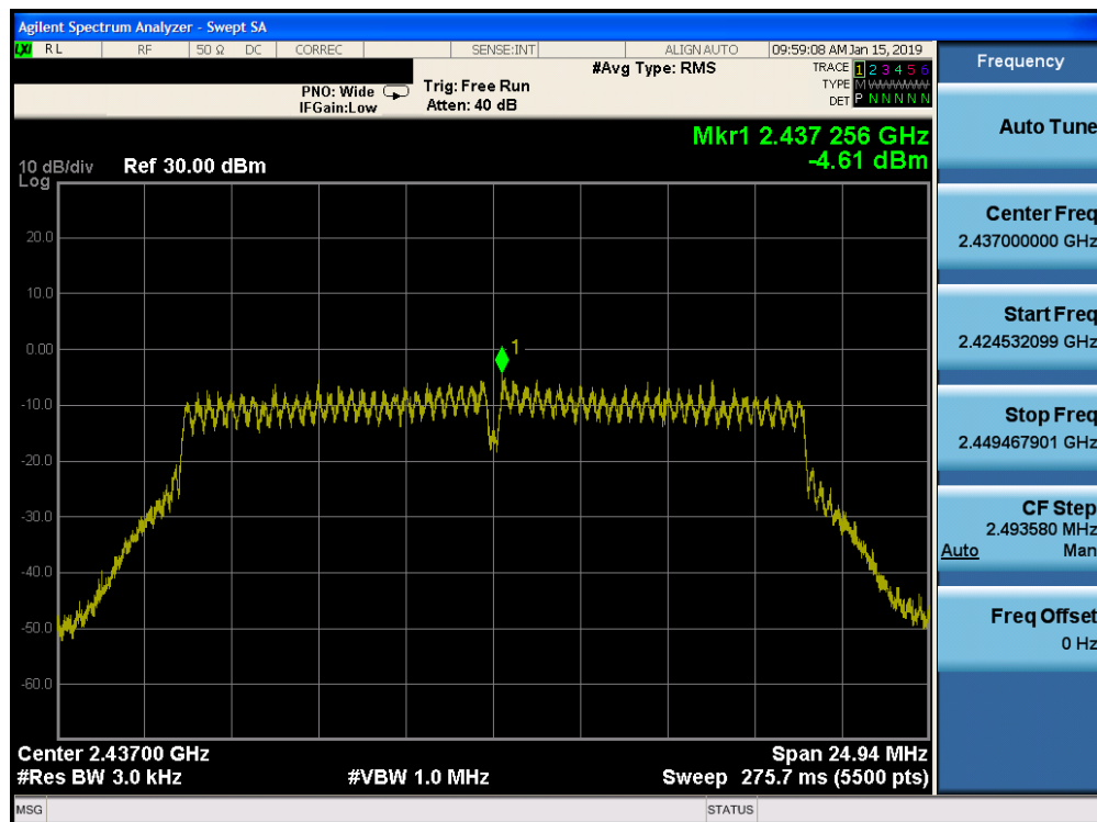
Plot 7-35. Power Spectral Density Plot SISO CORE 0 PRIMARY (802.11n (2.4GHz) – Ch. 6)
