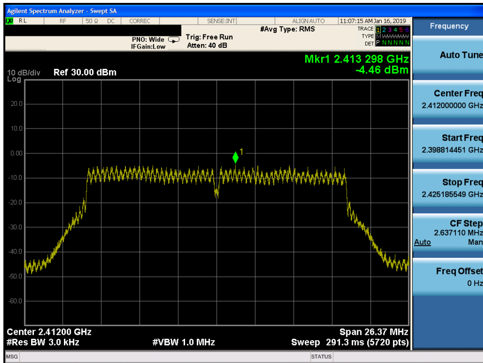
Plot 7-74. Power Spectral Density Plot CDD CORE 1 (802.11n (2.4GHz) – Ch. 1)
