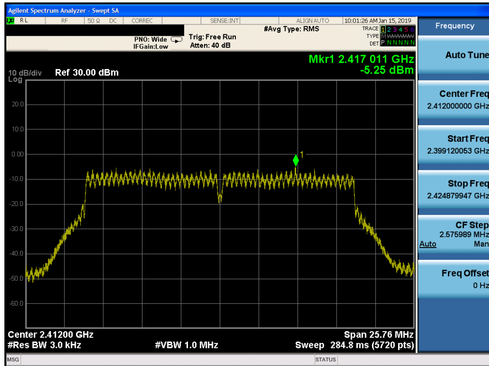
Plot 7-34. Power Spectral Density Plot SISO CORE 0 PRIMARY (802.11n (2.4GHz) – Ch. 1)
