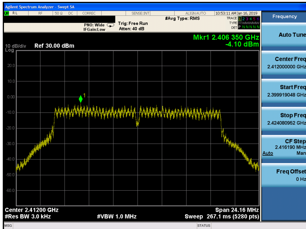
Plot 7-68. Power Spectral Density Plot CDD CORE 1 (802.11g – Ch. 1)
