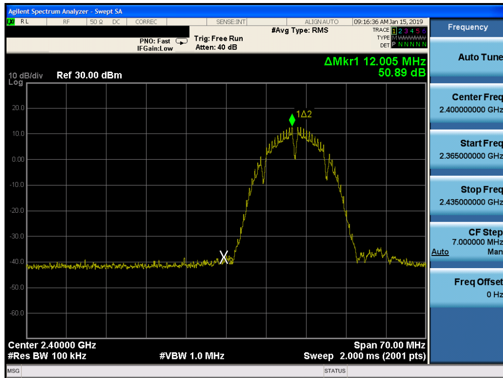
Plot 7-79. Band Edge Plot SISO CORE 0 PRIMARY (802.11b – Ch. 1)
