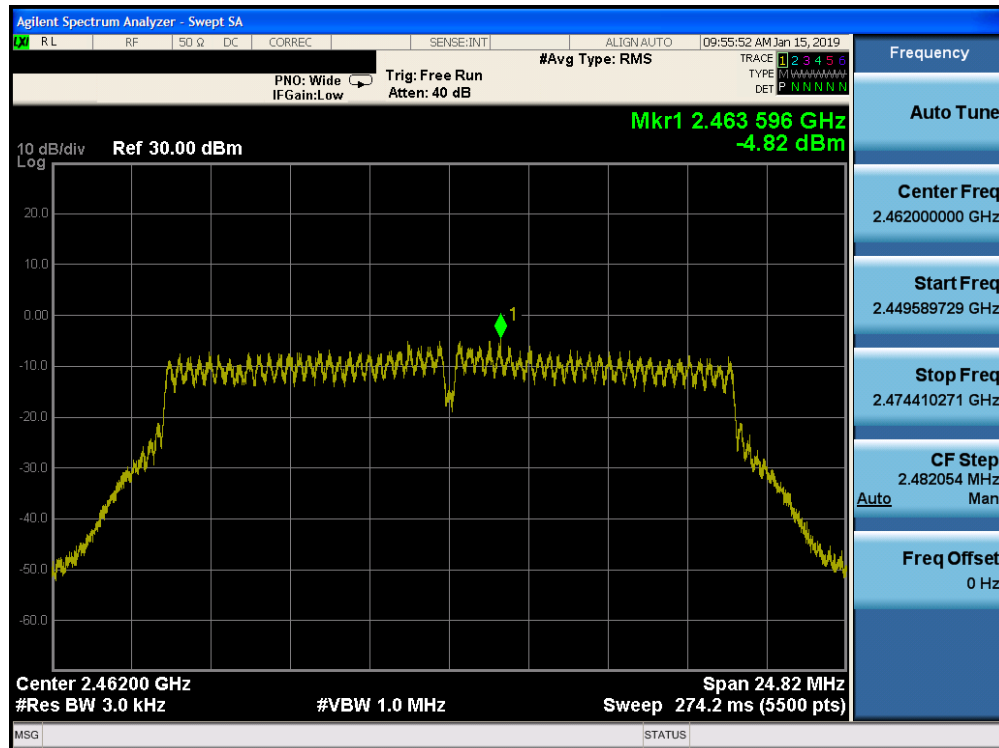
Plot 7-36. Power Spectral Density Plot SISO CORE 0 PRIMARY (802.11n (2.4GHz) – Ch. 11)
