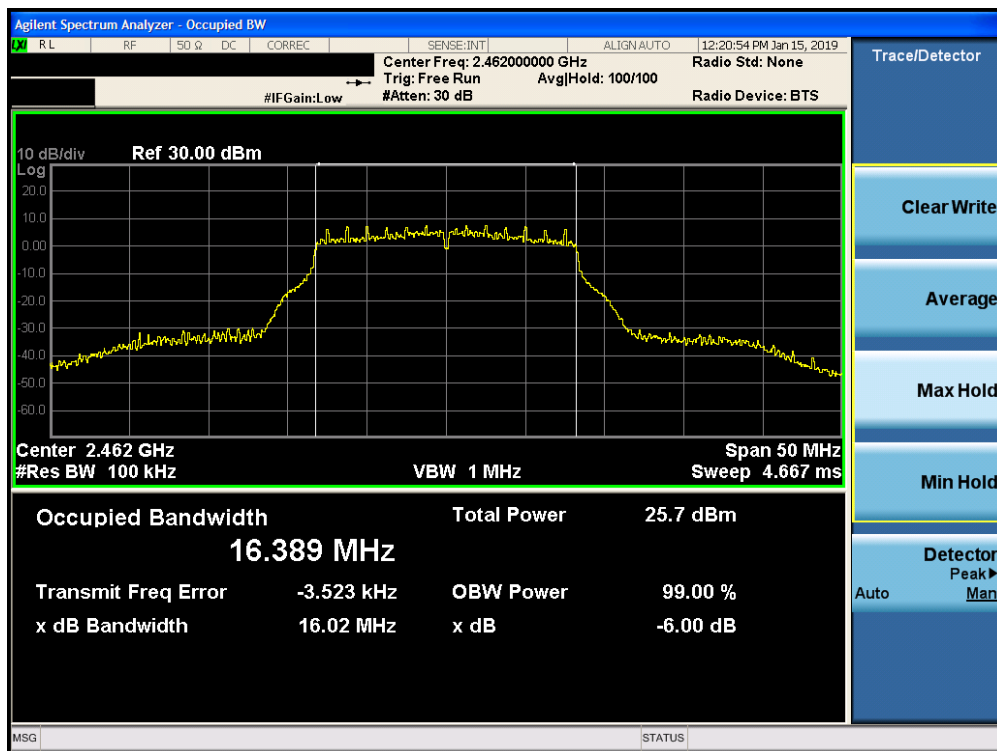
Plot 7-15. 6dB Bandwidth Plot SISO CORE 0 DIVERSITY (802.11g – Ch. 11)
