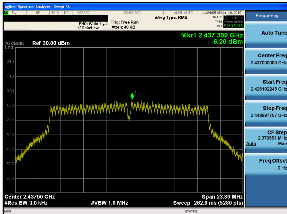
Plot 7-69. Power Spectral Density Plot CDD DIVERSITY CORE 0 (802.11g – Ch. 6)
