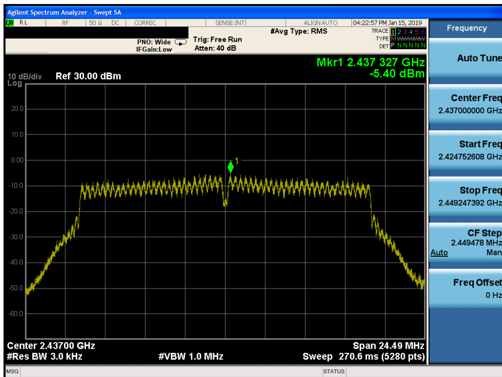
Plot 7-53. Power Spectral Density Plot SISO CORE 1 (802.11n (2.4GHz) – Ch. 6)
