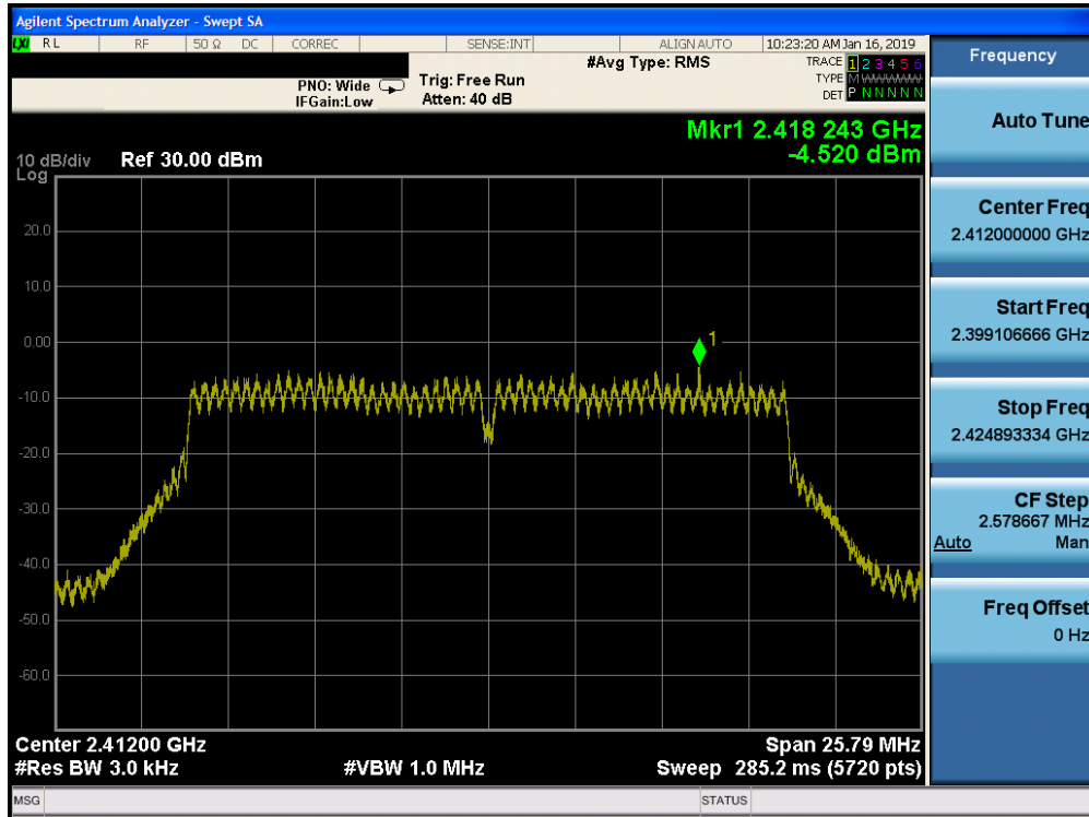
Plot 7-61. Power Spectral Density Plot CDD PRIMARY CORE 0 (802.11n (2.4GHz) - Ch. 1)
