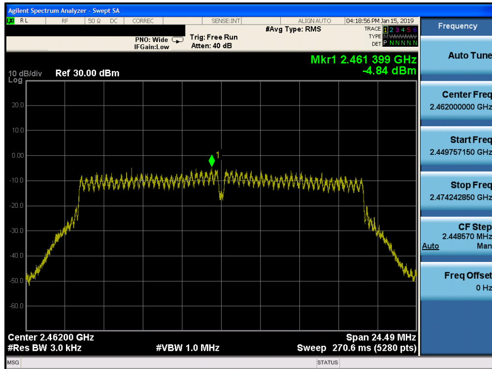
Plot 7-54. Power Spectral Density Plot SISO CORE 1 (802.11n (2.4GHz) – Ch. 11)
