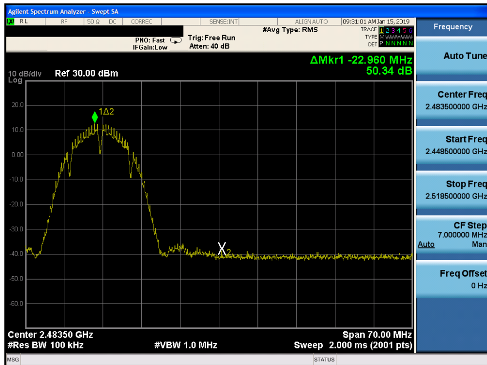
Plot 7-80. Band Edge Plot SISO CORE 0 PRIMARY (802.11b – Ch. 11)
