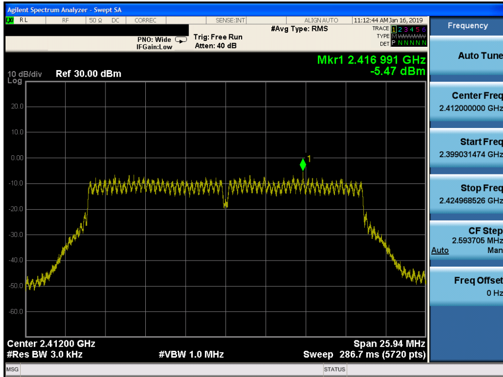
Plot 7-73. Power Spectral Density Plot CDD DIVERSITY CORE 0 (802.11n (2.4GHz) – Ch. 1)
