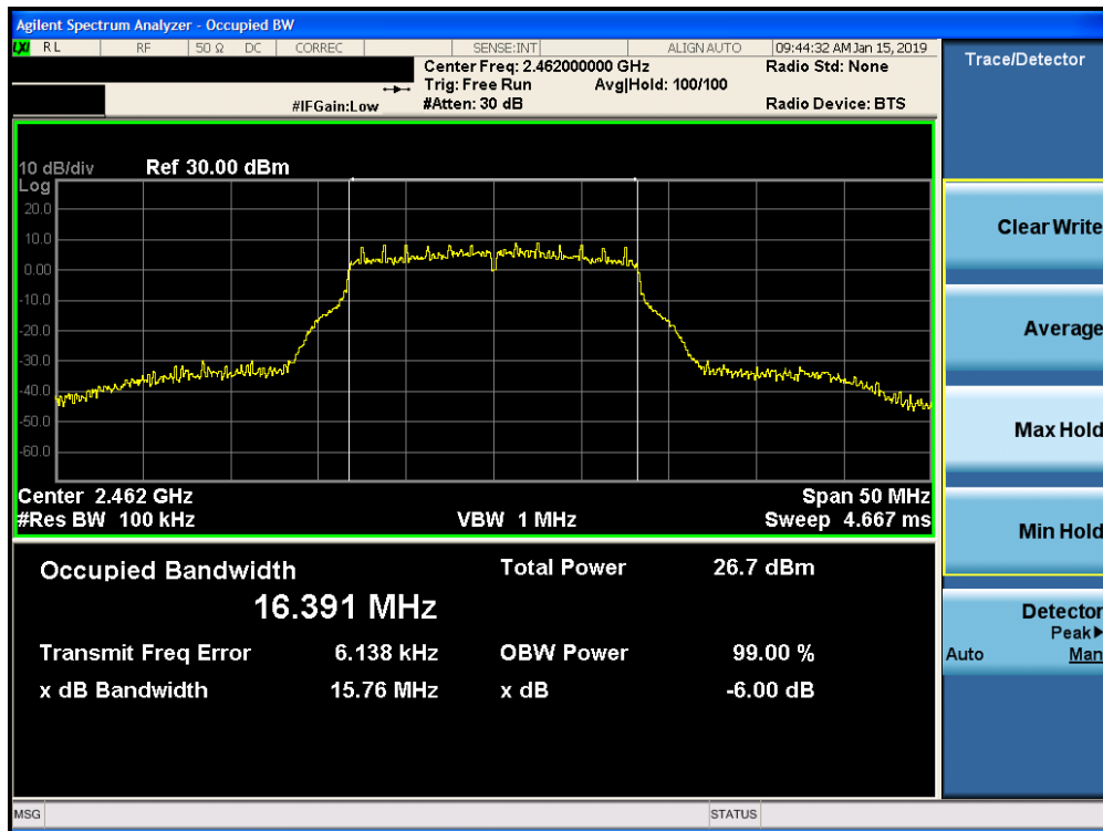
Plot 7-6. 6dB Bandwidth Plot SISO CORE 0 PRIMARY (802.11g – Ch. 11)
