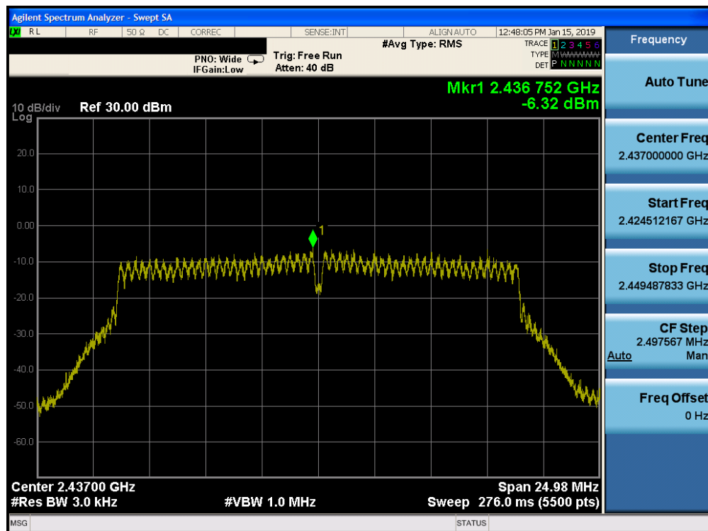
Plot 7-44. Power Spectral Density Plot SISO CORE 0 DIVERSITY (802.11n (2.4GHz) – Ch. 6)
