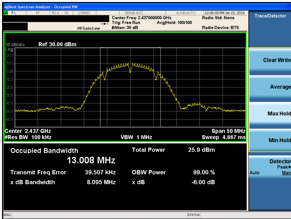
Plot 7-11. 6dB Bandwidth Plot SISO CORE 0 DIVERSITY (802.11b – Ch. 6)
