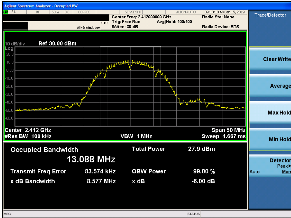
Plot 7-1. 6dB Bandwidth Plot SISO CORE 0 PRIMARY (802.11b – Ch. 1)
