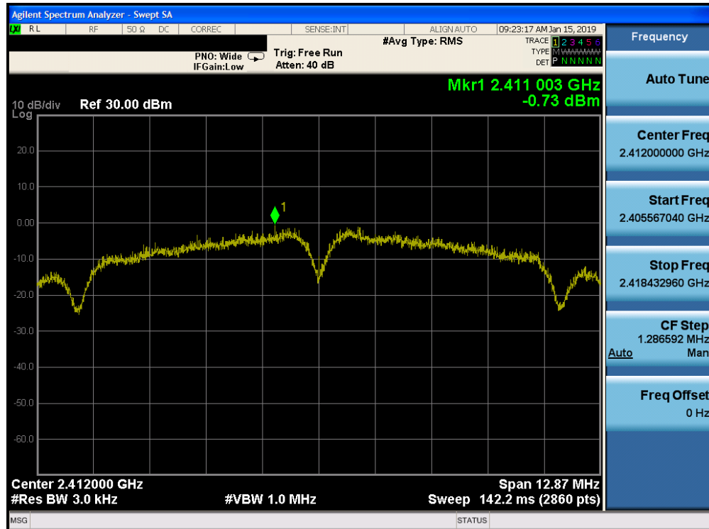
Plot 7-28. Power Spectral Density Plot SISO CORE 0 PRIMARY (802.11b – Ch. 1)
