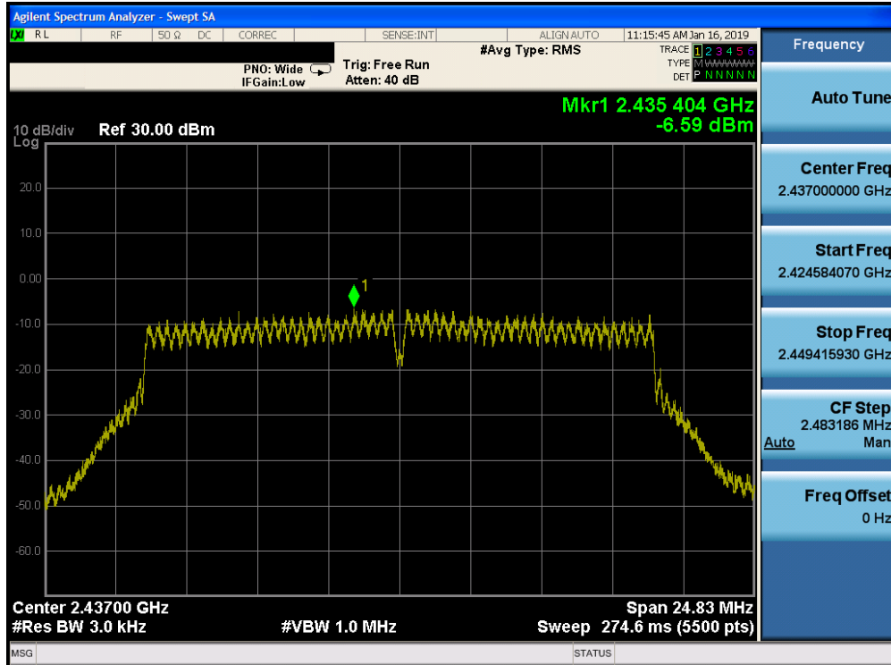
Plot 7-75. Power Spectral Density Plot CDD DIVERSITY CORE 0 (802.11n (2.4GHz) – Ch. 6)
