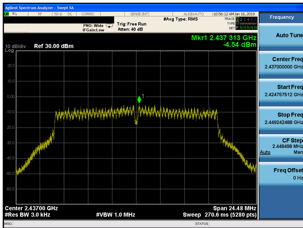
Plot 7-70. Power Spectral Density Plot CDD CORE 1 (802.11g – Ch. 6)
