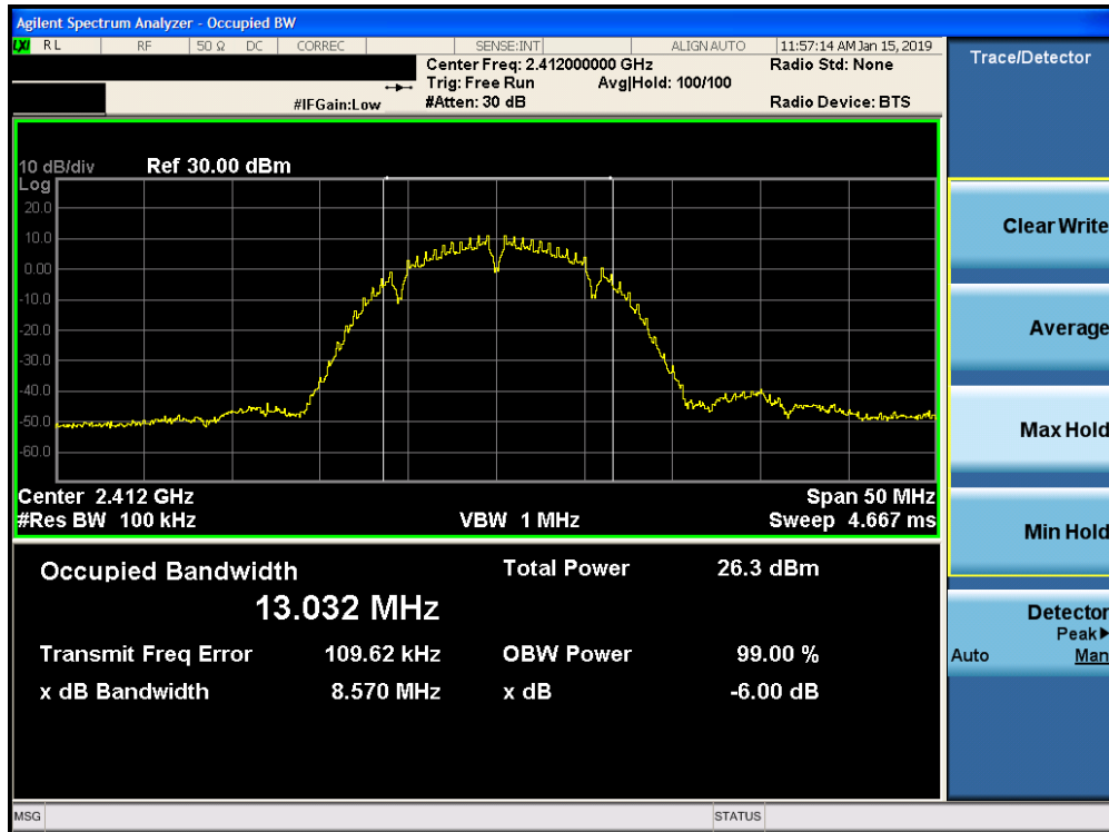
Plot 7-10. 6dB Bandwidth Plot SISO CORE 0 DIVERSITY (802.11b – Ch. 1)
