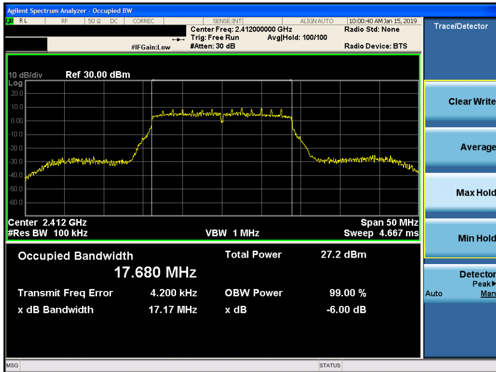
Plot 7-7. 6dB Bandwidth Plot SISO CORE 0 PRIMARY (802.11n (2.4GHz) – Ch. 1)
