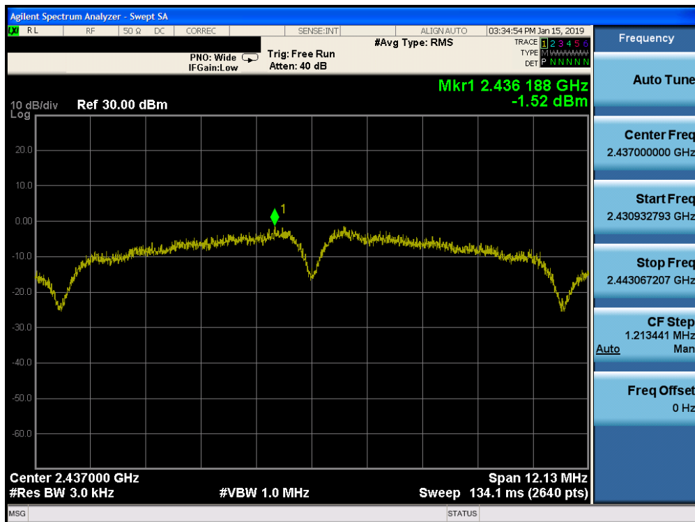
Plot 7-47. Power Spectral Density Plot SISO CORE 1 (802.11b – Ch. 6)
