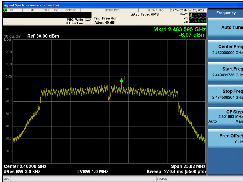
Plot 7-45. Power Spectral Density Plot SISO CORE 0 DIVERSITY (802.11n (2.4GHz) – Ch. 11)
