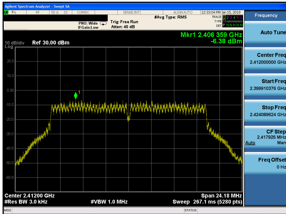
Plot 7-40. Power Spectral Density Plot SISO CORE 0 DIVERSITY (802.11g – Ch. 1)
