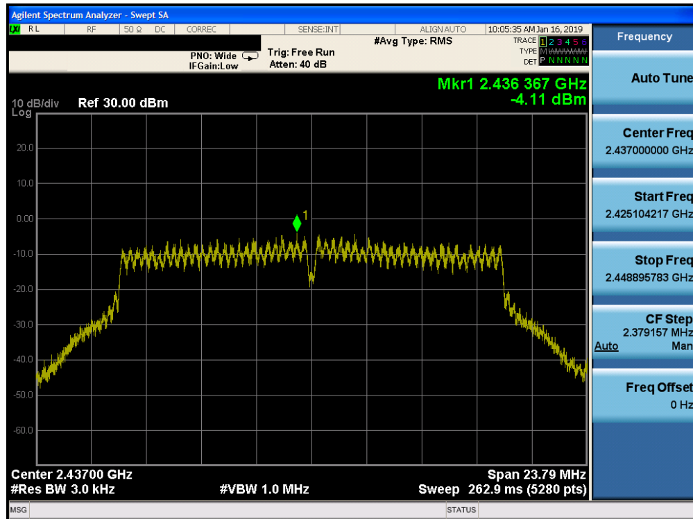
Plot 7-57. Power Spectral Density Plot CDD PRIMARY CORE 0 (802.11g – Ch. 6)
