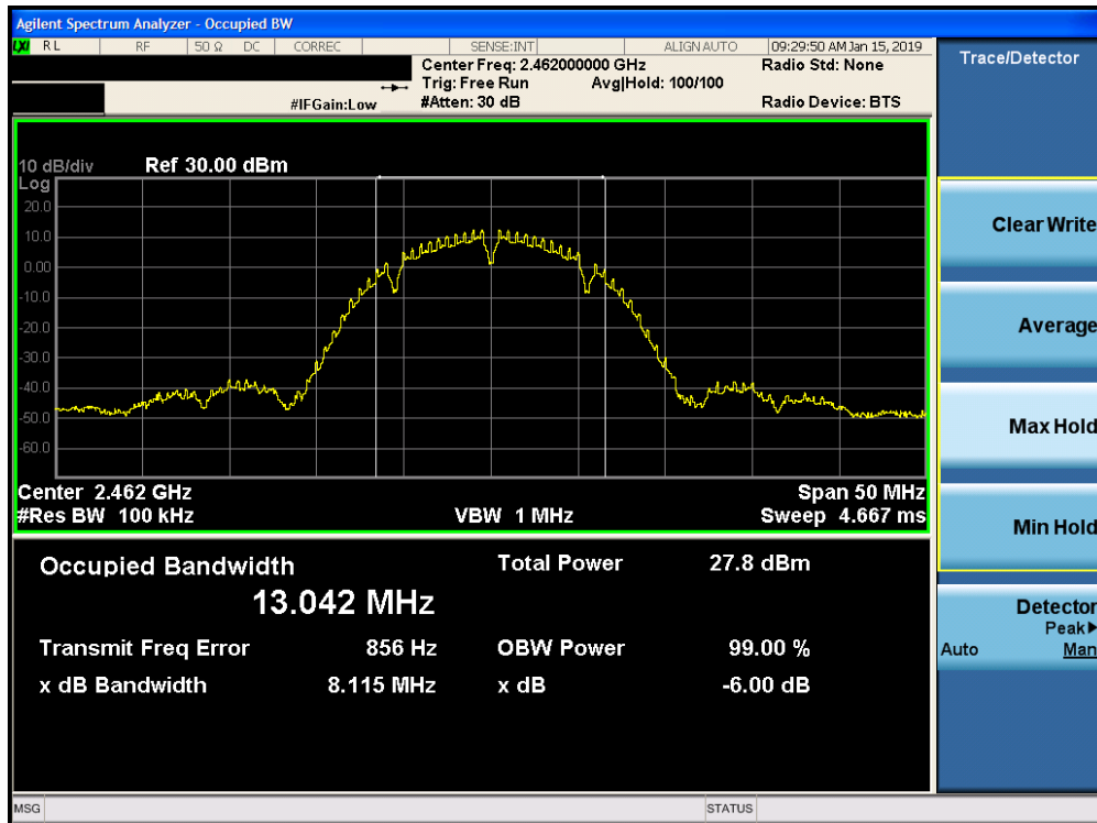
Plot 7-3. 6dB Bandwidth Plot SISO CORE 0 PRIMARY (802.11b – Ch. 11)
