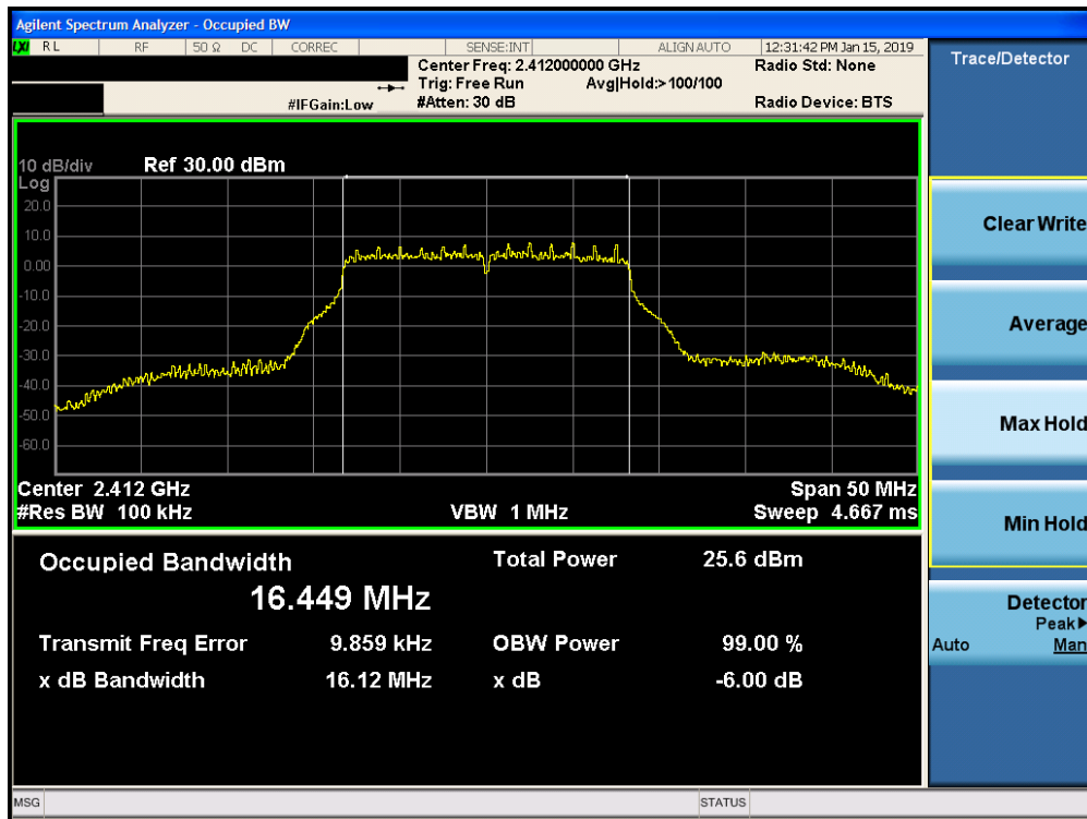
Plot 7-13. 6dB Bandwidth Plot SISO CORE 0 DIVERSITY (802.11g – Ch. 1)
