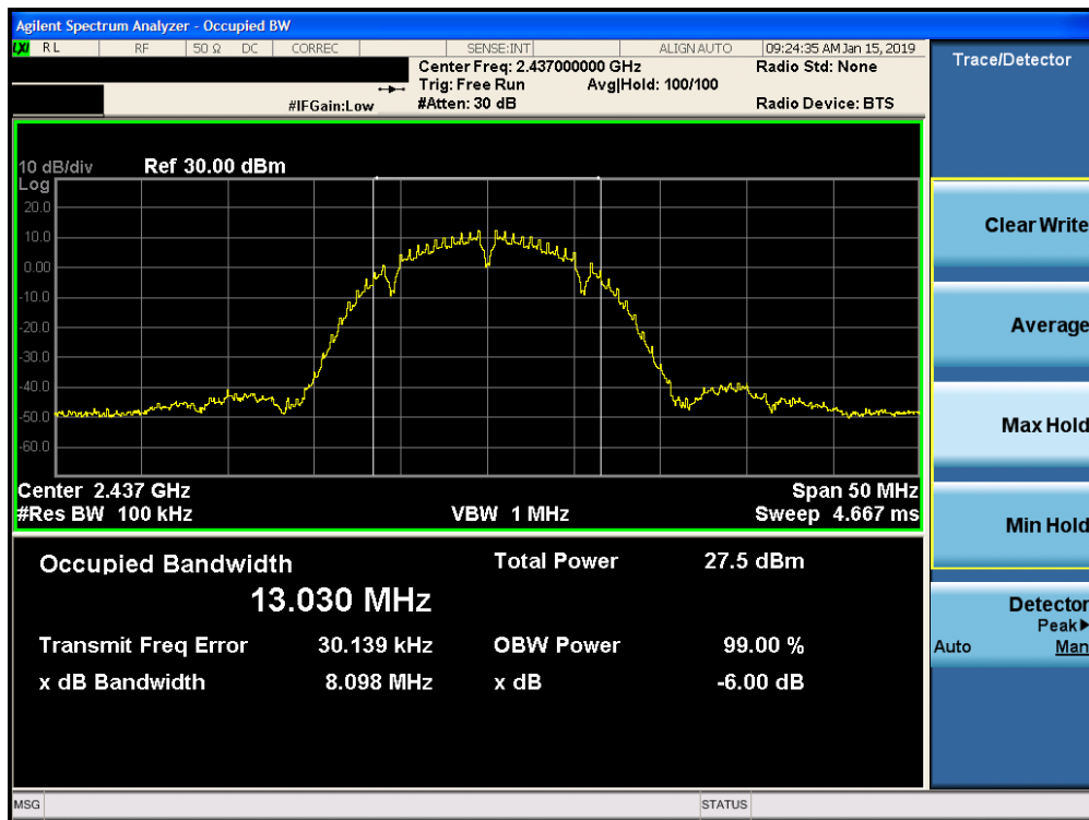
Plot 7-2. 6dB Bandwidth Plot SISO CORE 0 PRIMARY (802.11b – Ch. 6)
