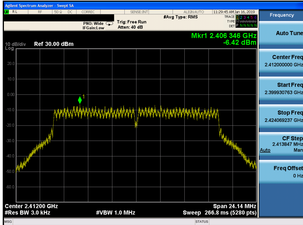
Plot 7-67. Power Spectral Density Plot CDD DIVERSITY CORE 0 (802.11g – Ch. 1)
