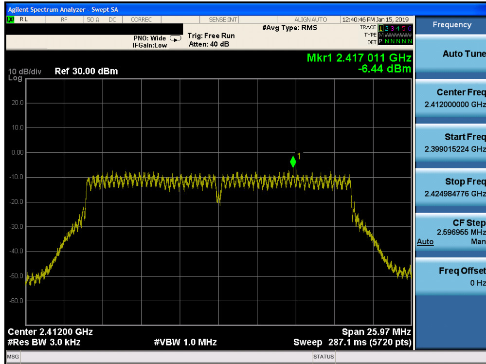
Plot 7-43. Power Spectral Density Plot SISO CORE 0 DIVERSITY (802.11n (2.4GHz) – Ch. 1)
