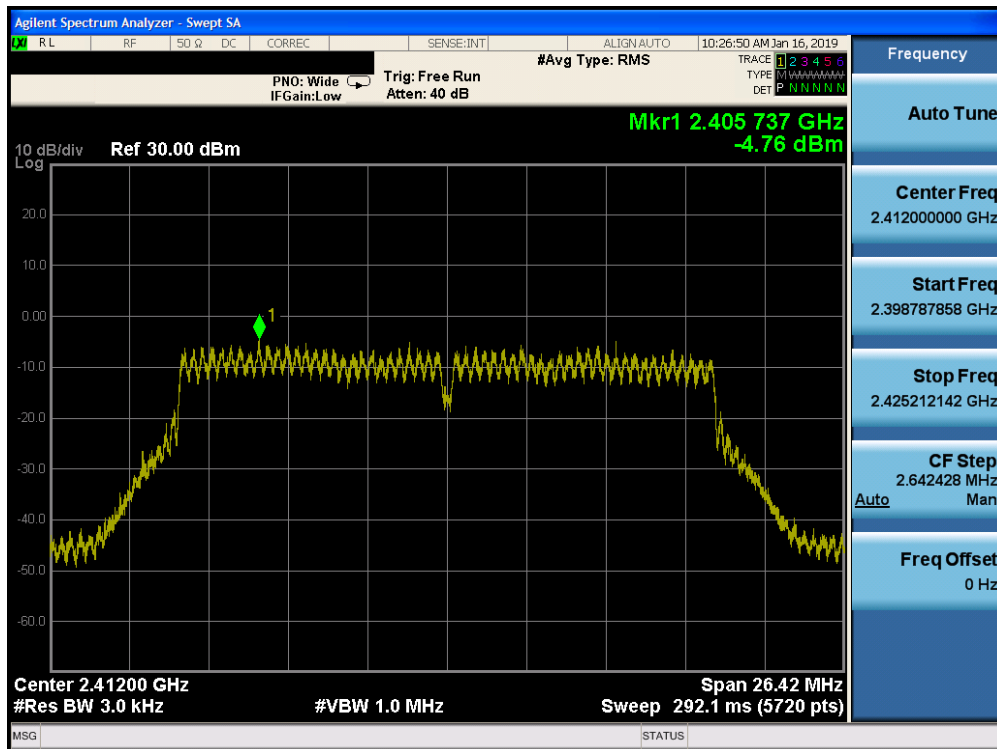
Plot 7-62. Power Spectral Density Plot CDD PRIMARY CORE 1 (802.11n (2.4GHz) - Ch. 1)
