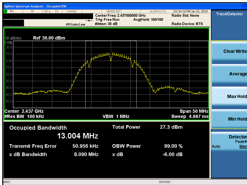
Plot 7-20. 6dB Bandwidth Plot SISO CORE 1 (802.11b – Ch. 6)
