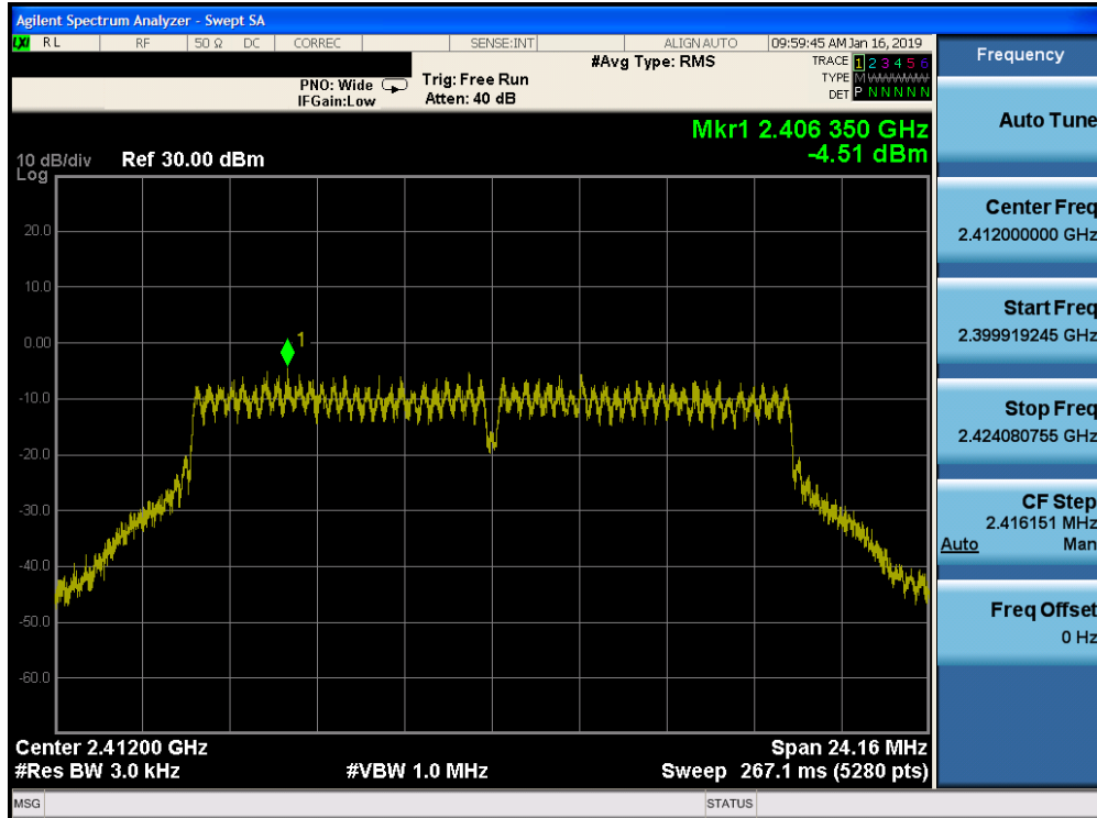
Plot 7-55. Power Spectral Density Plot CDD PRIMARY CORE 0 (802.11g - Ch. 1)
