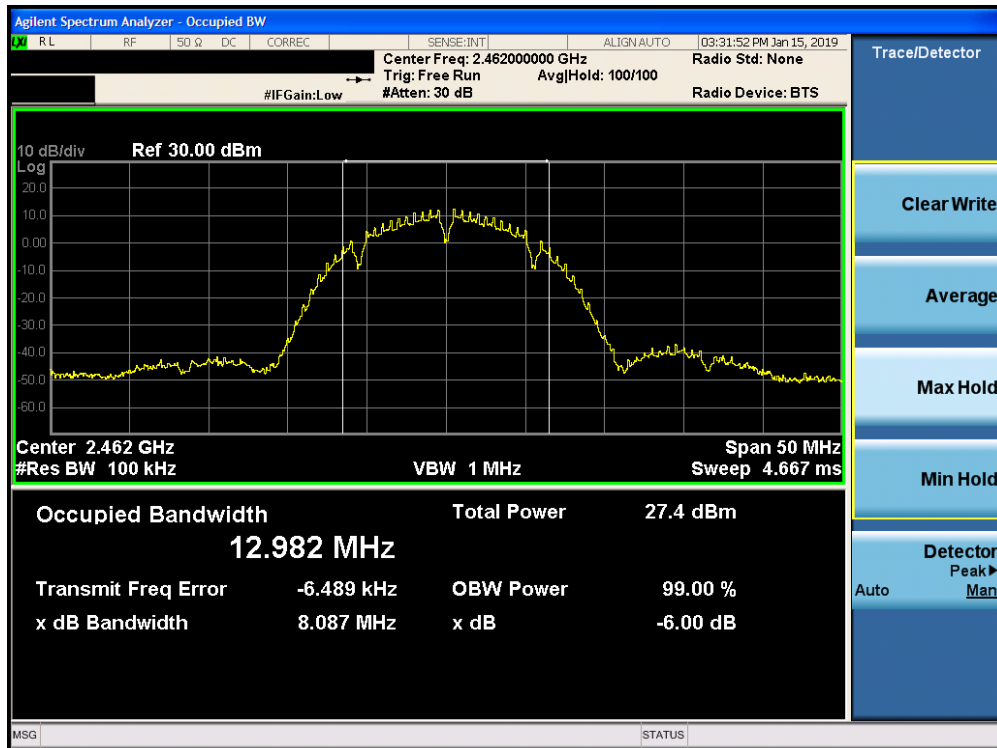
Plot 7-21. 6dB Bandwidth Plot SISO CORE 1 (802.11b – Ch. 11)
