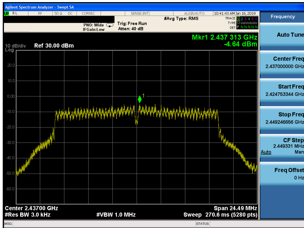
Plot 7-58. Power Spectral Density Plot CDD PRIMARY CORE 1 (802.11g – Ch. 6)
