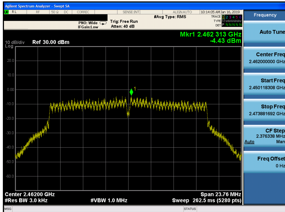
Plot 7-59. Power Spectral Density Plot CDD PRIMARY CORE 0 (802.11g – Ch. 11)
