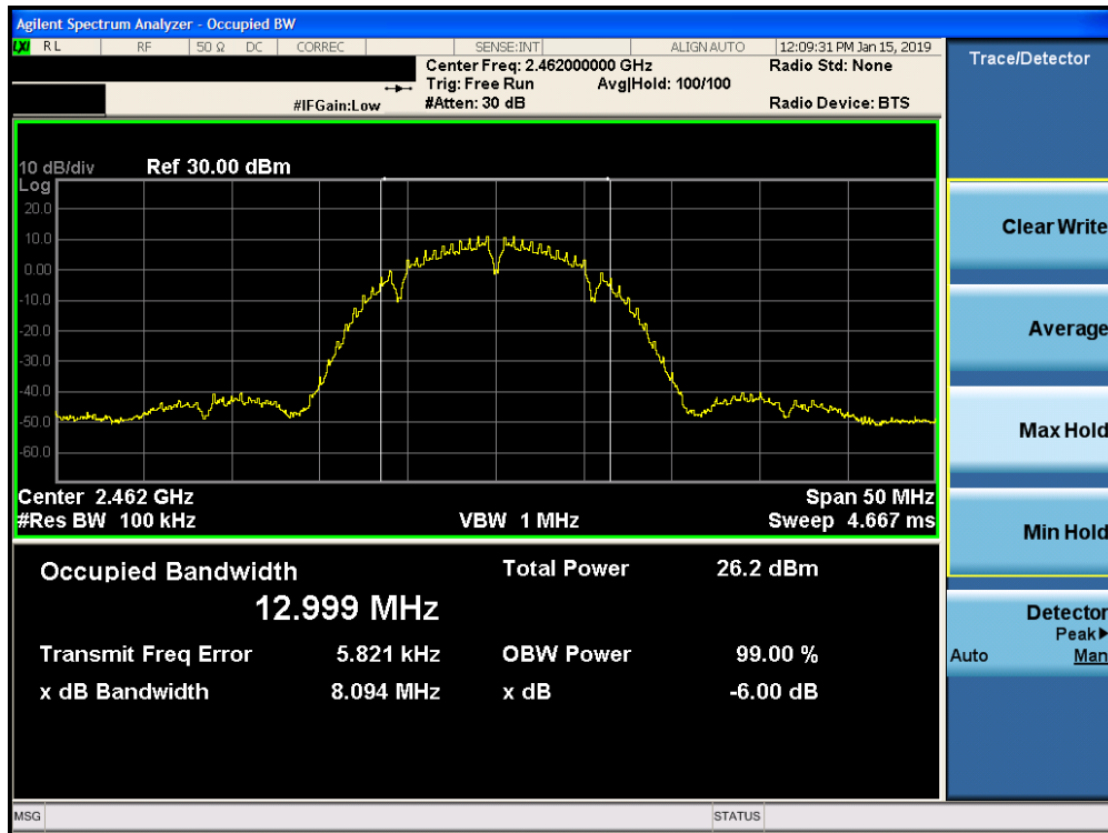
Plot 7-12. 6dB Bandwidth Plot SISO CORE 0 DIVERSITY (802.11b – Ch. 11)
