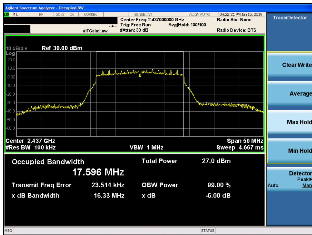
Plot 7-26. 6dB Bandwidth Plot SISO CORE 1 (802.11n) (2.4GHz) – Ch. 6)
