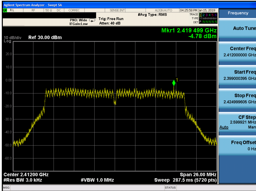
Plot 7-52. Power Spectral Density Plot SISO CORE 1 (802.11n (2.4GHz) – Ch. 1)
