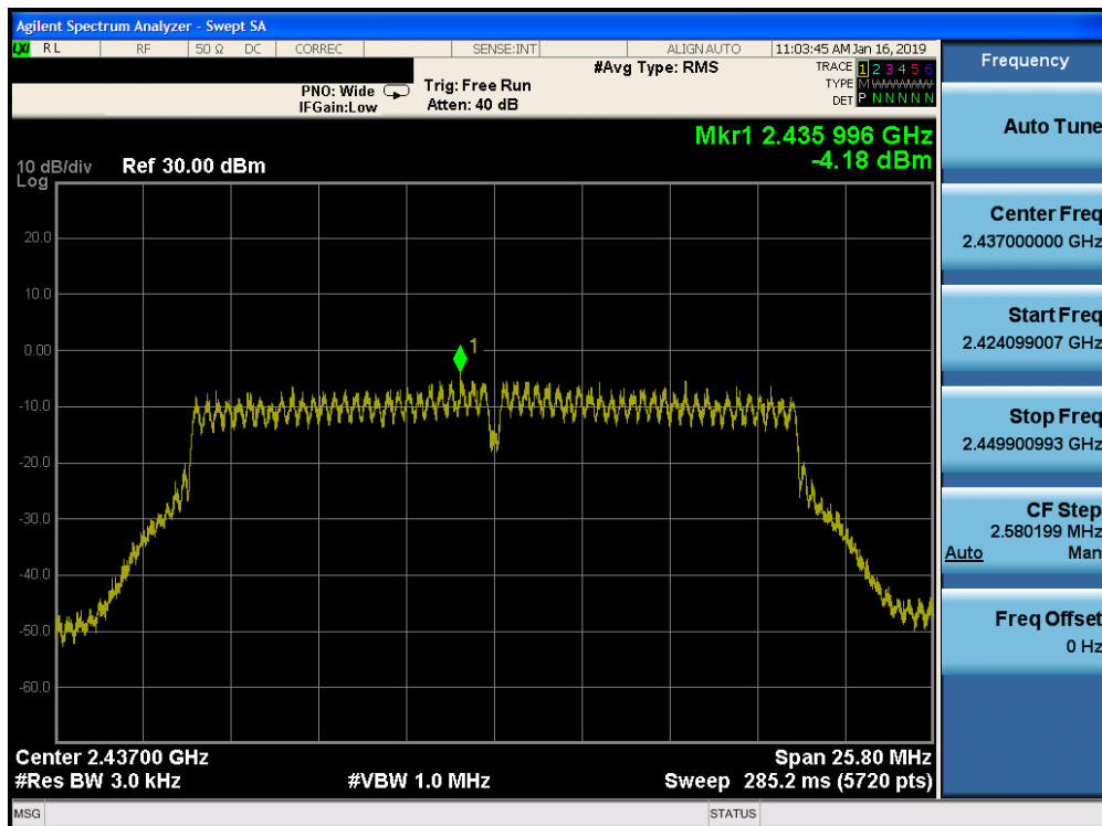
Plot 7-76. Power Spectral Density Plot CDD CORE 1 (802.11n (2.4GHz) – Ch. 6)
