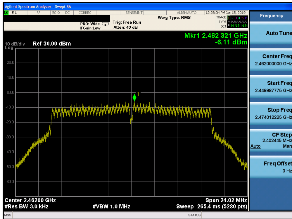
Plot 7-42. Power Spectral Density Plot SISO CORE 0 DIVERSITY (802.11g – Ch. 11)
