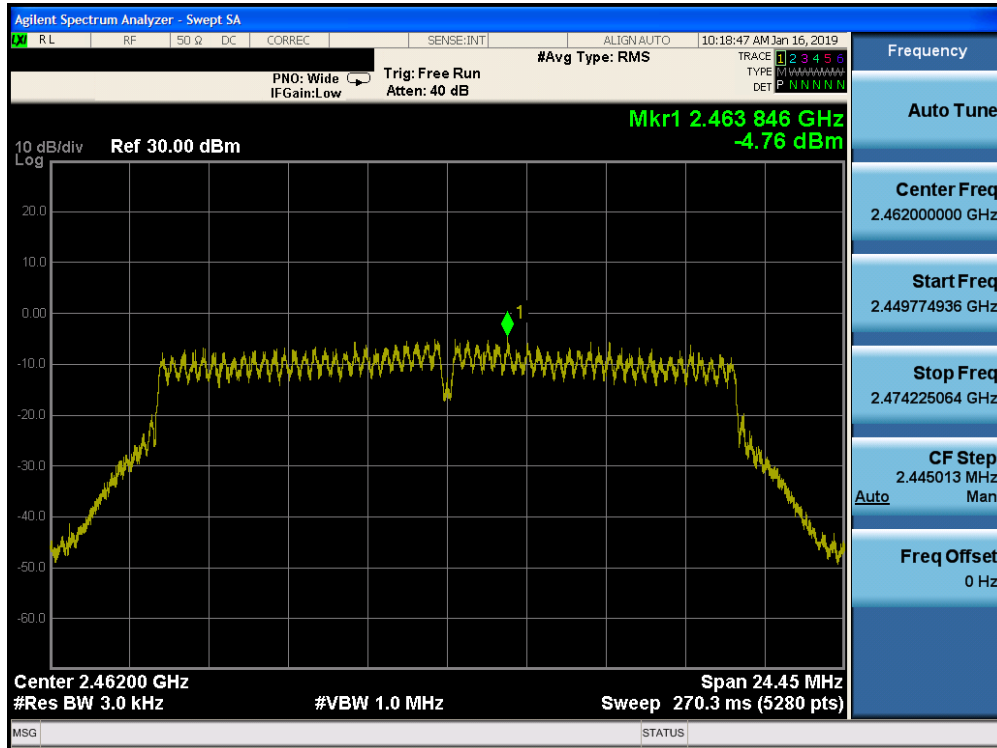
Plot 7-65. Power Spectral Density Plot CDD PRIMARY CORE 0 (802.11n (2.4GHz) – Ch. 11)
