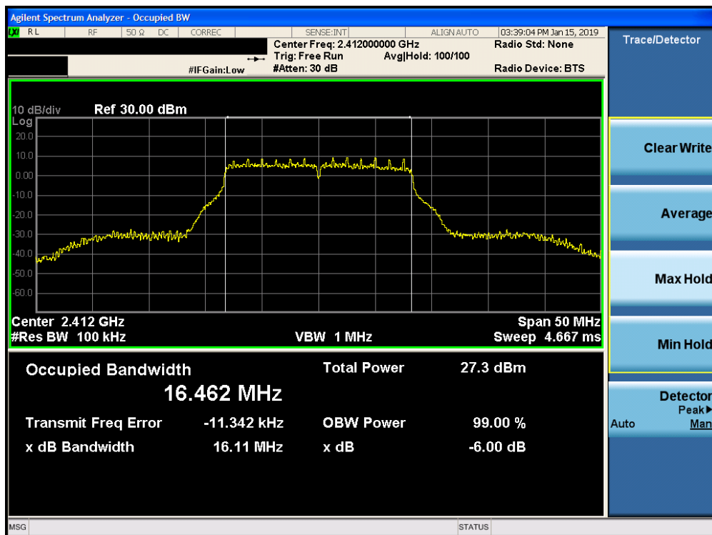
Plot 7-22. 6dB Bandwidth Plot SISO CORE 1 (802.11g – Ch. 1)
