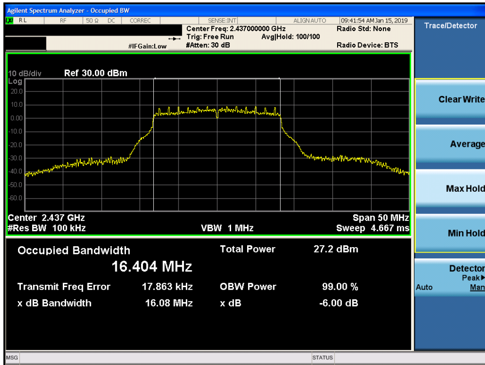
Plot 7-5. 6dB Bandwidth Plot SISO CORE 0 PRIMARY (802.11g – Ch. 6)
