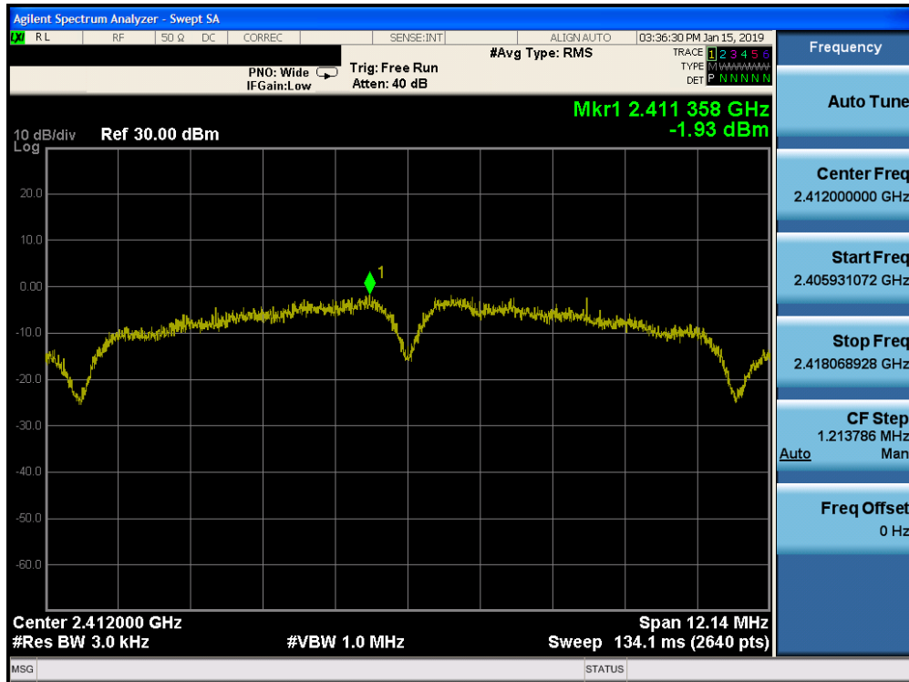
Plot 7-46. Power Spectral Density Plot SISO CORE 1 (802.11b – Ch. 1)
