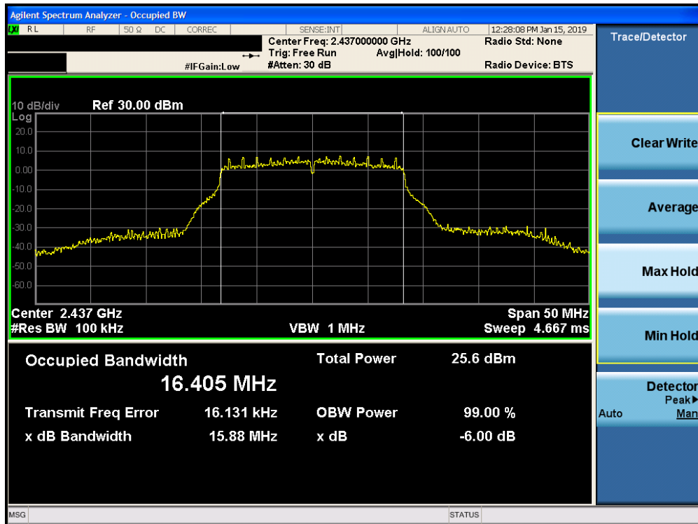
Plot 7-14. 6dB Bandwidth Plot SISO CORE 0 DIVERSITY (802.11g – Ch. 6)
