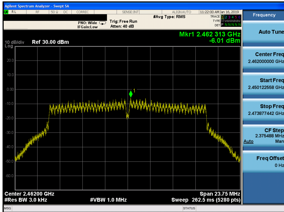
Plot 7-71. Power Spectral Density Plot CDD DIVERSITY CORE 0 (802.11g – Ch. 11)
