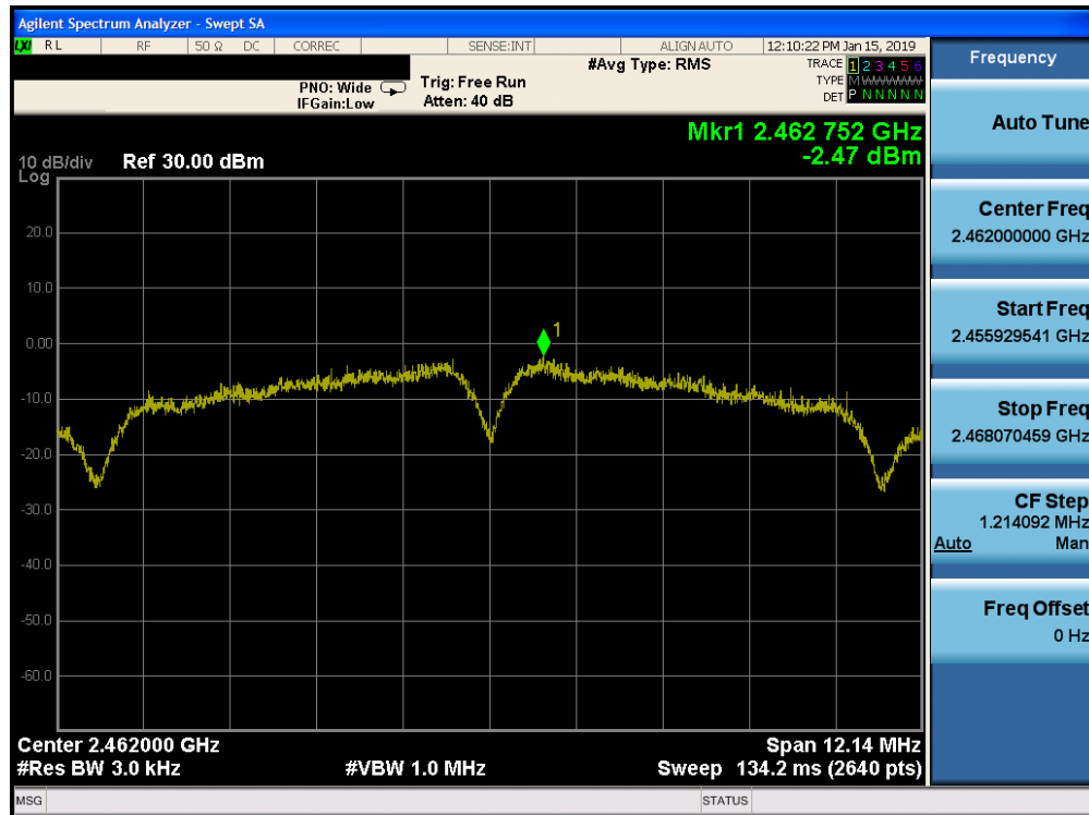
Plot 7-39. Power Spectral Density Plot SISO CORE 0 DIVERSITY (802.11b – Ch. 11)
