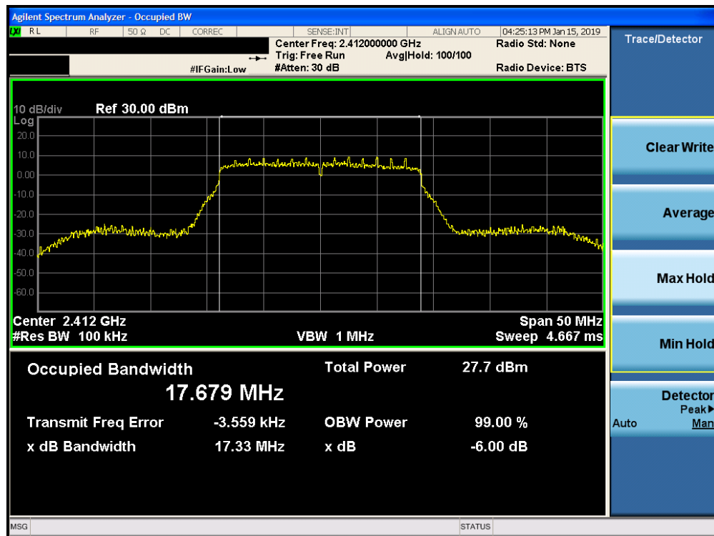
Plot 7-25. 6dB Bandwidth Plot SISO CORE 1 (802.11n) (2.4GHz) – Ch. 1)
