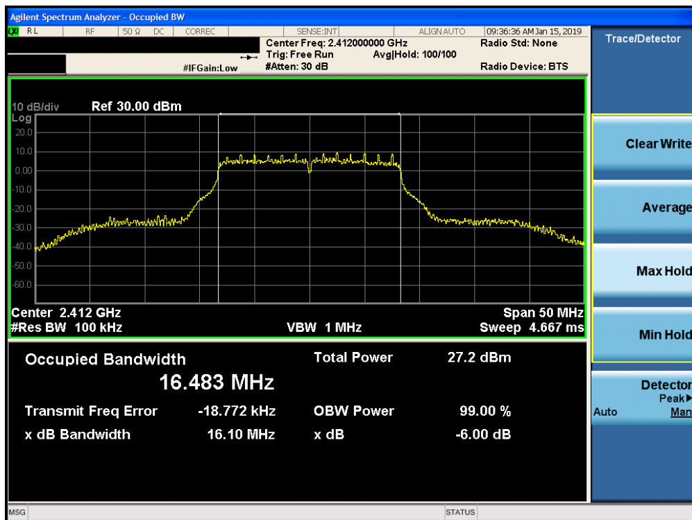
Plot 7-4. 6dB Bandwidth Plot SISO CORE 0 PRIMARY (802.11g – Ch. 1)
