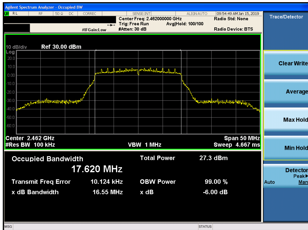
Plot 7-9. 6dB Bandwidth Plot SISO CORE 0 PRIMARY (802.11n (2.4GHz) – Ch. 11)
