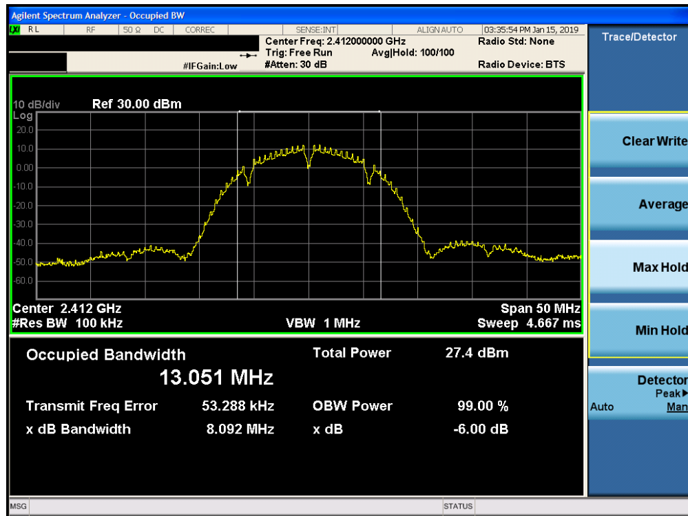
Plot 7-19. 6dB Bandwidth Plot SISO CORE 1 (802.11b – Ch. 1)
