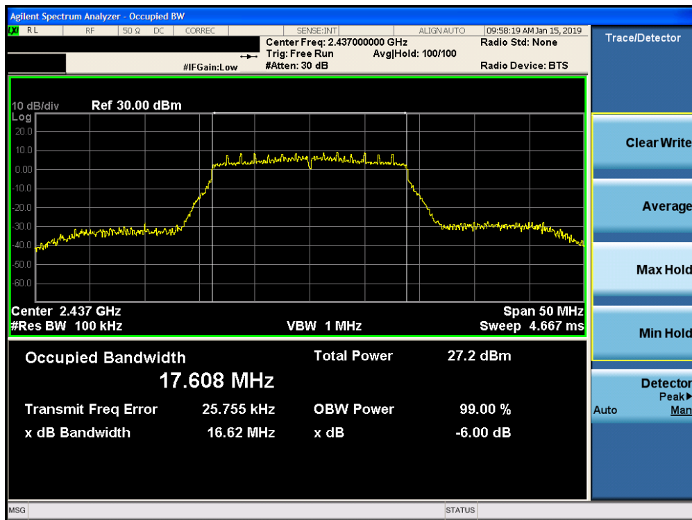
Plot 7-8. 6dB Bandwidth Plot SISO CORE 0 PRIMARY (802.11n (2.4GHz) – Ch. 6)
