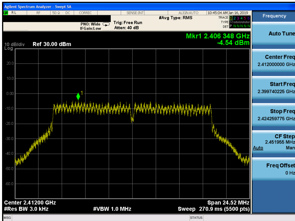
Plot 7-56. Power Spectral Density Plot CDD PRIMARY CORE 1 (802.11g - Ch. 1)
