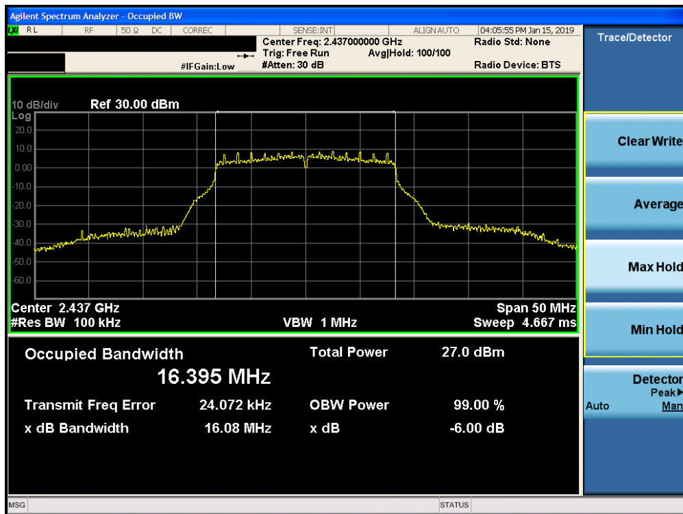
Plot 7-23. 6dB Bandwidth Plot SISO CORE 1 (802.11g - Ch. 6)
