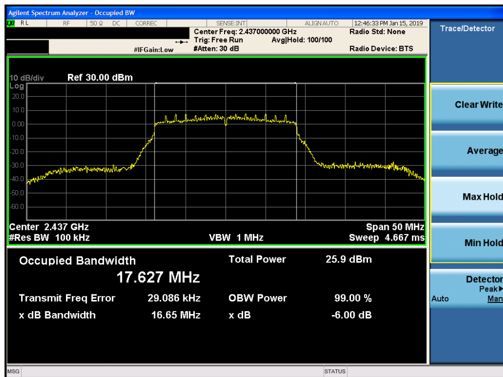
Plot 7-17. 6dB Bandwidth Plot SISO CORE 0 DIVERSITY (802.11n (2.4GHz) – Ch. 6)
