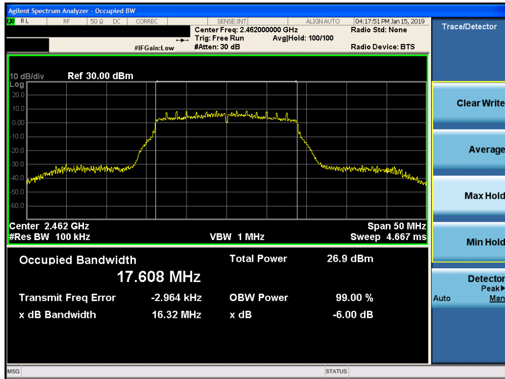
Plot 7-27. 6dB Bandwidth Plot SISO CORE 1 (802.11n (2.4GHz) – Ch. 11)
