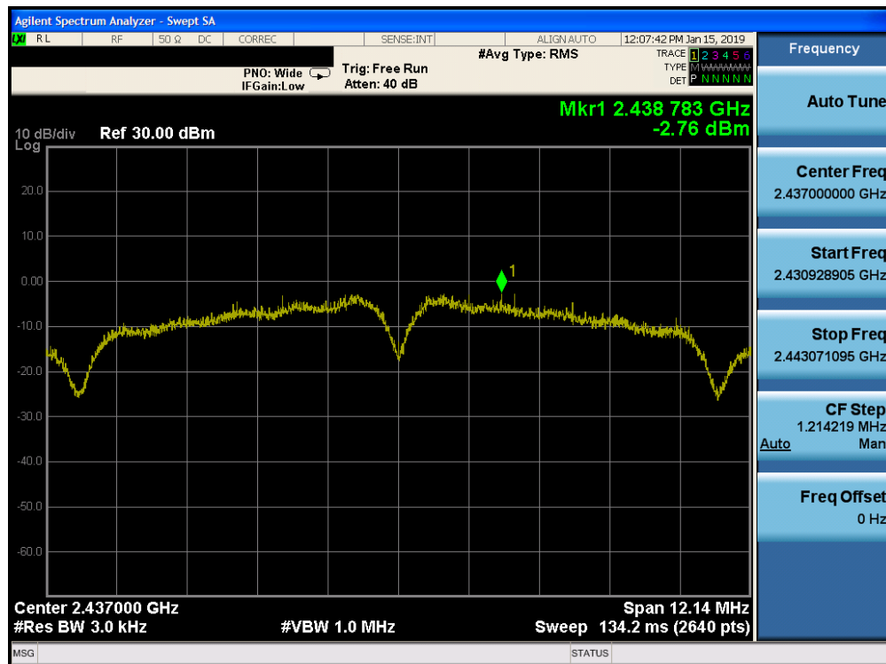
Plot 7-38. Power Spectral Density Plot SISO CORE 0 DIVERSITY (802.11b – Ch. 6)
