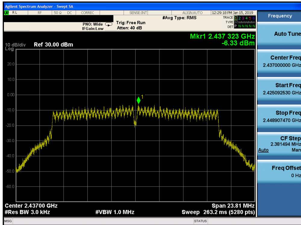
Plot 7-41. Power Spectral Density Plot SISO CORE 0 DIVERSITY (802.11g – Ch. 6)
