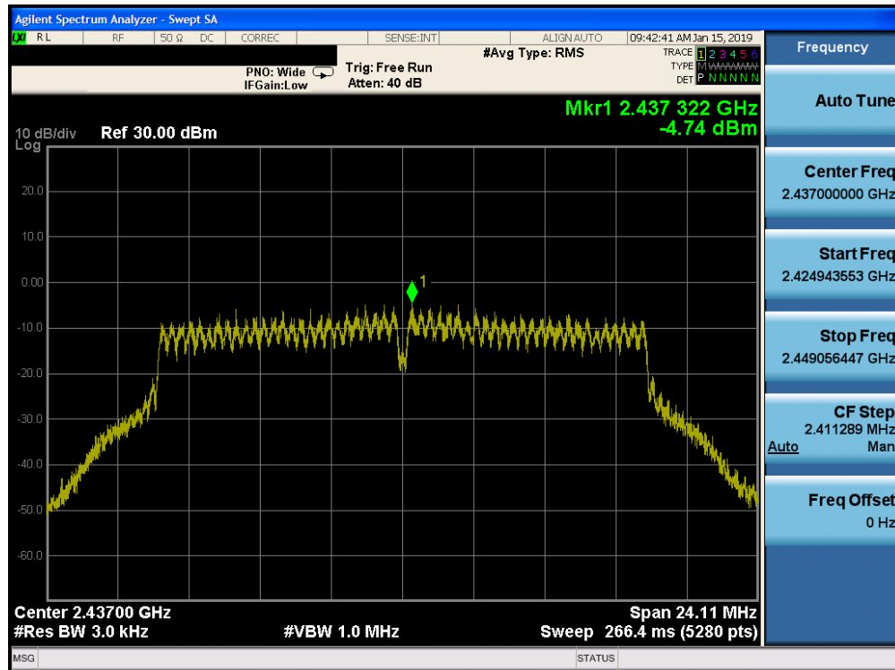
Plot 7-32. Power Spectral Density Plot SISO CORE 0 PRIMARY (802.11g – Ch. 6)
