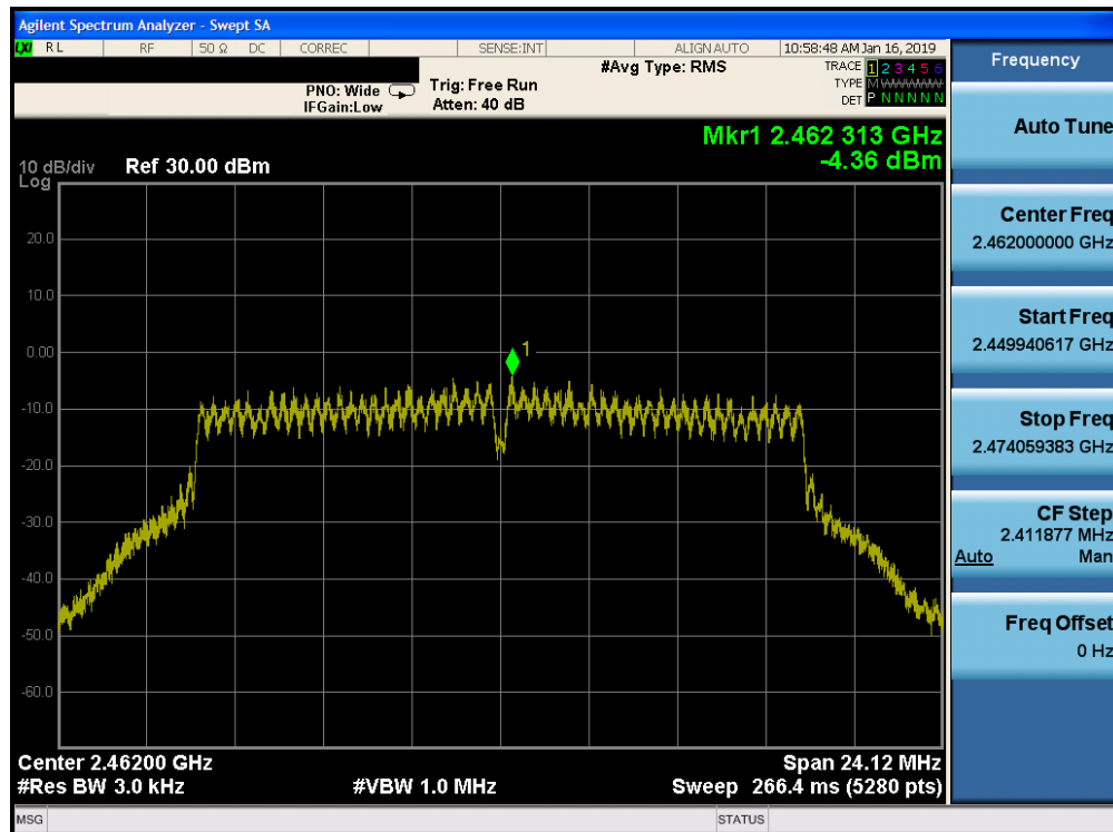
Plot 7-72. Power Spectral Density Plot CDD CORE 1 (802.11g – Ch. 11)
