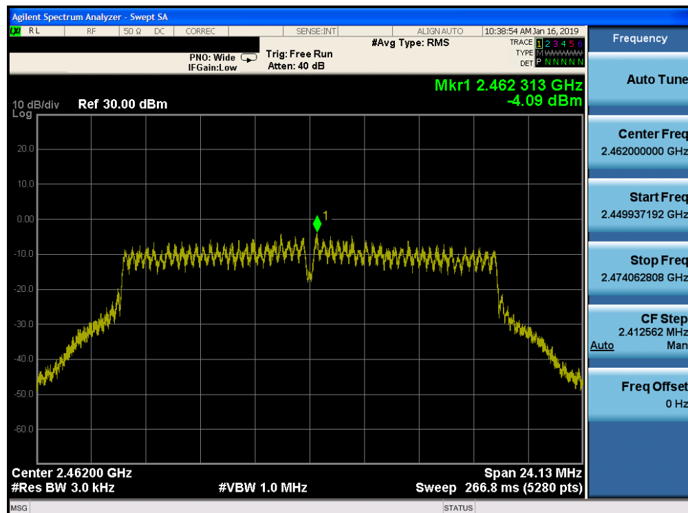
Plot 7-60. Power Spectral Density Plot CDD PRIMARY CORE 1 (802.11g – Ch. 11)
