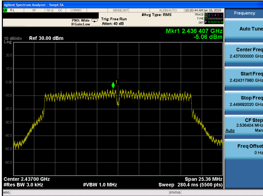
Plot 7-63. Power Spectral Density Plot CDD PRIMARY CORE 0 (802.11n (2.4GHz) – Ch. 6)
