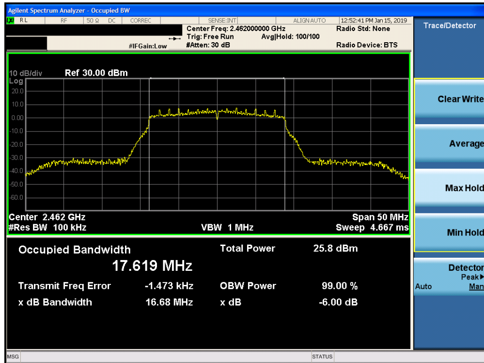
Plot 7-18. 6dB Bandwidth Plot SISO CORE 0 DIVERSITY (802.11n (2.4GHz) – Ch. 11)
