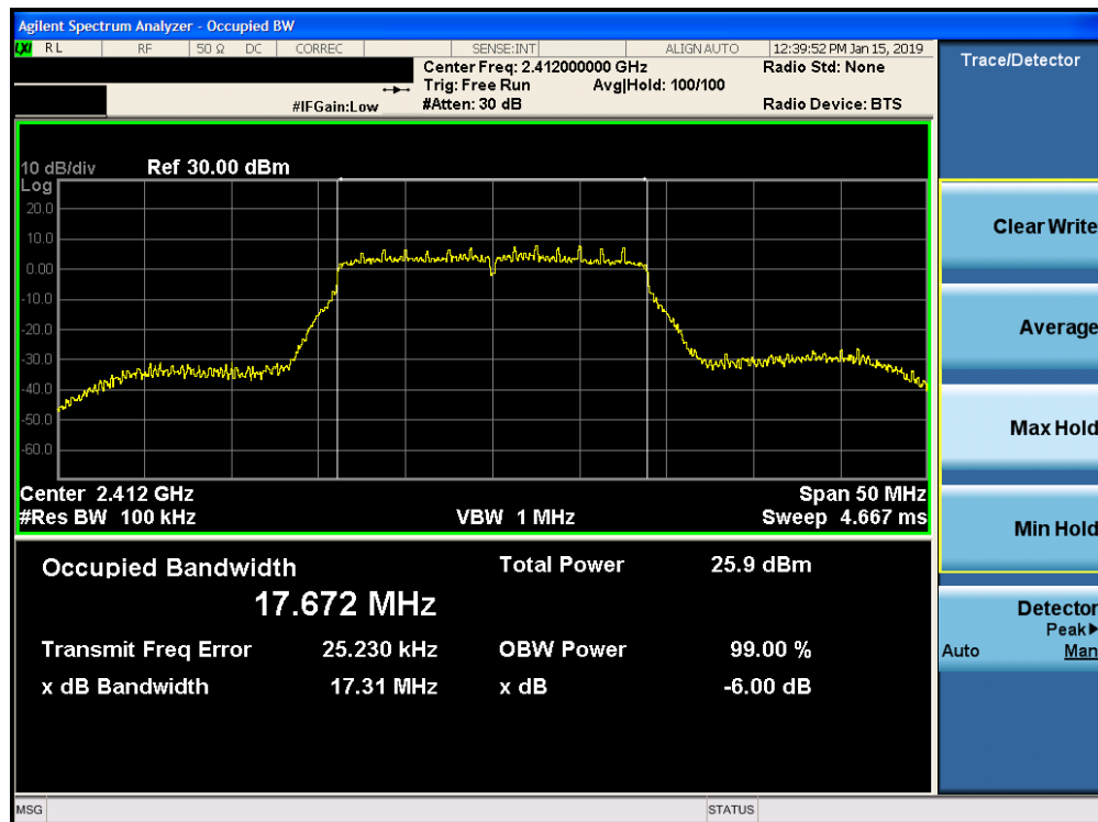
Plot 7-16. 6dB Bandwidth Plot SISO CORE 0 DIVERSITY (802.11n (2.4GHz) – Ch. 1)
