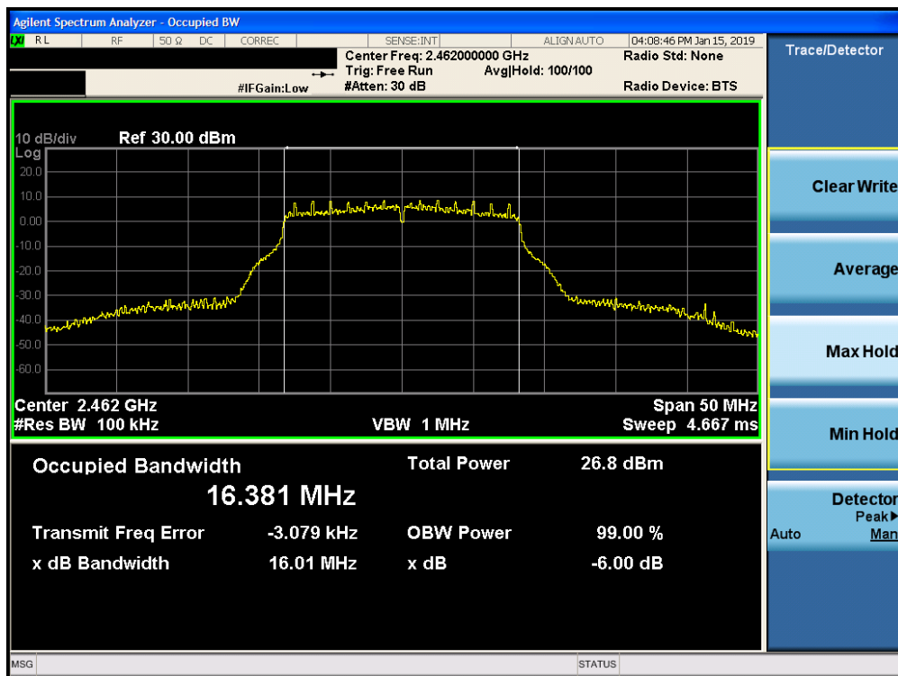
Plot 7-24. 6dB Bandwidth Plot SISO CORE 1 (802.11g - Ch. 11)
