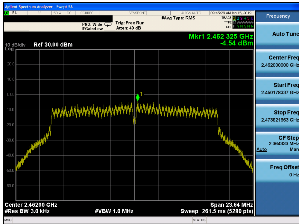
Plot 7-33. Power Spectral Density Plot SISO CORE 0 PRIMARY (802.11g – Ch. 11)
