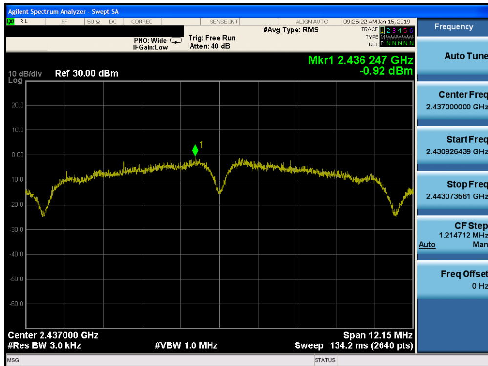
Plot 7-29. Power Spectral Density Plot SISO CORE 0 PRIMARY (802.11b – Ch. 6)
