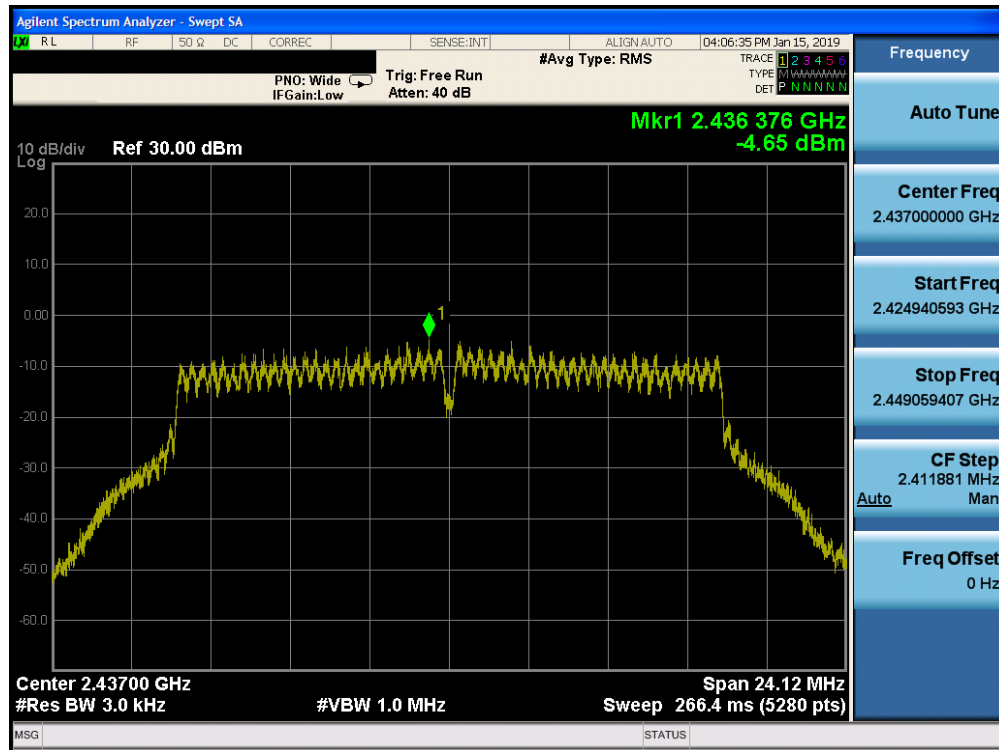
Plot 7-50. Power Spectral Density Plot SISO CORE 1 (802.11g – Ch. 6)
