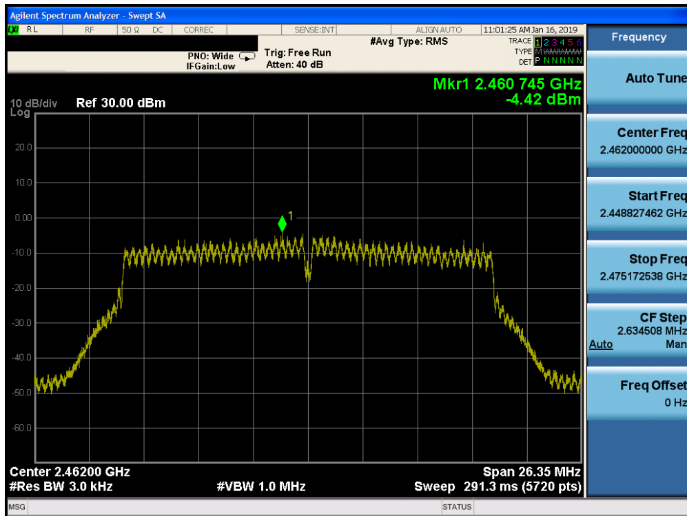
Plot 7-78. Power Spectral Density Plot CDD CORE 1 (802.11n (2.4GHz) – Ch. 11)
