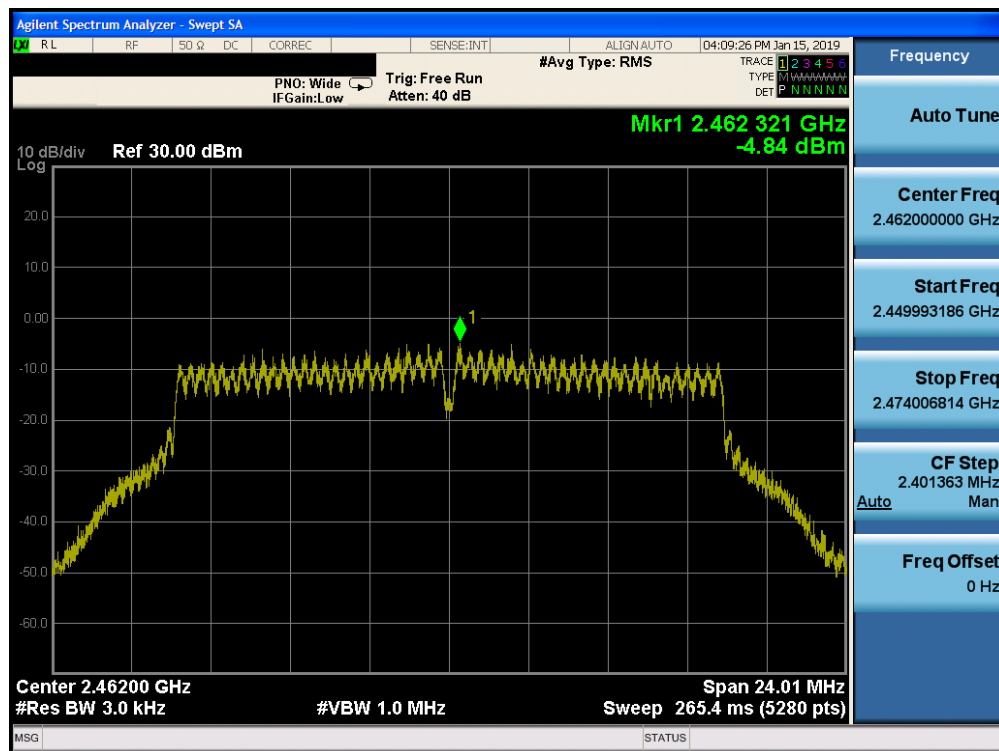
Plot 7-51. Power Spectral Density Plot SISO CORE 1 (802.11g – Ch. 11)
