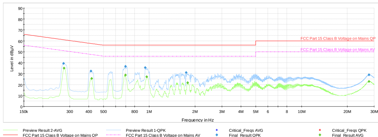
Plot 7-75. Line Conducted Plot with Bluetooth HDR4 – Ch.39 (N, with AC/DC Adapter)
