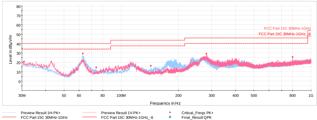
Plot 7-73. Radiated Spurious Plot below 1GHz (4Mbps, ePA – Ch.39 with Laptop)
