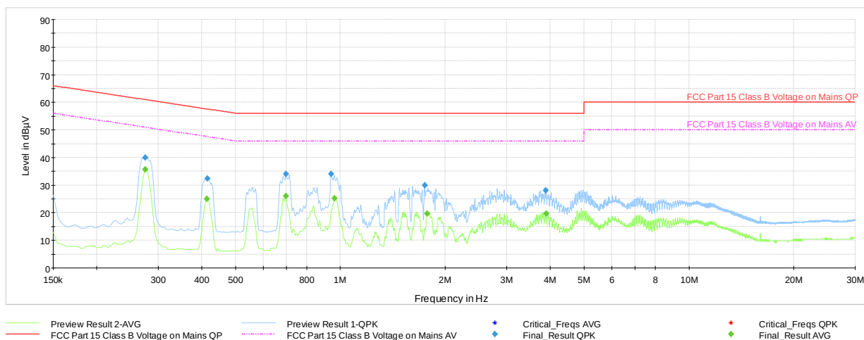
Plot 7-74. Line Conducted Plot with Bluetooth HDR4 – Ch.39 (L1, with AC/DC Adapter)
