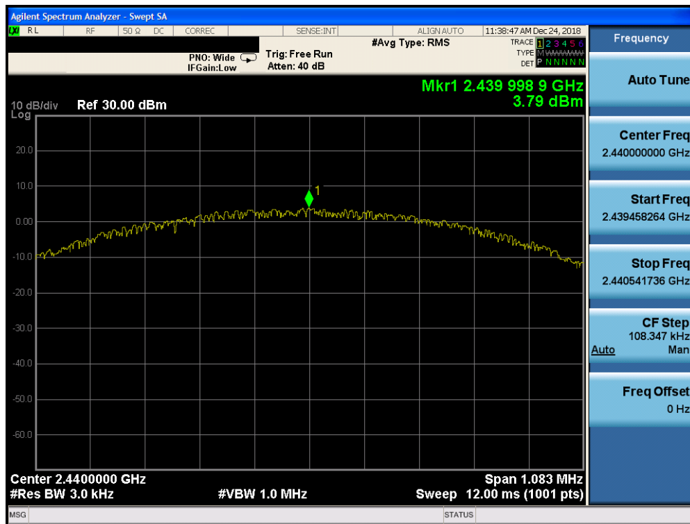
Plot 7-26. Power Spectral Density Plot ANT 1 (Bluetooth (LE), 1Mbps ePA – Ch. 19)
