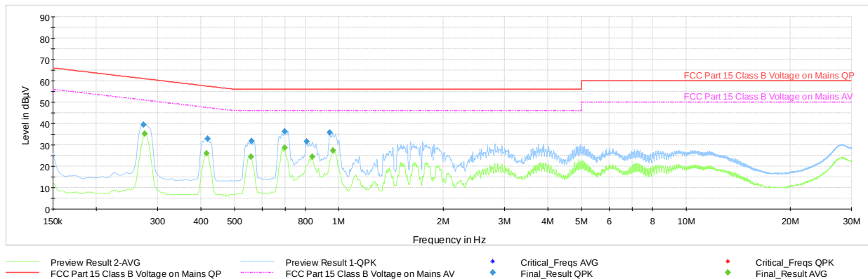
Plot 7-75. Line Conducted Plot with Bluetooth LE (N, with AC/DC Adapter)
