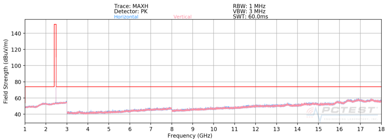
Plot 7-62. Radiated Spurious Plot Above 1GHz ANT 1 (1Mbps, ePA – Ch. 39)
