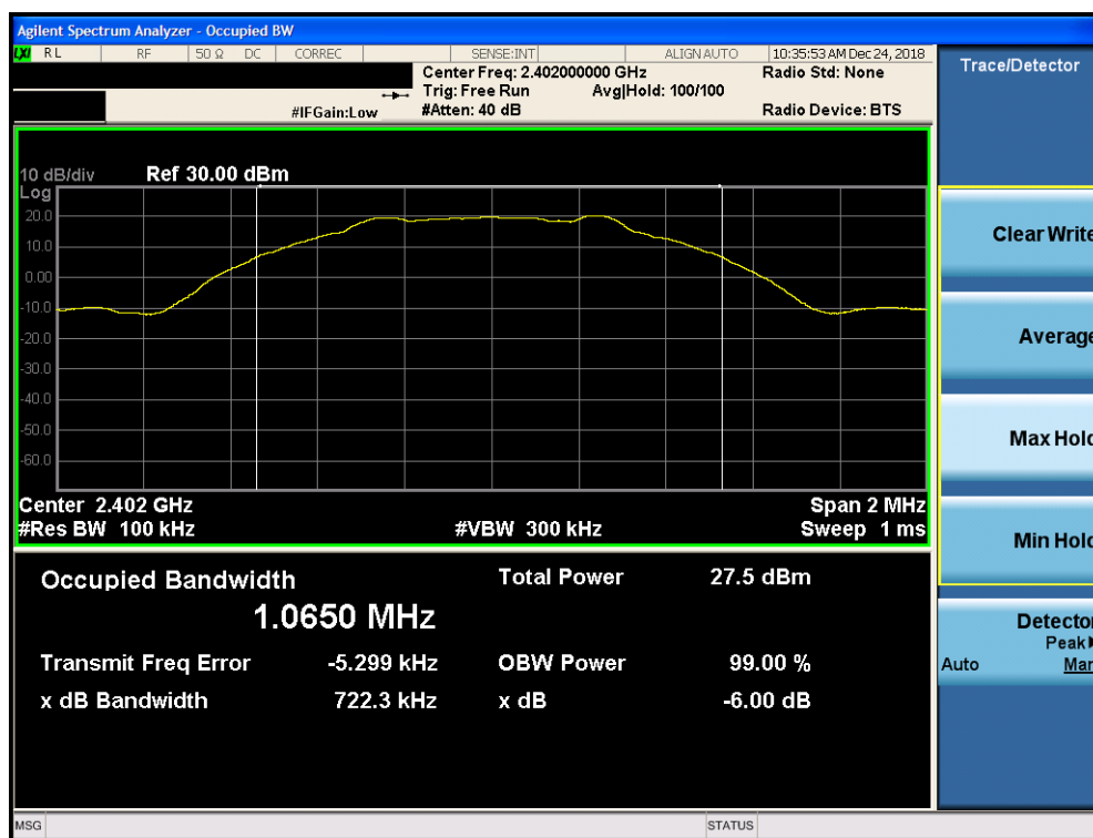
Plot 7-1. 6dB Bandwidth Plot ANT 0 (Bluetooth (LE), 1Mbps ePA – Ch. 0)
