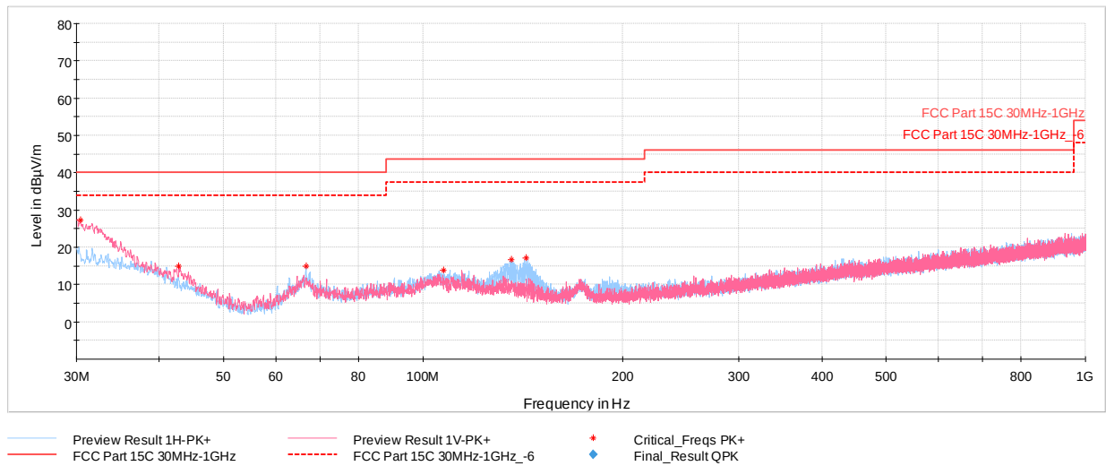
Plot 7-73. Radiated Spurious Plot below 1GHz (1Mbps, ePA, Ch.19 with AC/DC Adapter)
