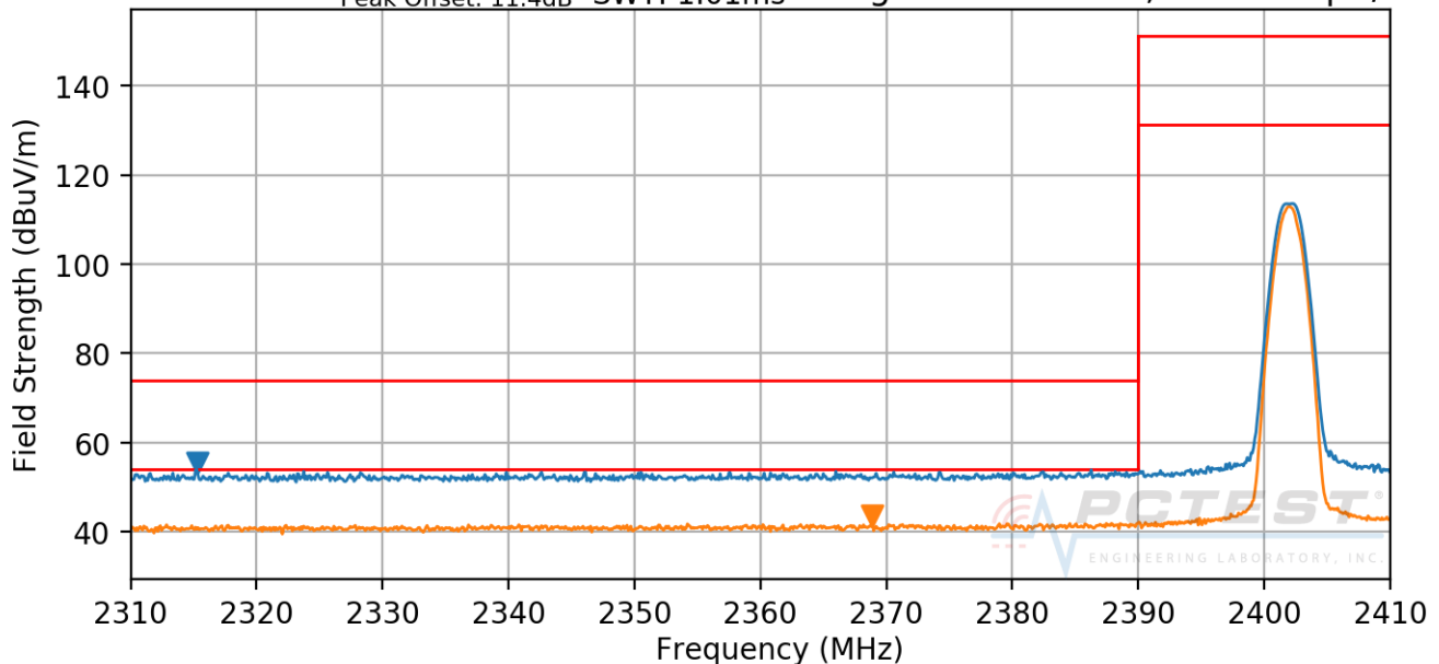
Plot 7-69. Radiated Restricted Lower Band Edge Measurement ANT 1 (Average & Peak)
