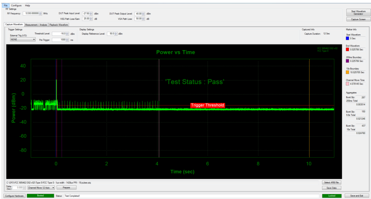
Figure 9-30. 5530MHz - Channel Move/ Closing Transmission Time - Mode 2 (80 MHz)
