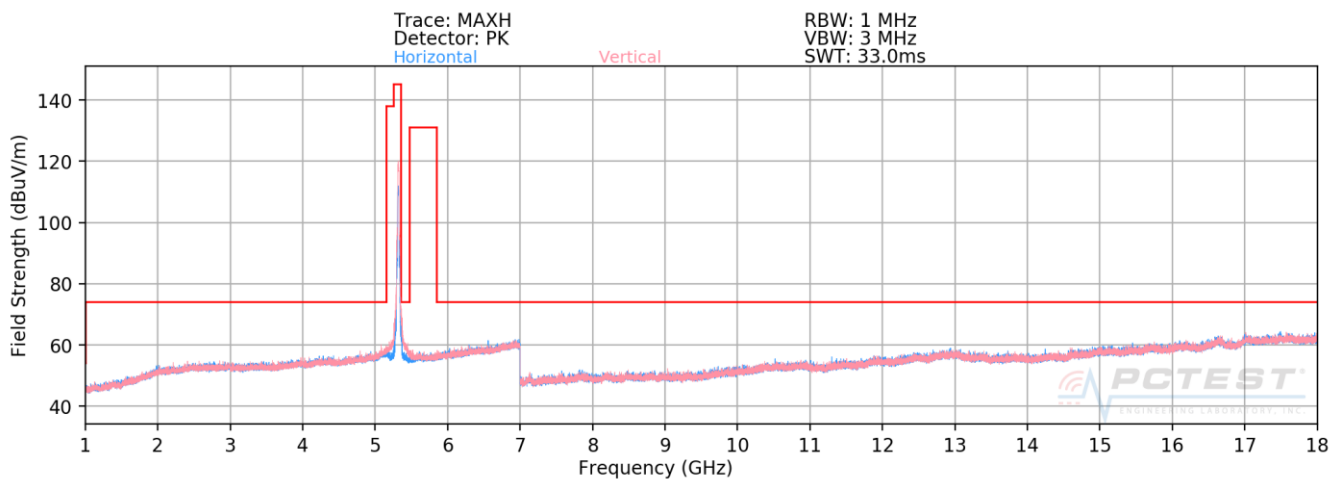
Plot 7-162. Radiated Spurious Plot above 1GHz SISO CORE0 (802.11n – U2A Ch. 64)
