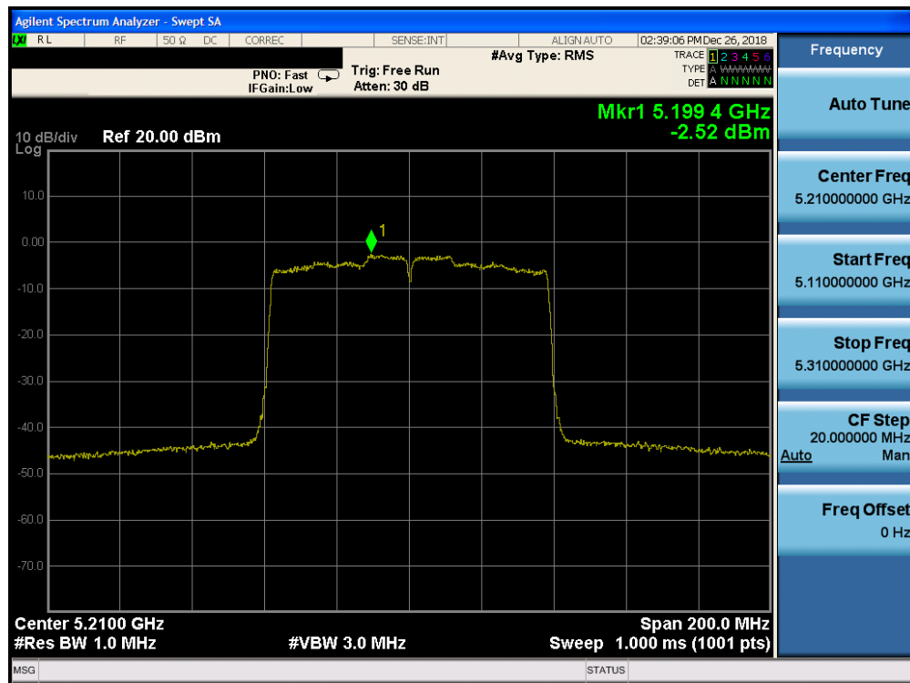
Plot 7-116. Power Spectral Density Plot MIMO/CDD CORE 1 (80MHz BW 802.11ac (UNII Band 1) – Ch. 42)
