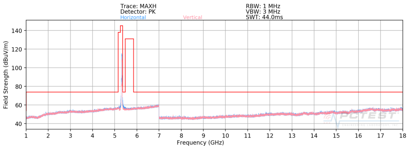
Plot 7-174. Radiated Spurious Plot above 1GHz SISO CORE 1 (802.11n – U2A Ch. 64)
