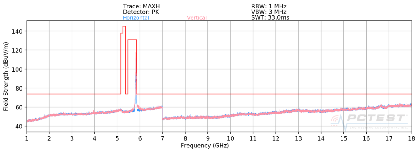
Plot 7-168. Radiated Spurious Plot above 1GHz SISO CORE0 (802.11n – U3 Ch. 165)
