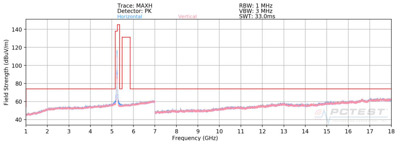
Plot 7-171. Radiated Spurious Plot above 1GHz SISO CORE 1 (802.11n – U1 Ch. 48)
