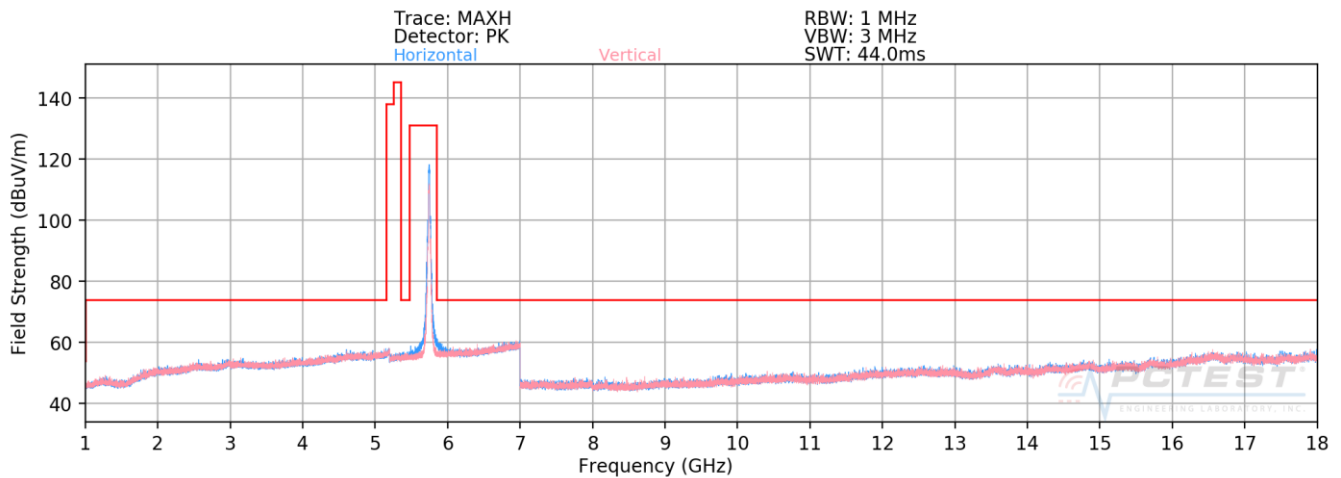
Plot 7-178. Radiated Spurious Plot above 1GHz SISO CORE 1 (802.11n – U3 Ch. 149)
