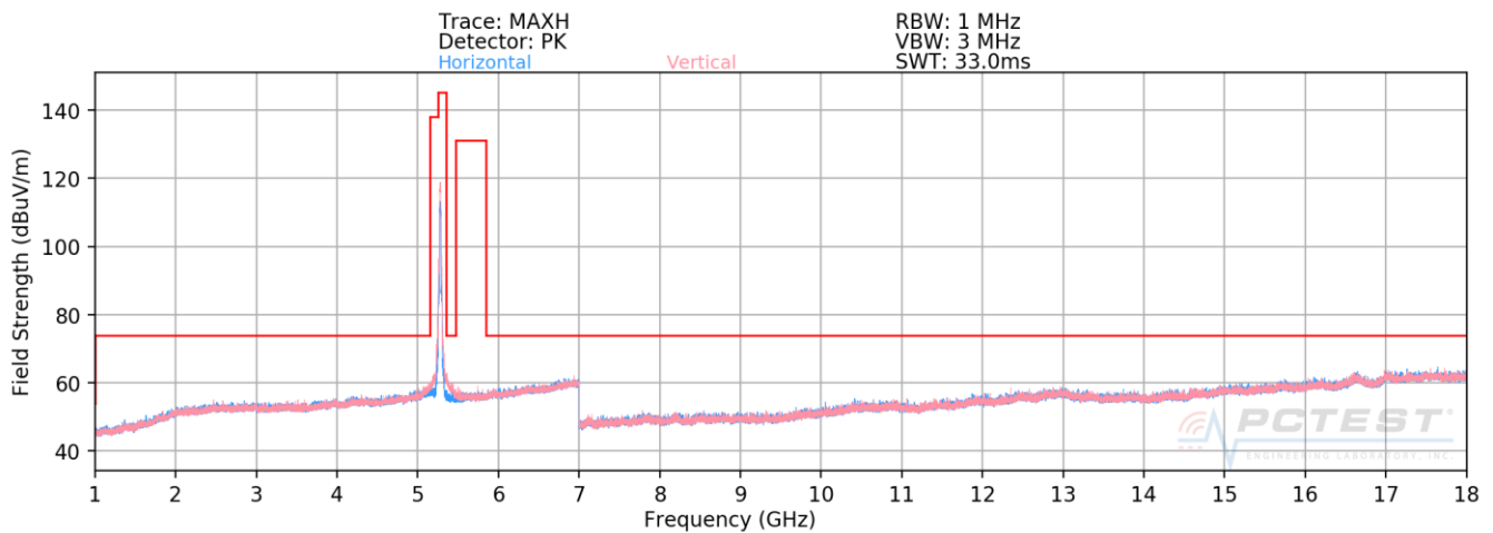
Plot 7-161. Radiated Spurious Plot above 1GHz SISO CORE0 (802.11n – U2A Ch. 56)
