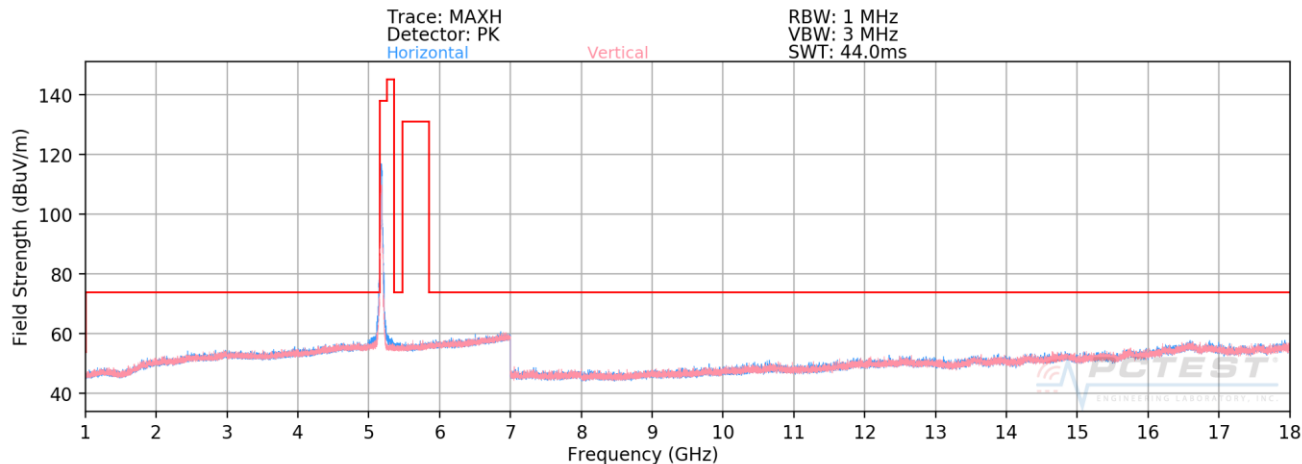
Plot 7-169. Radiated Spurious Plot above 1GHz SISO CORE 1 (802.11n – U1 Ch. 36)
