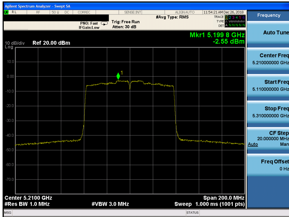
Plot 7-115. Power Spectral Density Plot MIMO/CDD CORE 0 (80MHz BW 802.11ac (UNII Band 1) – Ch. 42)
