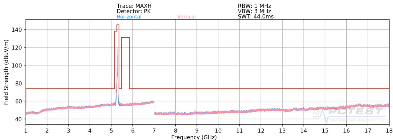
Plot 7-185. Radiated Spurious Plot above 1GHz MIMO/CDD (802.11n – U2A Ch. 56)
