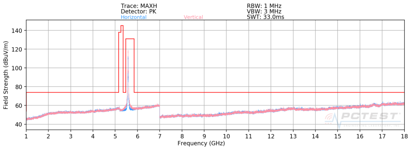
Plot 7-164. Radiated Spurious Plot above 1GHz SISO CORE0 (802.11n – U2C Ch. 116)
