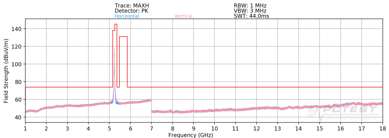
Plot 7-183. Radiated Spurious Plot above 1GHz MIMO/CDD (802.11n – U1 Ch. 48)
