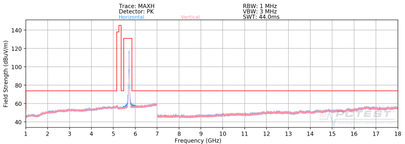
Plot 7-177. Radiated Spurious Plot above 1GHz SISO CORE 1 (802.11n – U2C Ch. 144)
