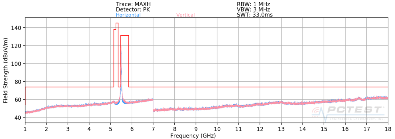
Plot 7-187. Radiated Spurious Plot above 1GHz MIMO/CDD (802.11n – U2C Ch. 100)
