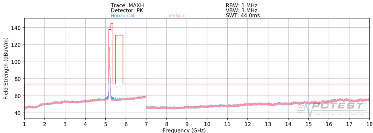
Plot 7-170. Radiated Spurious Plot above 1GHz SISO CORE 1 (802.11n – U1 Ch. 40)
