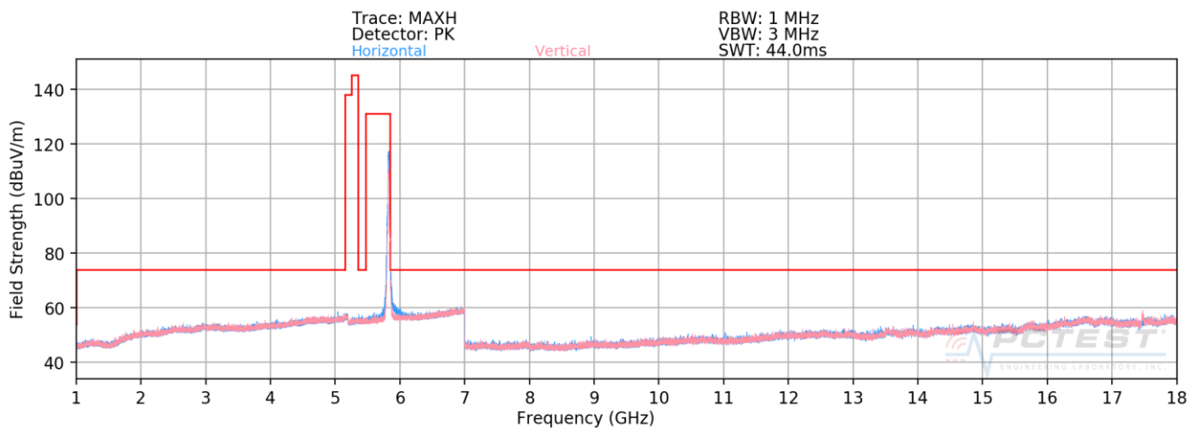
Plot 7-180. Radiated Spurious Plot above 1GHz SISO CORE 1 (802.11n – U3 Ch. 165)
