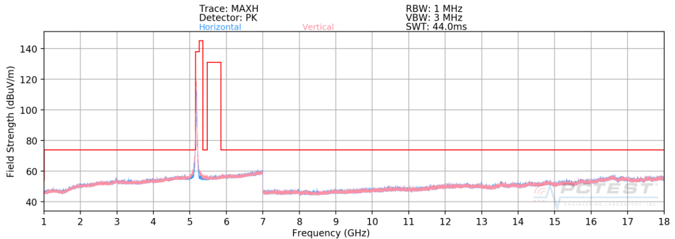
Plot 7-181. Radiated Spurious Plot above 1GHz MIMO/CDD (802.11n – U1 Ch. 36)
