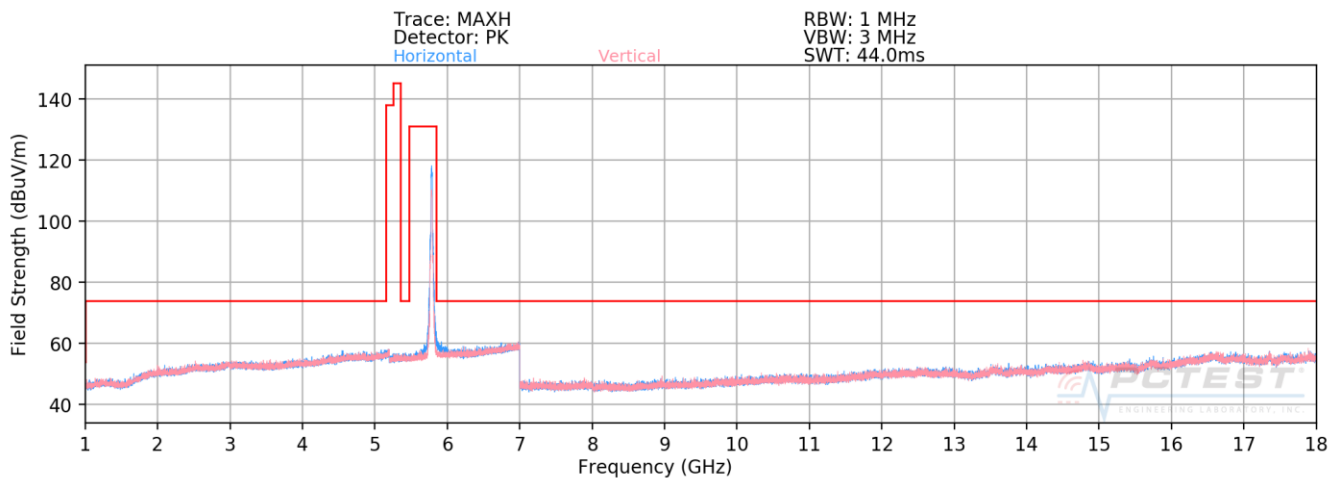
Plot 7-179. Radiated Spurious Plot above 1GHz SISO CORE 1 (802.11n – U3 Ch. 157)
