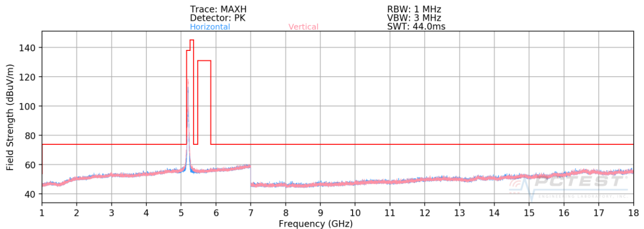
Plot 7-182. Radiated Spurious Plot above 1GHz MIMO/CDD (802.11n – U1 Ch. 40)
