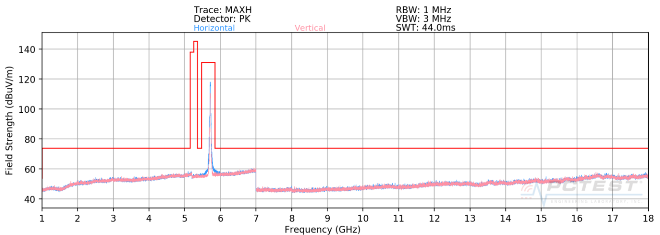
Plot 7-165. Radiated Spurious Plot above 1GHz SISO CORE0 (802.11n – U2C Ch. 144)
