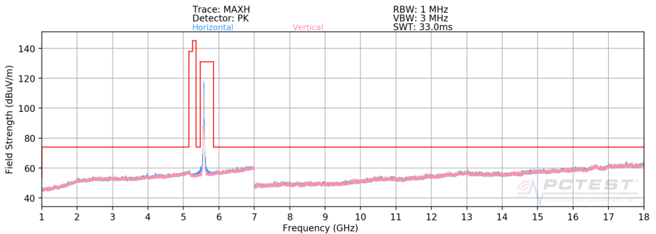
Plot 7-176. Radiated Spurious Plot above 1GHz SISO CORE 1 (802.11n – U2C Ch. 116)
