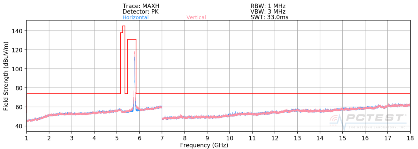
Plot 7-167. Radiated Spurious Plot above 1GHz SISO CORE0 (802.11n – U3 Ch. 157)
