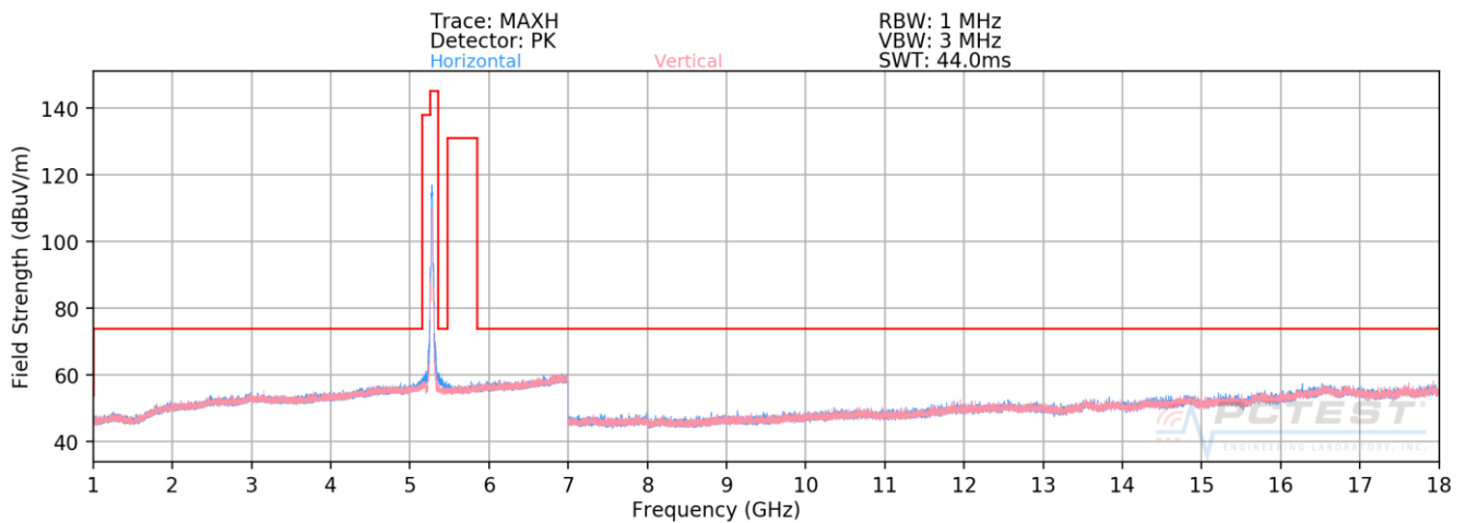
Plot 7-173. Radiated Spurious Plot above 1GHz SISO CORE 1 (802.11n – U2A Ch. 56)
