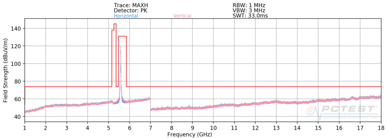
Plot 7-188. Radiated Spurious Plot above 1GHz MIMO/CDD (802.11n – U2C Ch. 116)
