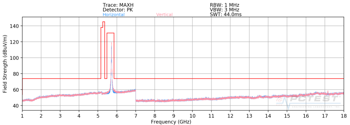
Plot 7-189. Radiated Spurious Plot above 1GHz MIMO/CDD (802.11n – U2C Ch. 144)
