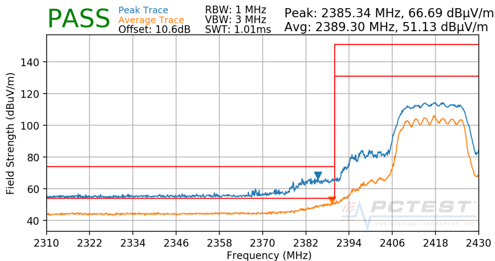
Plot 7-113. Radiated Restricted Lower Band Edge Measurement CDD
