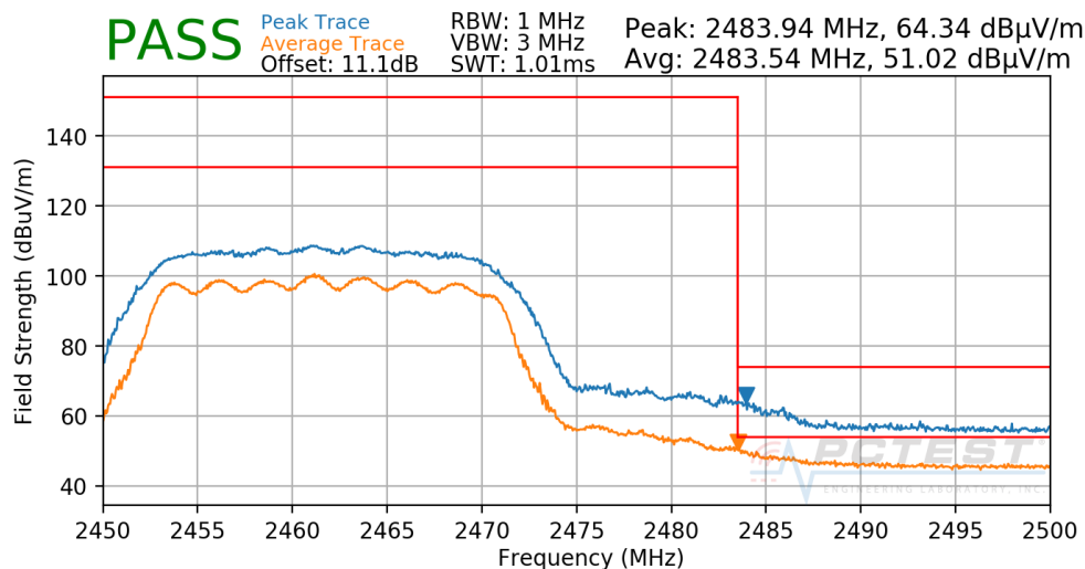
Plot 7-115. Radiated Restricted Upper Band Edge Measurement CDD
