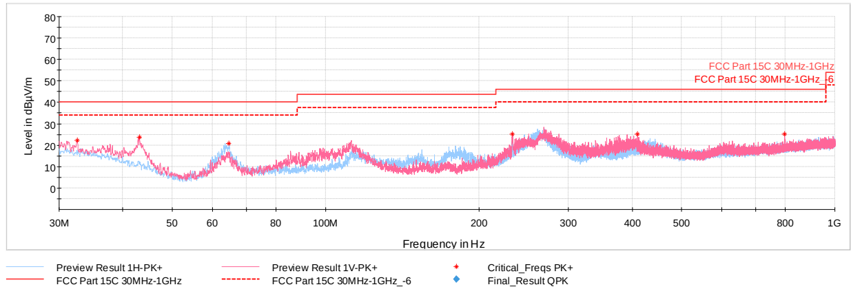
Plot 7-118. Radiated Spurious Plot below 1GHz CDD Ch.6, with Laptop
