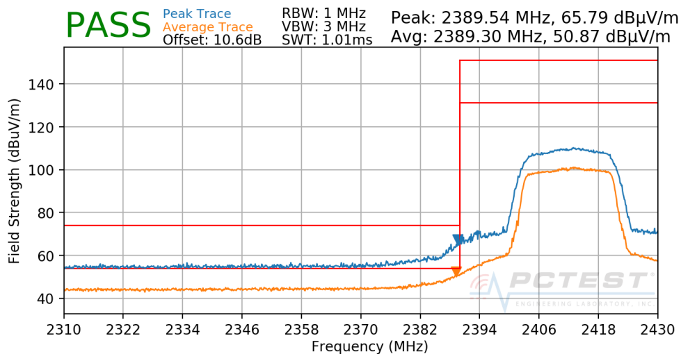
Plot 7-107. Radiated Restricted Lower Band Edge Measurement SISO CORE 1
