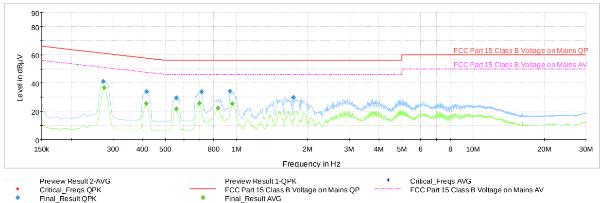
Plot 7-119. Line Conducted Plot with 802.11n CDD Ch.6 (L1, with AC/DC Adapter)
