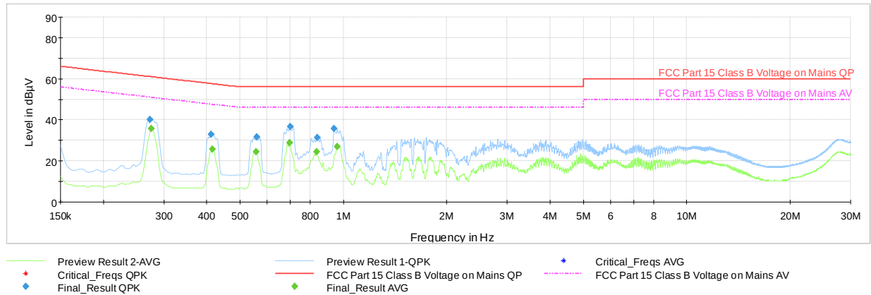
Plot 7-120. Line Conducted Plot with 802.11n CDD Ch.6 (N, WITH AC/DC Adapter)
