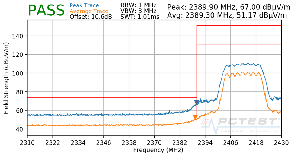
Plot 7-112. Radiated Restricted Lower Band Edge Measurement CDD
