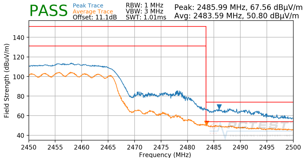
Plot 7-114. Radiated Restricted Upper Band Edge Measurement CDD
