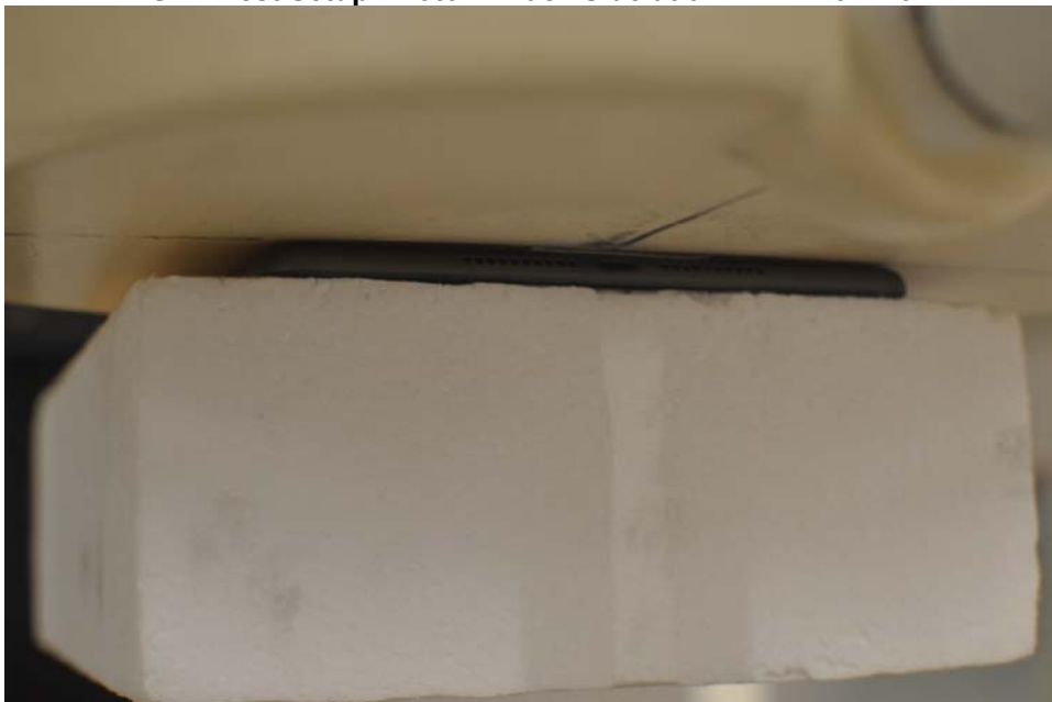
SAR Test Setup Photo 2: Back Side at 0 mm – Ant WF1
