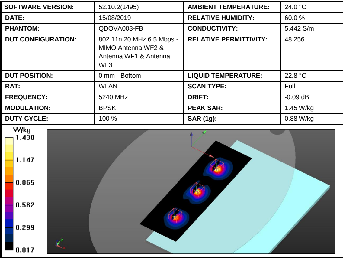
Figure 32: SAR Body Testing Results for the A2141 at 5240 MHz.
