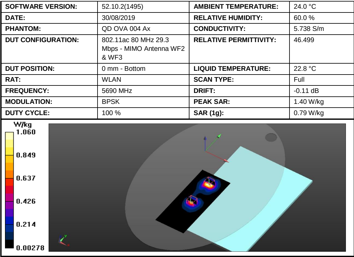
Figure 45: SAR Body Testing Results for the A2141 at 5690 MHz.
