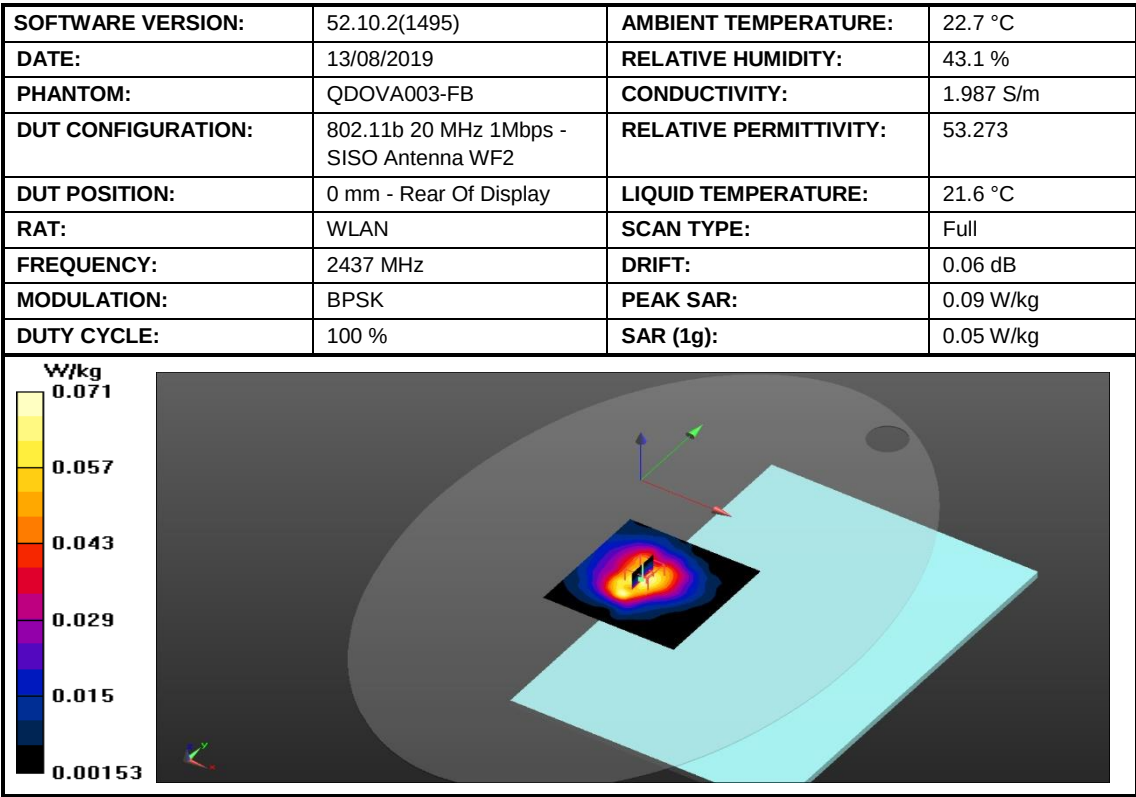
Figure 6: SAR Body Testing Results for the A2141 at 2437 MHz.
