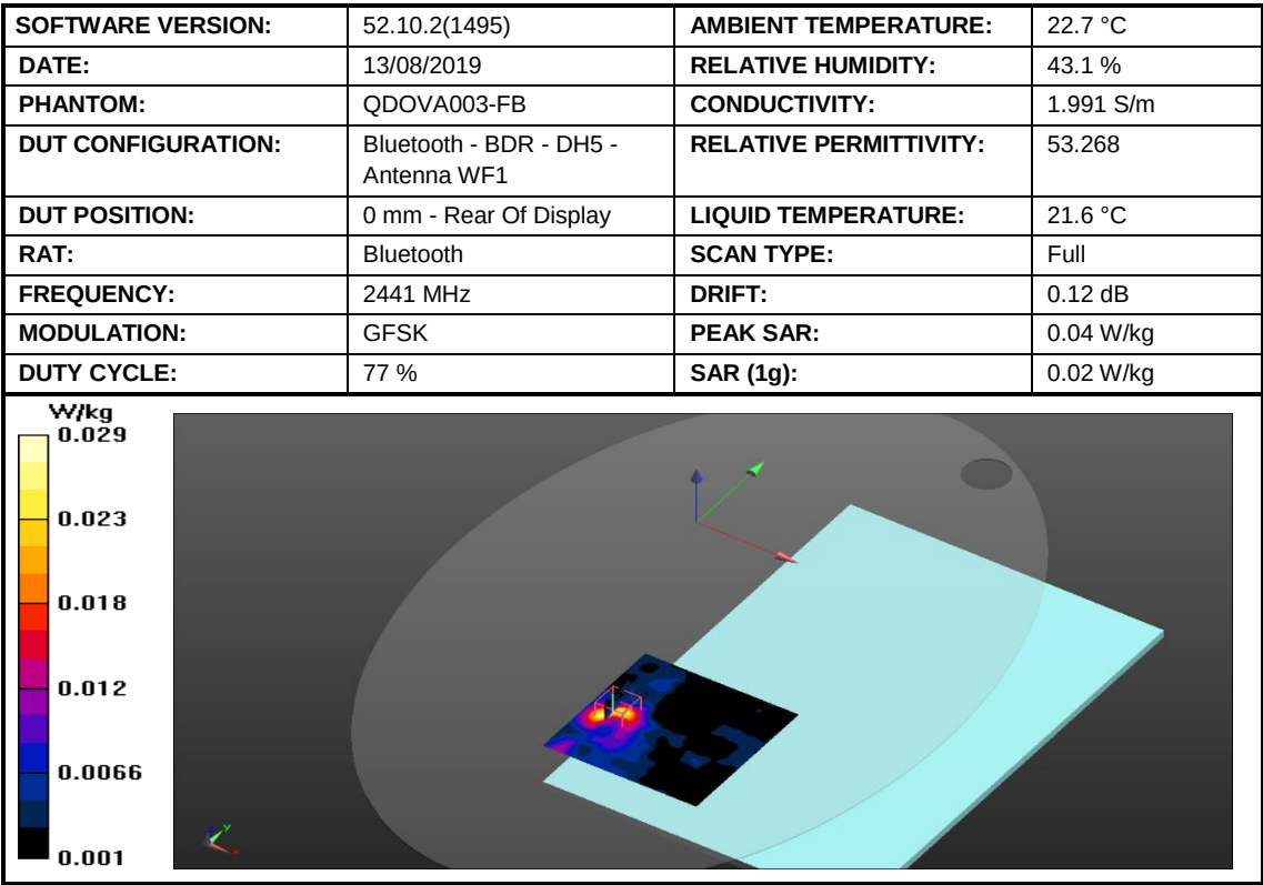
Figure 4: SAR Body Testing Results for the A2141 at 2441 MHz.
