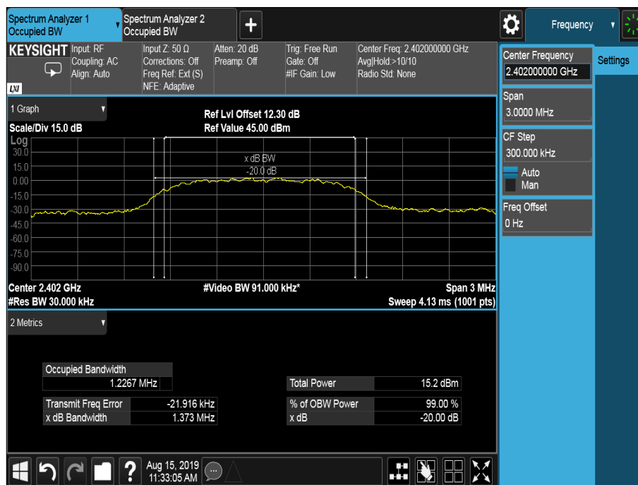
Figure 18 - 2402 MHz - 8-DPSK
