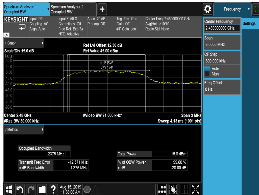
Figure 24 - 2480 MHz - 8-DPSK
