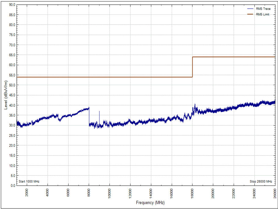
Figure 34 - 2480 MHz - 1 GHz to 26 GHz, Vertical (Average)
