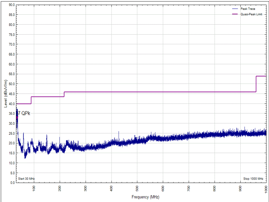
Figure 22 - 2440 MHz, 30 MHz to 1 GHz, Polarity: Vertical
