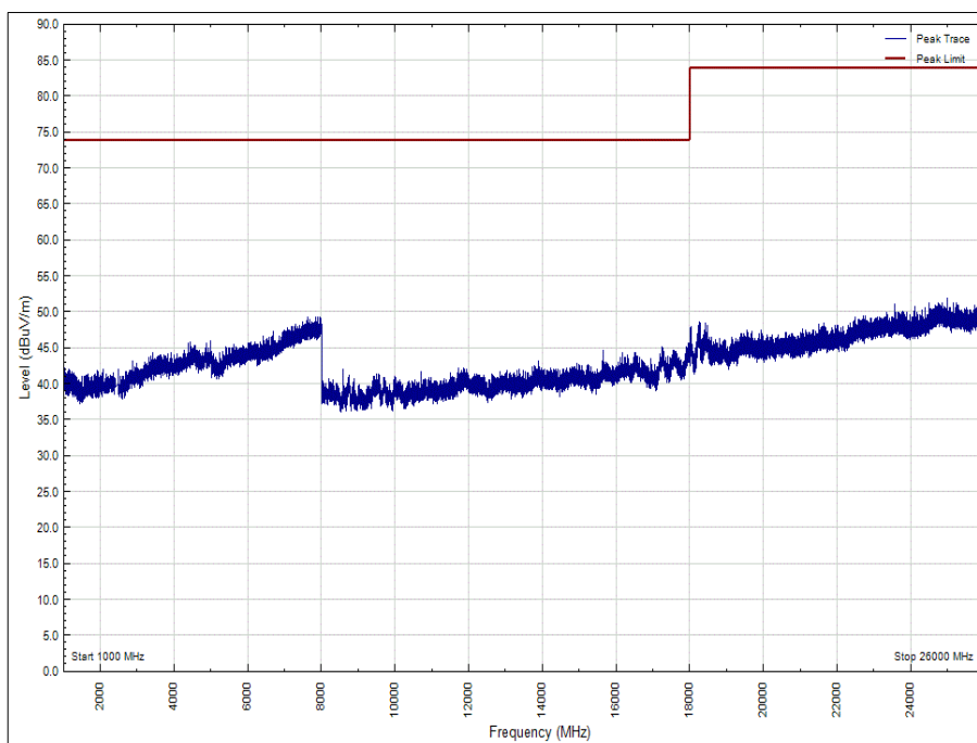
Figure 27 - 2440 MHz - 1 GHz to 26 GHz, Polarity: Horizontal (Peak)
