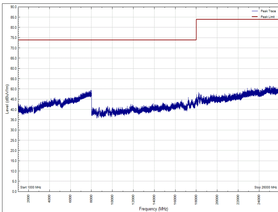
Figure 31 - 2480 MHz - 1 GHz to 26 GHz, Horizontal (Peak)
