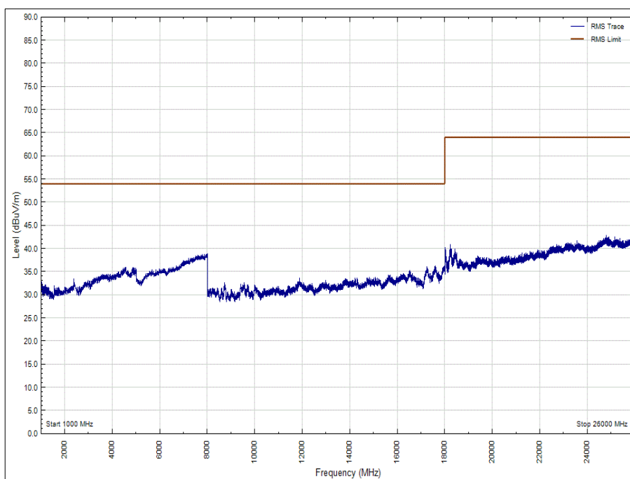
Figure 24 - 2402 MHz - 1 GHz to 26 GHz, Polarity: Horizontal (Average)
