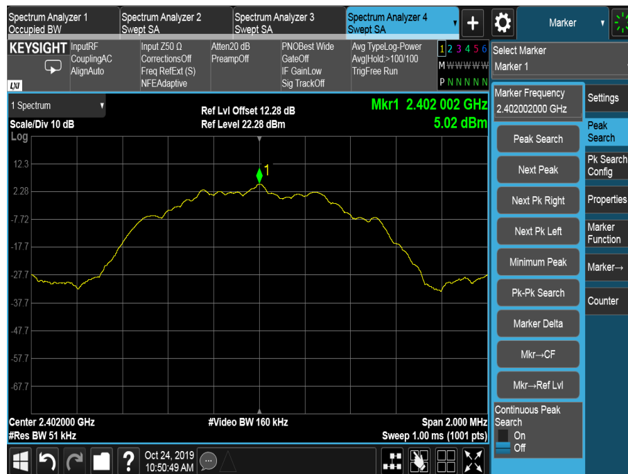
Figure 3 - 2402 MHz, Power Spectral Density
