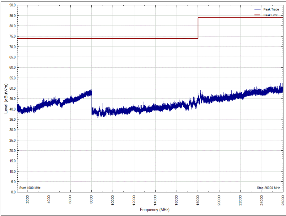
Figure 29 - 2440 MHz - 1 GHz to 26 GHz, Polarity: Vertical (Peak)
