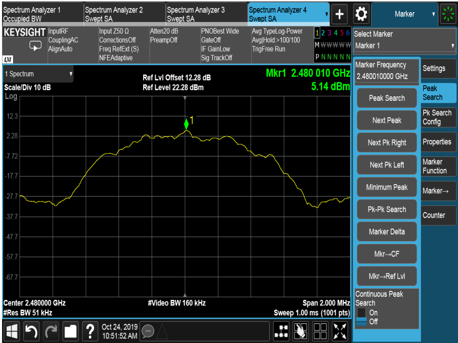
Figure 5 - 2480 MHz, Power Spectral Density
