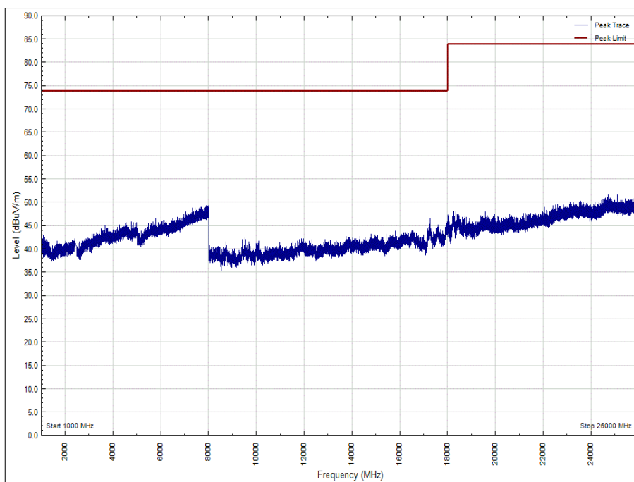
Figure 23 - 2402 MHz - 1 GHz to 26 GHz, Polarity: Horizontal (Peak)
