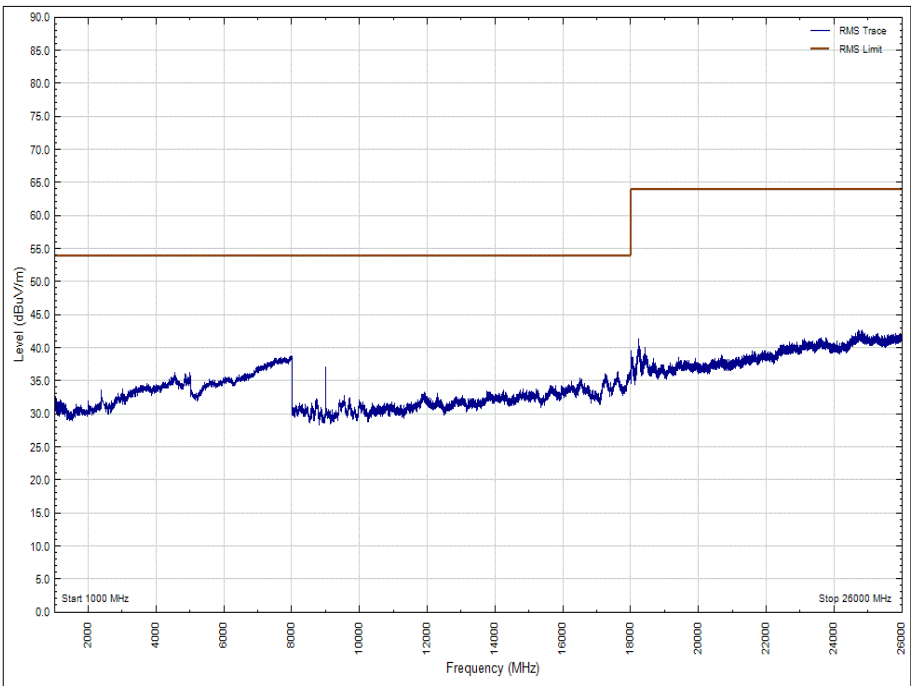
Figure 26 - 2402 MHz - 1 GHz to 26 GHz, Polarity: Vertical (Average)
