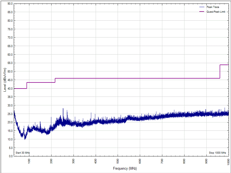
Figure 21 - 2440 MHz, 30 MHz to 1 GHz, Polarity: Horizontal
