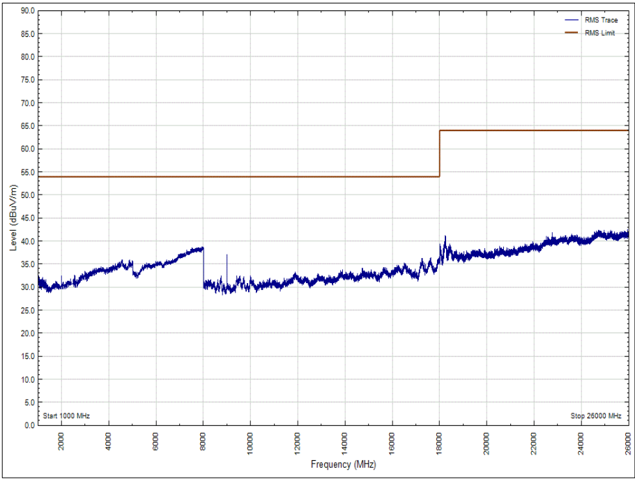
Figure 30 - 2440 MHz - 1 GHz to 26 GHz, Polarity: Vertical (Average)
