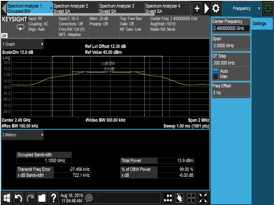
Figure 11 - 2480 MHz
