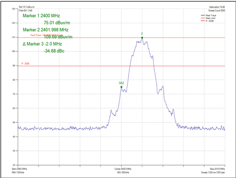
Figure 16 - GFSK/DH1 - 2402 MHz - Band Edge Frequency 2400.0 MHz
