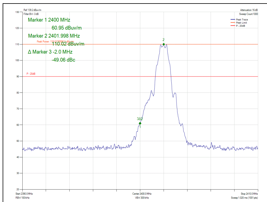
Figure 15 - GFSK/DH1- 2402 MHz – Band Edge Frequency 2400.0 MHz
