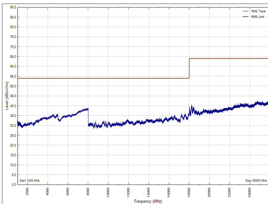
Figure 28 - 2440 MHz - 1 GHz to 26 GHz, Polarity: Horizontal (Average)
