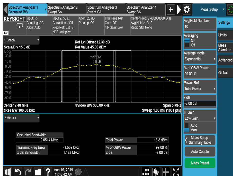
Figure 14 - 2480 MHz
