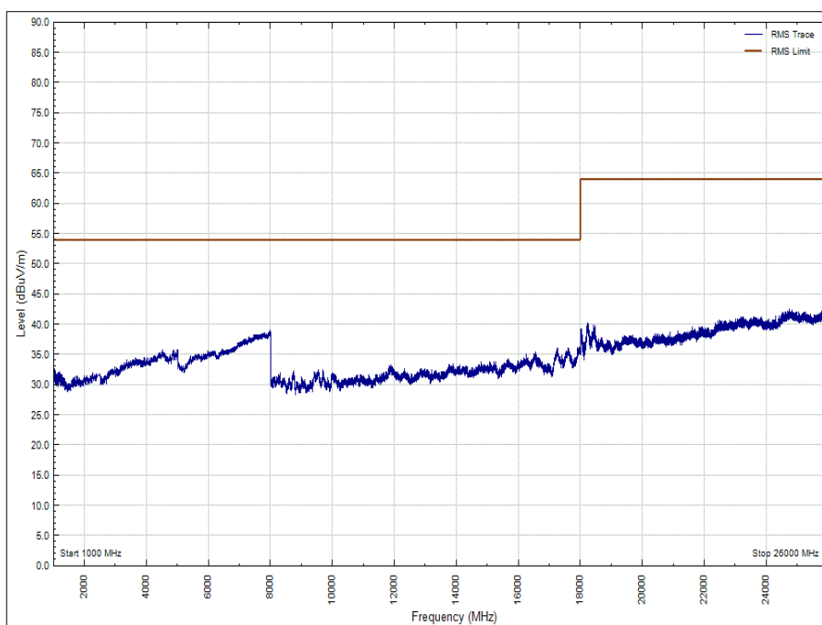
Figure 32 - 2480 MHz - 1 GHz to 26 GHz, Horizontal (Average)
