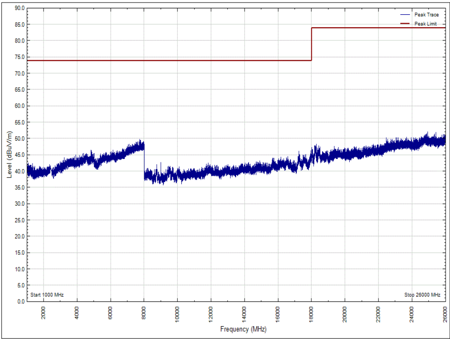
Figure 25 - 2402 MHz - 1 GHz to 26 GHz, Polarity: Vertical (Peak)
