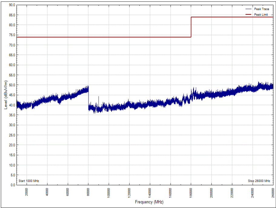
Figure 33 - 2480 MHz - 1 GHz to 26 GHz, Vertical (Peak)
