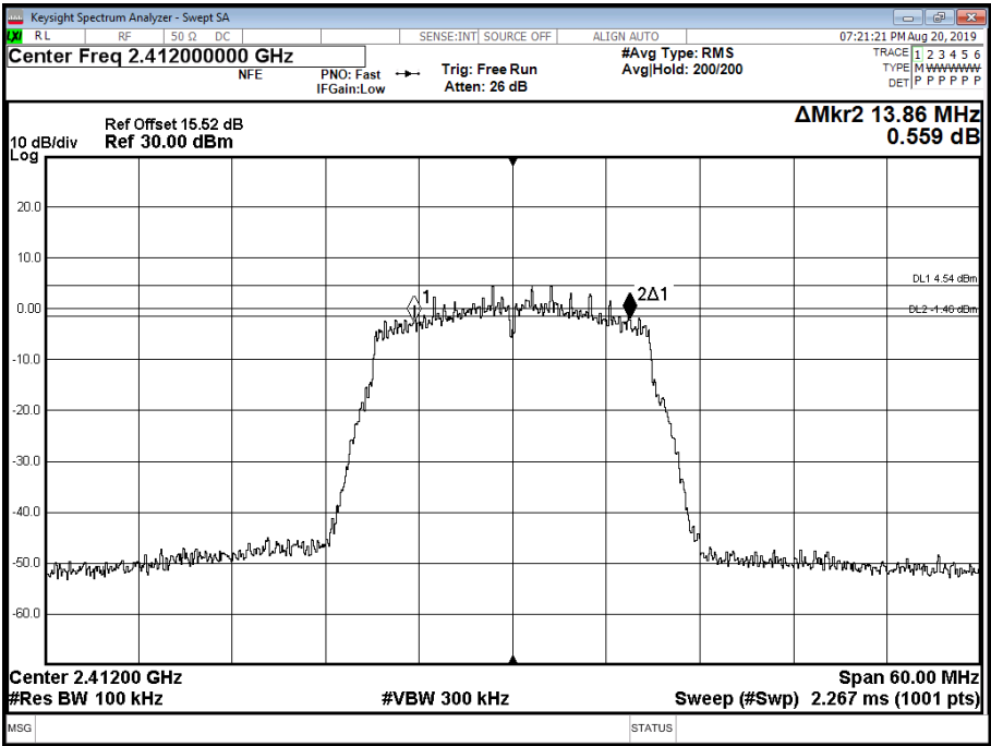
Figure 74 - 2412 MHz - 6 dB DTS Bandwidth
