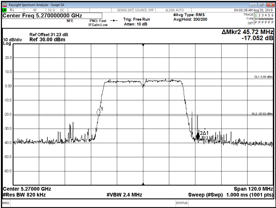
Figure 303 - 5270 MHz - 26 dB Emission Bandwidth
