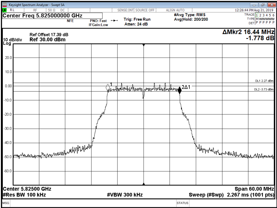
Figure 572 - 5825 MHz - 6 dB DTS Bandwidth
