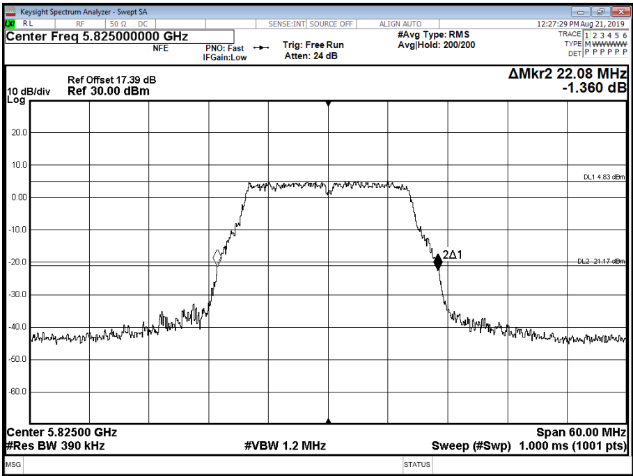
Figure 573 - 5825 MHz - 26 dB Emission Bandwidth
