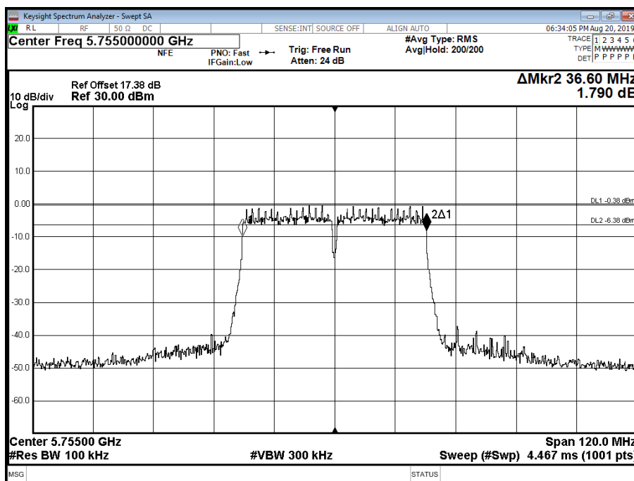
Figure 692 - 5755 MHz - 6 dB DTS Bandwidth
