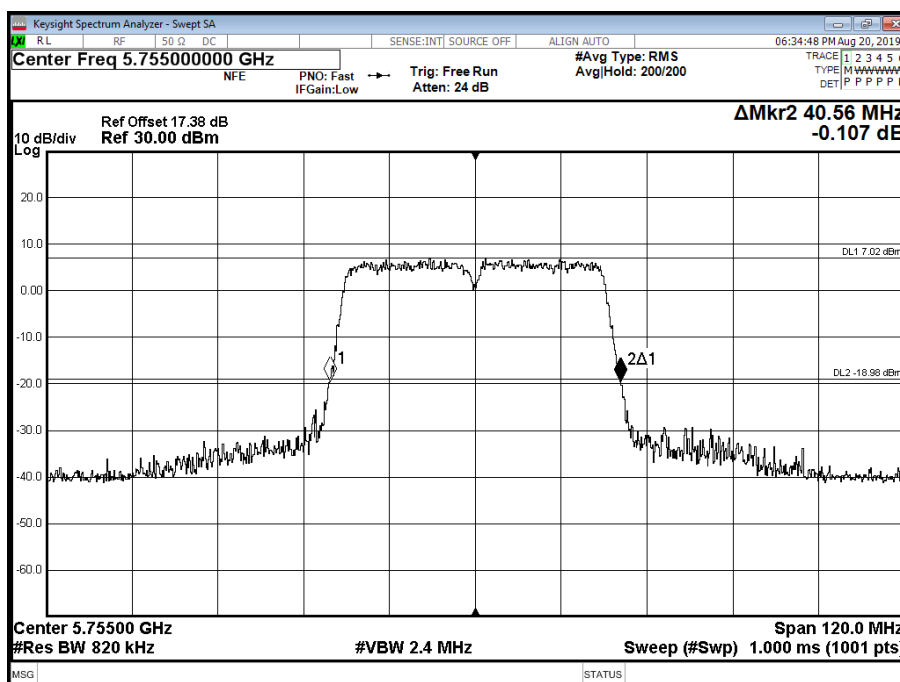
Figure 693 - 5755 MHz - 26 dB Emission Bandwidth
