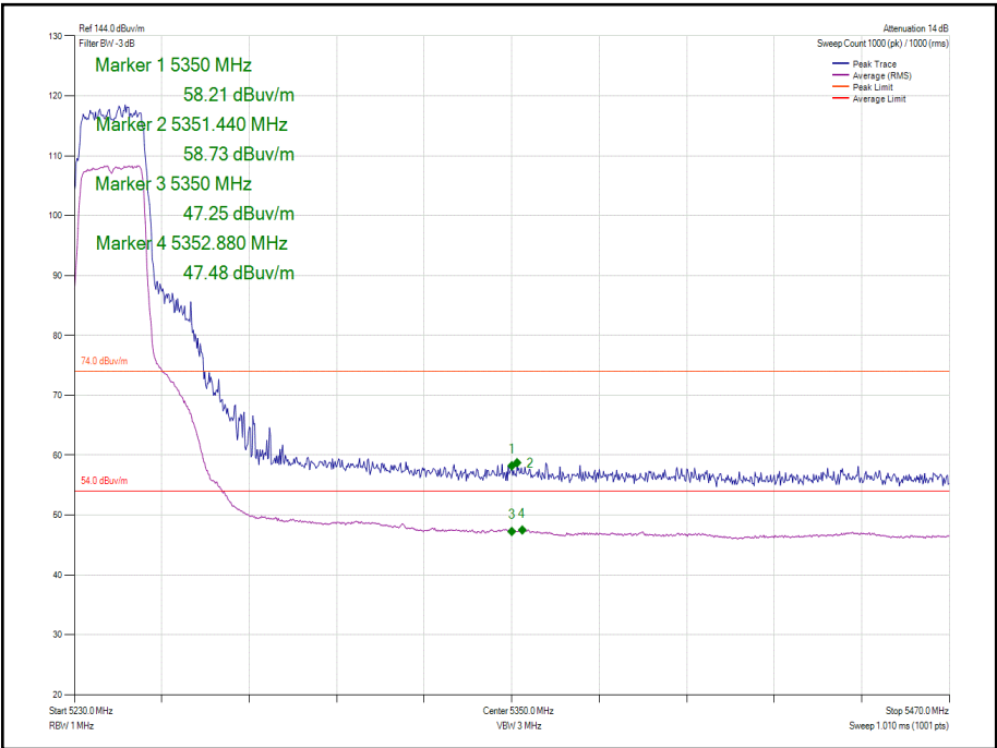
Figure 1061 - 802.11n HT20 SDM Cores 0-1-2 - 5240 MHz Band Edge Frequency 5350 MHz
