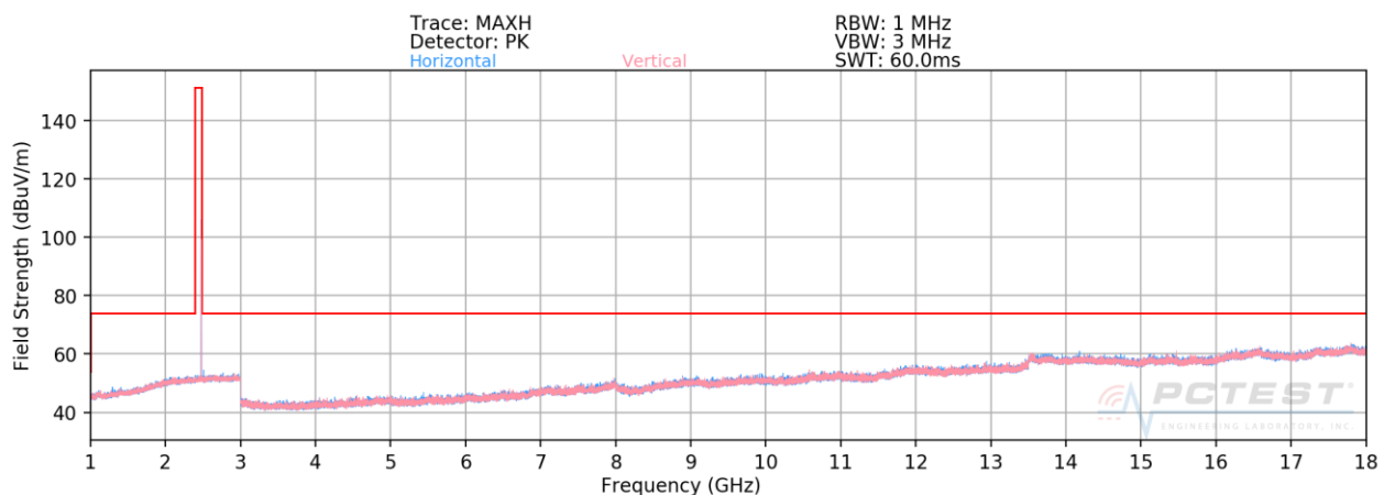
Plot 7-62. Radiated Spurious Plot 1-18GHz Ant-1 (4Mbps, HDR4, ePA – Ch. 75, Ant. Pol. H & V)
