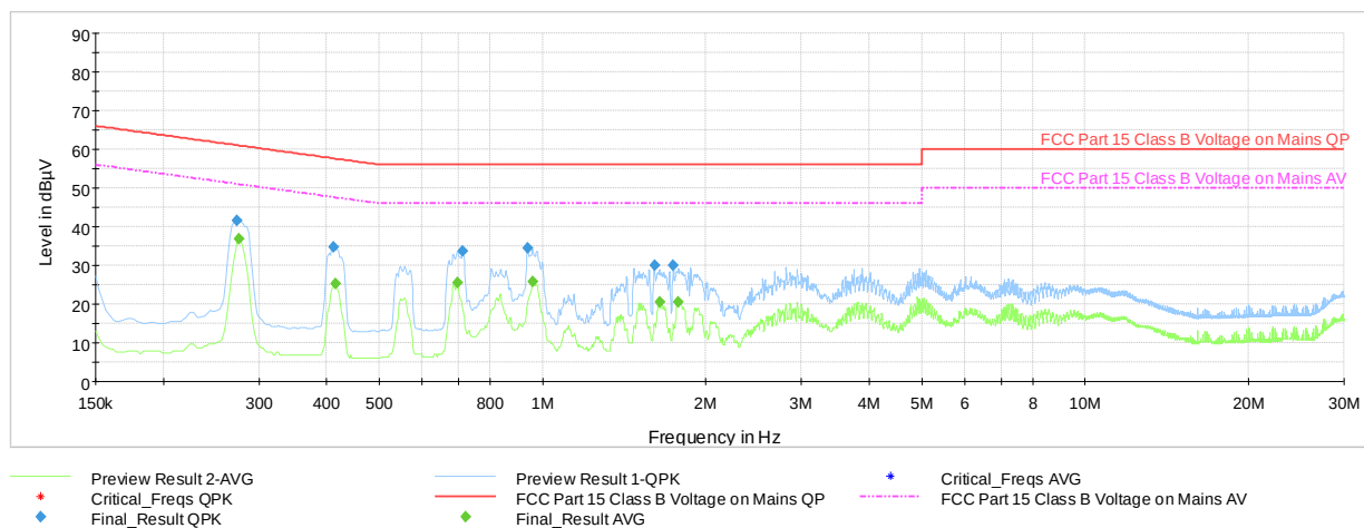
Plot 7-74. AC Line Conducted Plot with Bluetooth HDR4 ePA – Ch.38 (L1, with AC/DC Adapter)
