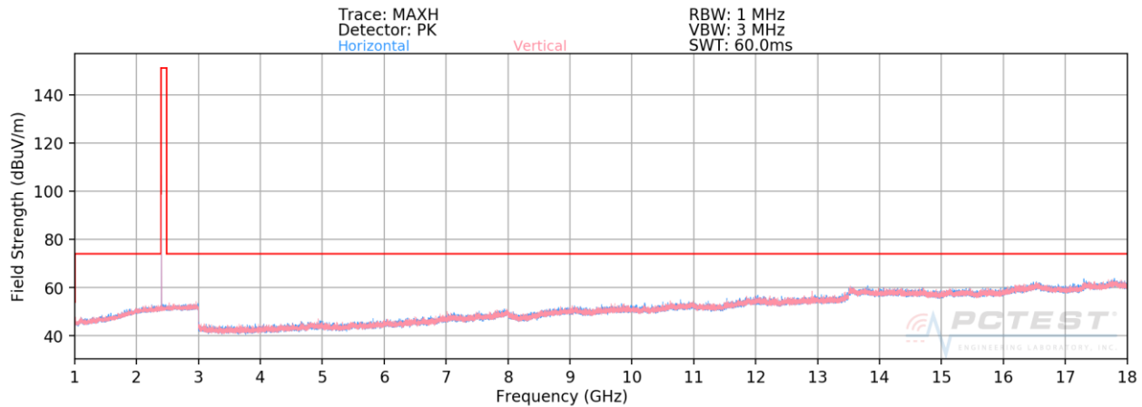
Plot 7-60. Radiated Spurious Plot 1-18GHz Ant-1 (4Mbps, HDR4, ePA – Ch. 1, Ant. Pol. H & V)
