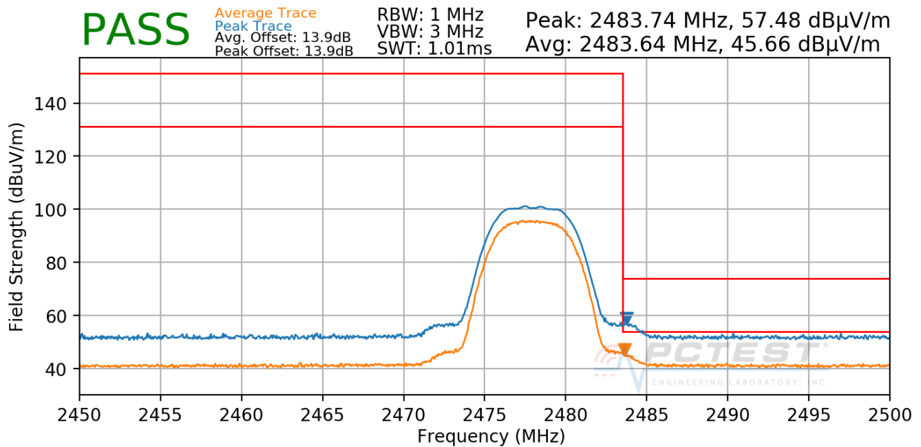
Plot 7-72. Radiated Restricted Upper Band Edge Measurement Ant-1 (Average & Peak)
