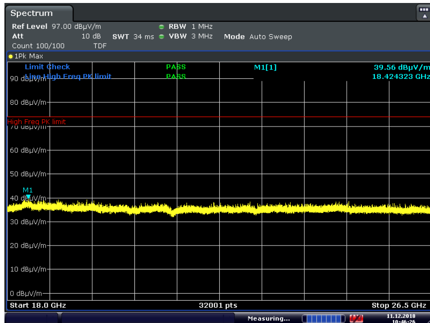
Plot 7-64. Radiated Spurious Plot Above 18GHz Ant-0 (4Mbps, HDR4, ePA – Ch.38, Ant. Pol. V)
