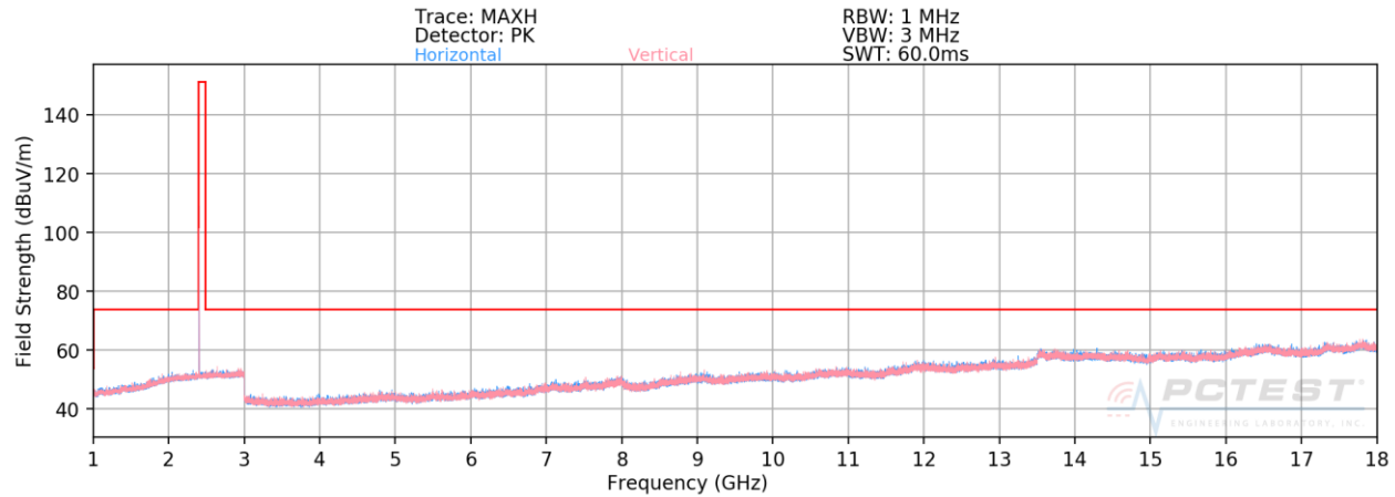
Plot 7-57. Radiated Spurious Plot 1-18GHz Ant-0 (4Mbps, HDR4, ePA – Ch. 1, Ant. Pol. H & V)
