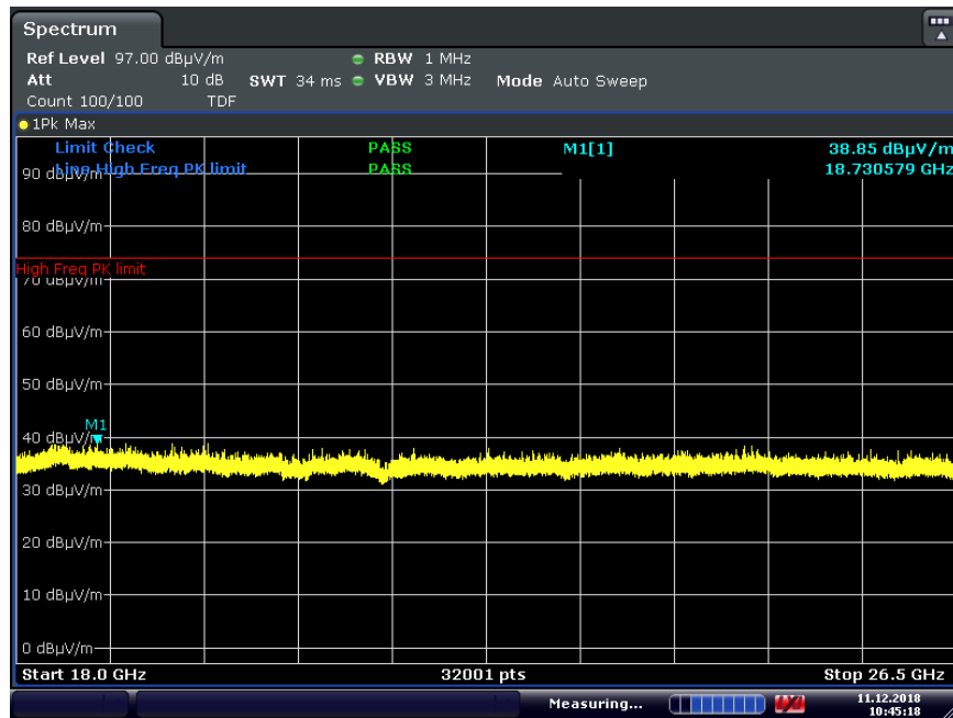
Plot 7-63. Radiated Spurious Plot Above 18GHz Ant-0 (4Mbps, HDR4, ePA – Ch.38, Ant. Pol. H)
