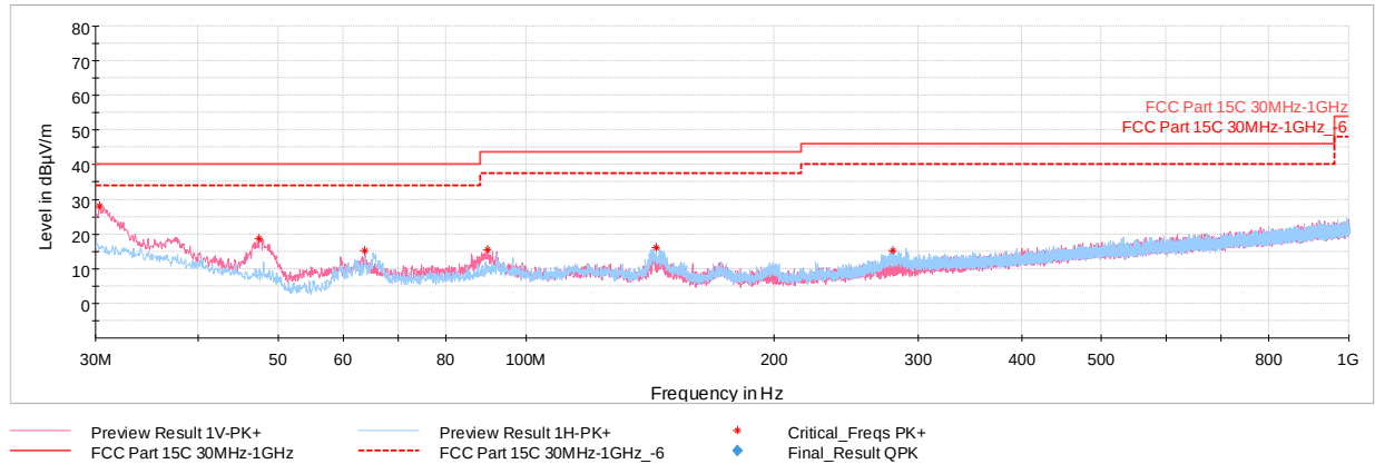
Plot 7-73. Radiated Spurious Plot below 1GHz (4Mbps, HDR4 ePA – Ch.1, Pol. H & V, with AC/DC Adapter)
