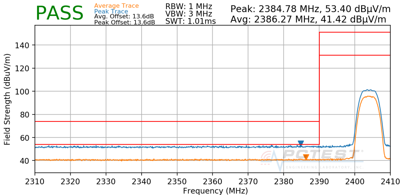
Plot 7-70. Radiated Restricted Lower Band Edge Measurement Ant-1 (Average & Peak)
