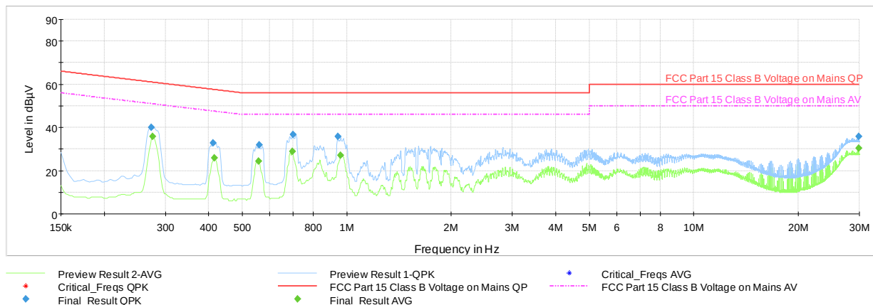
Plot 7-75. AC Line Conducted Plot with Bluetooth HDR4 ePA – Ch.38 (N, with AC/DC Adapter)
