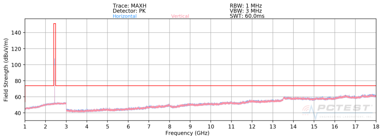
Plot 7-61. Radiated Spurious Plot 1-18GHz Ant-1 (4Mbps, HDR4, ePA – Ch. 38, Ant. Pol. H & V)
