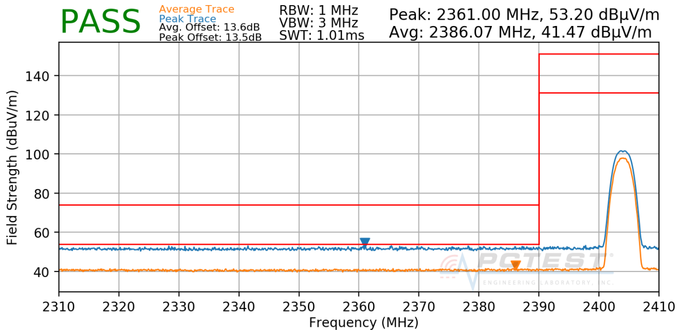
Plot 7-69. Radiated Restricted Lower Band Edge Measurement Ant-1 (Average & Peak)
