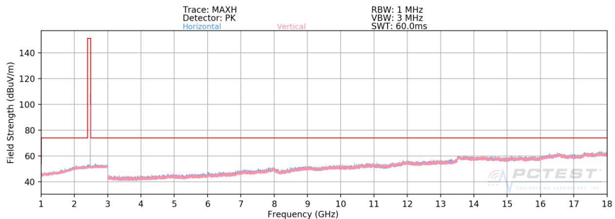
Plot 7-59. Radiated Spurious Plot 1-18GHz Ant-0 (4Mbps, HDR4, ePA – Ch. 75, Ant. Pol. H & V)
