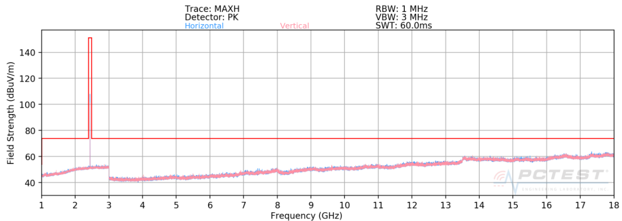
Plot 7-58. Radiated Spurious Plot 1-18GHz Ant-0 (4Mbps, HDR4, ePA – Ch. 38, Ant. Pol. H & V)
