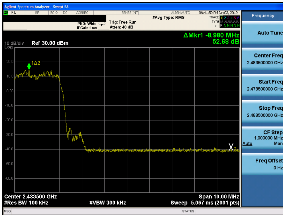
Plot 7-28. Band Edge Plot ANT 1 (Bluetooth with Hopping Enabled, 8DPSK, ePA)
