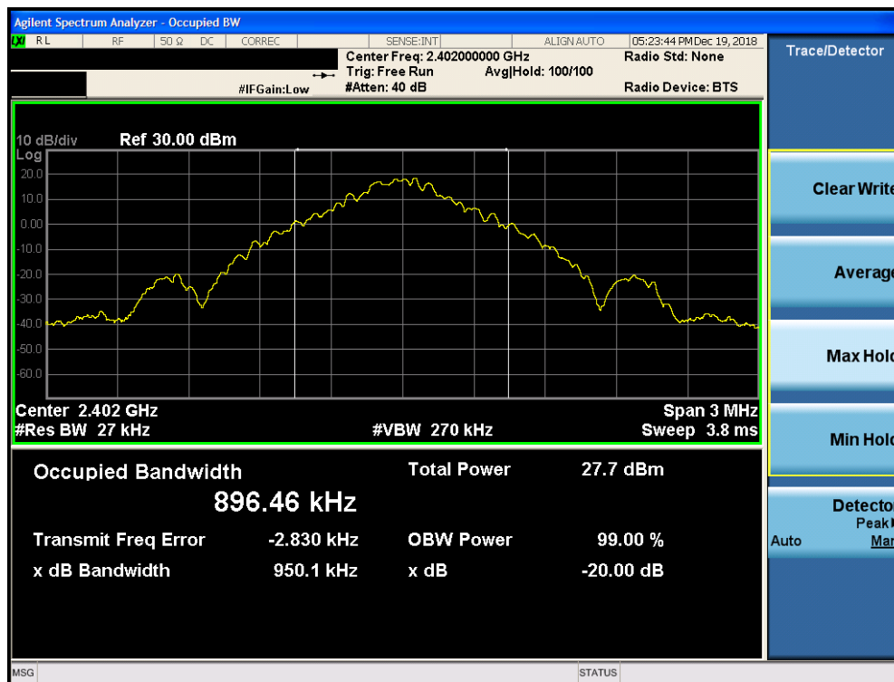
Plot 7-7. 20dB Bandwidth Plot ANT 1 (Bluetooth, GFSK, ePA – Ch. 0)
