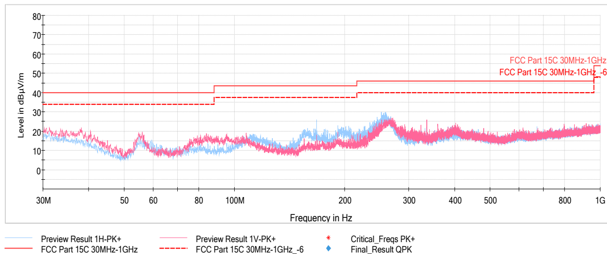
Plot 7-281. Radiated Spurious Plot below 1GHz (2.4GHz Ch 78– 5GHz Ch 36), with Laptop
