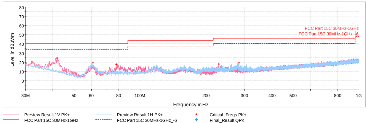
Plot 7-126. Radiated Spurious Plot below 1GHz 802.11n CDD Ch. 6 with Laptop
