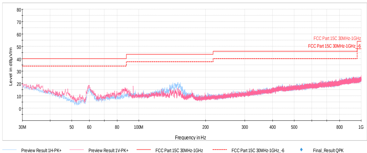
Plot 7-73. Radiated Spurious Plot below 1GHz (1Mbps, ePA – Ch.0, Pol. H & V, with AC/DC Adapter)
