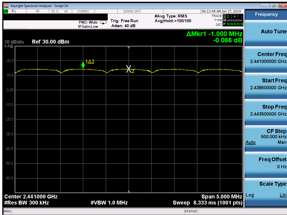
Plot 7-30. Channel Spacing Plot ANT 0 (Bluetooth, 8DPSK, ePA)
