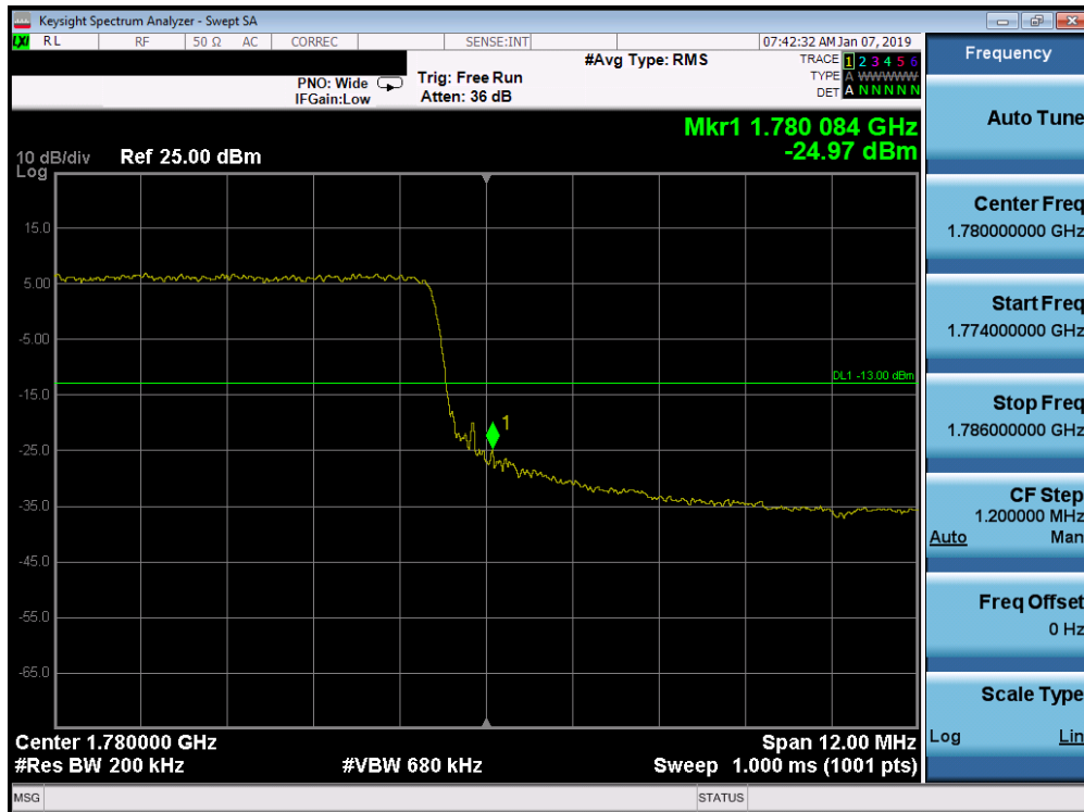
Plot 7-248. Upper Band Edge Plot (Band 66 - 15.0MHz QPSK - Full RB Configuration)
