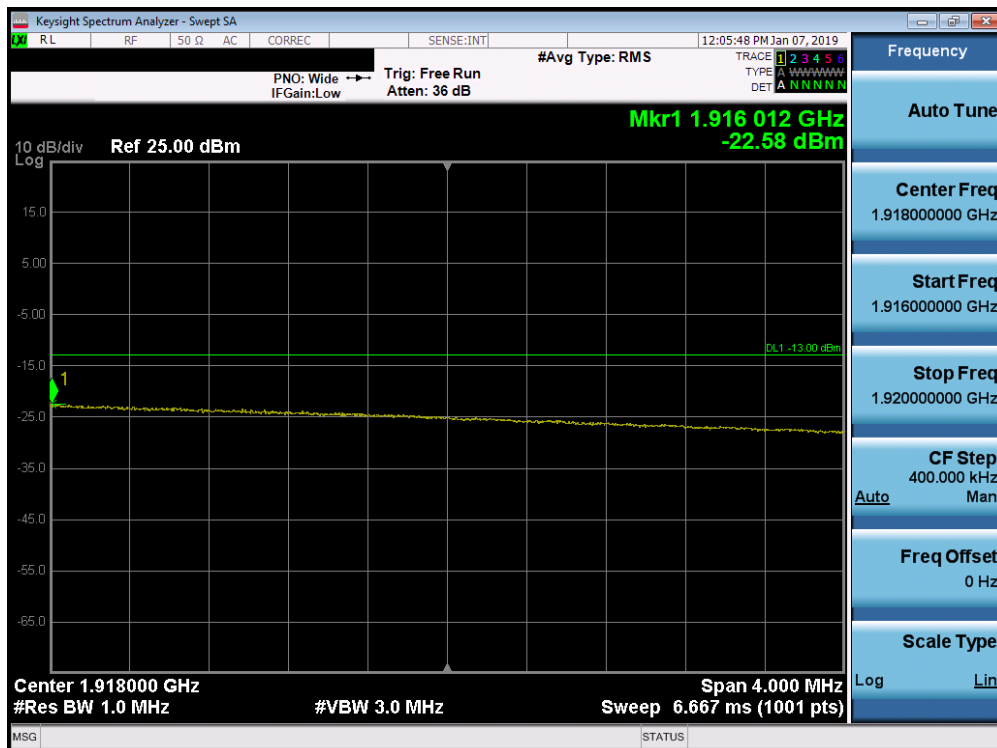
Plot 7-301. Upper Extended Band Edge Plot (Band 25 - 20.0MHz QPSK - Full RB Configuration)
