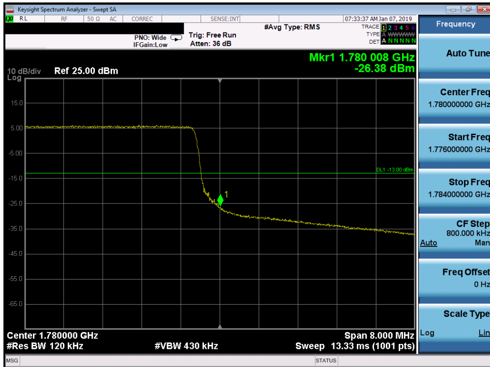
Plot 7-244. Upper Band Edge Plot (Band 66 - 10.0MHz QPSK - Full RB Configuration)
