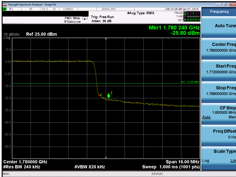
Plot 7-252. Upper Band Edge Plot (Band 66 - 20.0MHz QPSK - Full RB Configuration)
