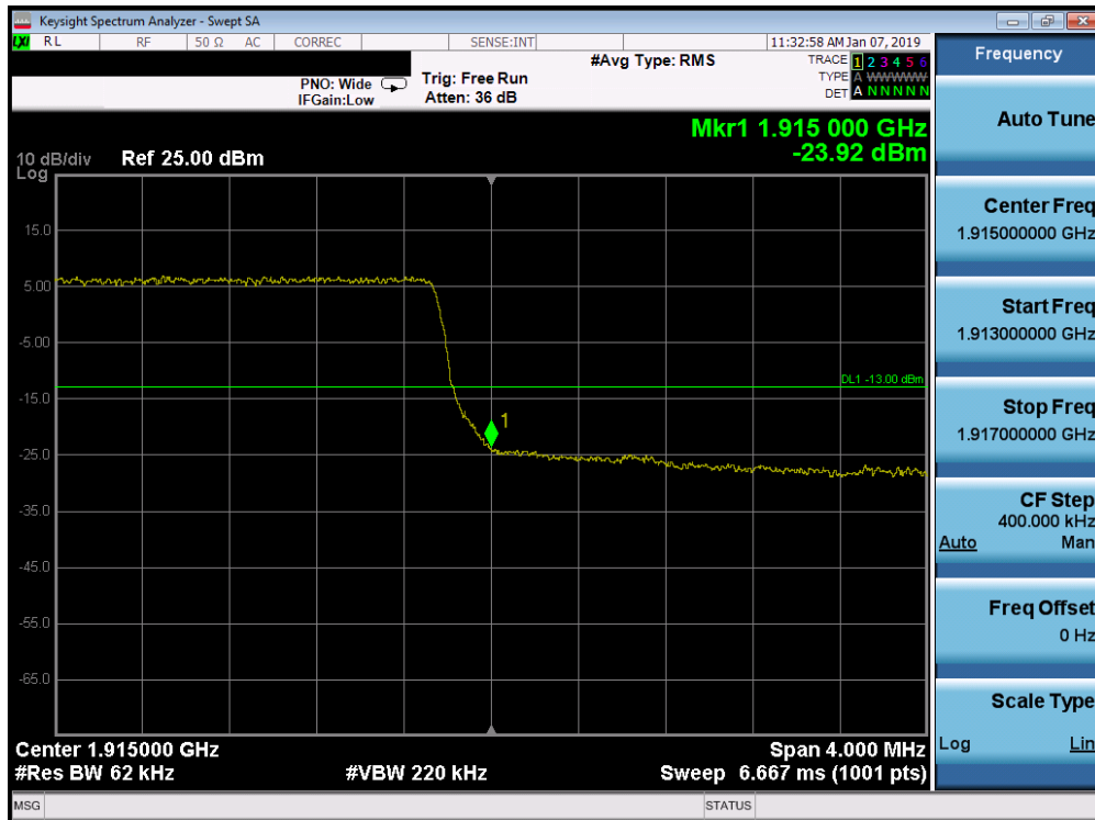
Plot 7-288. Upper Band Edge Plot (Band 25 - 5.0MHz QPSK - Full RB Configuration)
