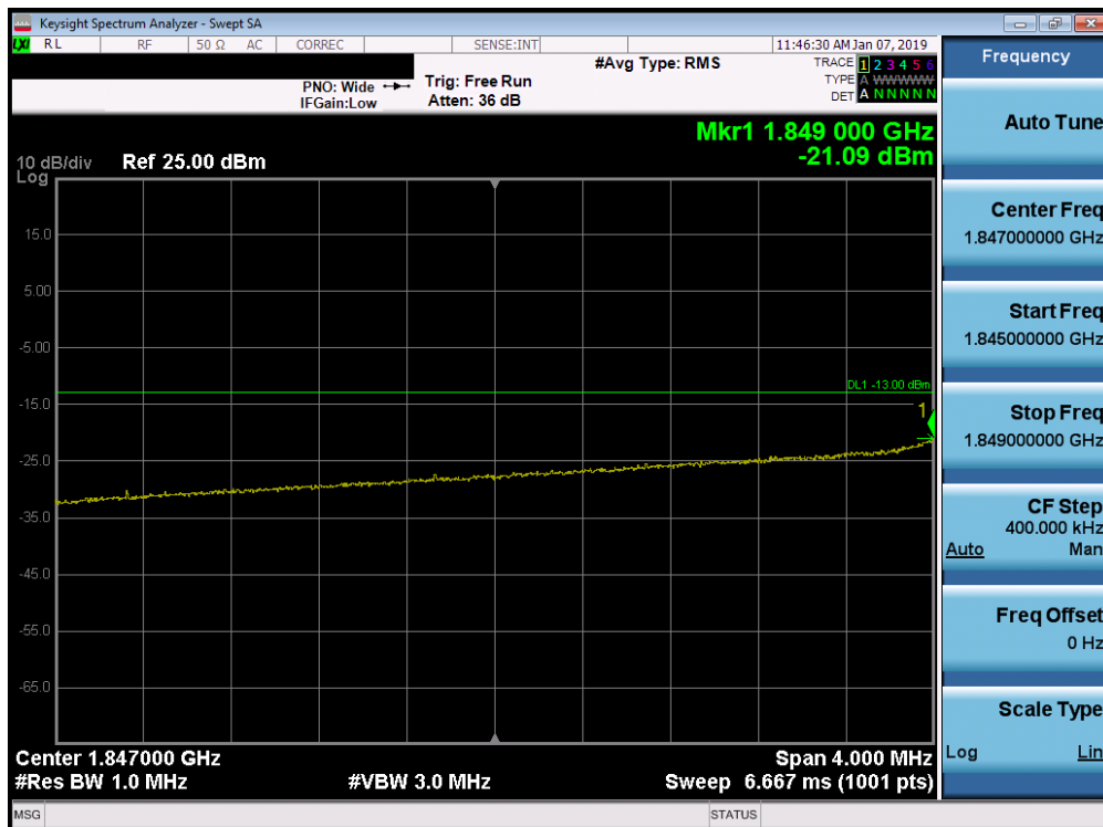
Plot 7-291. Lower Extended Band Edge Plot (Band 25 - 10.0MHz QPSK - Full RB Configuration)
