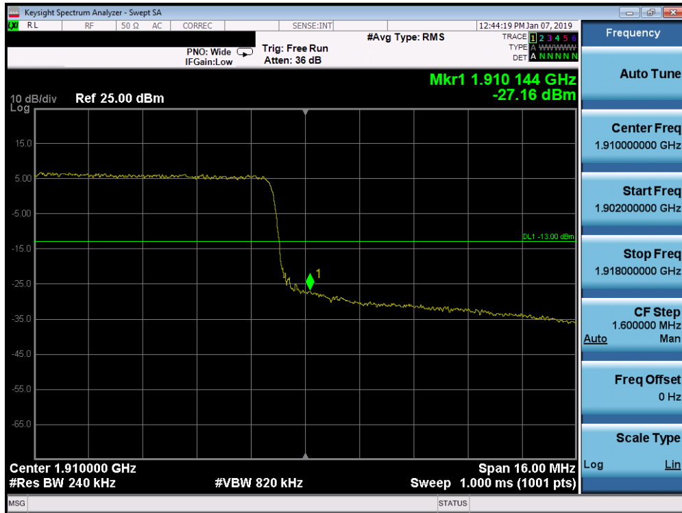
Plot 7-324. Upper Band Edge Plot (Band 2 - 20.0MHz QPSK - Full RB Configuration)
