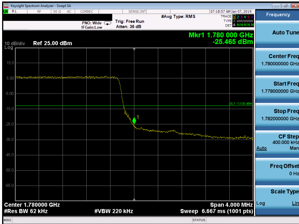
Plot 7-240. Upper Band Edge Plot (Band 66 - 5.0MHz QPSK - Full RB Configuration)
