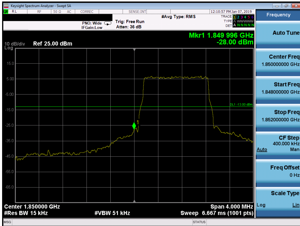
Plot 7-302. Lower Band Edge Plot (Band 2 - 1.4MHz QPSK - Full RB Configuration)
