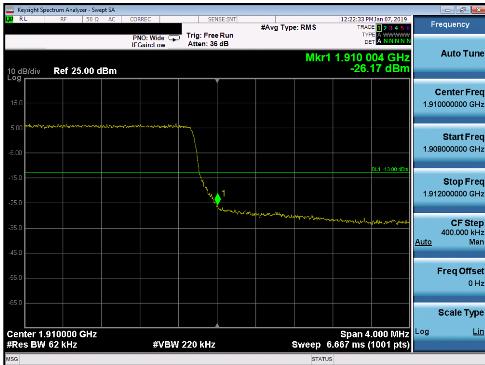
Plot 7-312. Upper Band Edge Plot (Band 2 - 5.0MHz QPSK - Full RB Configuration)
