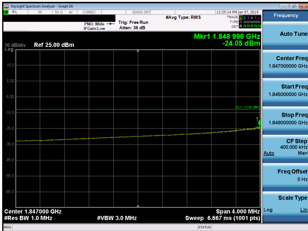
Plot 7-319. Lower Extended Band Edge Plot (Band 2 - 15.0MHz QPSK - Full RB Configuration)
