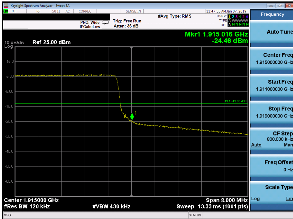
Plot 7-292. Upper Band Edge Plot (Band 25 - 10.0MHz QPSK - Full RB Configuration)
