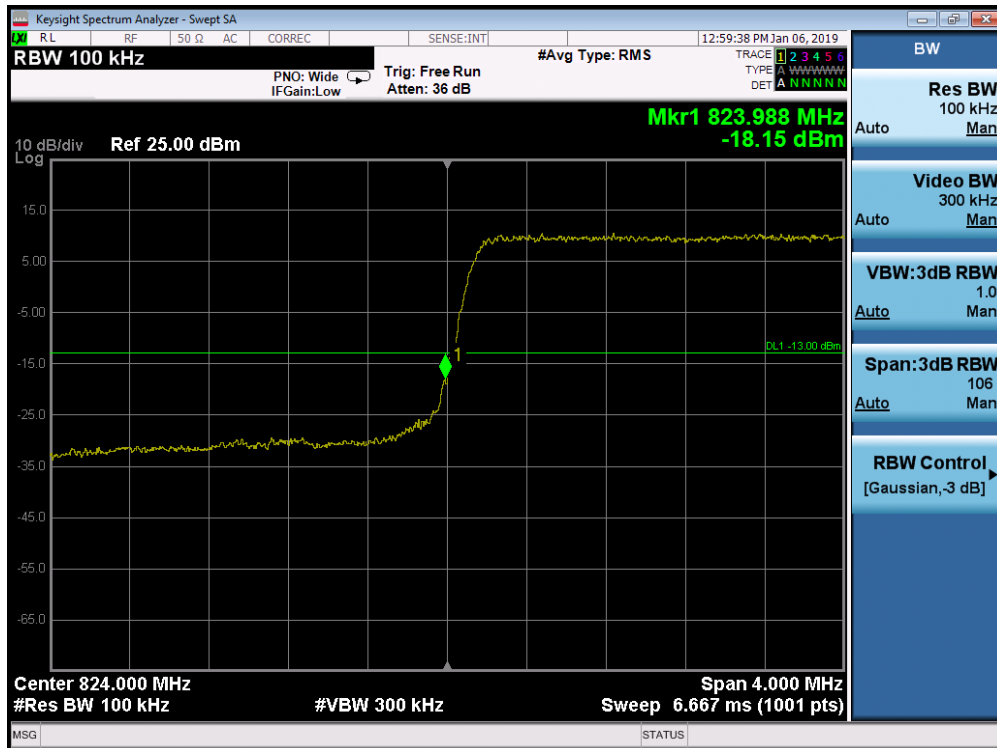
Plot 7-216. Lower Band Edge Plot (Band 26 - 3.0MHz QPSK - Full RB Configuration)
