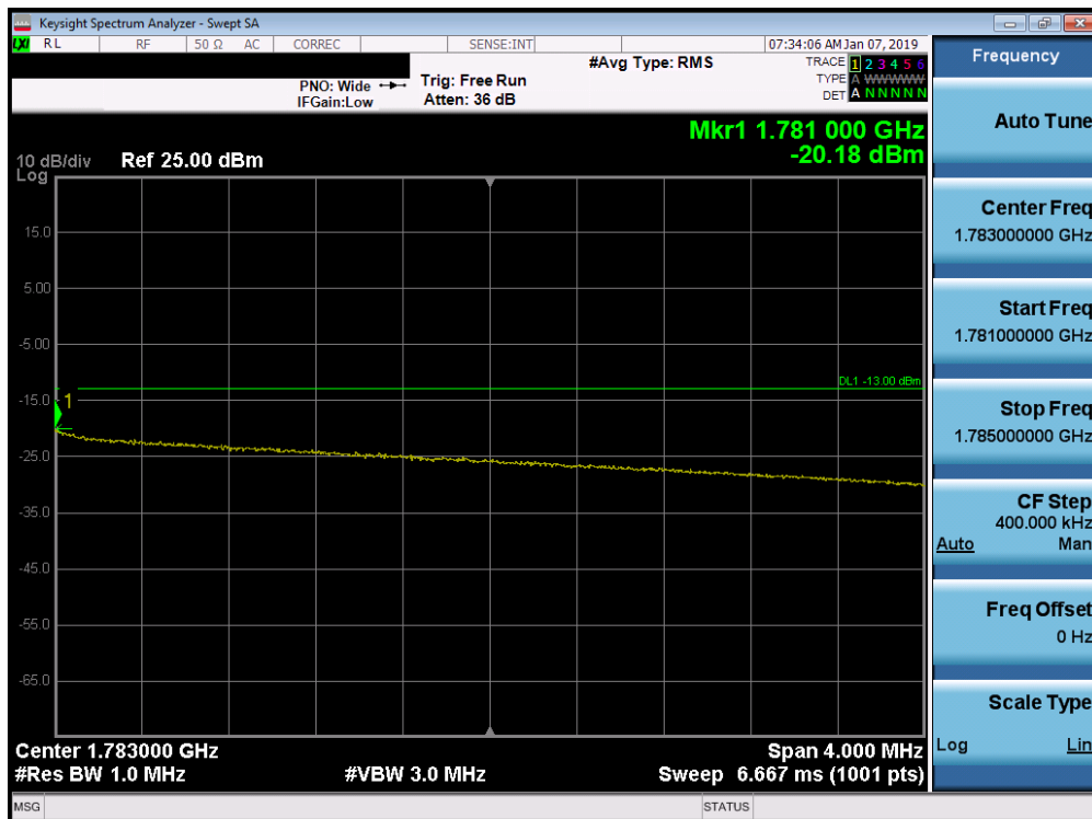
Plot 7-245. Upper Extended Band Edge Plot (Band 66 - 10.0MHz QPSK - Full RB Configuration)
