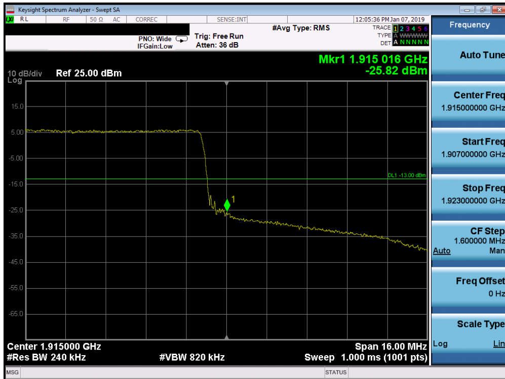
Plot 7-300. Upper Band Edge Plot (Band 25 - 20.0MHz QPSK - Full RB Configuration)
