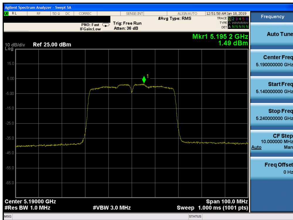
Plot 7-125. Power Spectral Density Plot MIMO/CDD CORE1 (40MHz BW 802.11n (UNII Band 1) – Ch. 38)
