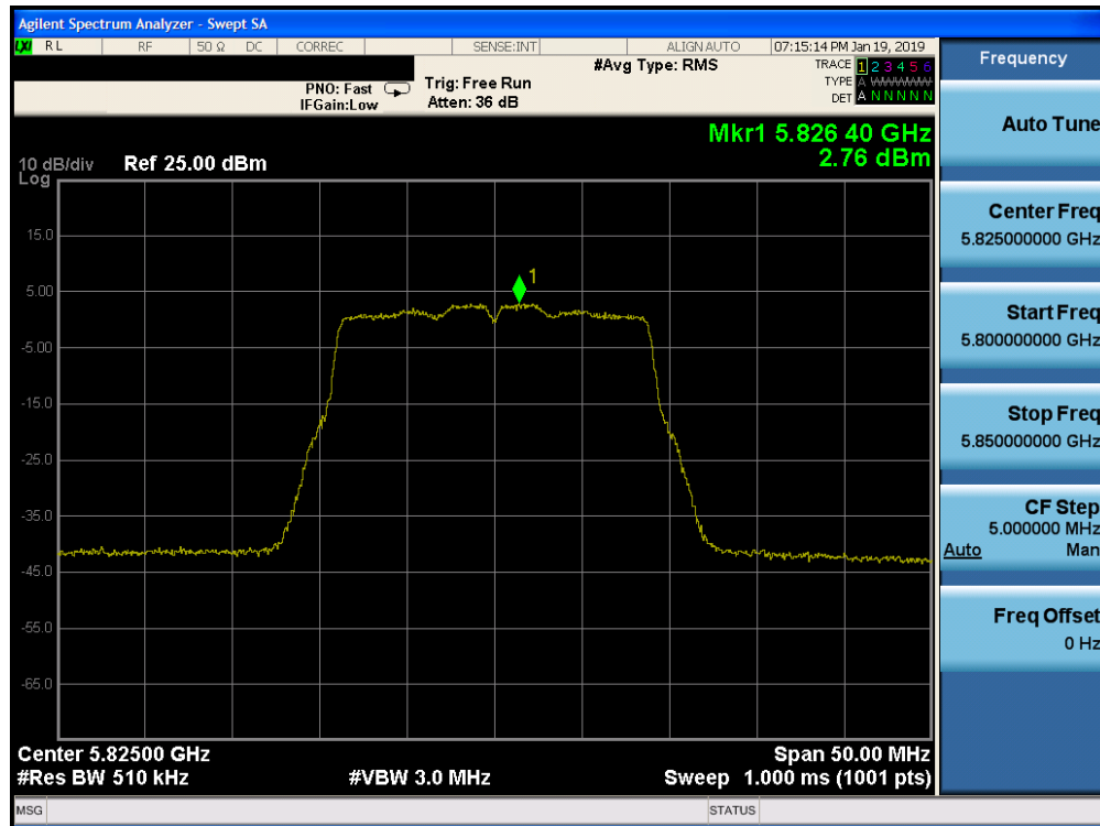
Plot 7-163. Power Spectral Density Plot MIMO/CDD CORE1 (20MHz BW 802.11n (UNII Band 3) – Ch. 165)
