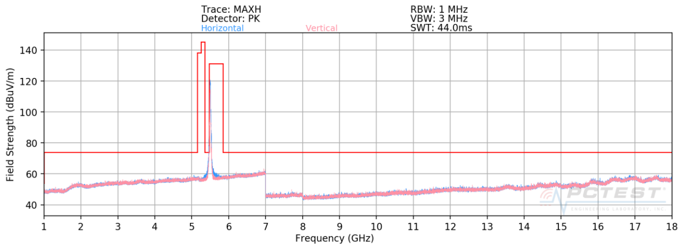
Plot 7-176. Radiated Spurious Plot above 1GHz SISO CORE0 (802.11n – U2C Ch. 100)
