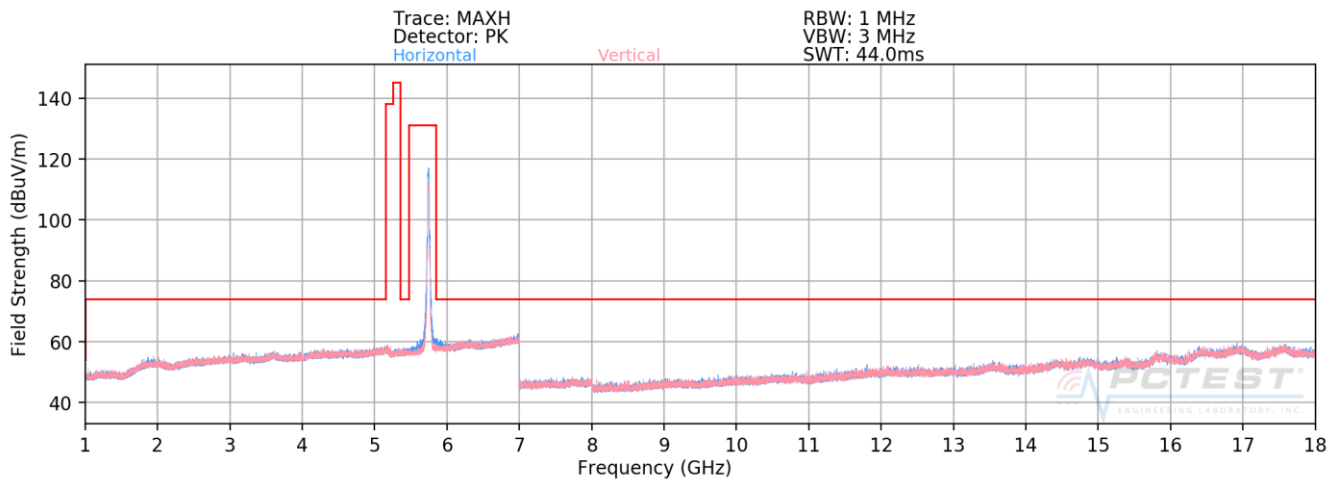
Plot 7-191. Radiated Spurious Plot above 1GHz SISO CORE1 (802.11n – U3 Ch. 149)
