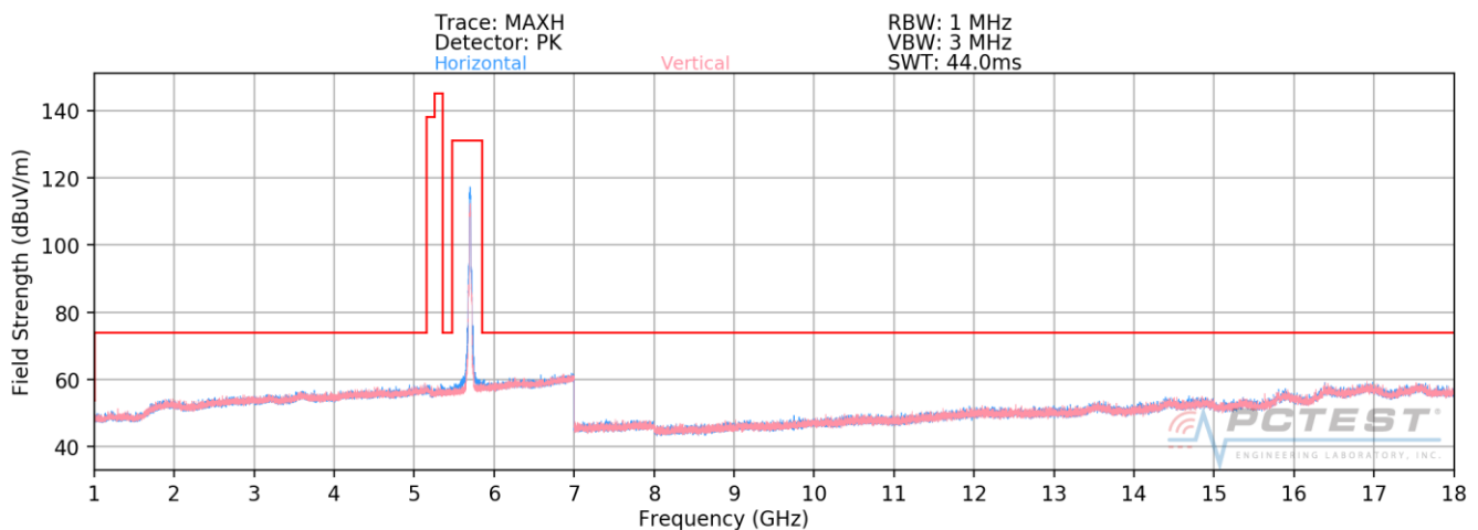
Plot 7-190. Radiated Spurious Plot above 1GHz SISO CORE1 (802.11n – U2C Ch. 144)
