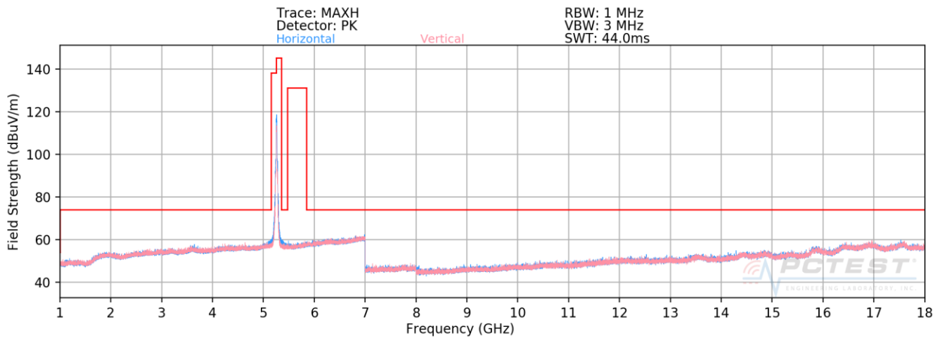
Plot 7-185. Radiated Spurious Plot above 1GHz SISO CORE1 (802.11n – U2A Ch. 52)
