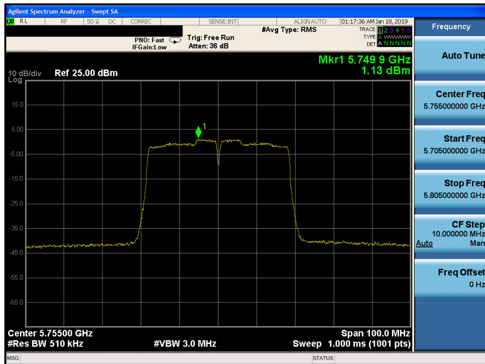
Plot 7-164. Power Spectral Density Plot MIMO/CDD CORE0 (40MHz BW 802.11n (UNII Band 3) – Ch. 151)
