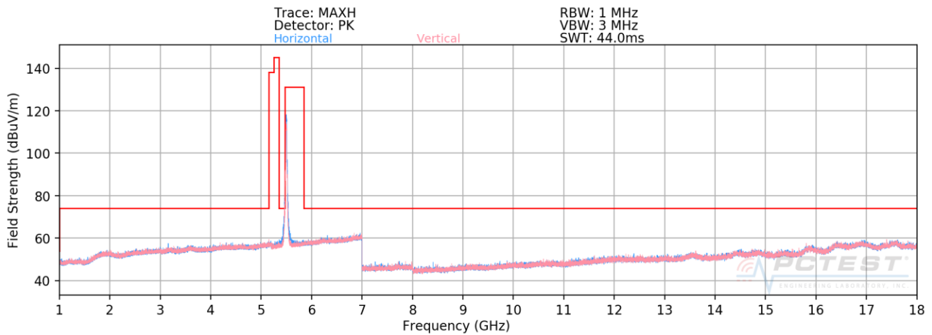
Plot 7-188. Radiated Spurious Plot above 1GHz SISO CORE1 (802.11n – U2C Ch. 100)
