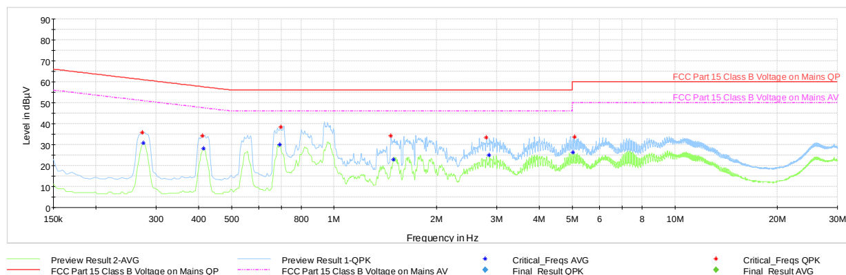
Plot 7-281. Line Conducted Plot with 802.11n UNII Band 1 Ch 36 (N), with AC/DC Adapter
