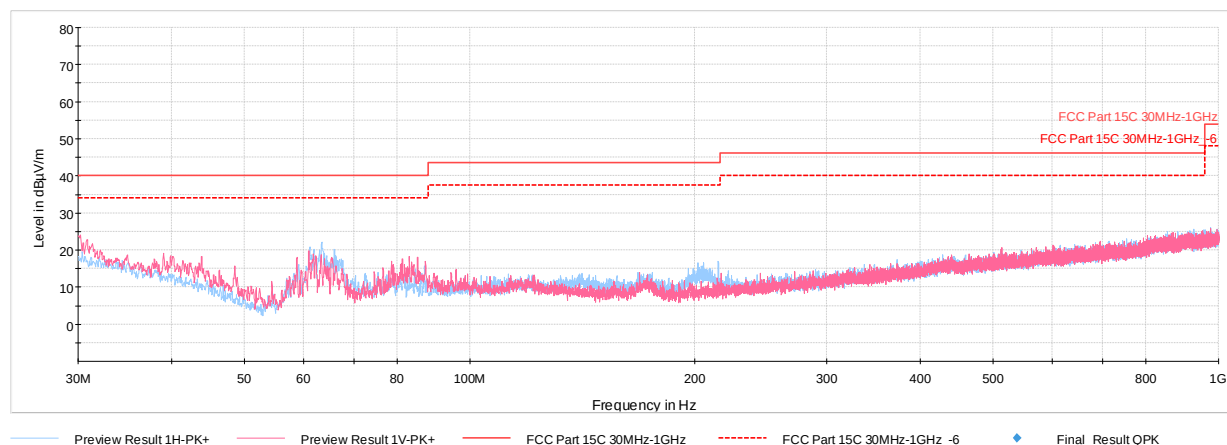
Plot 7-130. Radiated Spurious Plot below 1GHz 802.11n CDD Ch.6, with Laptop
