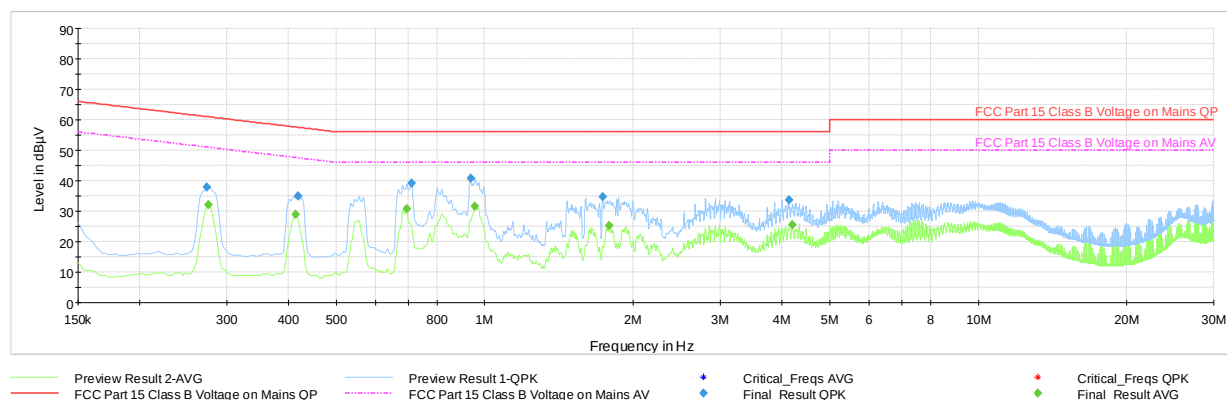
Plot 7-132. AC Line Conducted Plot with 802.11n CDD Ch.6 (N, with AC/DC Adapter)
