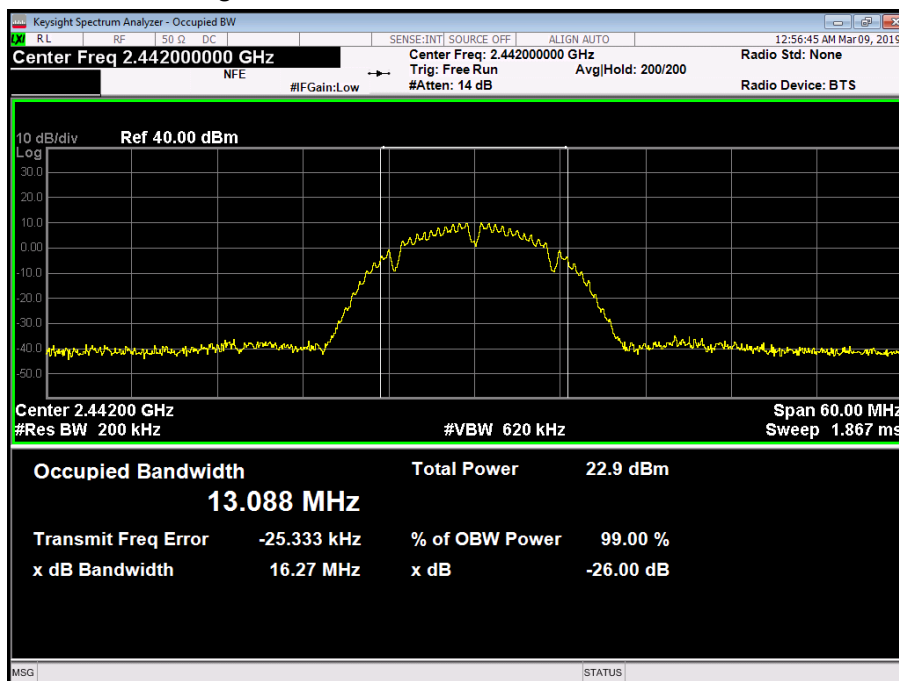
Figure 6 - 2442 MHz - 99% Occupied Bandwidth
