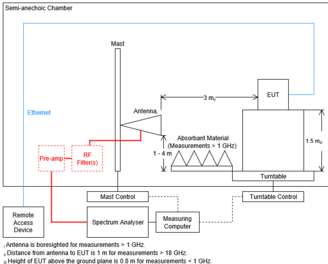
Figure 2 – Radiated Test Setup Diagram
