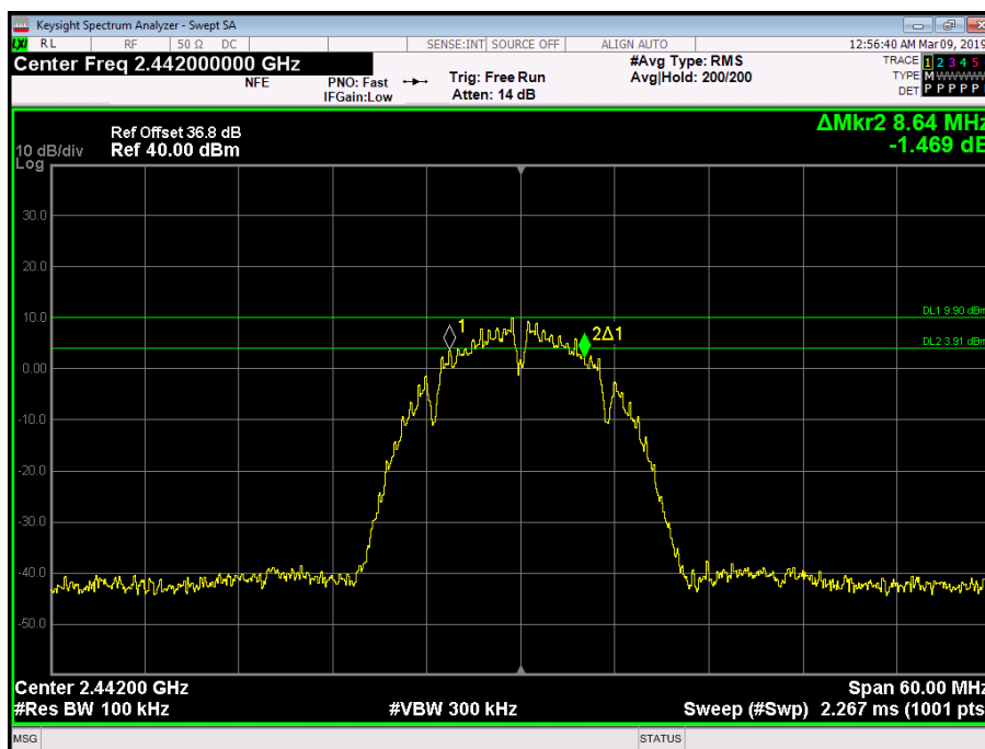
Figure 5 - 2442 MHz - 6 dB DTS Bandwidth
