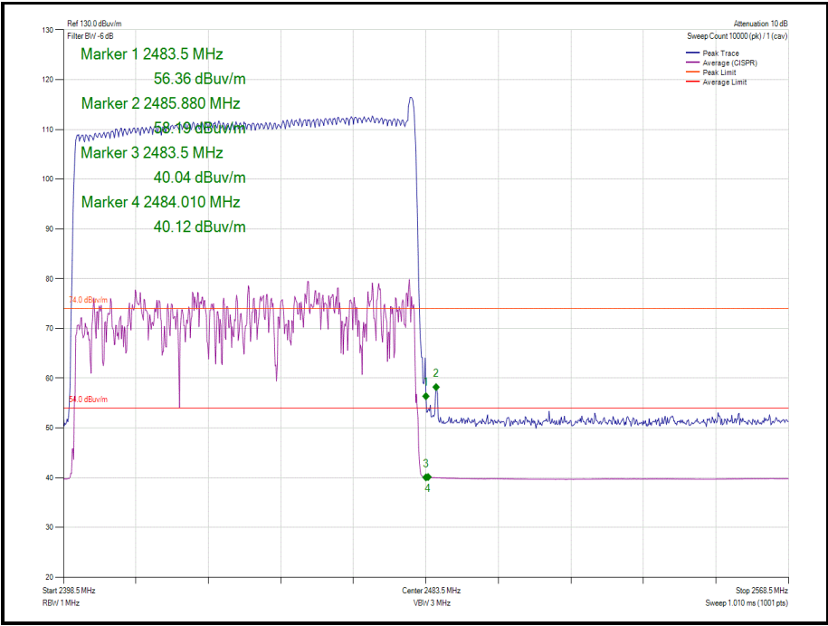
Hopping - 8-DPSK/3DH5 - 2480 MHz – Band Edge Frequency 2483.5 MHz
