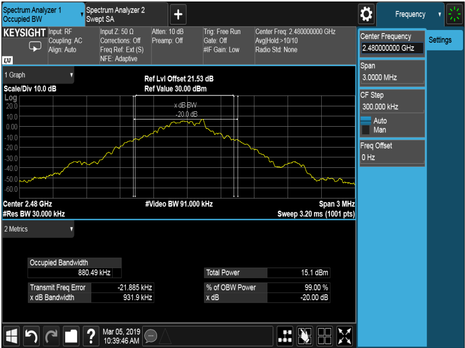
Figure 26 - 2480 MHz - GFSK
