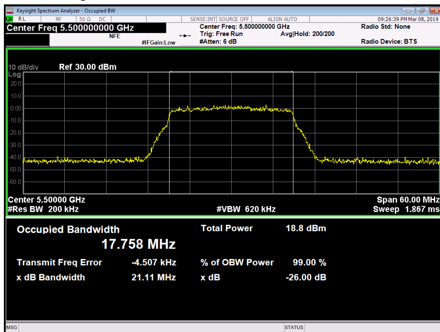
Figure 192 - 5500 MHz - 99% Occupied Bandwidth
