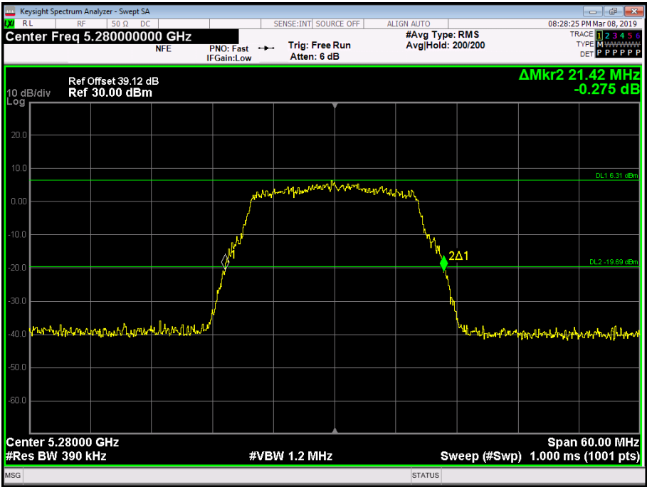
Figure 115 - 5280 MHz - 26 dB Emission Bandwidth
