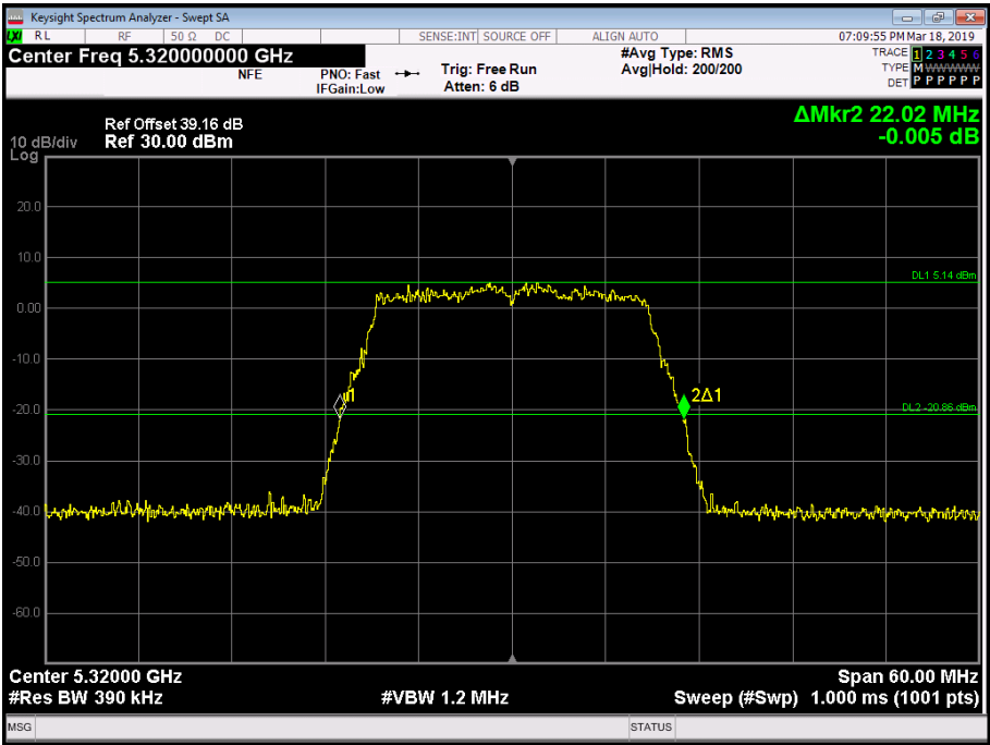
Figure 141 - 5320 MHz - 26 dB Emission Bandwidth
