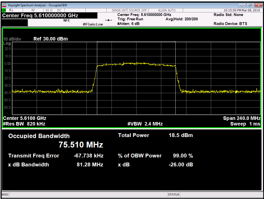
Figure 242 - 5610 MHz - 99% Occupied Bandwidth
