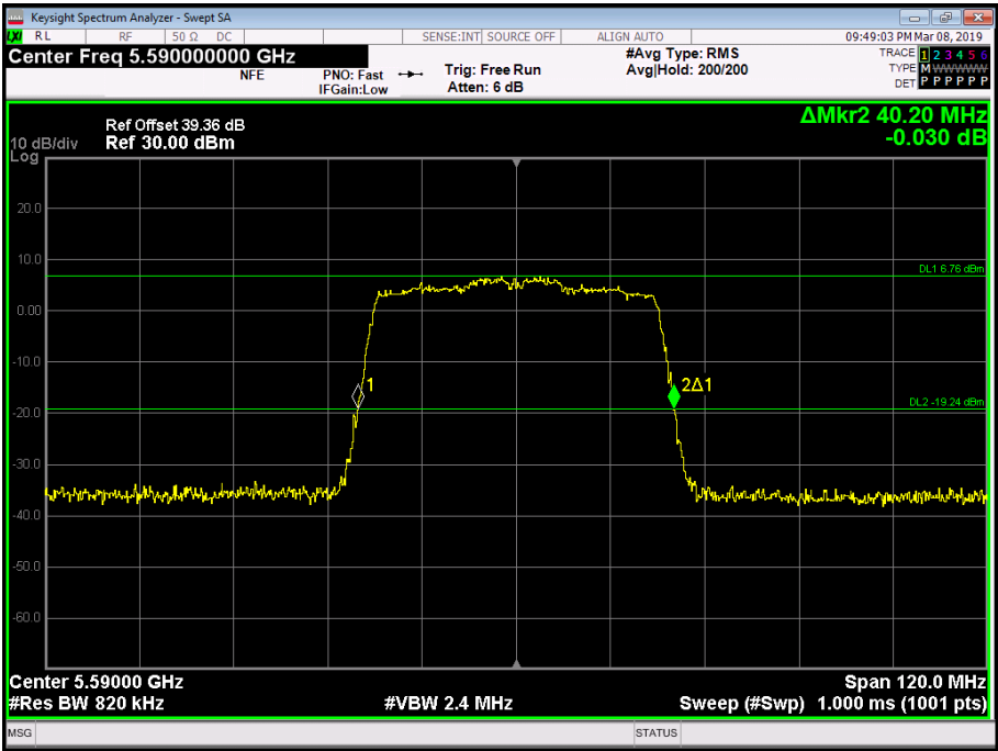
Figure 209 - 5590 MHz - 26 dB Emission Bandwidth
