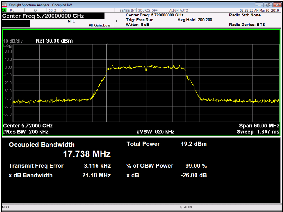
Figure 182 - 5720 MHz - 99% Occupied Bandwidth
