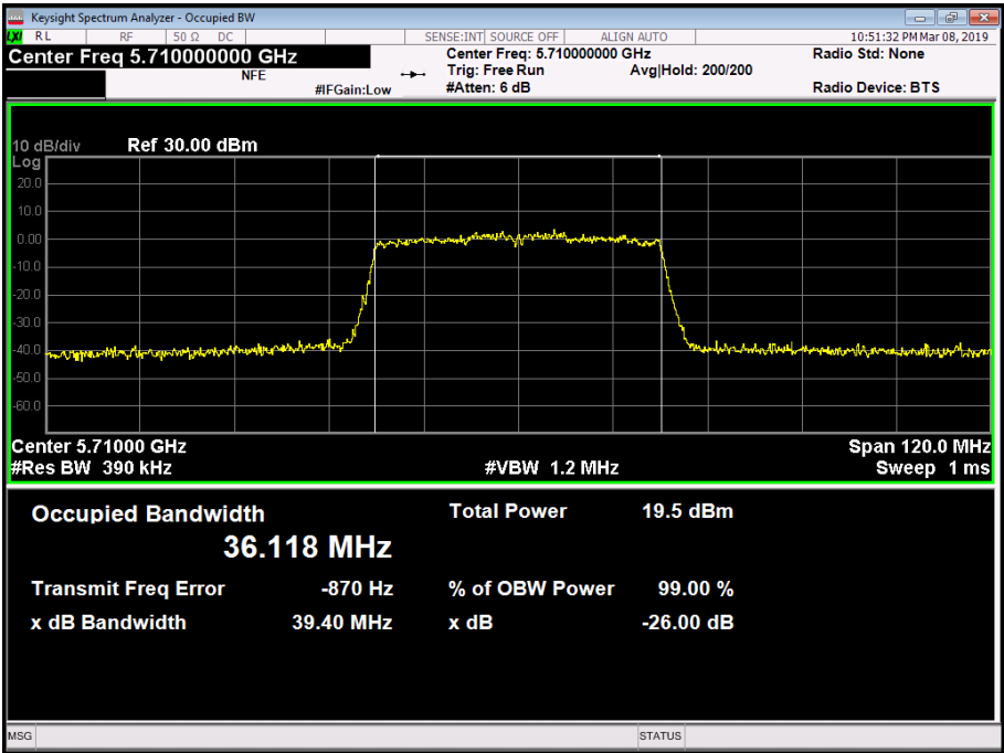
Figure 214 - 5710 MHz - 99% Occupied Bandwidth
