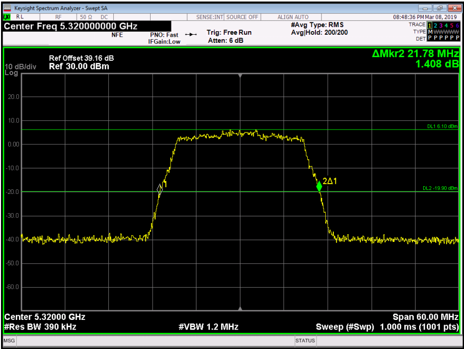
Figure 135 - 5320 MHz - 26 dB Emission Bandwidth
