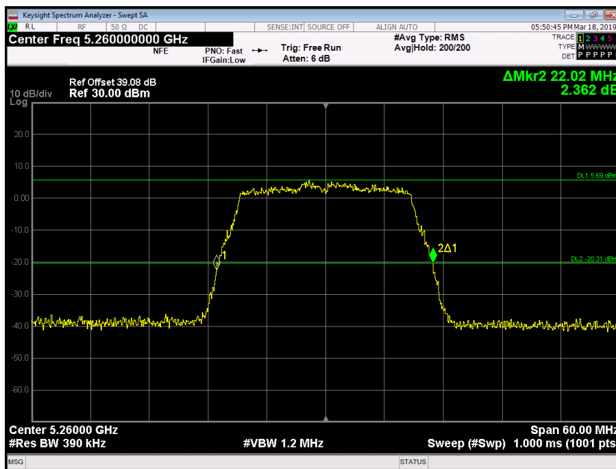
Figure 137 - 5260 MHz - 26 dB Emission Bandwidth
