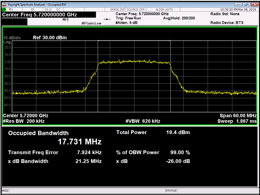
Figure 190 - 5720 MHz - 99% Occupied Bandwidth
