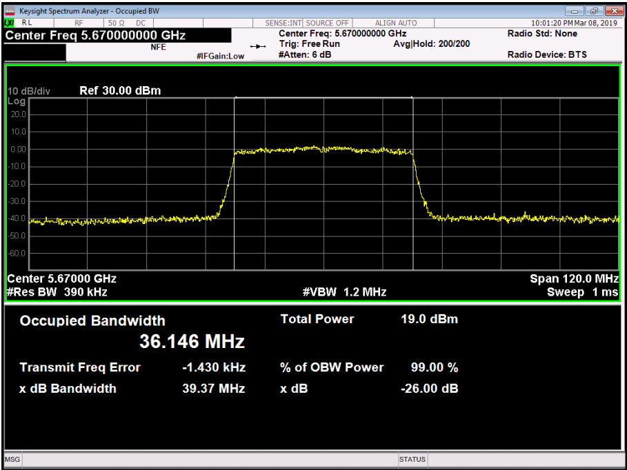
Figure 220 - 5670 MHz - 99% Occupied Bandwidth
