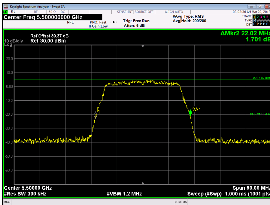
Figure 175 - 5500 MHz - 26 dB Emission Bandwidth
