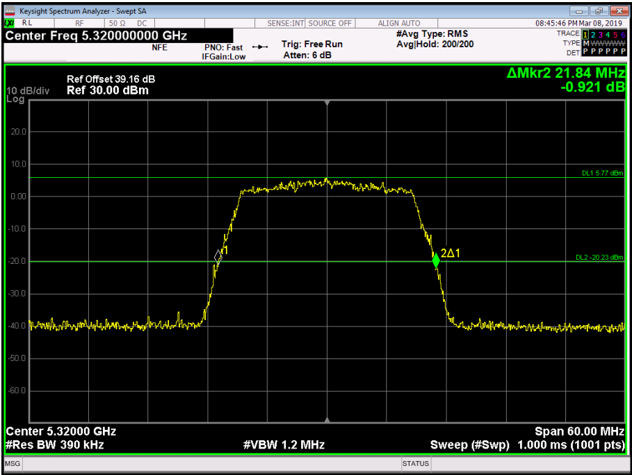
Figure 129 - 5320 MHz - 26 dB Emission Bandwidth
