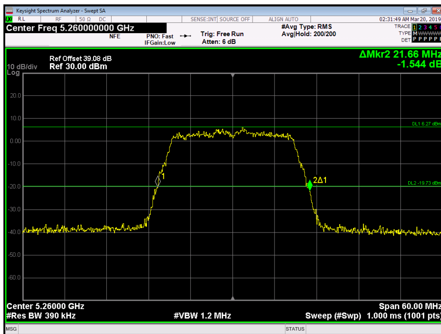
Figure 131 - 5260 MHz - 26 dB Emission Bandwidth
