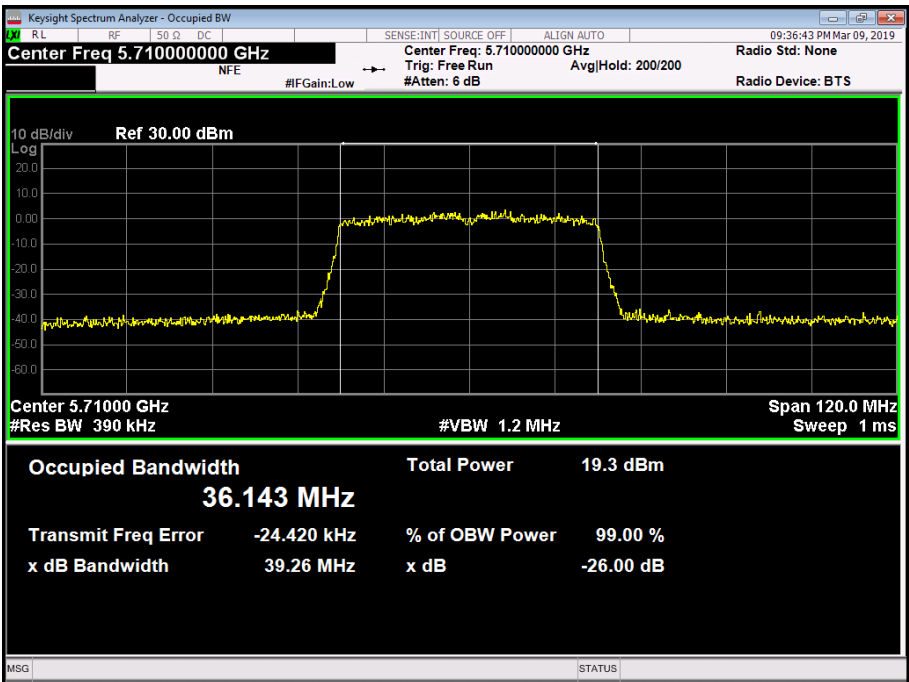
Figure 222 - 5710 MHz - 99% Occupied Bandwidth
