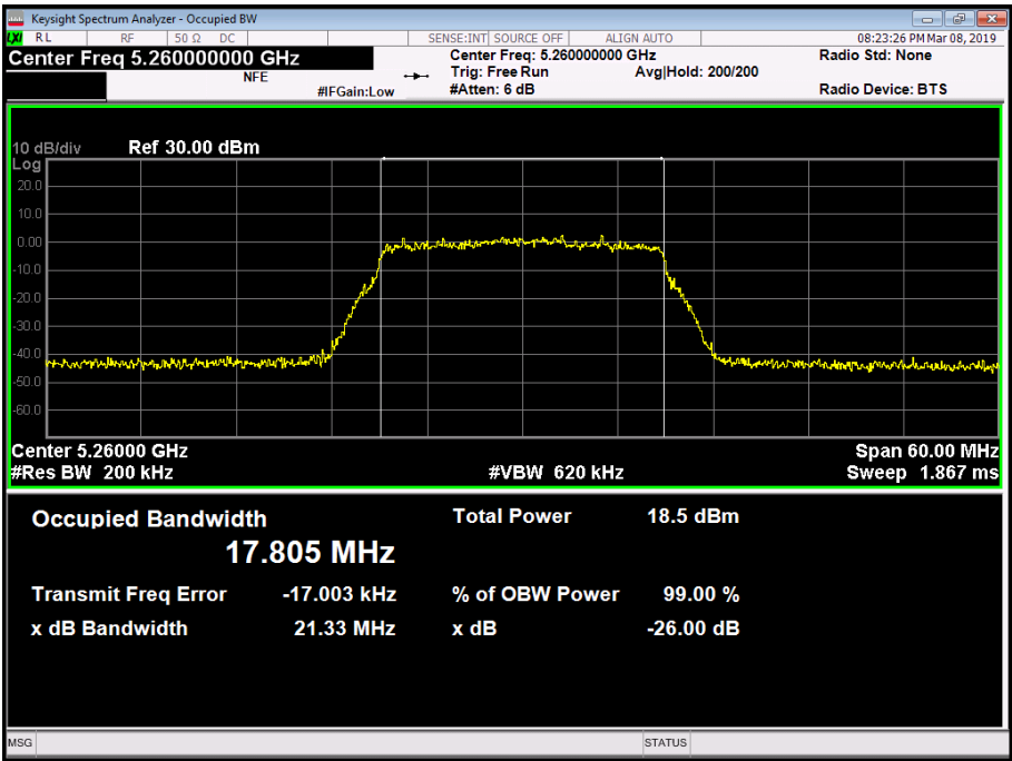
Figure 126 - 5260 MHz - 99% Occupied Bandwidth
