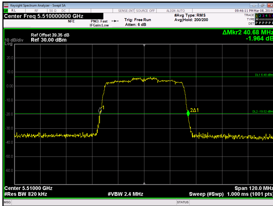
Figure 223 - 5510 MHz - 26 dB Emission Bandwidth
