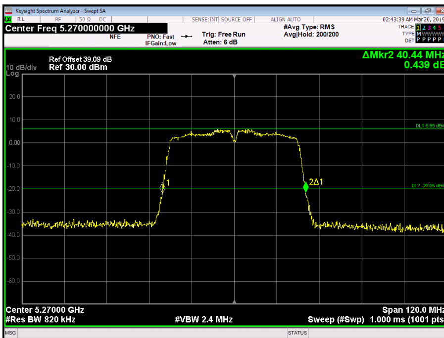
Figure 143 - 5270 MHz - 26 dB Emission Bandwidth
