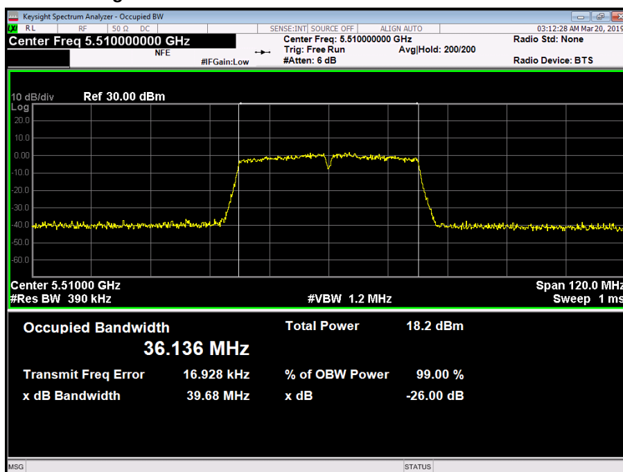
Figure 208 - 5510 MHz - 99% Occupied Bandwidth
