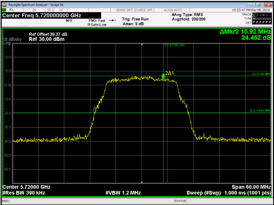
Figure 173 - 5720 MHz - 26 dB Emission Bandwidth
