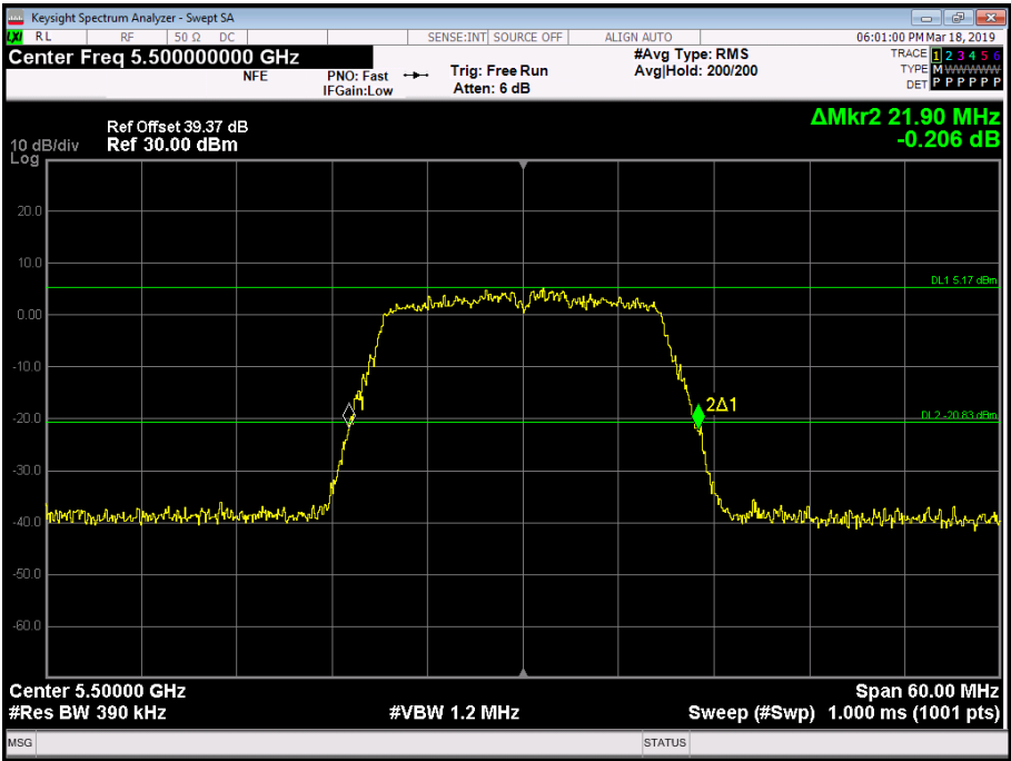
Figure 199 - 5500 MHz - 26 dB Emission Bandwidth
