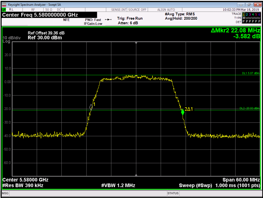
Figure 185 - 5580 MHz - 26 dB Emission Bandwidth
