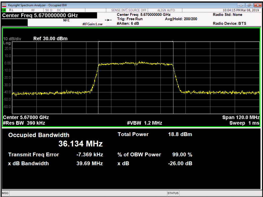
Figure 228 - 5670 MHz - 99% Occupied Bandwidth
