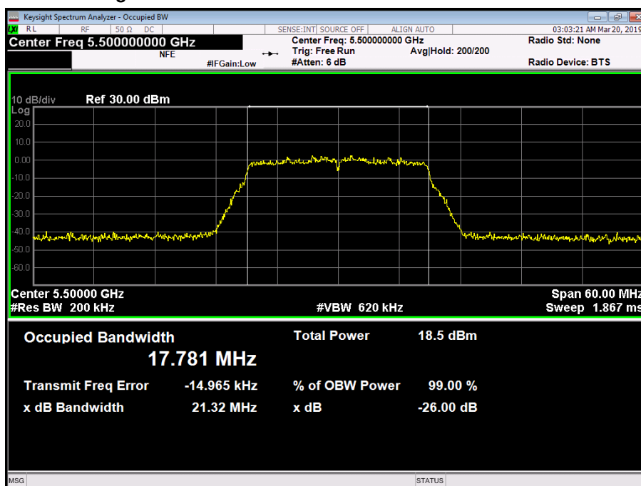
Figure 176 - 5500 MHz - 99% Occupied Bandwidth
