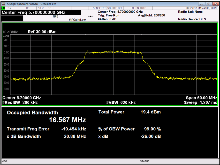
Figure 172 - 5700 MHz - 99% Occupied Bandwidth
