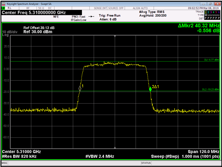
Figure 149 - 5310 MHz - 26 dB Emission Bandwidth
