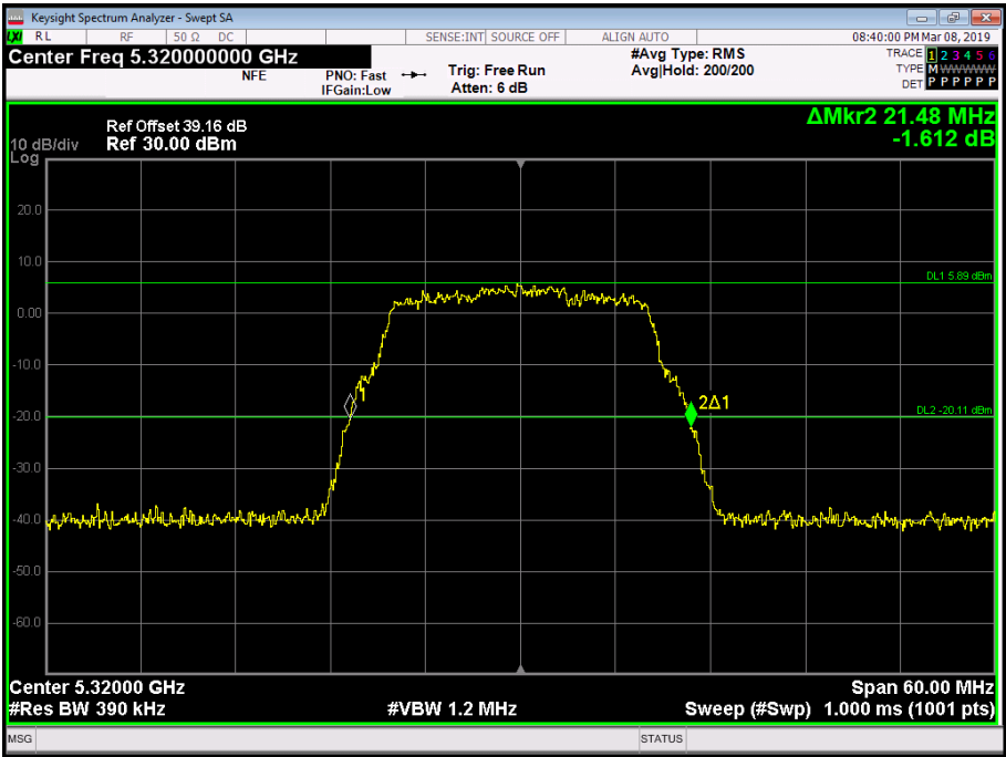
Figure 117 - 5320 MHz - 26 dB Emission Bandwidth
