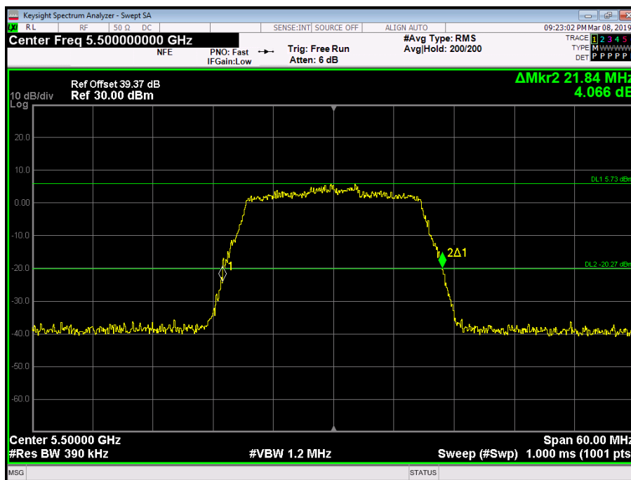
Figure 183 - 5500 MHz - 26 dB Emission Bandwidth
