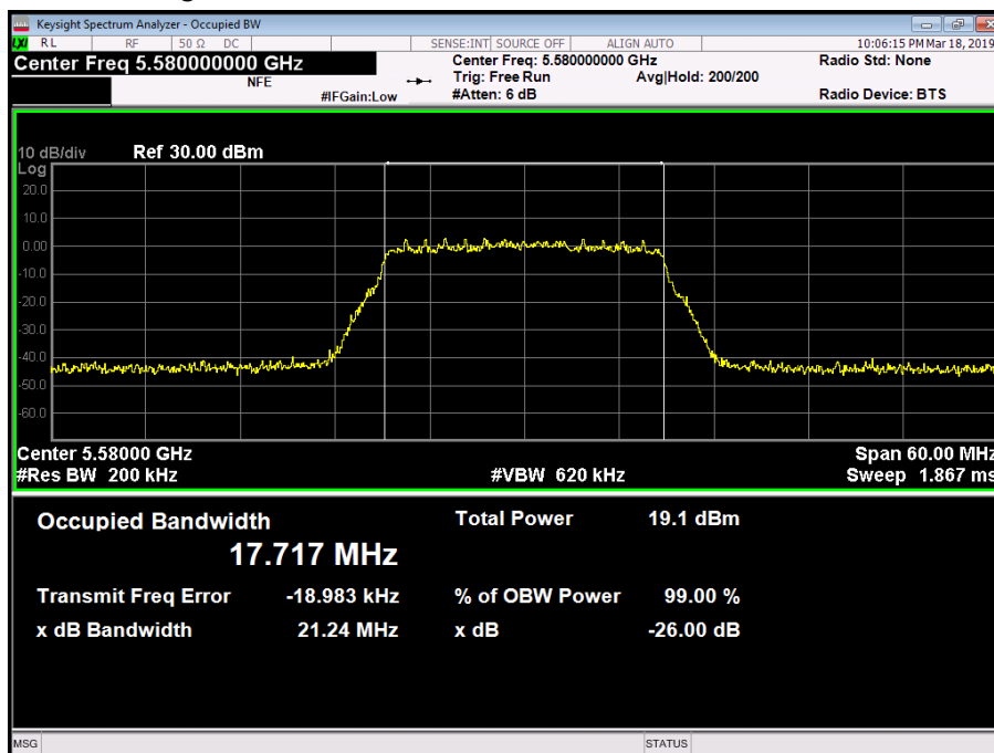
Figure 194 - 5580 MHz - 99% Occupied Bandwidth
