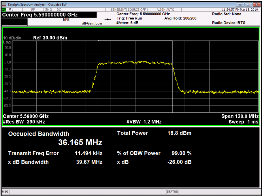
Figure 226 - 5590 MHz - 99% Occupied Bandwidth
