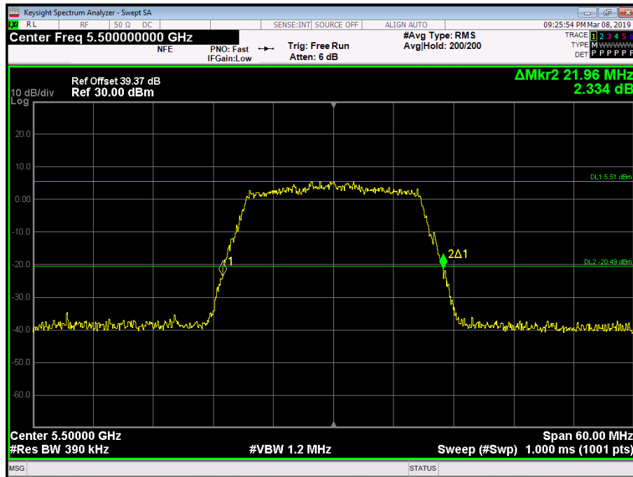
Figure 191 - 5500 MHz - 26 dB Emission Bandwidth
