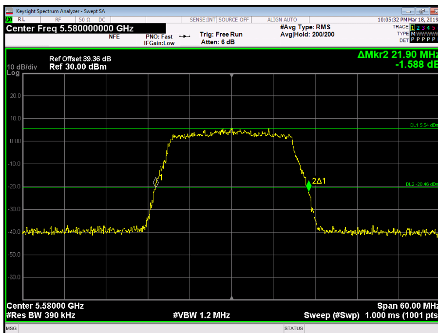
Figure 193 - 5580 MHz - 26 dB Emission Bandwidth
