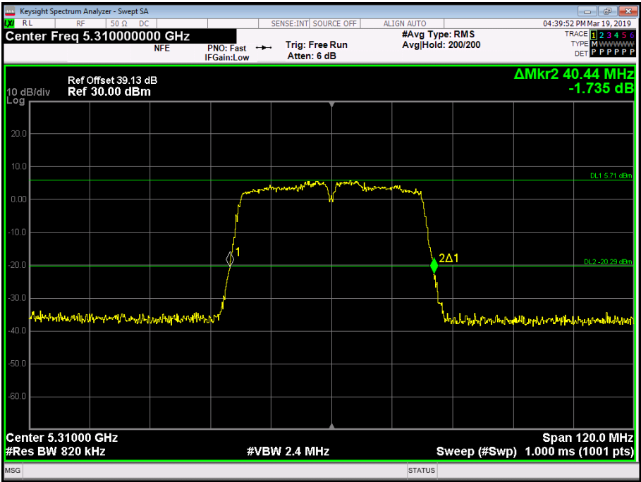
Figure 157 - 5310 MHz - 26 dB Emission Bandwidth
