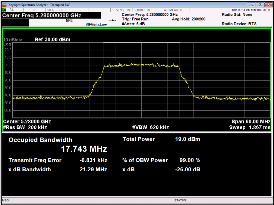
Figure 128 - 5280 MHz - 99% Occupied Bandwidth
