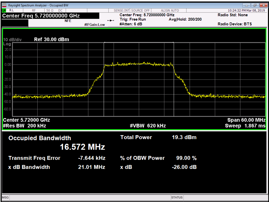
Figure 174 - 5720 MHz - 99% Occupied Bandwidth
