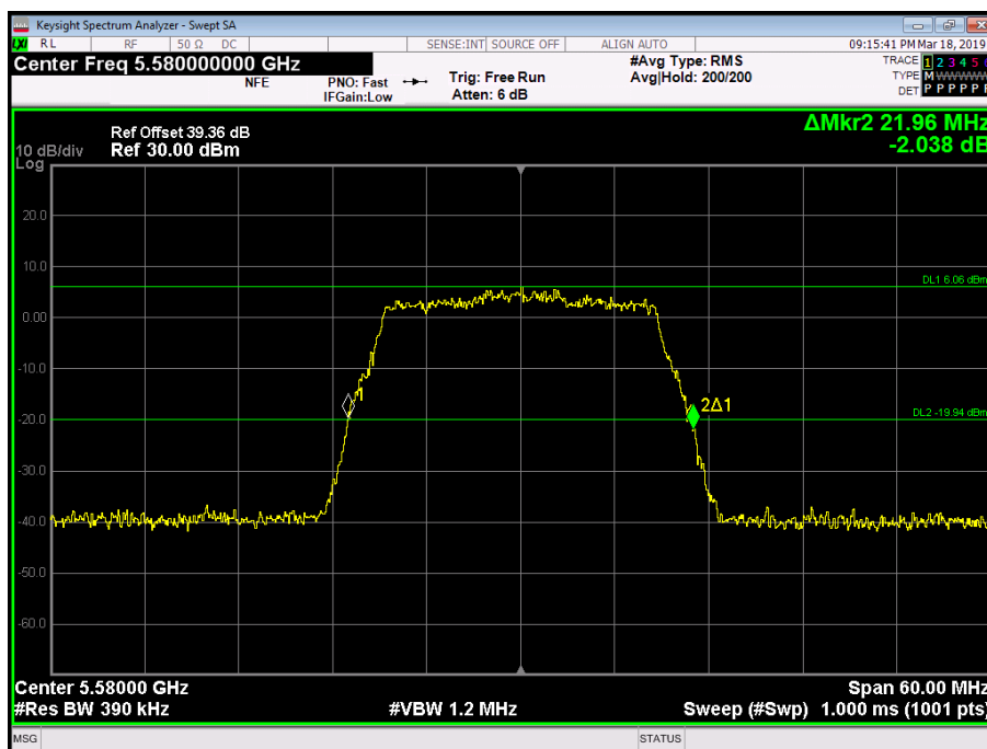
Figure 177 - 5580 MHz - 26 dB Emission Bandwidth
