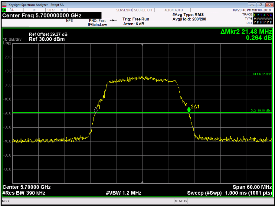
Figure 171 - 5700 MHz - 26 dB Emission Bandwidth
