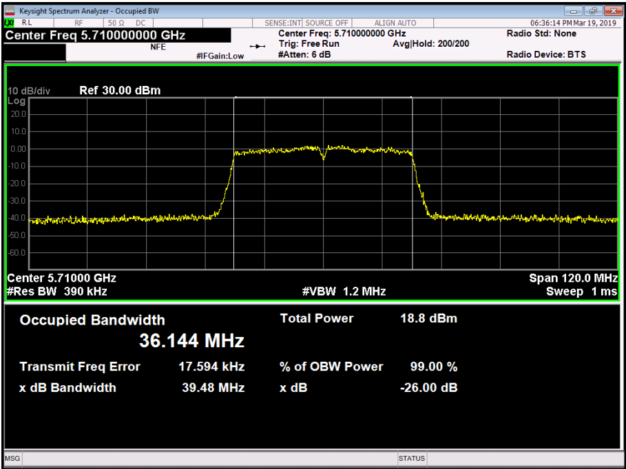
Figure 238 - 5710 MHz - 99% Occupied Bandwidth
