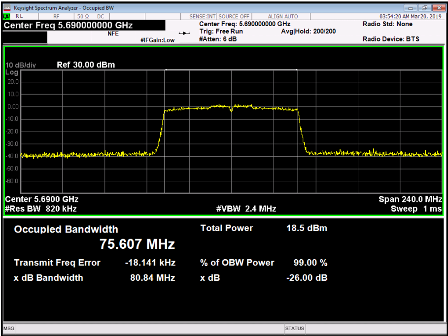
Figure 250 - 5690 MHz - 99% Occupied Bandwidth
