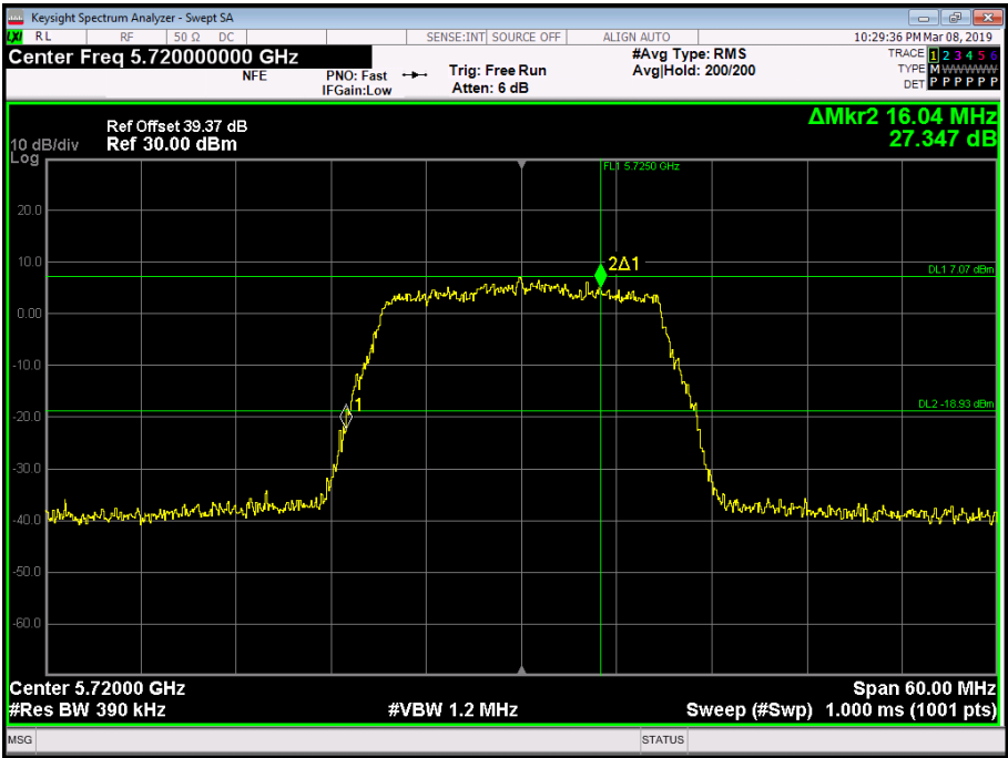
Figure 189 - 5720 MHz - 26 dB Emission Bandwidth
