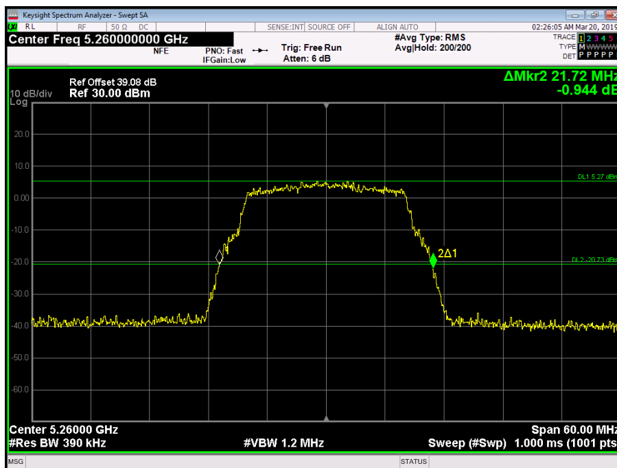
Figure 113 - 5260 MHz - 26 dB Emission Bandwidth
