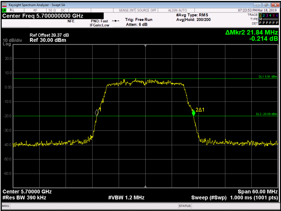
Figure 203 - 5700 MHz - 26 dB Emission Bandwidth
