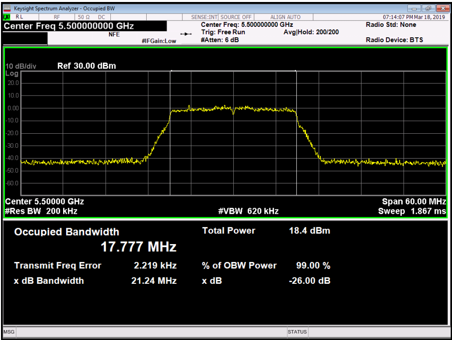
Figure 200 - 5500 MHz - 99% Occupied Bandwidth
