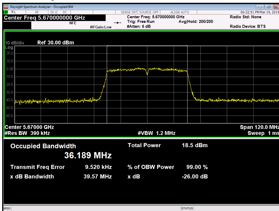
Figure 236 - 5670 MHz - 99% Occupied Bandwidth
