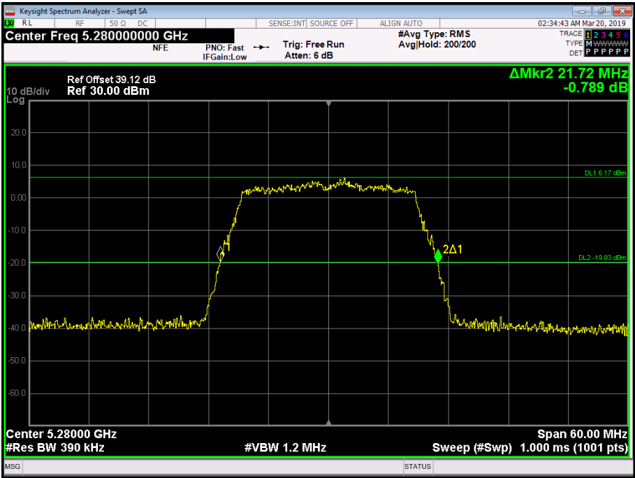
Figure 121 - 5280 MHz - 26 dB Emission Bandwidth
