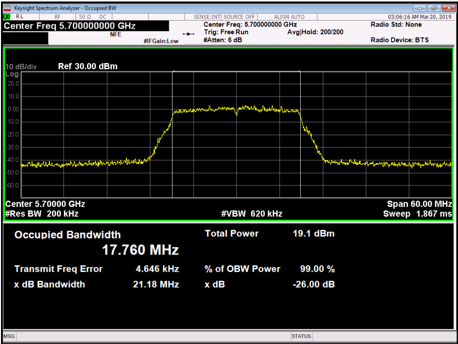
Figure 180 - 5700 MHz - 99% Occupied Bandwidth
