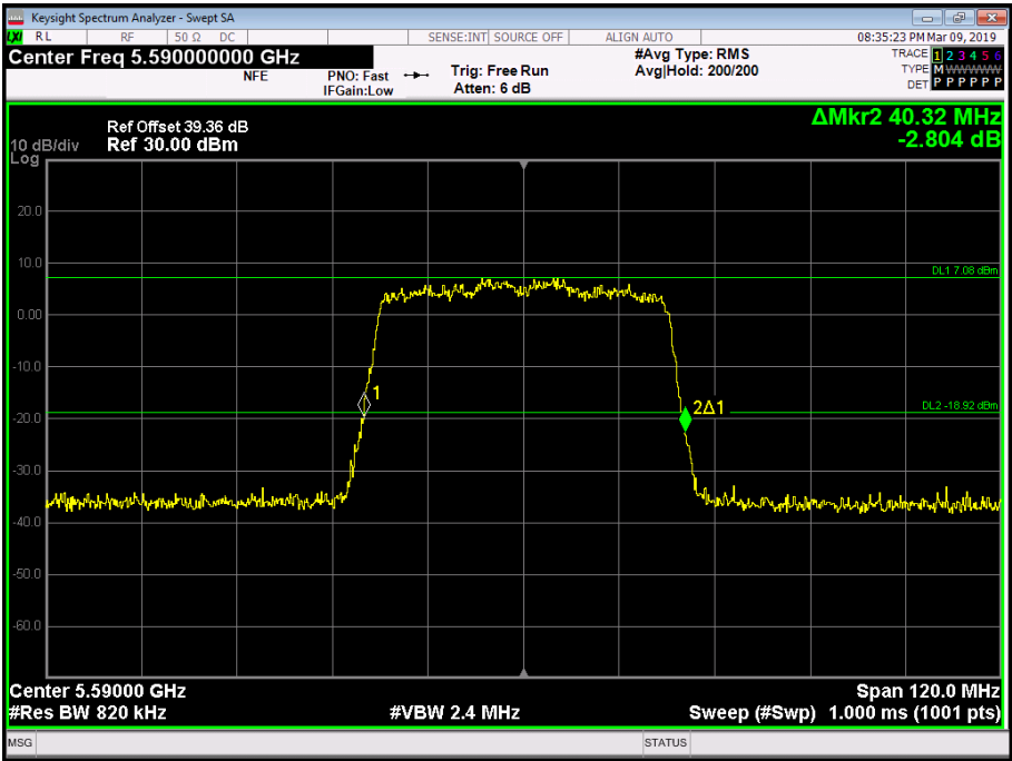
Figure 225 - 5590 MHz - 26 dB Emission Bandwidth
