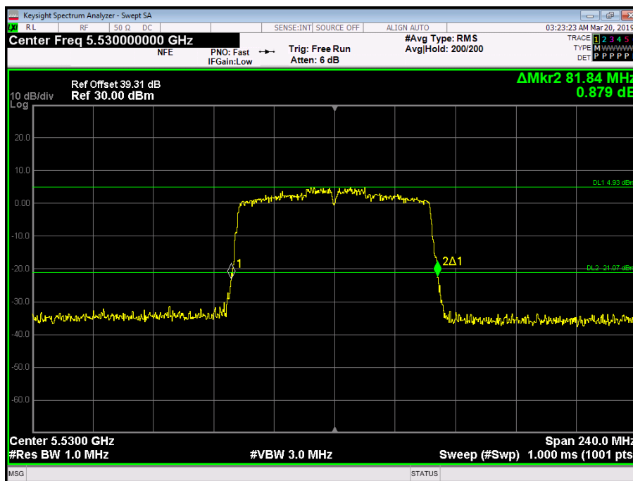
Figure 245 - 5530 MHz - 26 dB Emission Bandwidth
