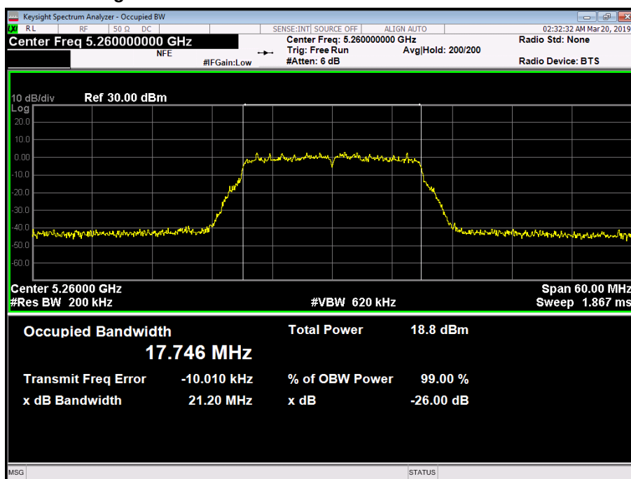
Figure 132 - 5260 MHz - 99% Occupied Bandwidth
