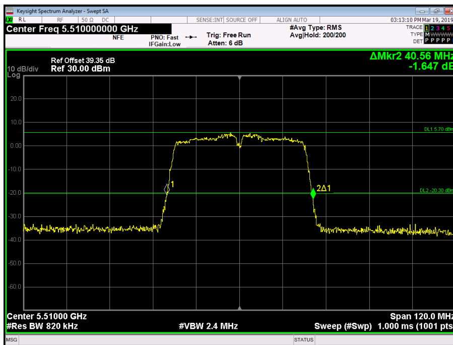
Figure 231 - 5510 MHz - 26 dB Emission Bandwidth
