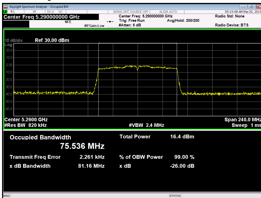
Figure 166 - 5290 MHz - 99% Occupied Bandwidth
