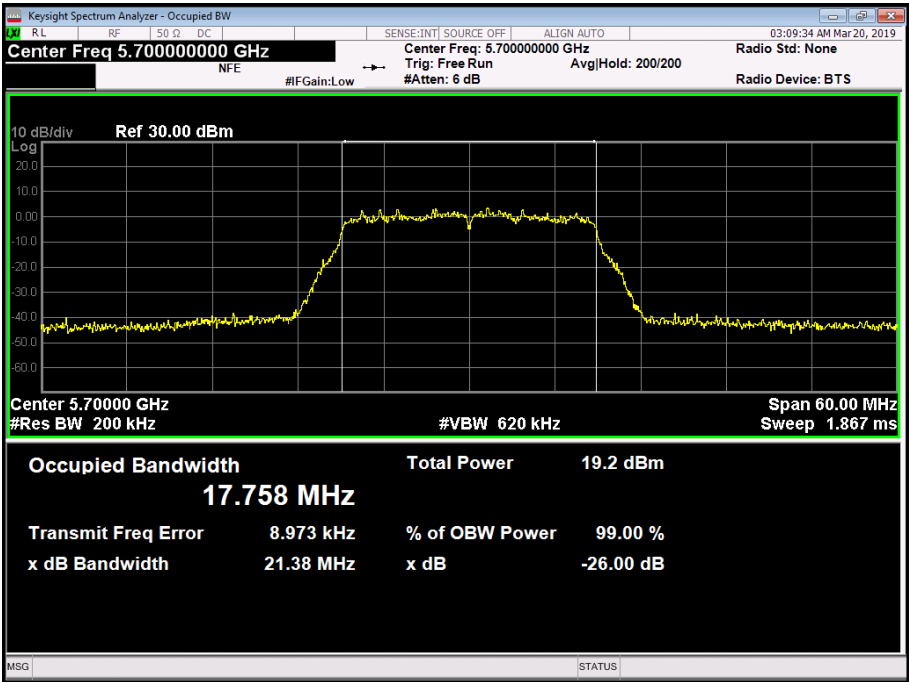
Figure 188 - 5700 MHz - 99% Occupied Bandwidth
