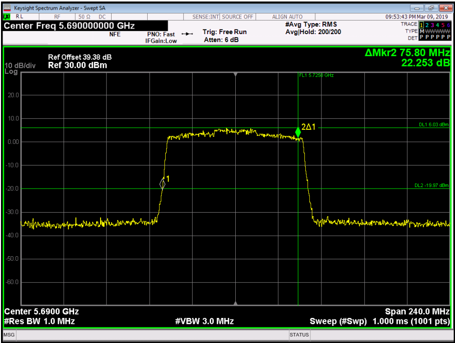
Figure 243 - 5690 MHz - 26 dB Emission Bandwidth
