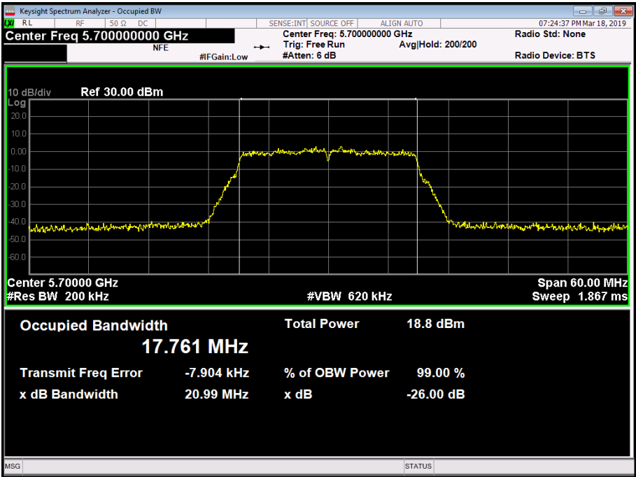
Figure 204 - 5700 MHz - 99% Occupied Bandwidth
