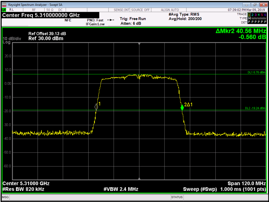
Figure 145 - 5310 MHz - 26 dB Emission Bandwidth
