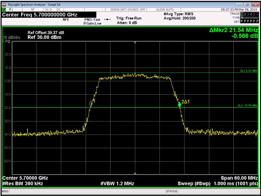
Figure 195 - 5700 MHz - 26 dB Emission Bandwidth
