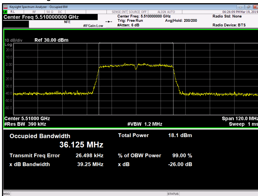
Figure 232 - 5510 MHz - 99% Occupied Bandwidth
