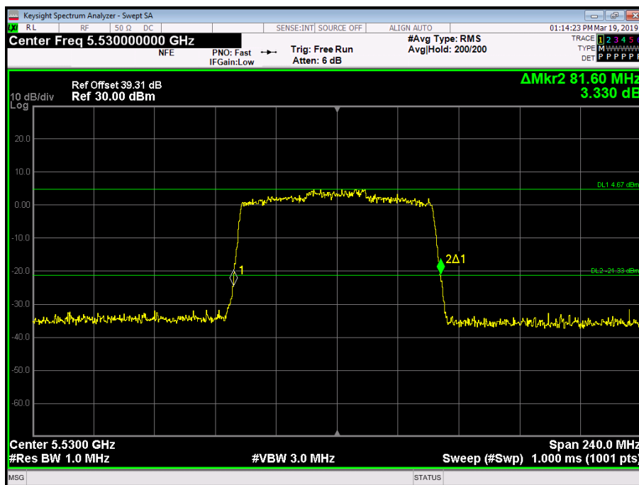
Figure 239 - 5530 MHz - 26 dB Emission Bandwidth
