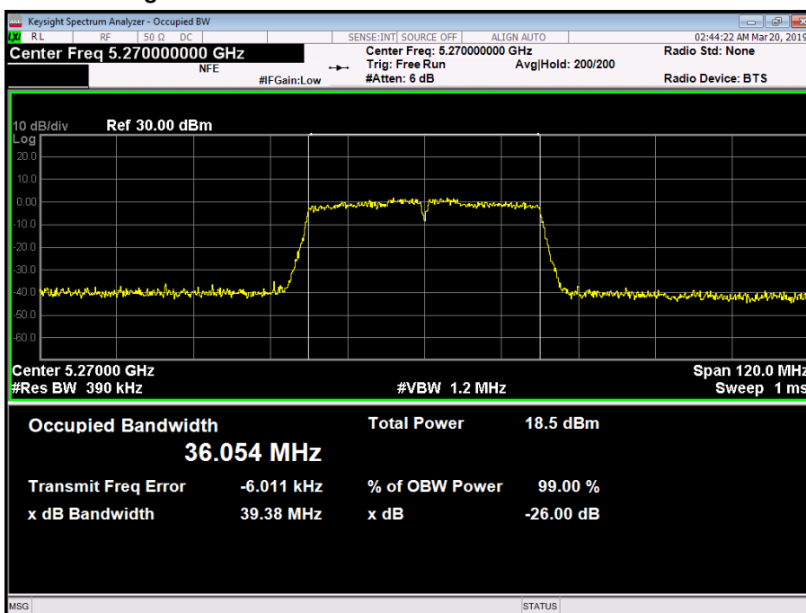
Figure 144 - 5270 MHz - 99% Occupied Bandwidth
