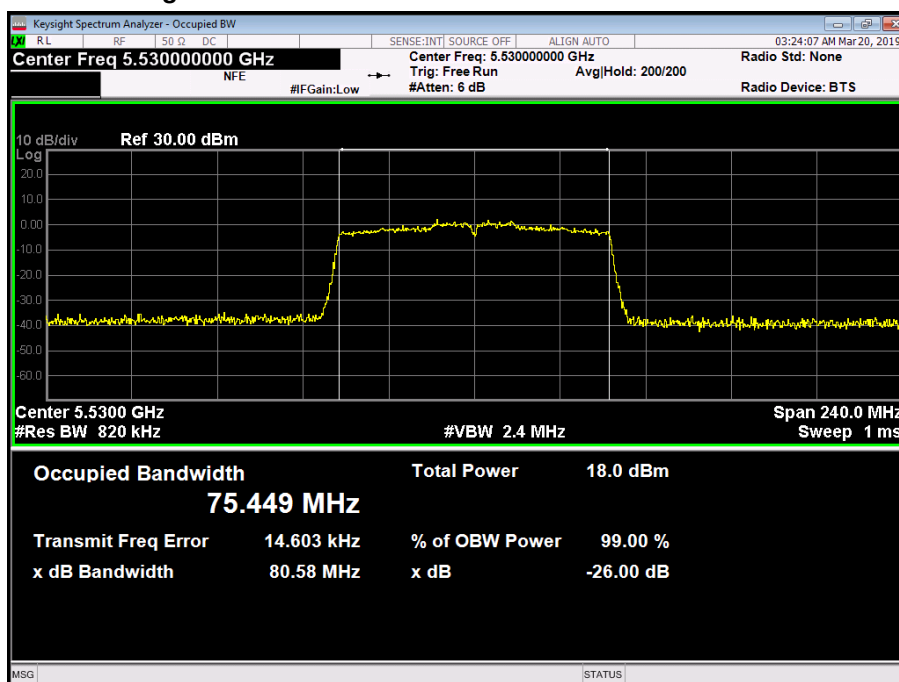
Figure 246 - 5530 MHz - 99% Occupied Bandwidth
