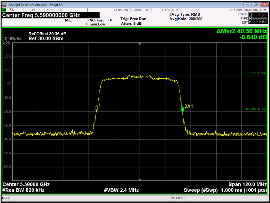
Figure 217 - 5590 MHz - 26 dB Emission Bandwidth
