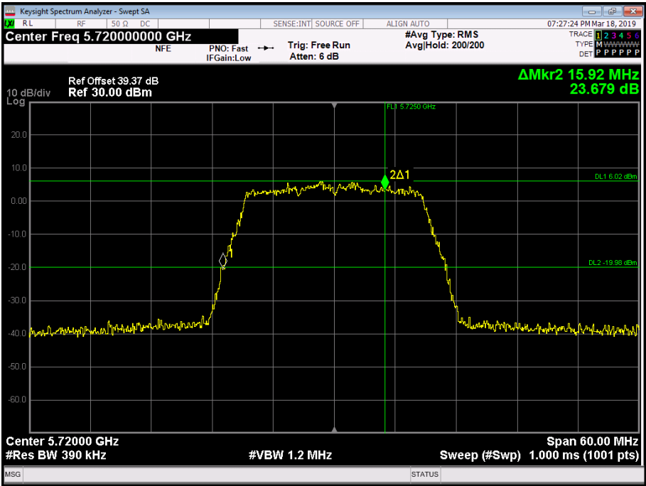
Figure 205 - 5720 MHz - 26 dB Emission Bandwidth
