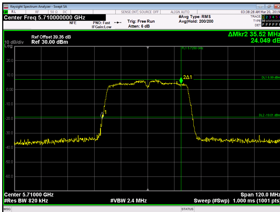
Figure 229 - 5710 MHz - 26 dB Emission Bandwidth
