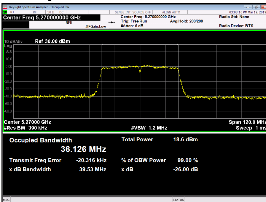
Figure 156 - 5270 MHz - 99% Occupied Bandwidth
