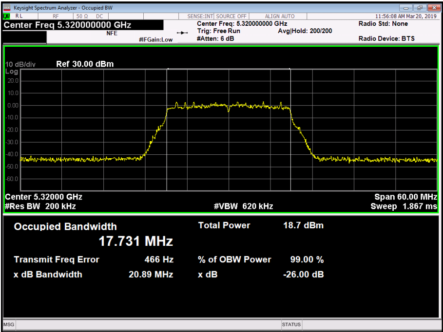
Figure 136 - 5320 MHz - 99% Occupied Bandwidth
