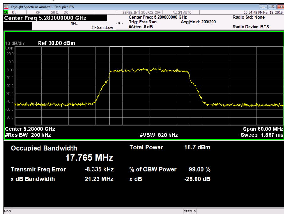
Figure 140 - 5280 MHz - 99% Occupied Bandwidth
