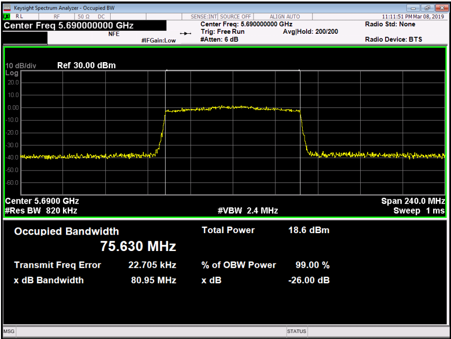
Figure 244 - 5690 MHz - 99% Occupied Bandwidth
