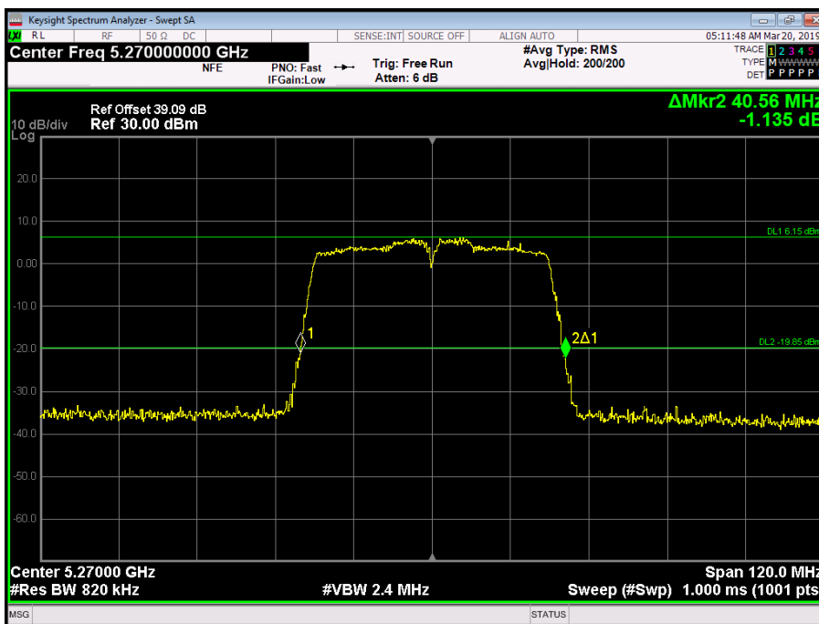
Figure 155 - 5270 MHz - 26 dB Emission Bandwidth
