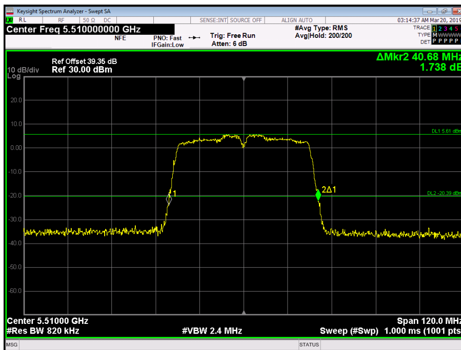
Figure 215 - 5510 MHz - 26 dB Emission Bandwidth
