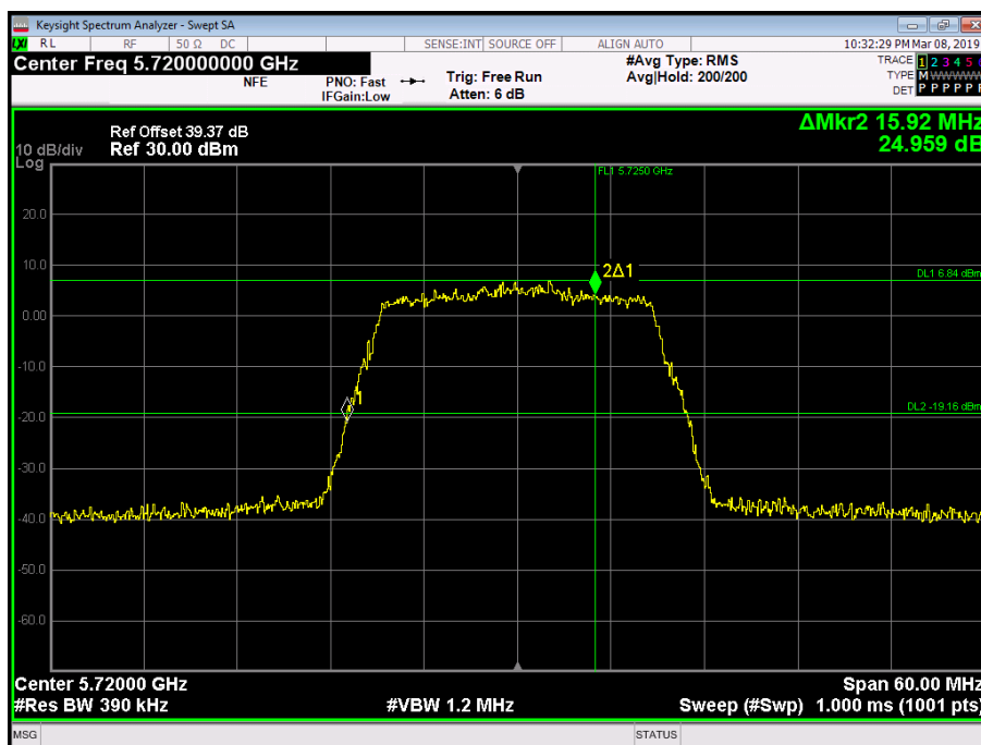
Figure 197 - 5720 MHz - 26 dB Emission Bandwidth
