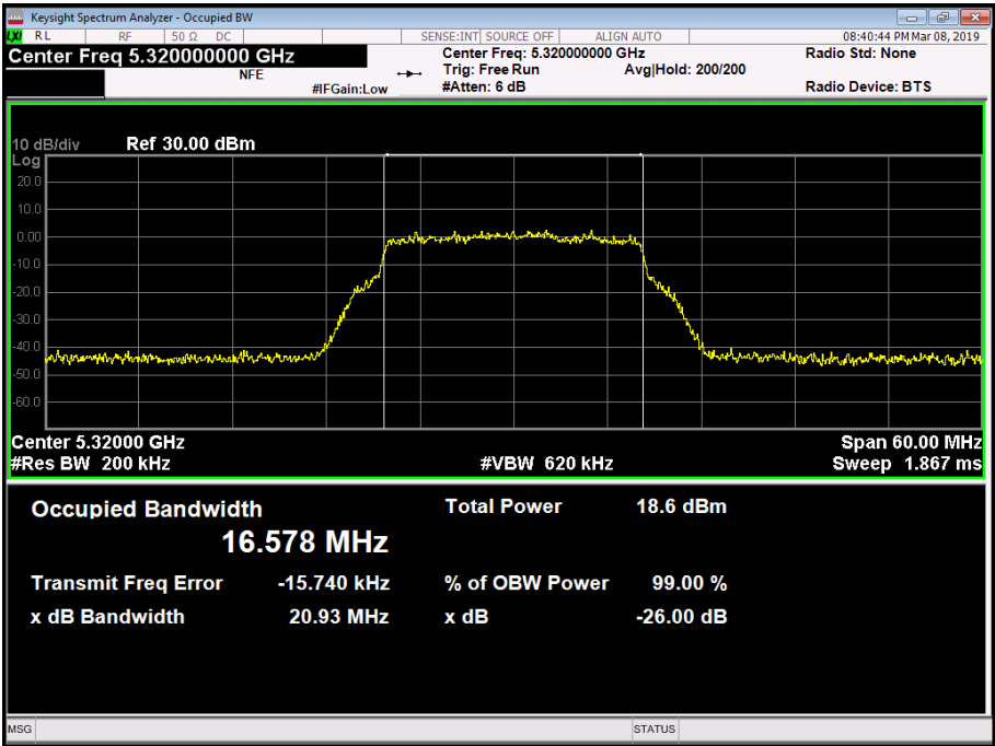
Figure 118 - 5320 MHz - 99% Occupied Bandwidth
