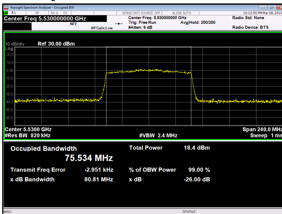
Figure 252 - 5530 MHz - 99% Occupied Bandwidth
