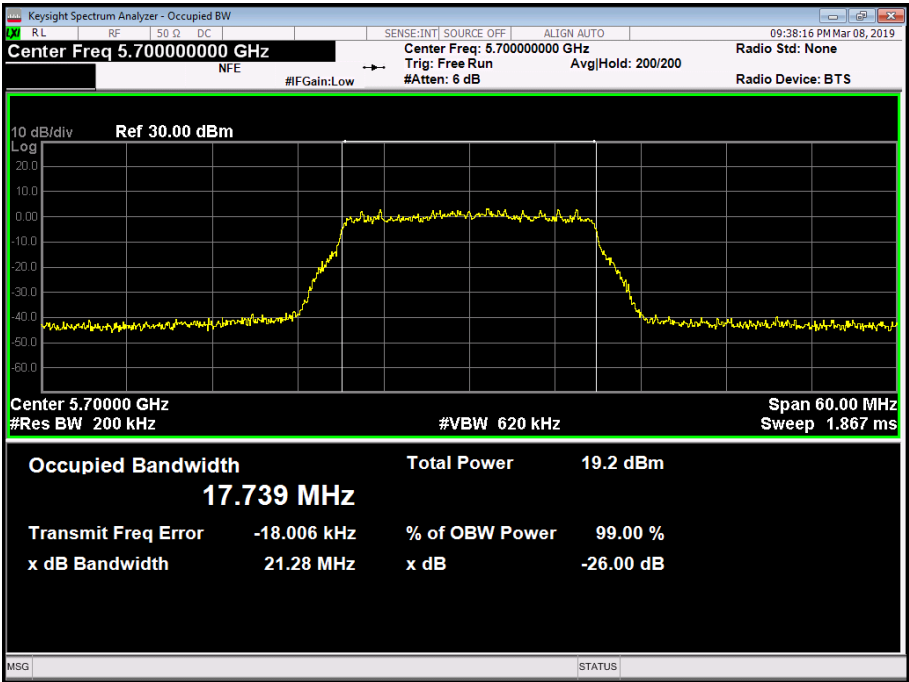
Figure 196 - 5700 MHz - 99% Occupied Bandwidth
