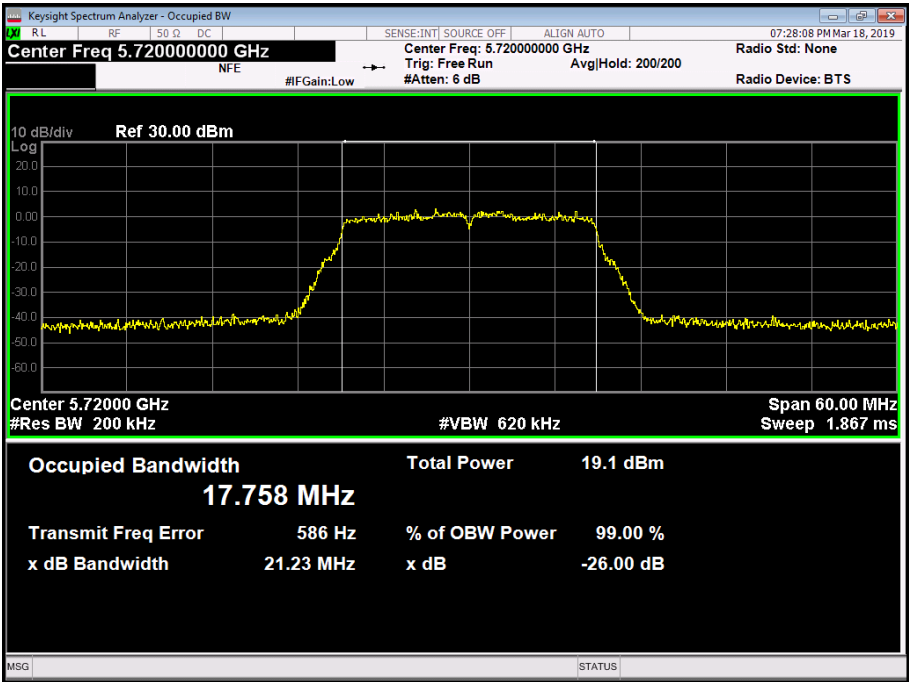
Figure 206 - 5720 MHz - 99% Occupied Bandwidth
