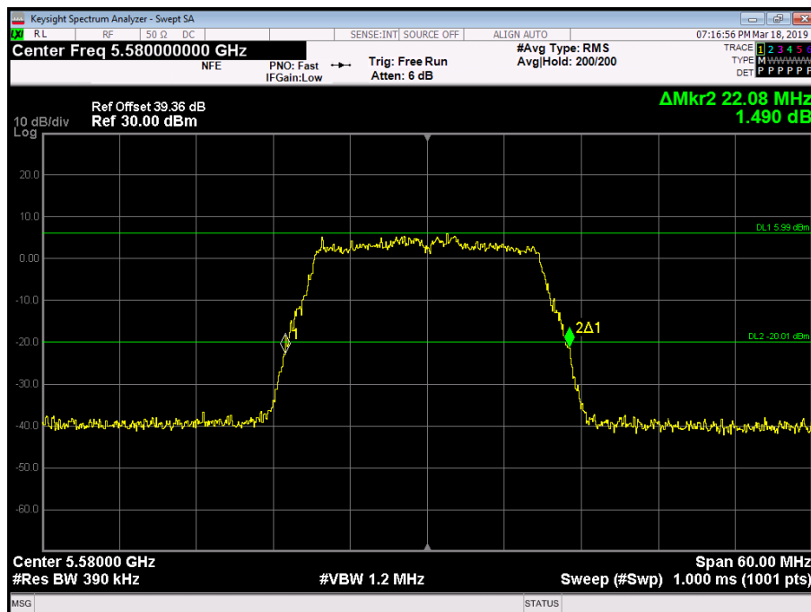
Figure 201 - 5580 MHz - 26 dB Emission Bandwidth
