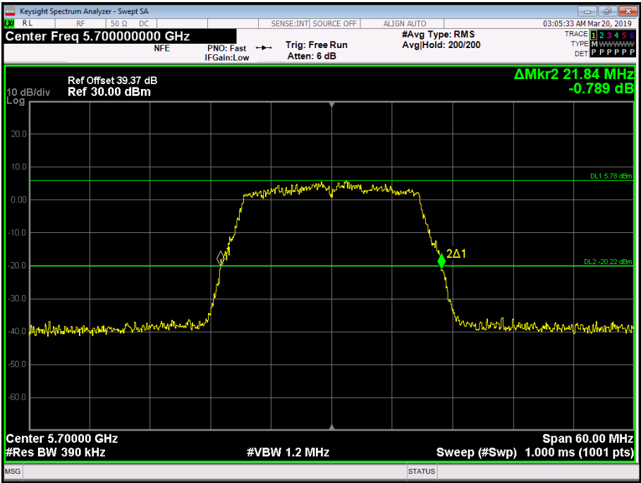
Figure 179 - 5700 MHz - 26 dB Emission Bandwidth
