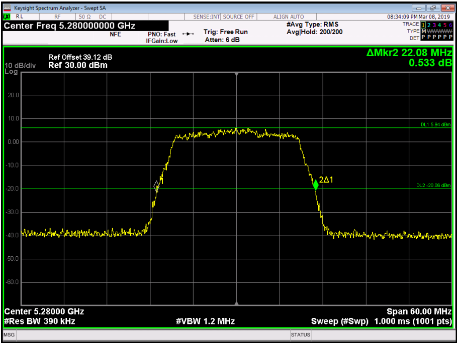
Figure 127 - 5280 MHz - 26 dB Emission Bandwidth
