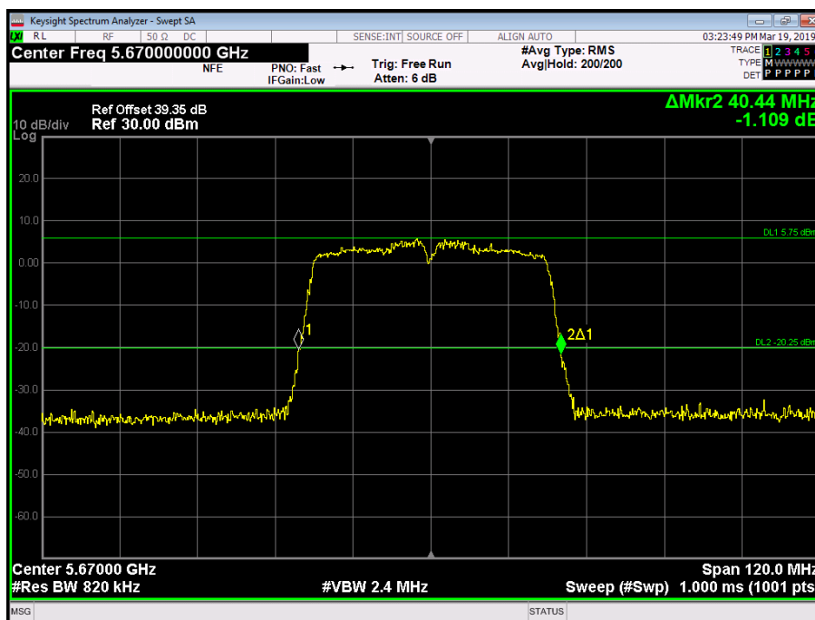
Figure 235 - 5670 MHz - 26 dB Emission Bandwidth
