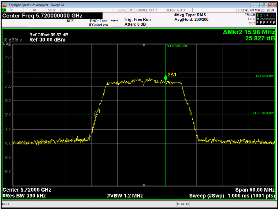
Figure 181 - 5720 MHz - 26 dB Emission Bandwidth
