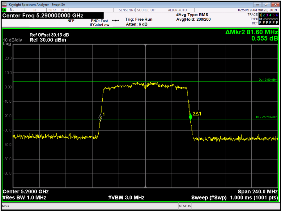
Figure 163 - 5290 MHz - 26 dB Emission Bandwidth
