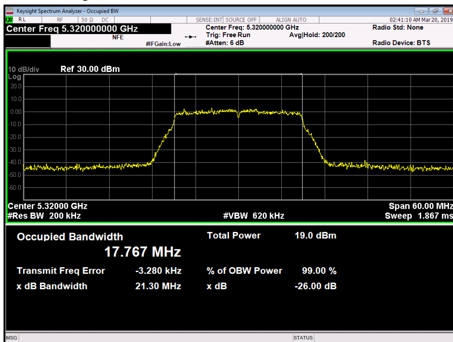
Figure 124 - 5320 MHz - 99% Occupied Bandwidth
