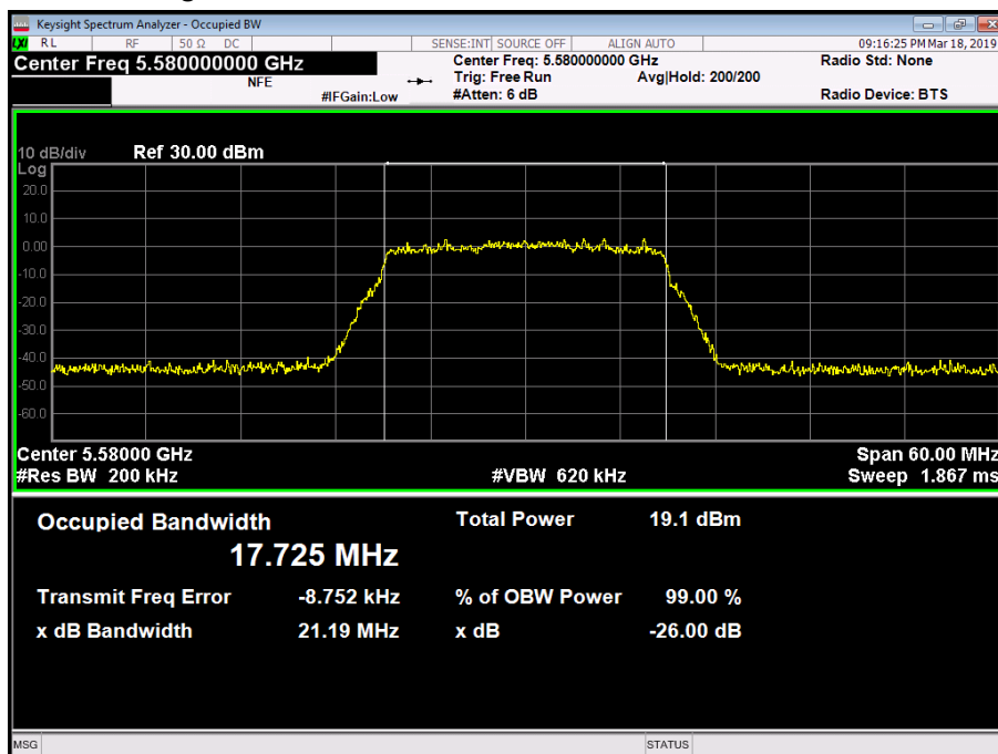
Figure 178 - 5580 MHz - 99% Occupied Bandwidth
