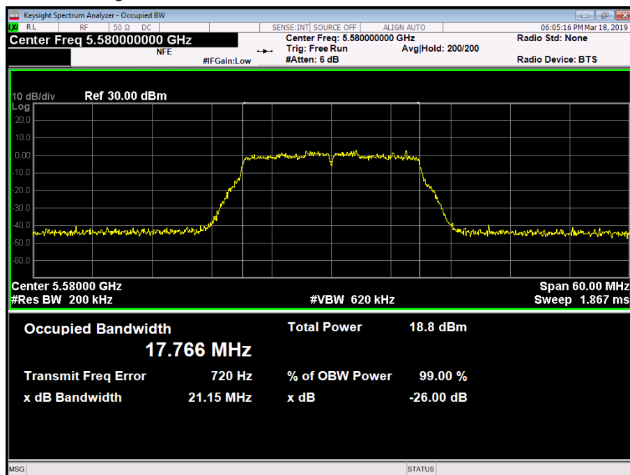
Figure 202 - 5580 MHz - 99% Occupied Bandwidth
