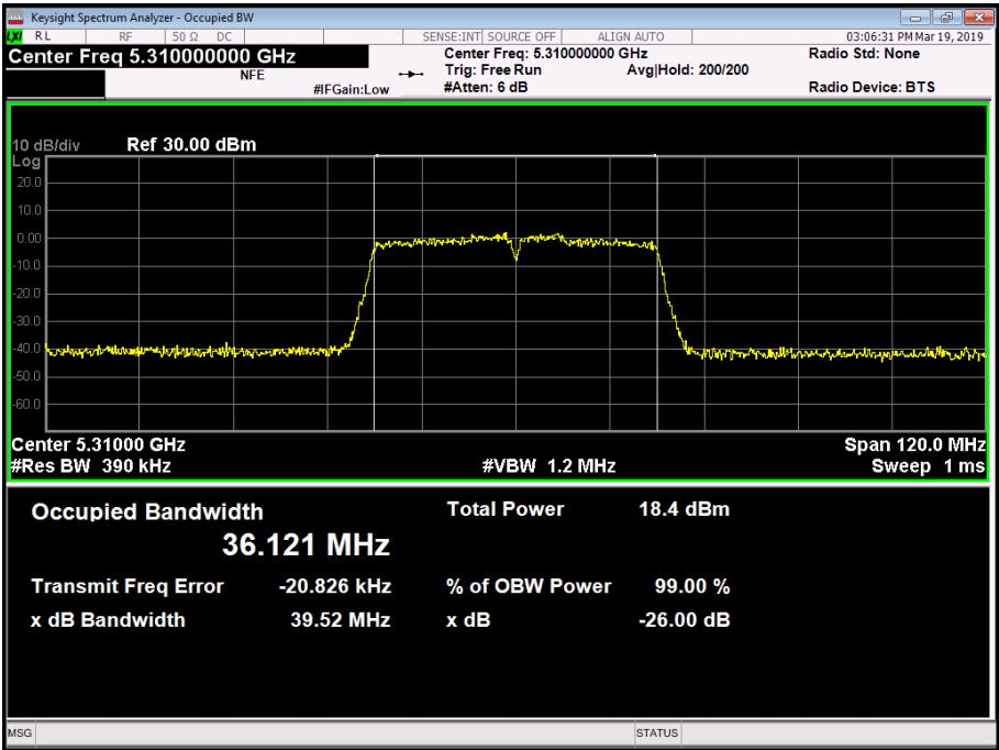
Figure 158 - 5310 MHz - 99% Occupied Bandwidth
