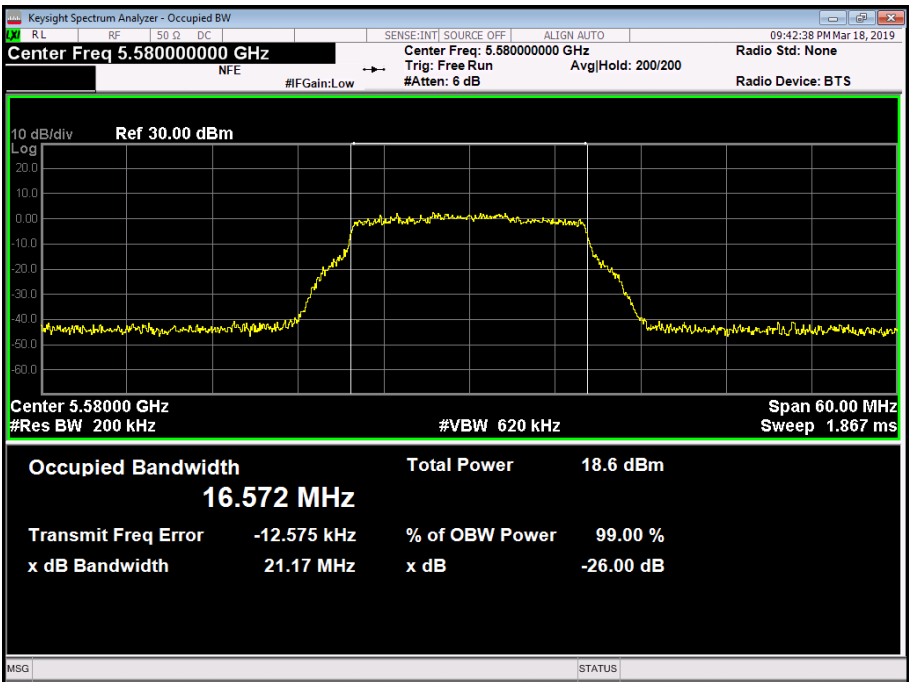
Figure 170 - 5580 MHz - 99% Occupied Bandwidth
