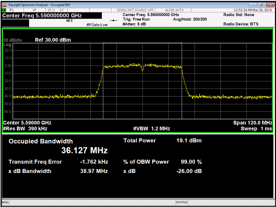
Figure 218 - 5590 MHz - 99% Occupied Bandwidth
