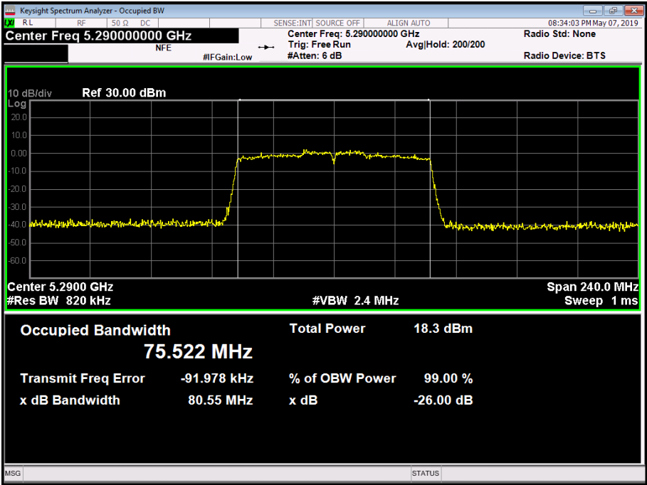
Figure 162 - 5290 MHz - 99% Occupied Bandwidth 802.11ac / VHT80 MCS0x2 / MIMO SDM / Cores 0+1
