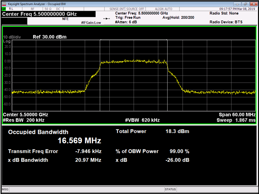
Figure 168 - 5500 MHz - 99% Occupied Bandwidth
