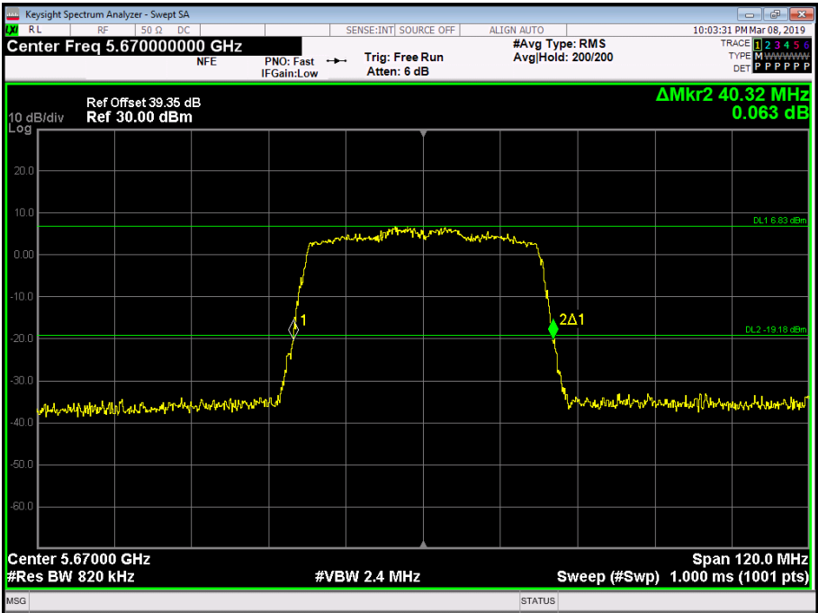
Figure 227 - 5670 MHz - 26 dB Emission Bandwidth
