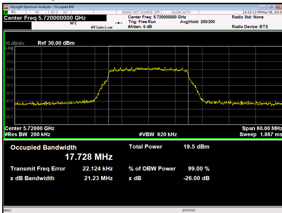
Figure 198 - 5720 MHz - 99% Occupied Bandwidth
