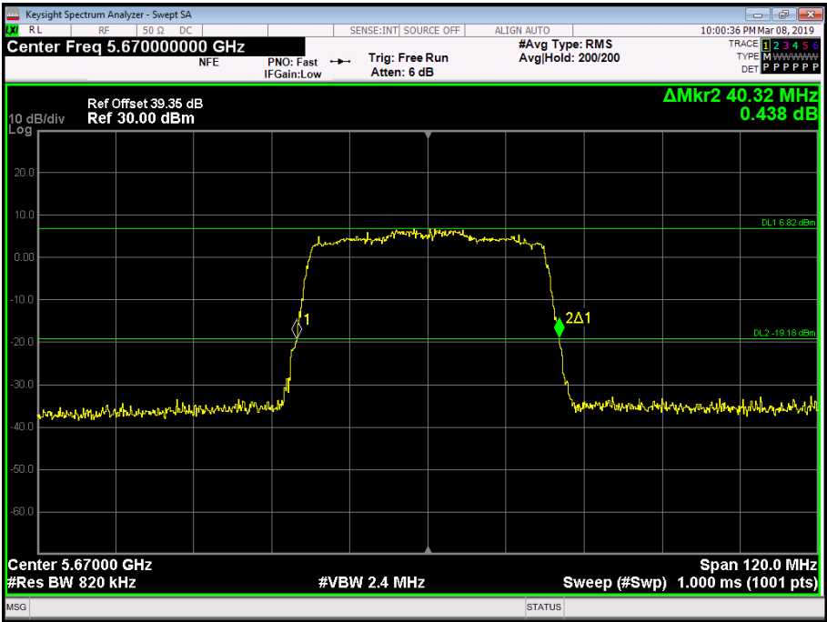
Figure 219 - 5670 MHz - 26 dB Emission Bandwidth
