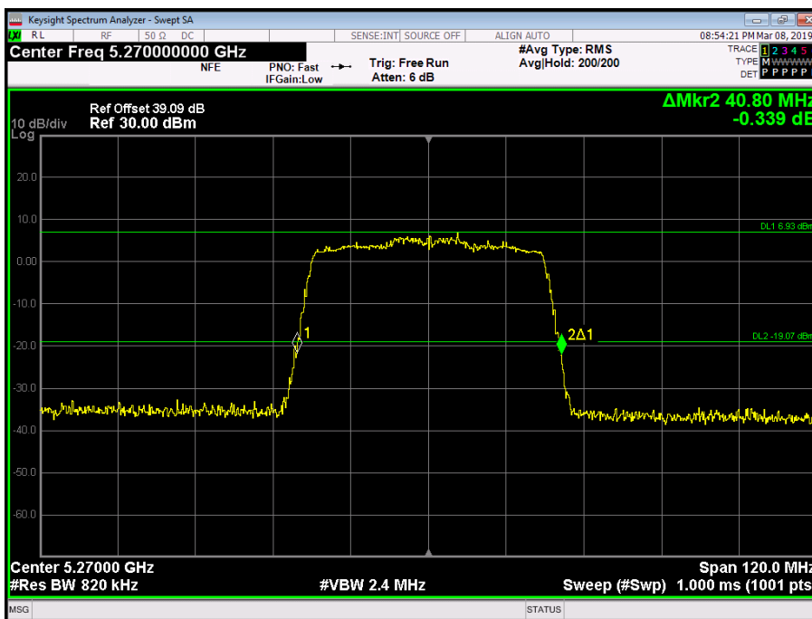
Figure 147 - 5270 MHz - 26 dB Emission Bandwidth
