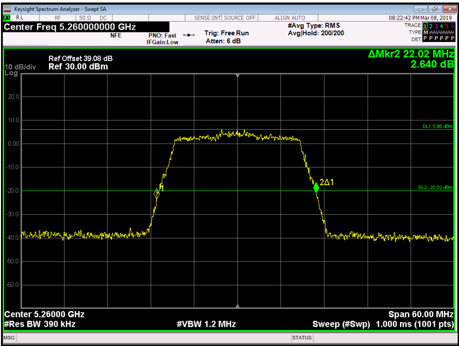
Figure 125 - 5260 MHz - 26 dB Emission Bandwidth
