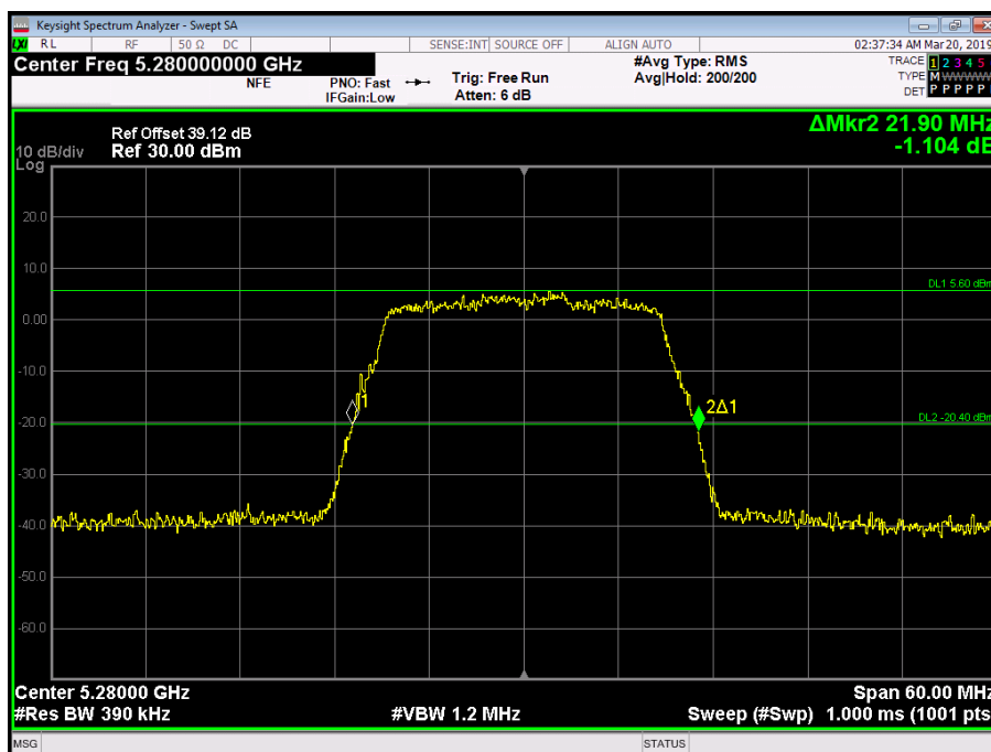
Figure 133 - 5280 MHz - 26 dB Emission Bandwidth
