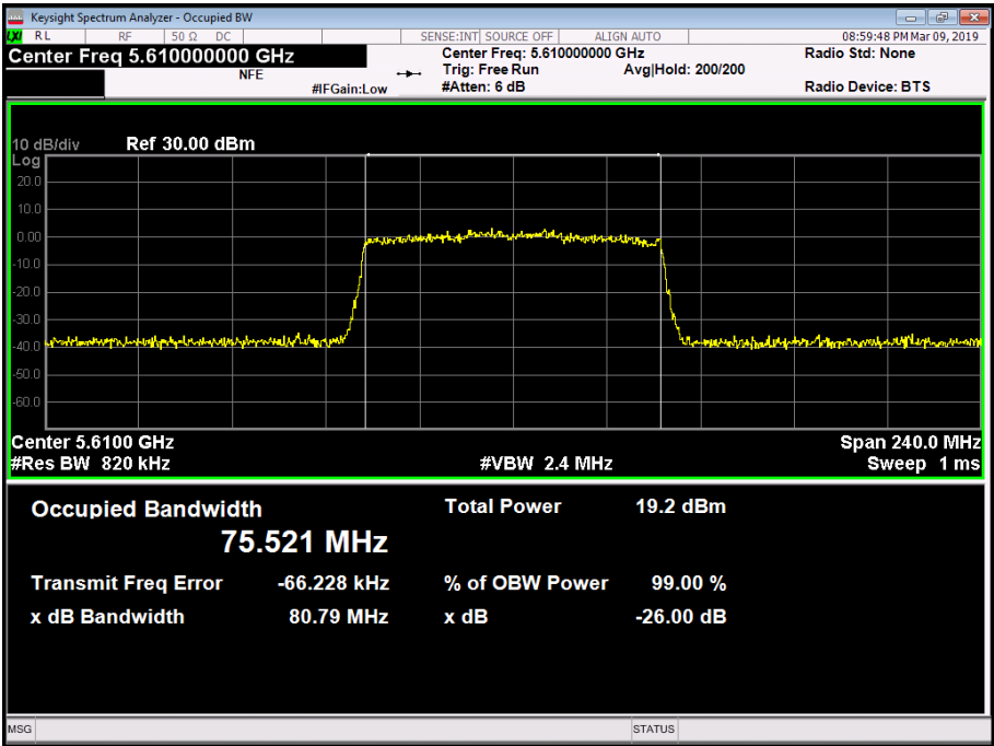
Figure 248 - 5610 MHz - 99% Occupied Bandwidth
