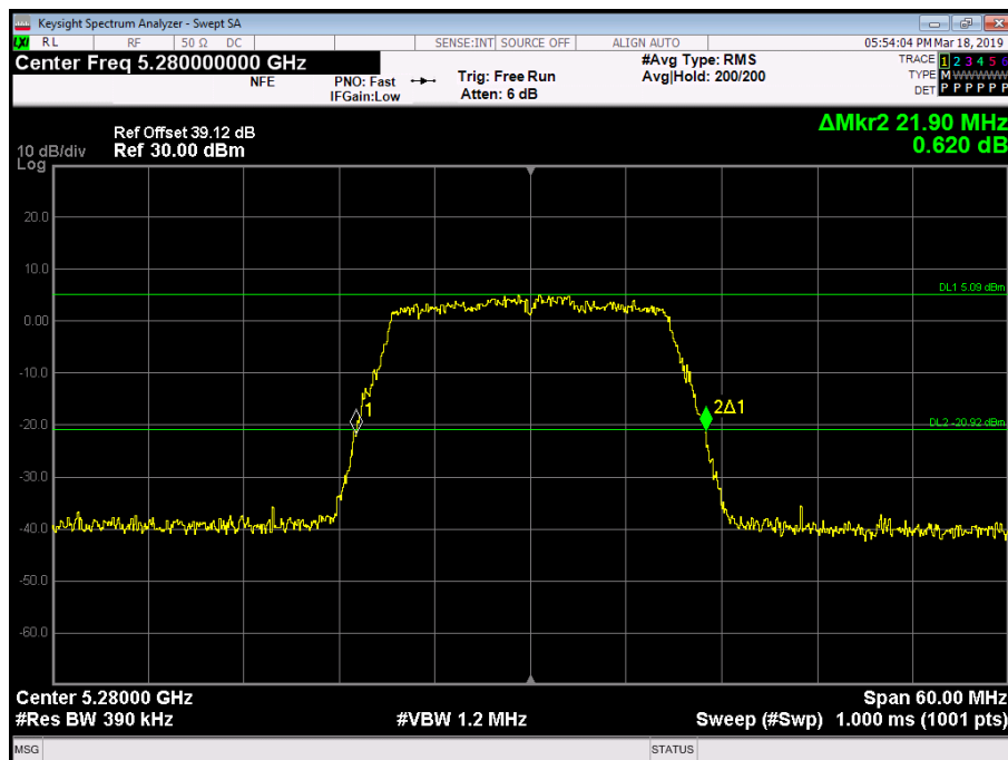
Figure 139 - 5280 MHz - 26 dB Emission Bandwidth
