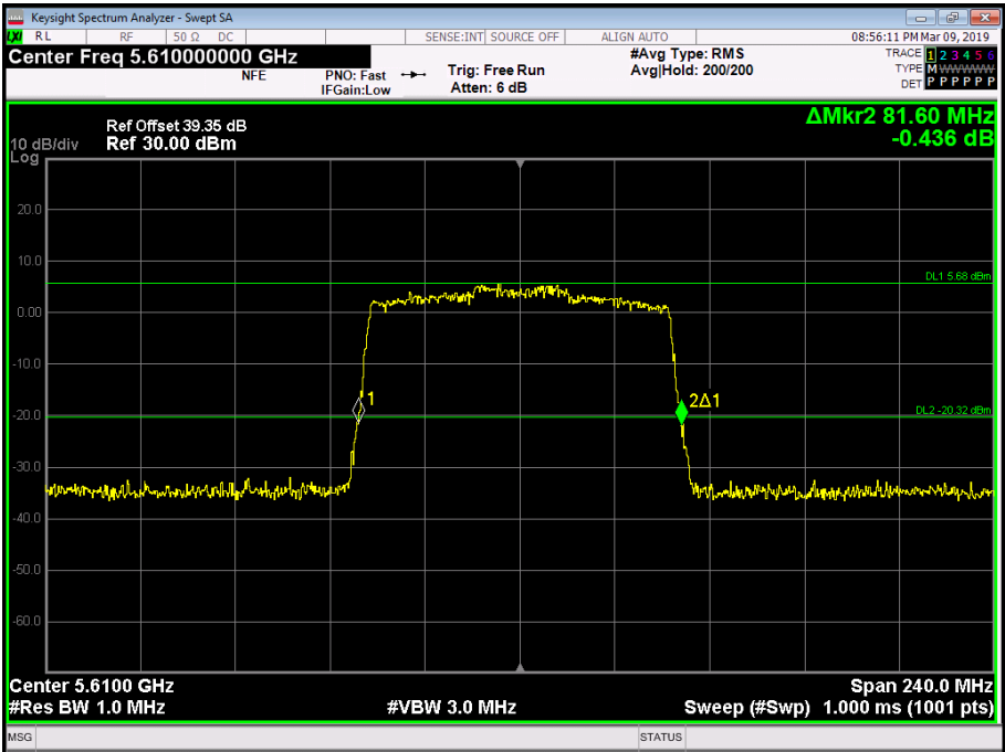
Figure 241 - 5610 MHz - 26 dB Emission Bandwidth
