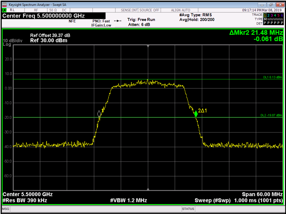
Figure 167 - 5500 MHz - 26 dB Emission Bandwidth
