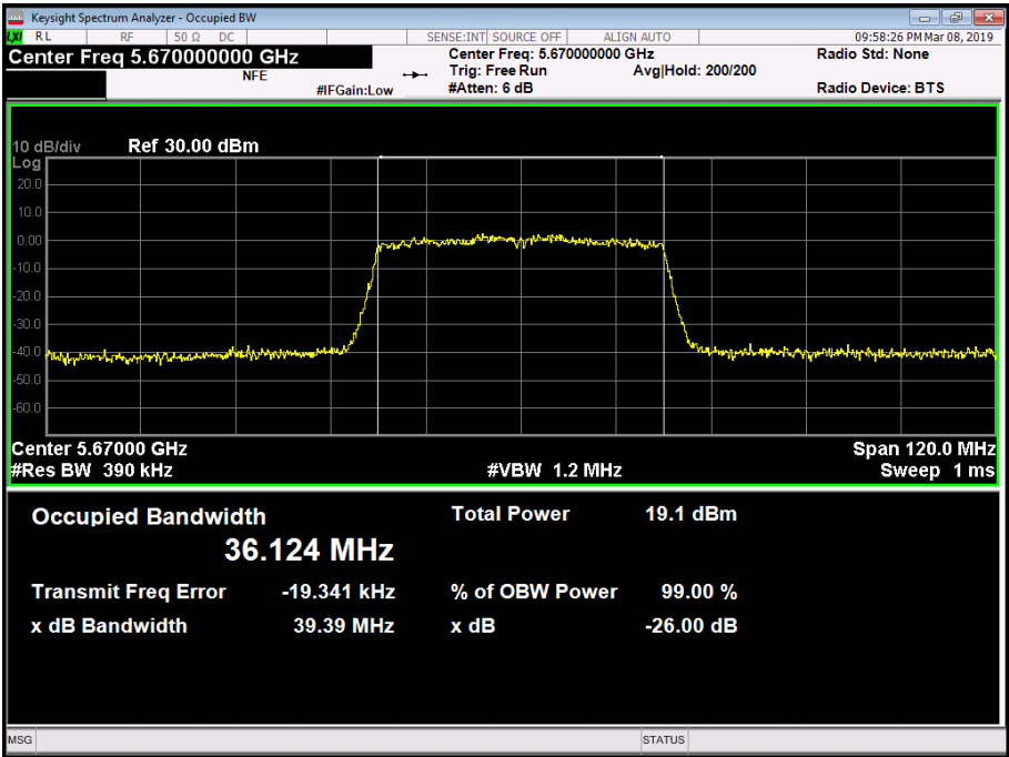
Figure 212 - 5670 MHz - 99% Occupied Bandwidth
