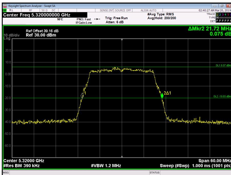
Figure 123 - 5320 MHz - 26 dB Emission Bandwidth
