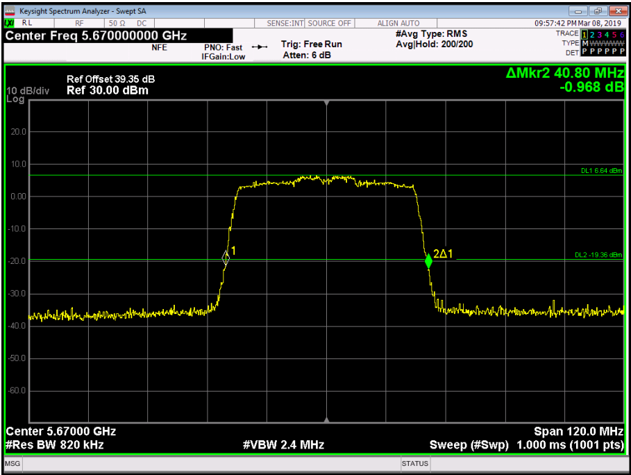
Figure 211 - 5670 MHz - 26 dB Emission Bandwidth
