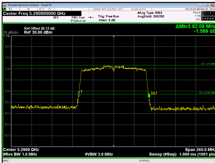
Figure 165 - 5290 MHz - 26 dB Emission Bandwidth
