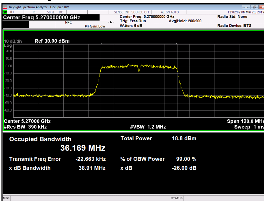
Figure 148 - 5270 MHz - 99% Occupied Bandwidth
