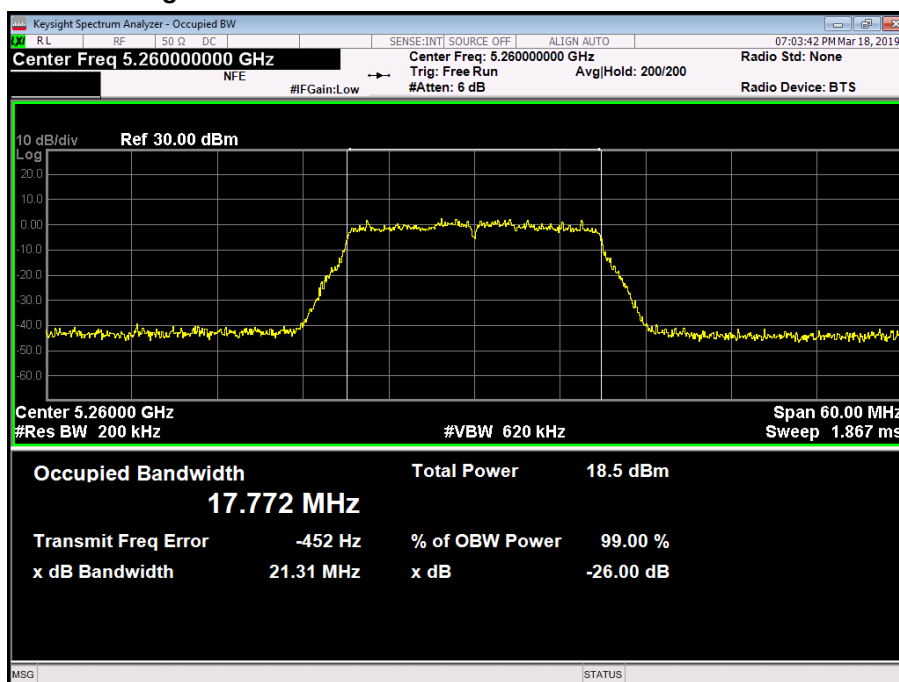
Figure 138 - 5260 MHz - 99% Occupied Bandwidth
