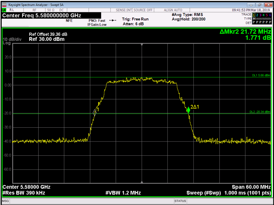
Figure 169 - 5580 MHz - 26 dB Emission Bandwidth
