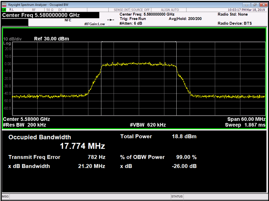
Figure 186 - 5580 MHz - 99% Occupied Bandwidth
