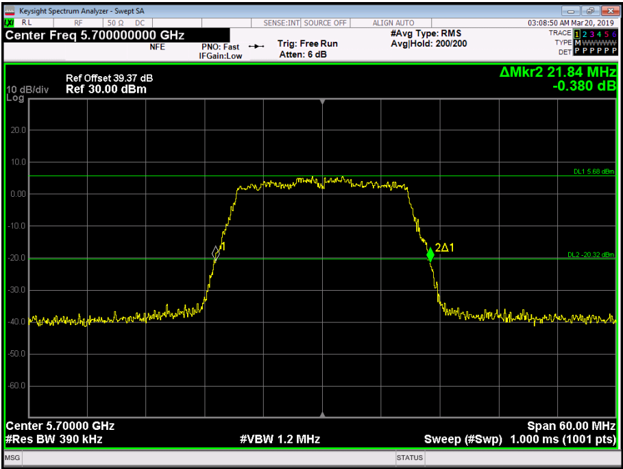
Figure 187 - 5700 MHz - 26 dB Emission Bandwidth
