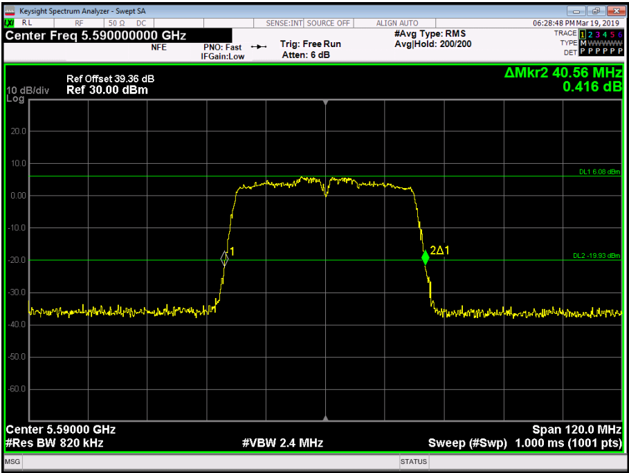
Figure 233 - 5590 MHz - 26 dB Emission Bandwidth
