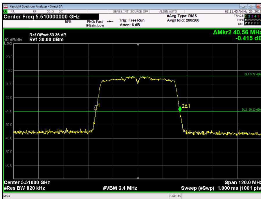
Figure 207 - 5510 MHz - 26 dB Emission Bandwidth
