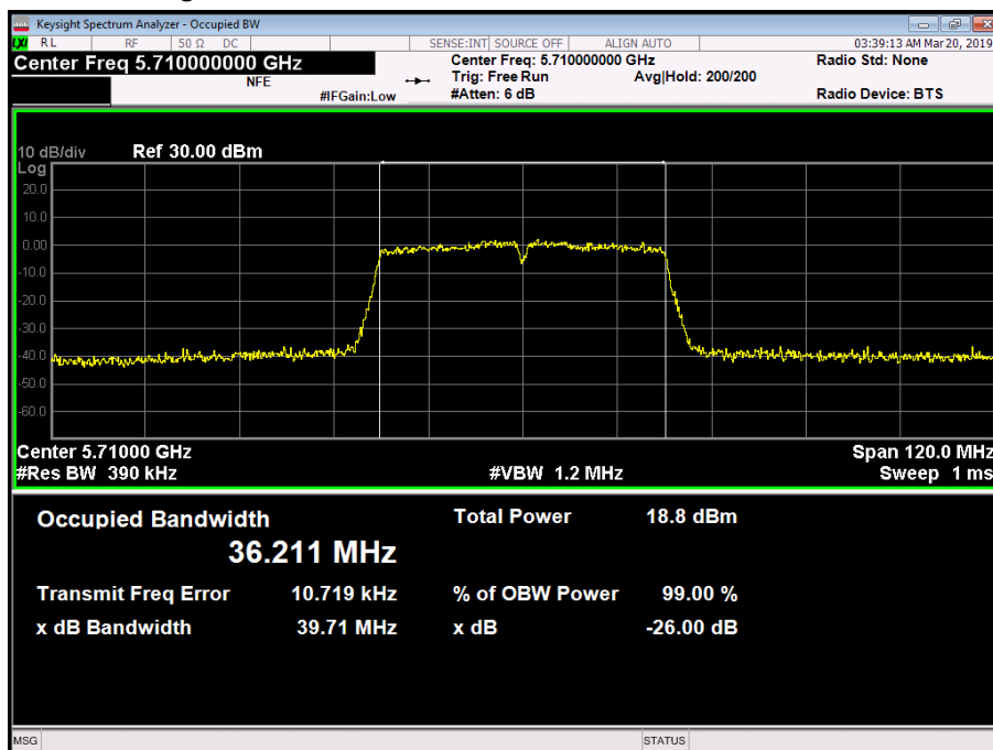
Figure 230 - 5710 MHz - 99% Occupied Bandwidth
