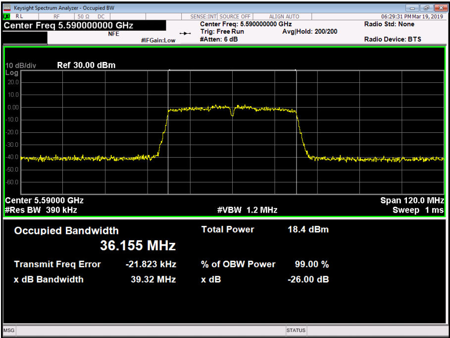
Figure 234 - 5590 MHz - 99% Occupied Bandwidth
