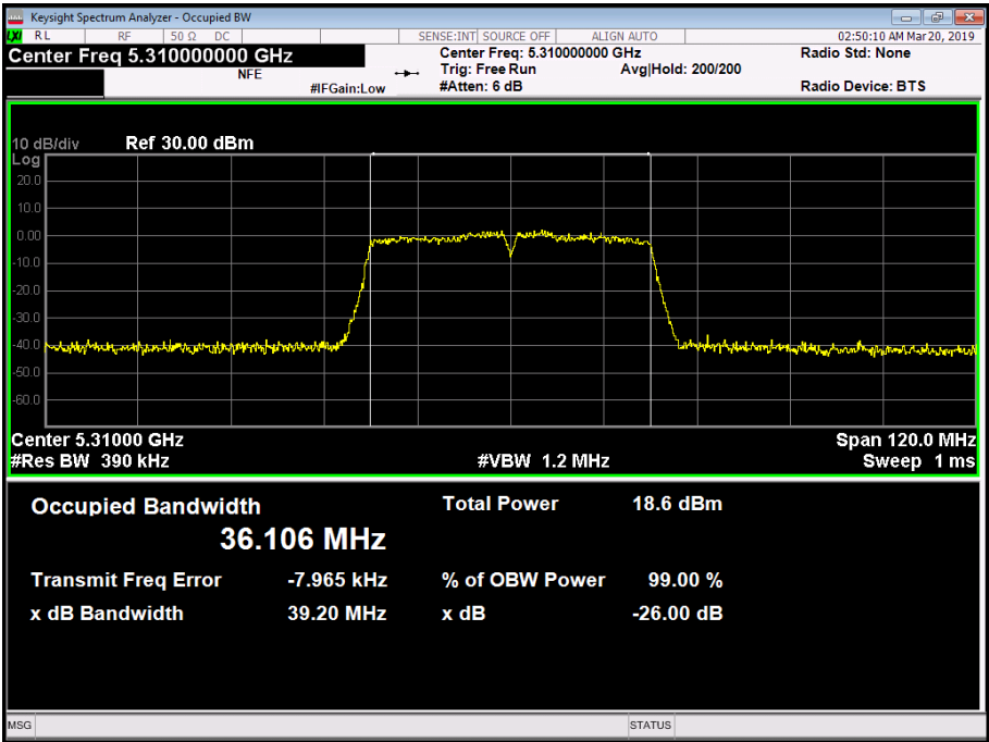
Figure 146 - 5310 MHz - 99% Occupied Bandwidth
