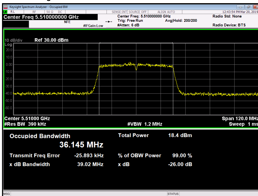
Figure 216 - 5510 MHz - 99% Occupied Bandwidth
