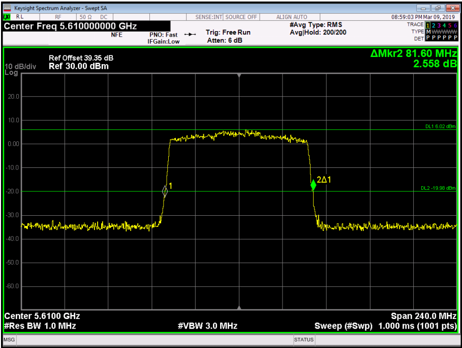
Figure 247 - 5610 MHz - 26 dB Emission Bandwidth
