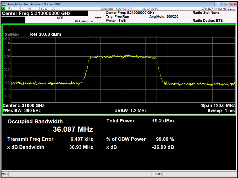
Figure 150 - 5310 MHz - 99% Occupied Bandwidth
