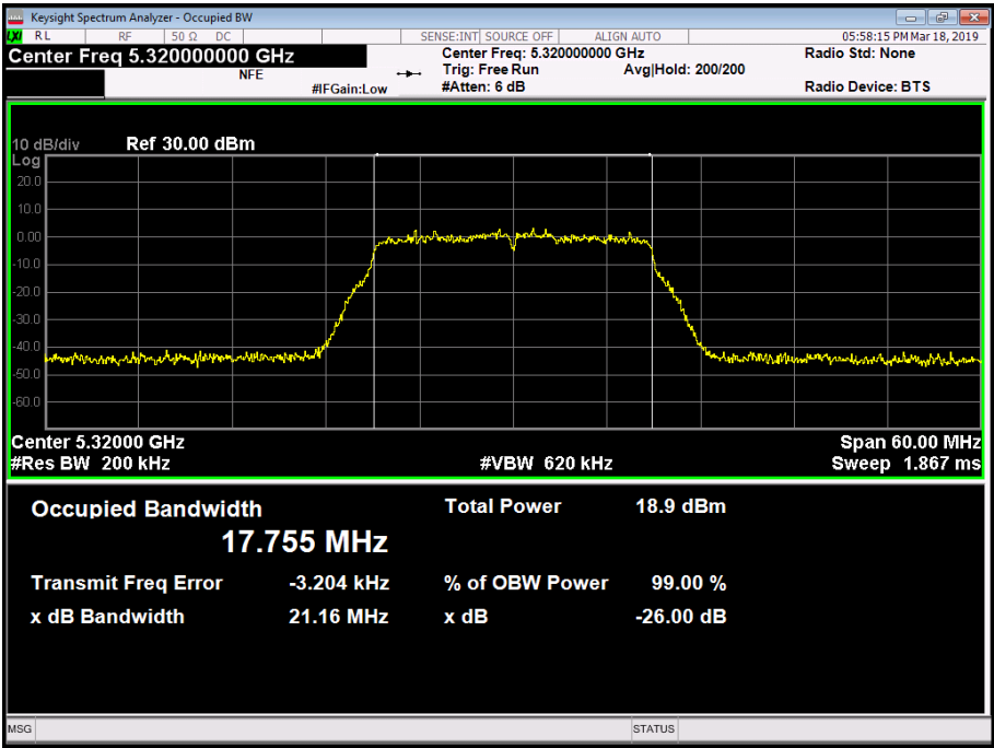
Figure 142 - 5320 MHz - 99% Occupied Bandwidth
