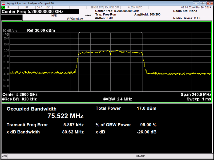
Figure 164 - 5290 MHz - 99% Occupied Bandwidth 802.11ac / VHT80 MCS0x1 / MIMO TxBF / Cores 0+1
