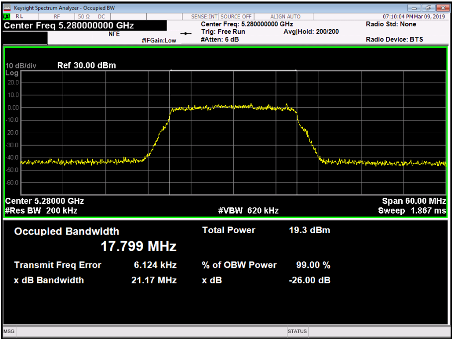
Figure 122 - 5280 MHz - 99% Occupied Bandwidth
