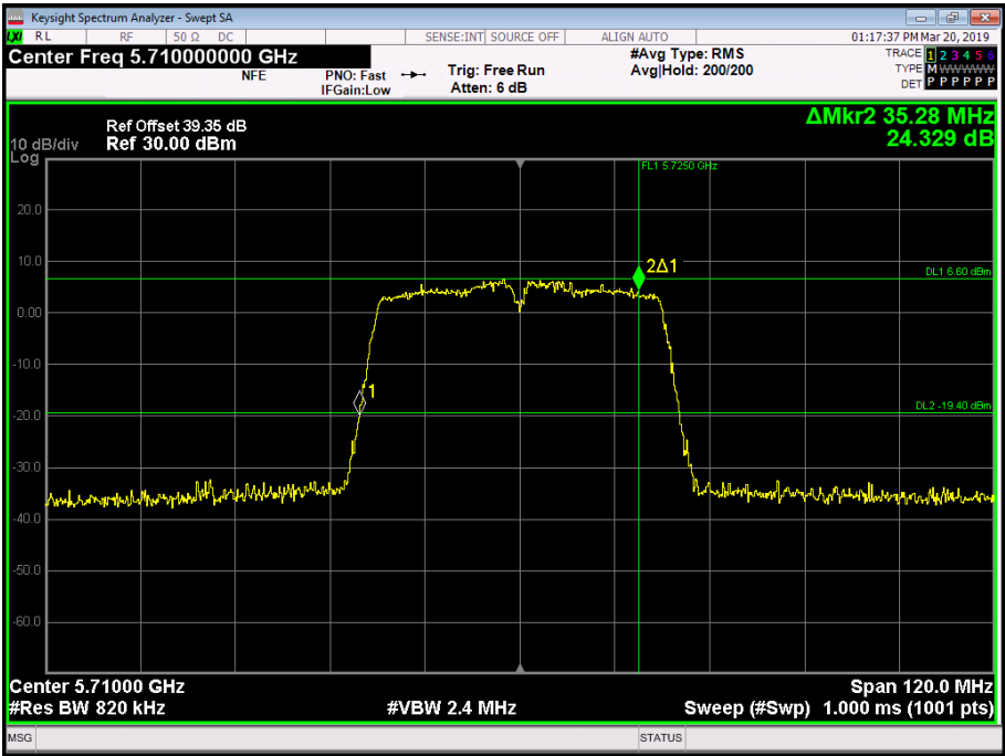
Figure 237 - 5710 MHz - 26 dB Emission Bandwidth
