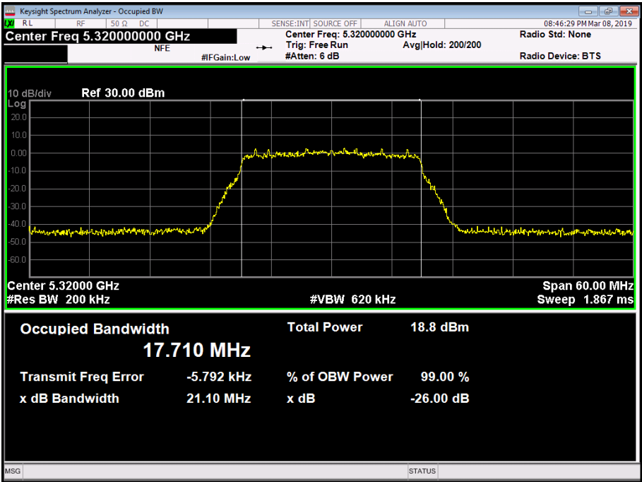
Figure 130 - 5320 MHz - 99% Occupied Bandwidth
