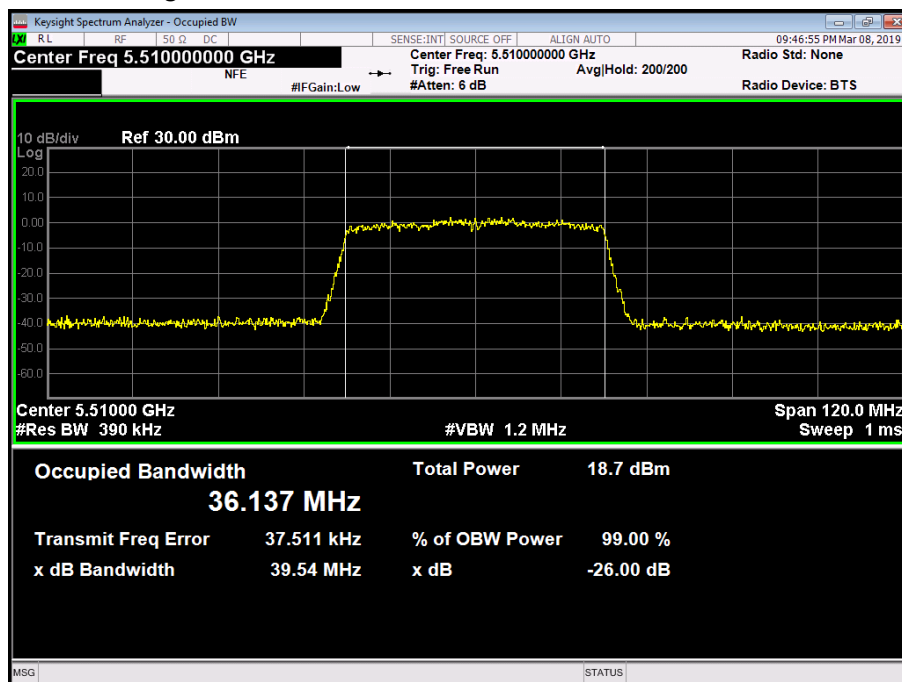
Figure 224 - 5510 MHz - 99% Occupied Bandwidth
