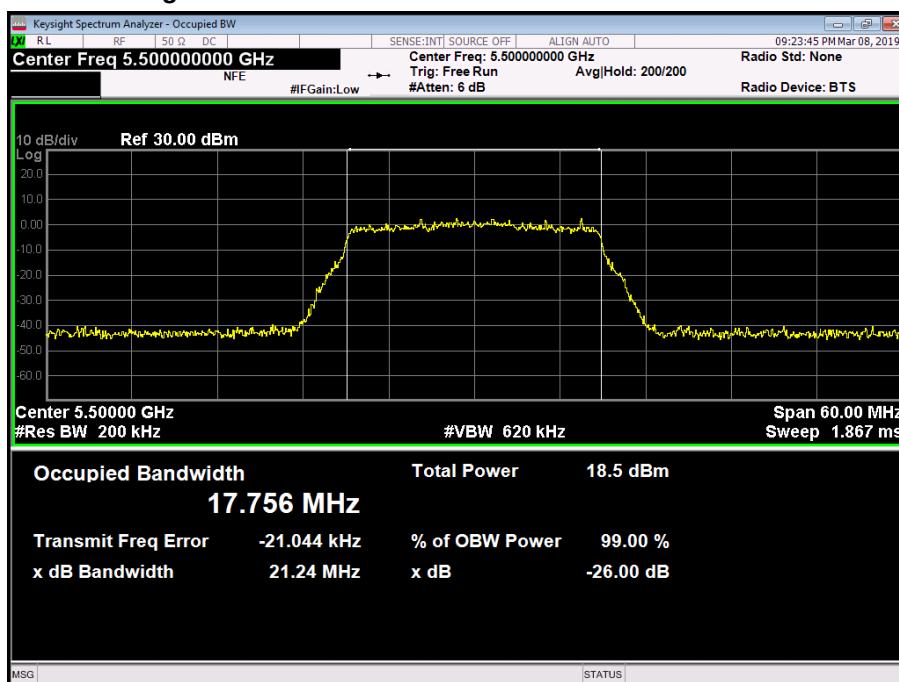
Figure 184 - 5500 MHz - 99% Occupied Bandwidth
