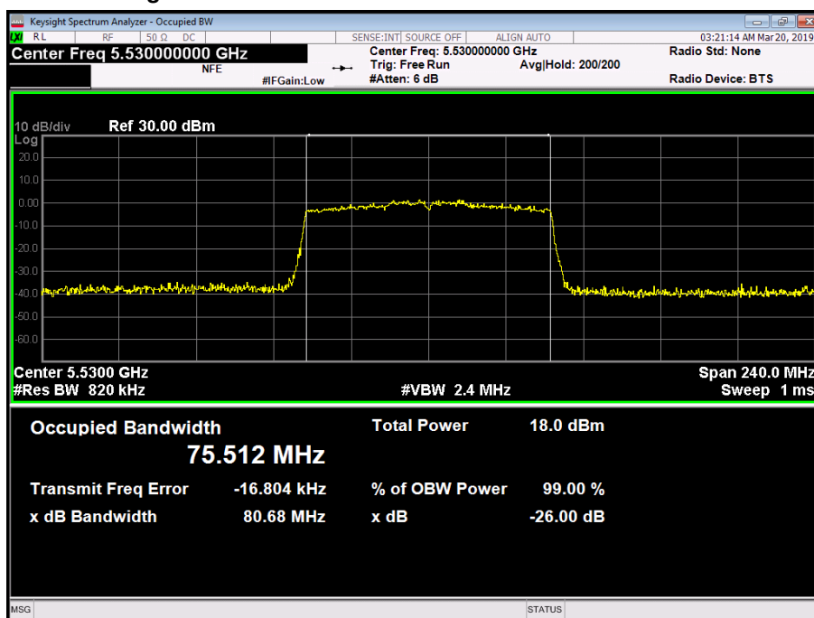
Figure 240 - 5530 MHz - 99% Occupied Bandwidth
