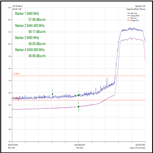
Figure 453 – Channel 100 – Restricted Band Edge
